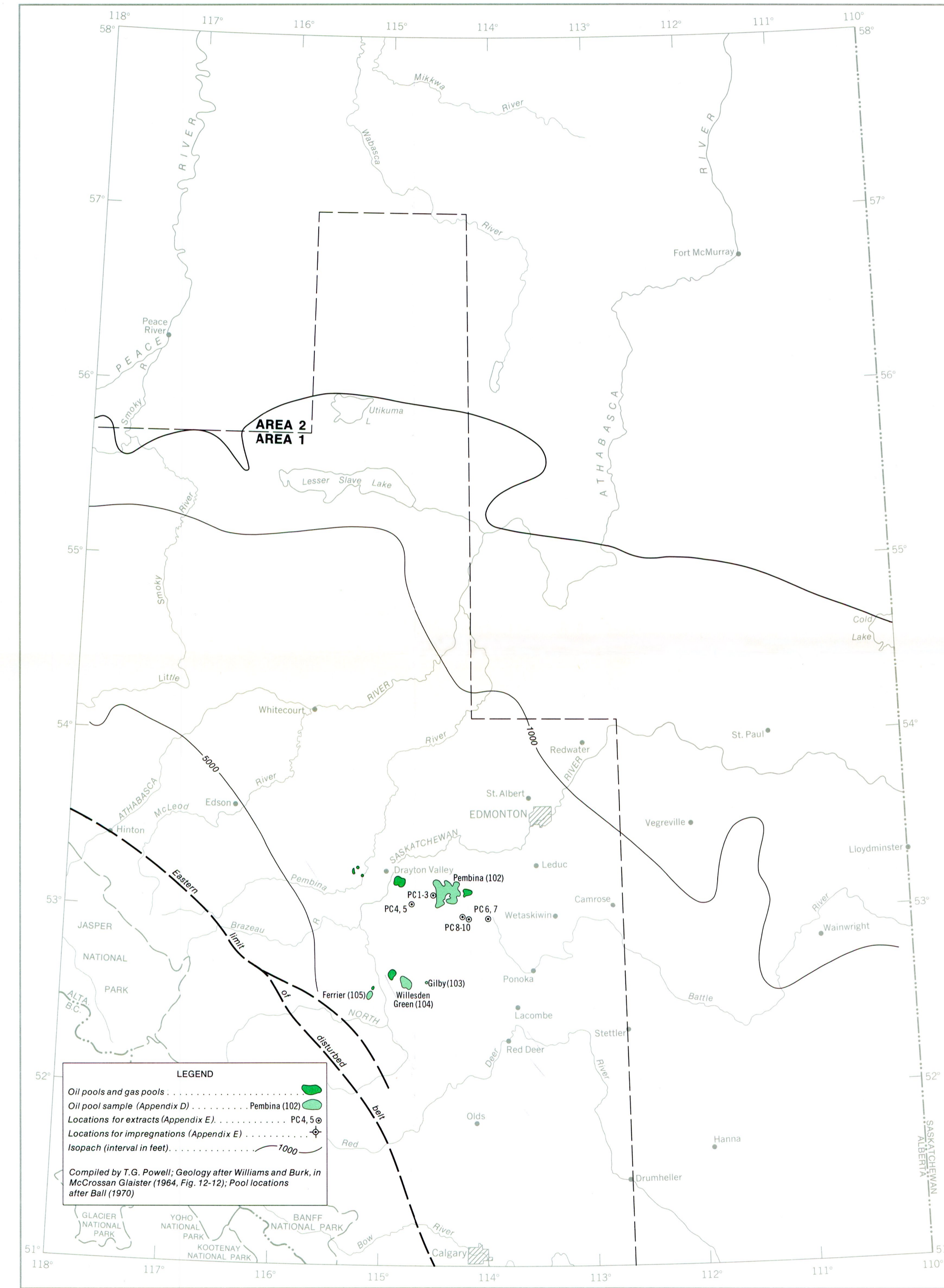
Figure 2-14. Generalized isopach map of the post-Coloredo Group within the study-area showing the distribution of oil and gas pools and sample locations in the post-Coloredo Group (after McCrossan and Glaister, 1964)
