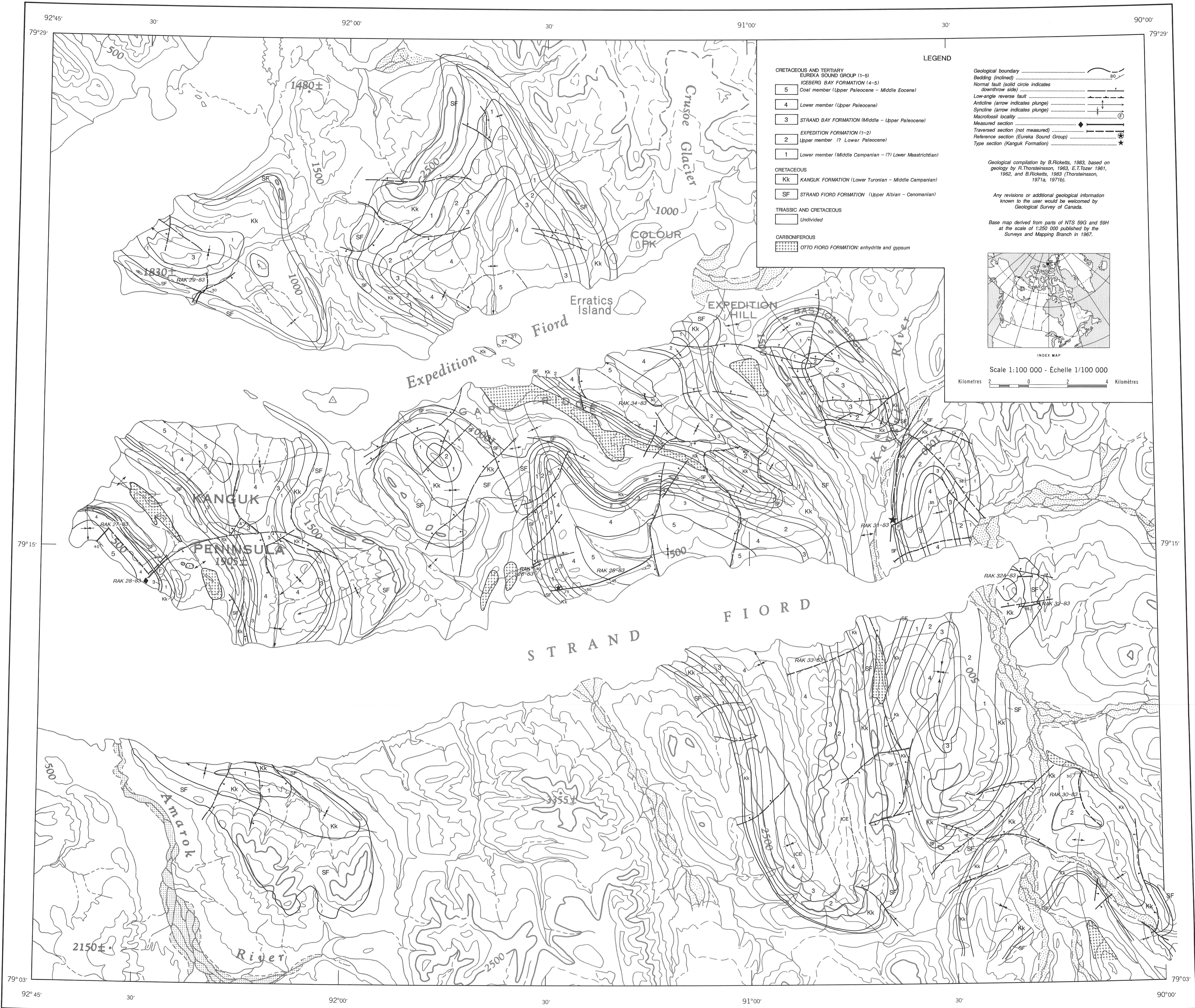
Figure 2. Geological map of the Upper Cretaceous and Tertiary, Strand and Expedition fiords, Axel Heiberg Island.
