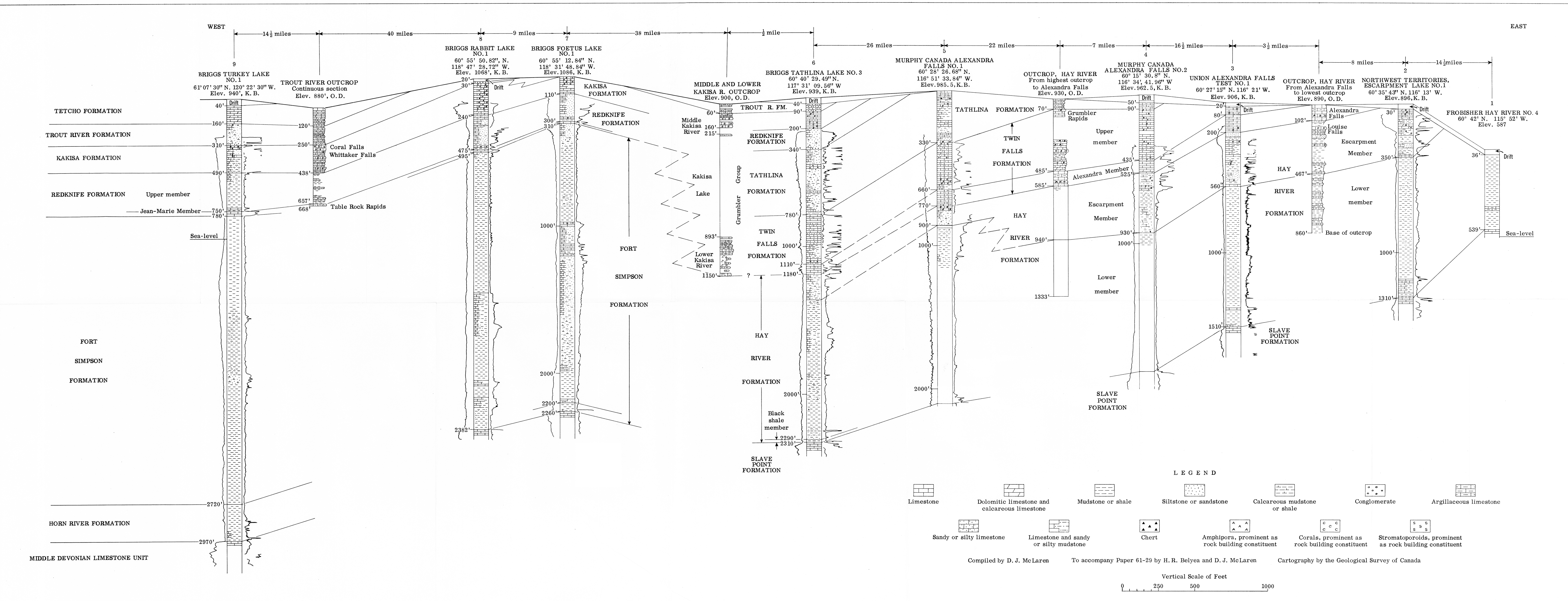
Figure 3. East-west cross-section showing wells between Frobisher Hay River No. 4. and Briggs Turkey Lake No. 1
