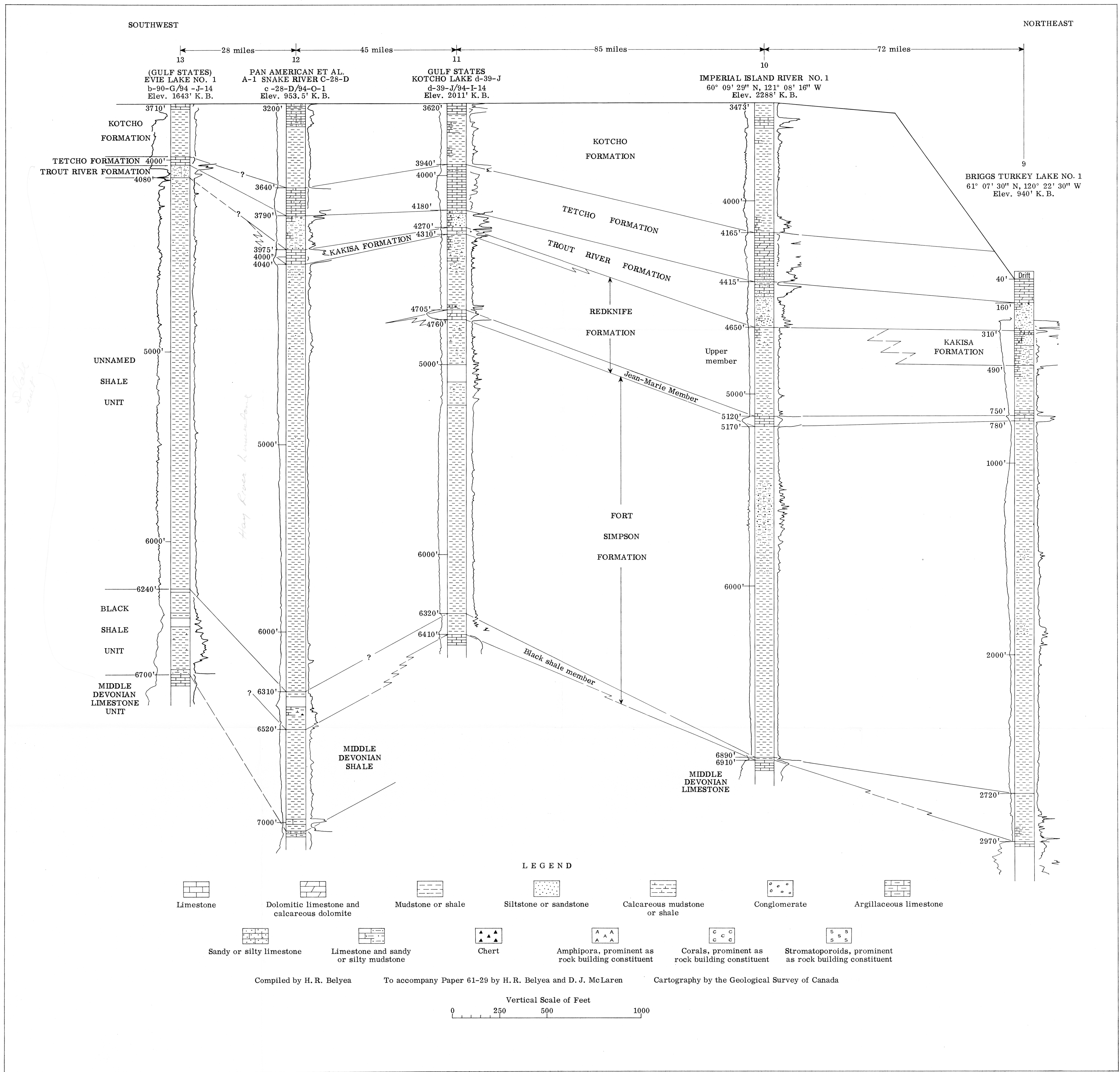
Figure 4. Northeast-southwest cross-section showing wells between Briggs Turkey Lake No.1 and (Gulf States) Evie Lake No.1
