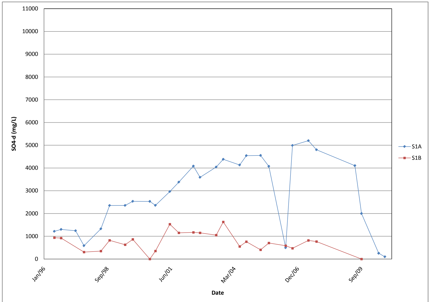
Figure 6-3: S-Wells Area Sulfate Concentration (Dissolved) S1A+B (1996-2010)
