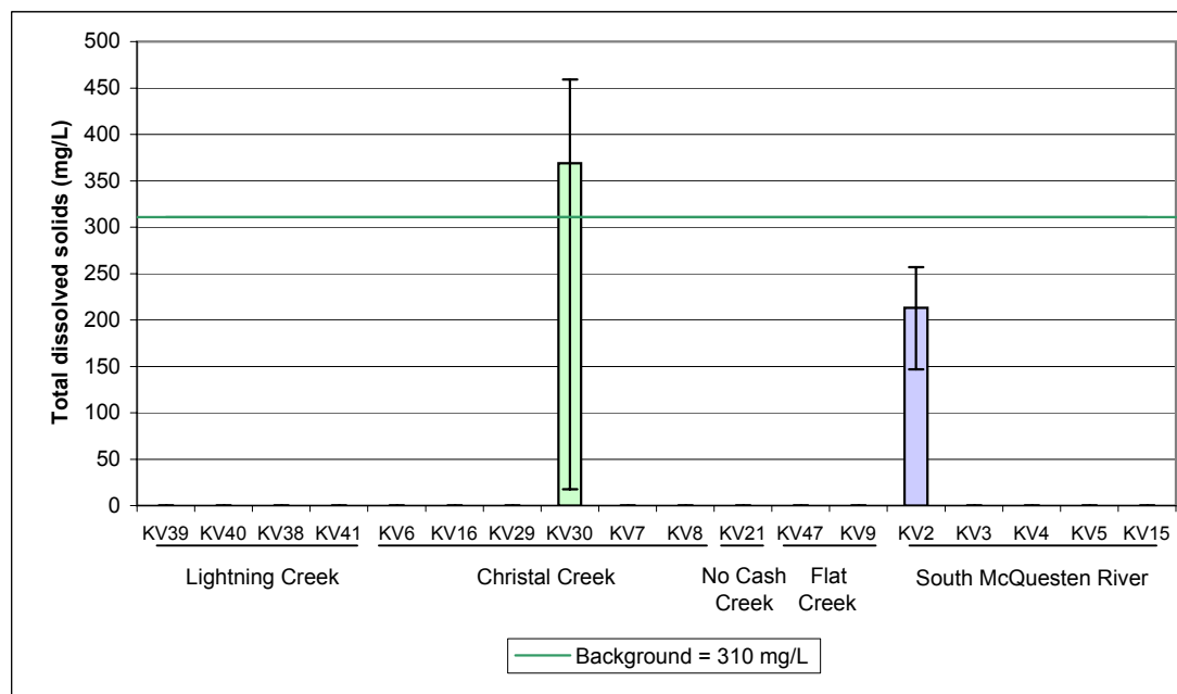
Figure A.45: Total Dissolved Solids (mg/L) Median Values with Minimum and Maximum for Receiving Environment Stations, 1994 - 2007.
