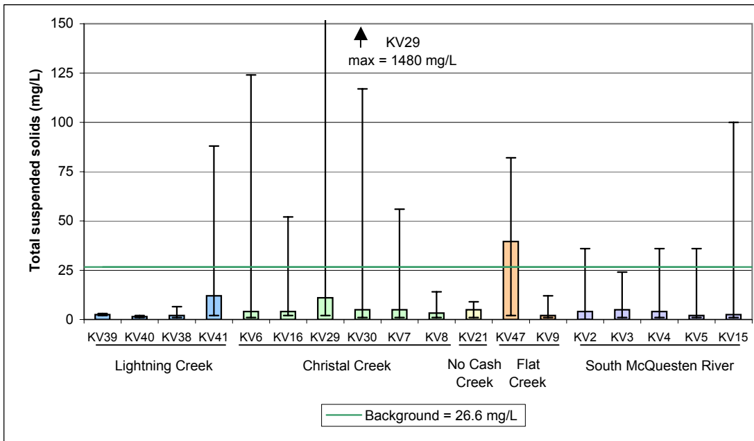
Figure A.46: Total Suspended Solids (mg/L) Median Values with Minimum and Maximum for Receiving Environment Stations, 1994 - 2007.
