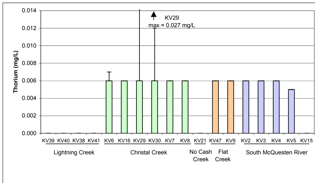
Figure A.42: Thorium (mg/L) Median Values with Minimum and Maximum for Receiving Environment Stations, July 20, 2004 - 2007.
