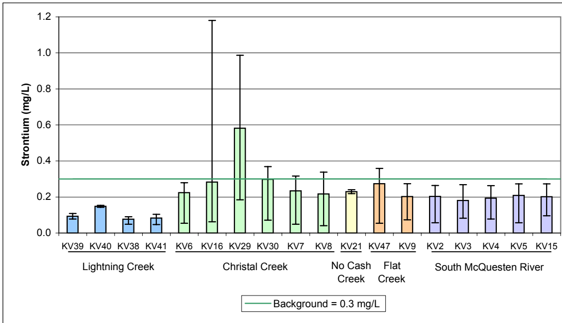
Figure A.38: Strontium (mg/L) Median Values with Minimum and Maximum for Receiving Environment Stations, 1994 - 2007.
