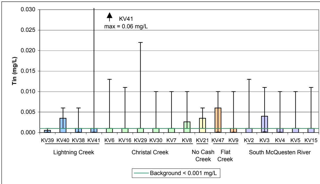
Figure A.43: Tin (mg/L) Median Values with Minimum and Maximum for Receiving Environment Stations, 1994 - 2007.
