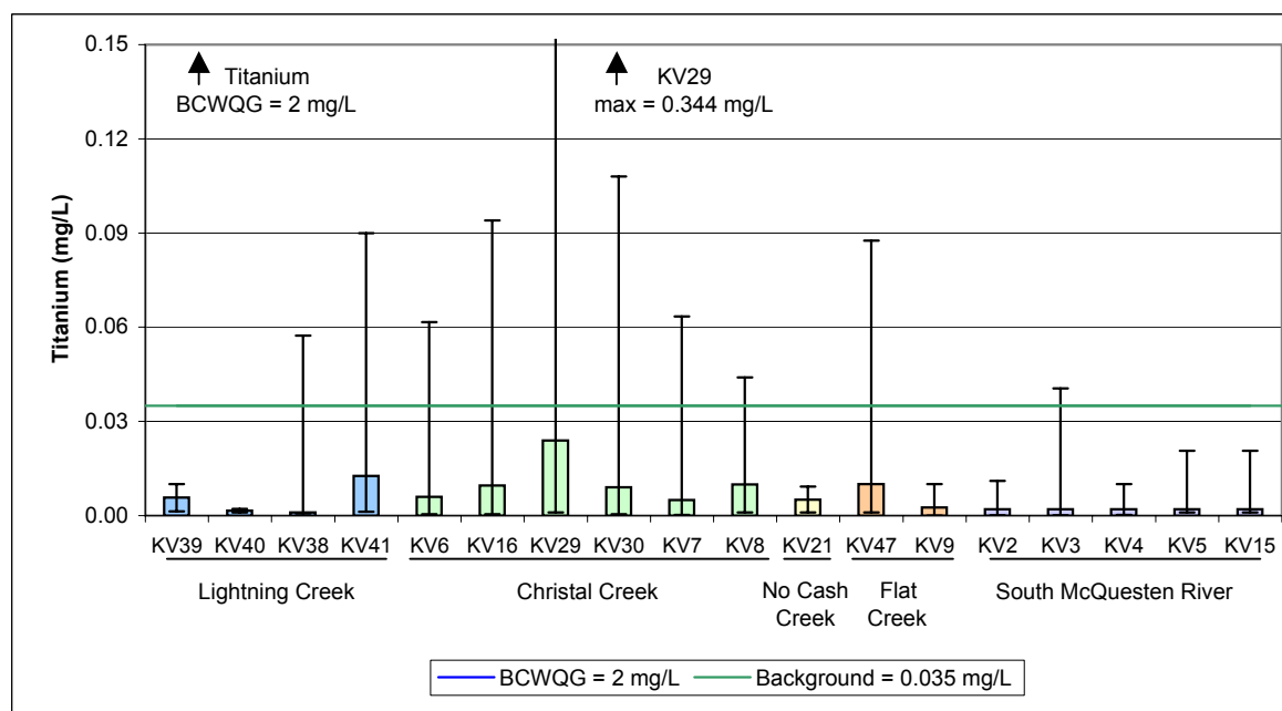
Figure A.44: Titanium (mg/L) Median Values with Minimum and Maximum for Receiving Environment Stations, 1994 - 2007.
