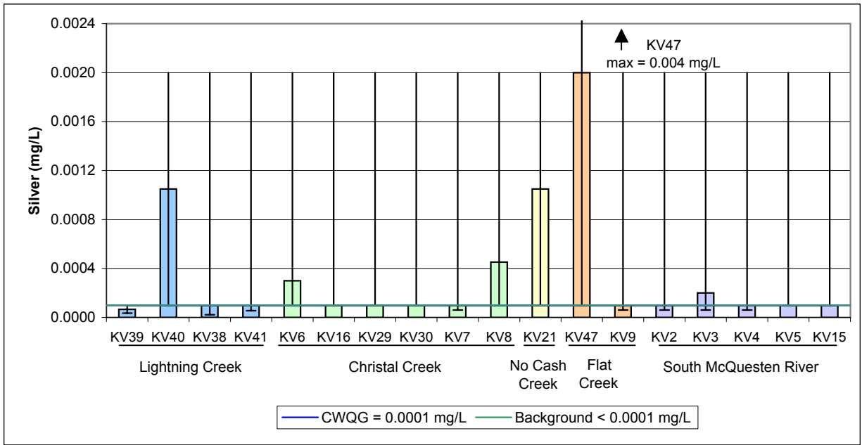
Figure A.36: Silver (mg/L) Median Values with Minimum and Maximum for Receiving Environment Stations, 1994 - 2007.
