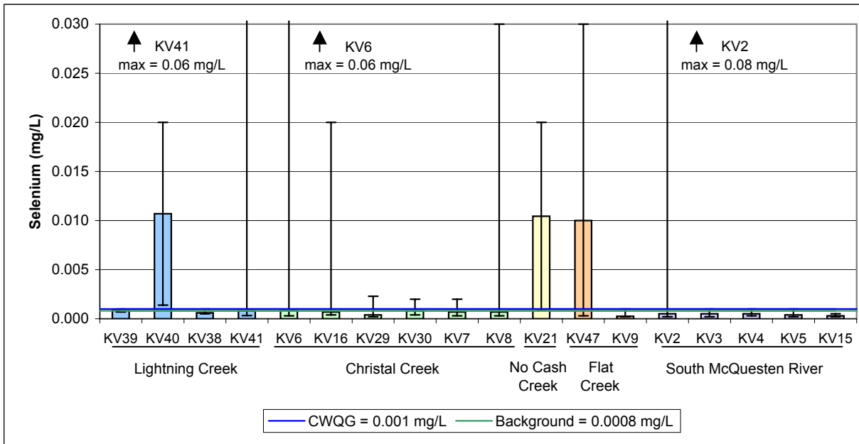
Figure A.34: Selenium (mg/L) Median Values with Minimum and Maximum for Receiving Environment Stations, 1994 - 2007.
