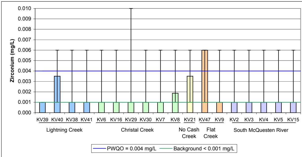
Figure A.50: Zirconium (mg/L) Median Values with Minimum and Maximum for Receiving Environment Stations, 1994 - 2007.
