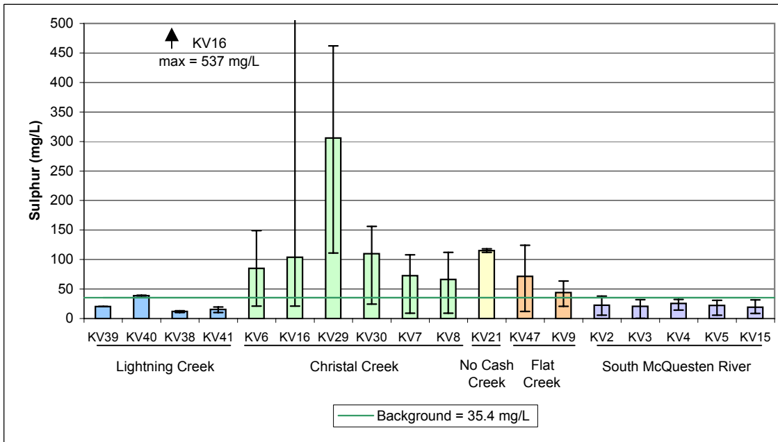
Figure A.40: Sulphur (mg/L) Median Values with Minimum and Maximum for Receiving Environment Stations, 1994 - 2007.
