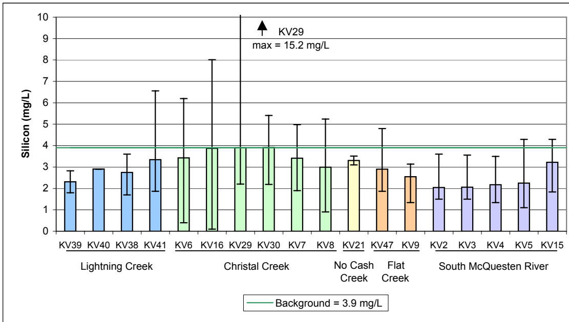
Figure A.35: Silicon (mg/L) Median Values with Minimum and Maximum for Receiving Environment Stations, 1994 - 2007.
