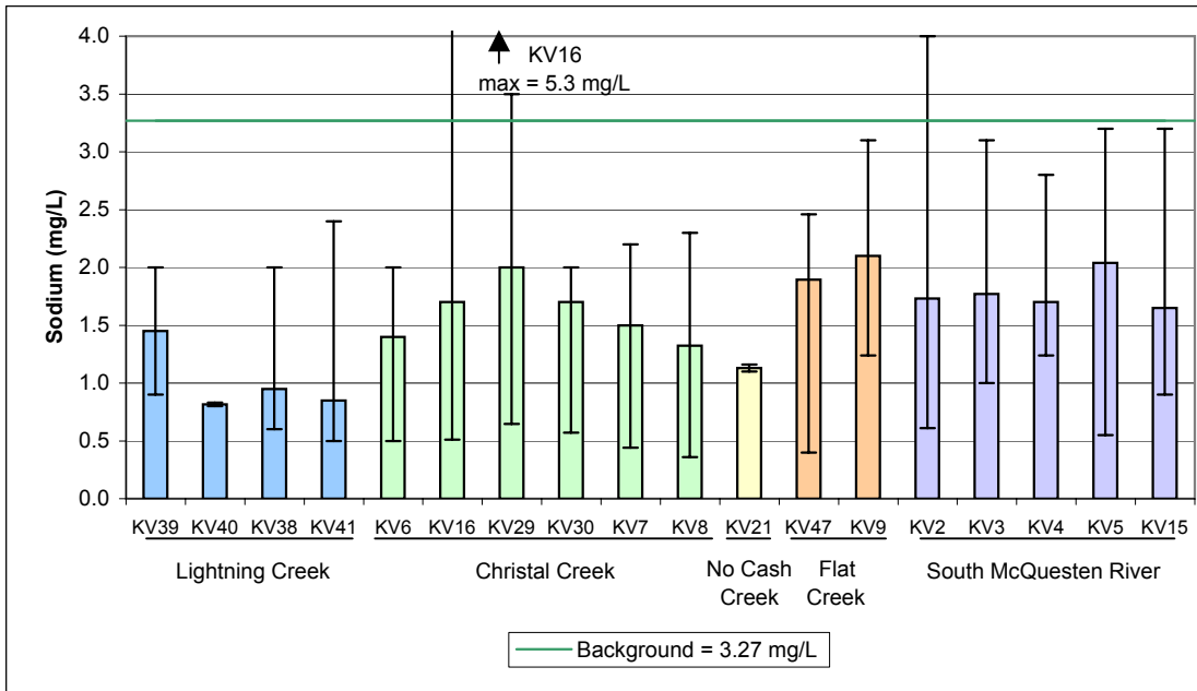
Figure A.37: Sodium (mg/L) Median Values with Minimum and Maximum for Receiving Environment Stations, 1994 - 2007.
