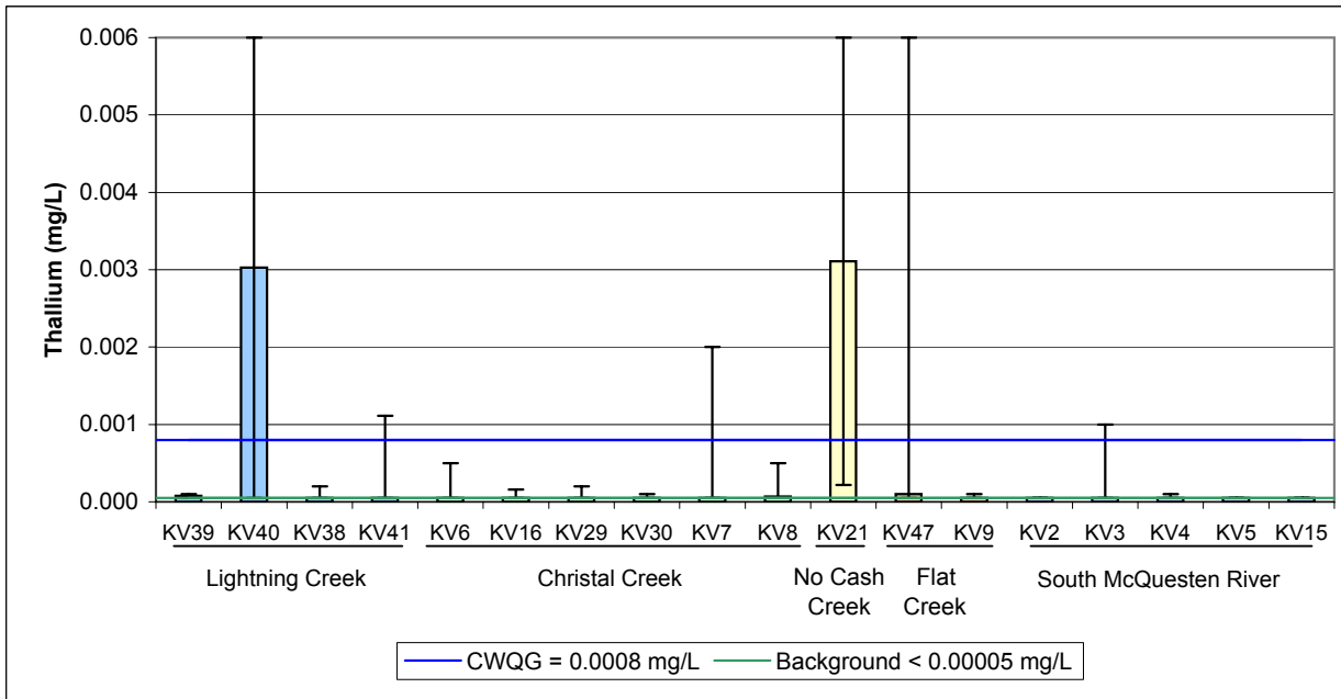
Figure A.41: Thallium (mg/L) Median Values with Minimum and Maximum for Receiving Environment Stations, 1994 - 2007.
