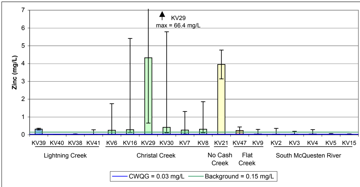
Figure A.49: Zinc (mg/L) Median Values with Minimum and Maximum for Receiving Environment Stations, 1994 - 2007.
