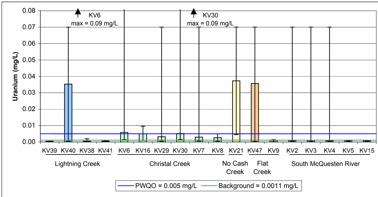
Figure A.47: Uranium (mg/L) Median Values with Minimum and Maximum for Receiving Environment Stations, 1994 - 2007.
