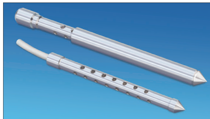
Model 615 Drive-Point and Shielded Drive-Point Piezometer
