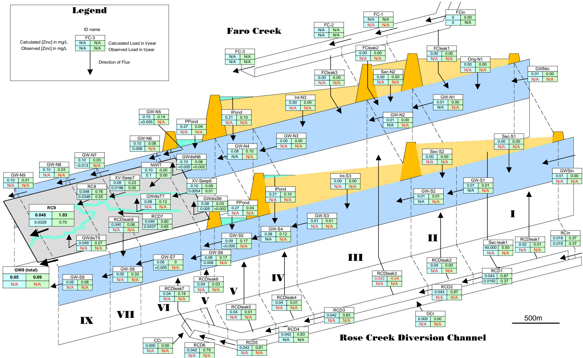
Figure 4.11 Zinc Load Balance for Rose Creek Valley - Scenario C1a (R=7).
