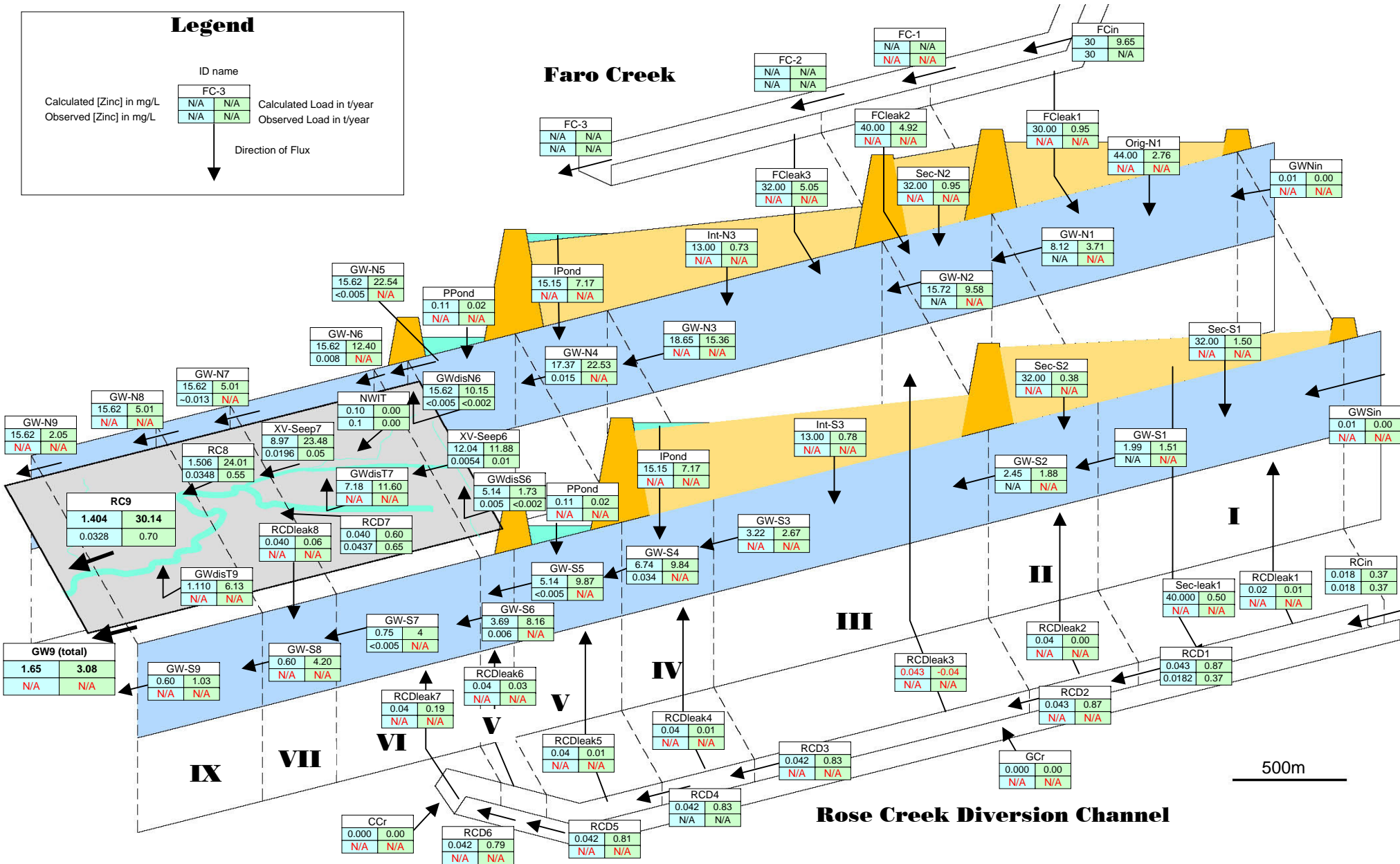
Figure 4.9 Zinc Load Balance for Rose Creek Valley - Scenario C1 (R=1).
