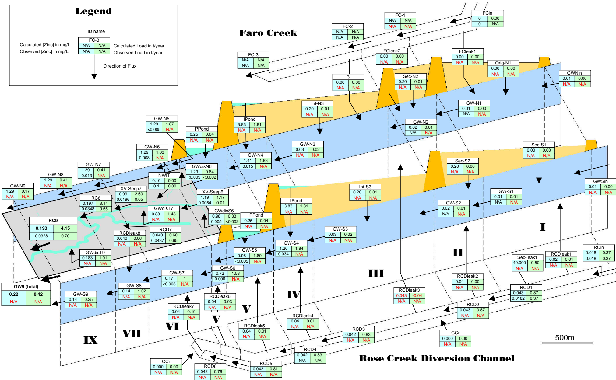
Figure 4.10 Zinc Load Balance for Rose Creek Valley - Scenario C1a (R=2).
