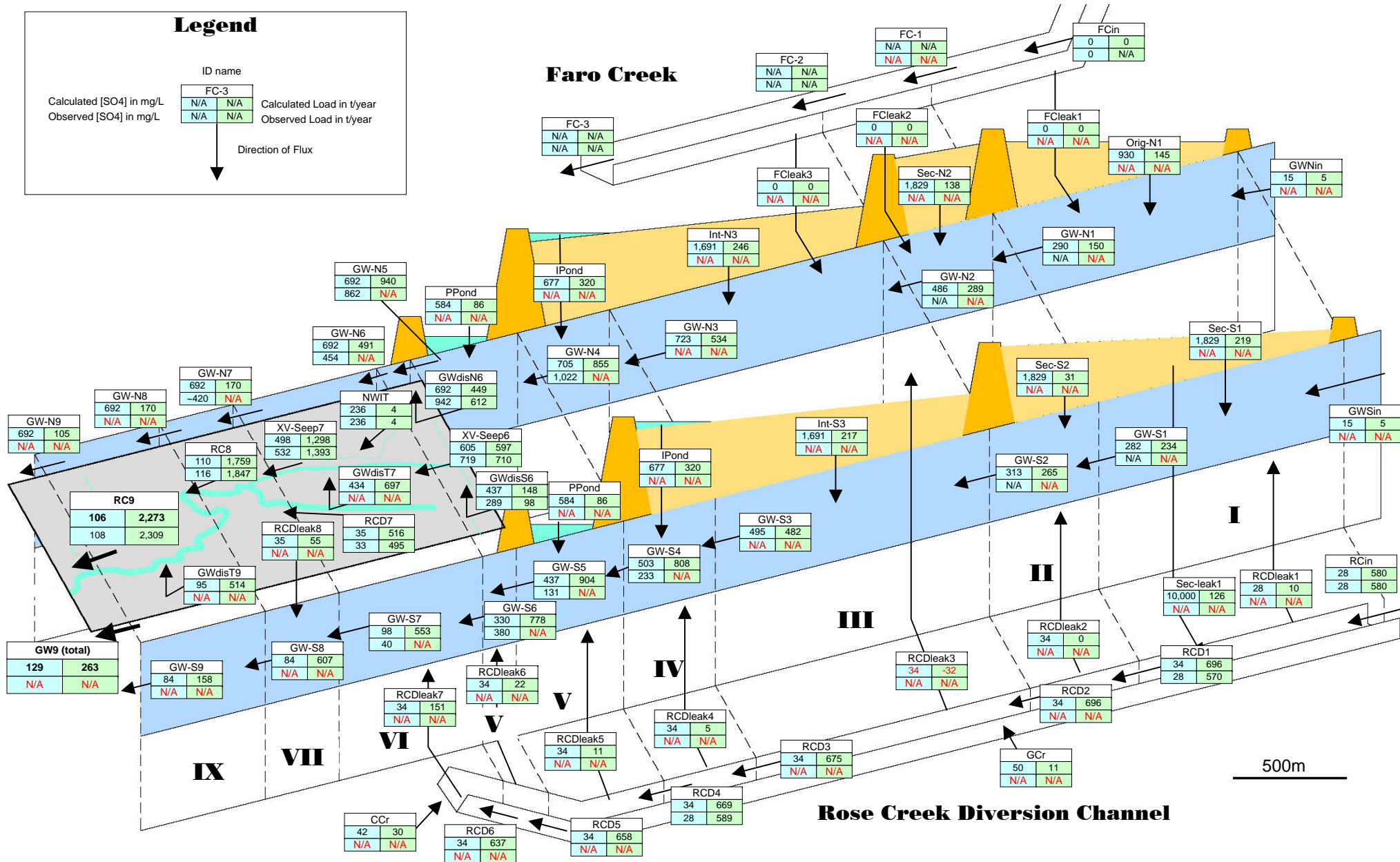
Figure 4.7 Sulphate Load Balance for Rose Creek Valley - Scenario C3.
