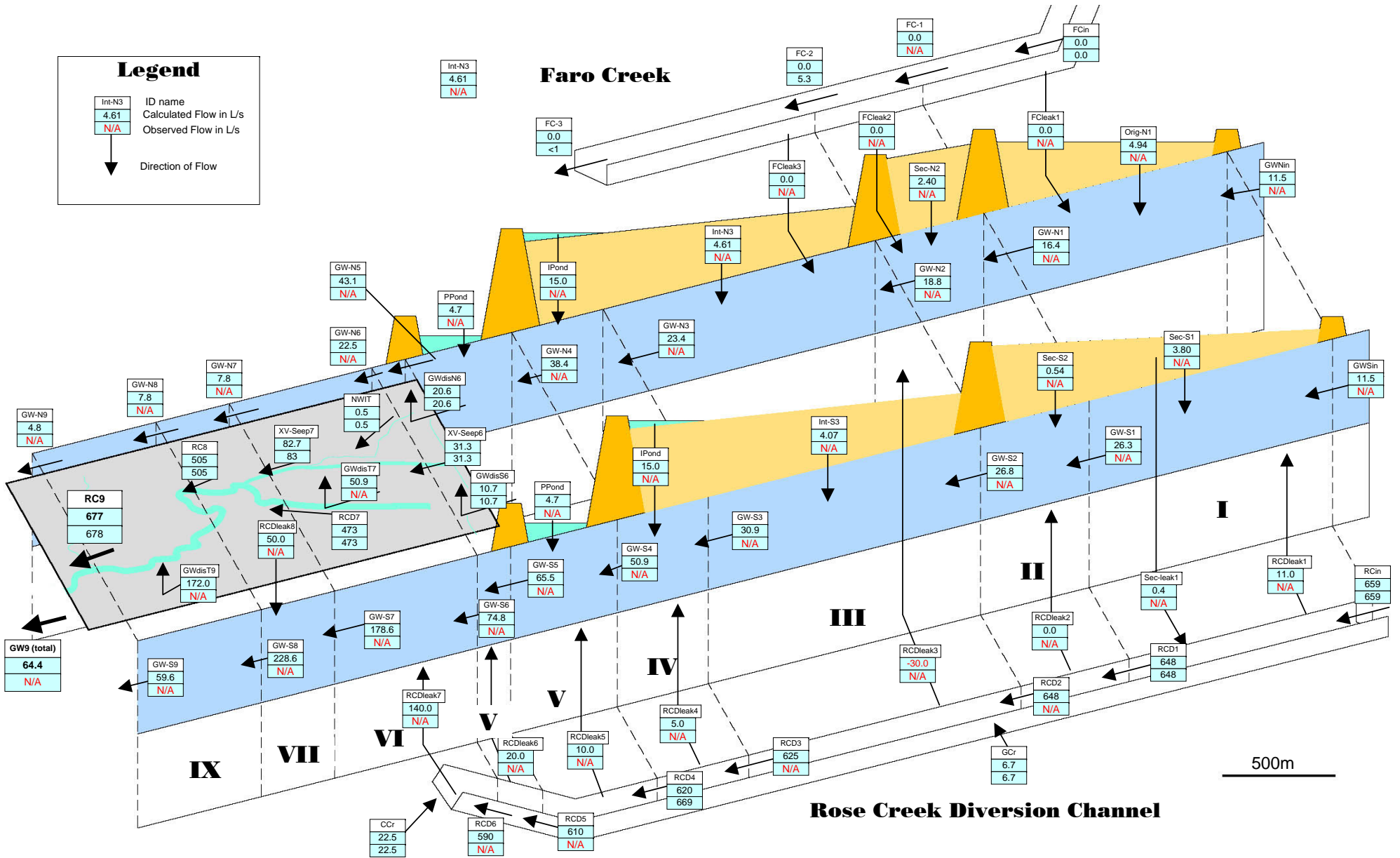
Figure 4.3 Water Balance for Rose Creek Valley - Scenario C3.
