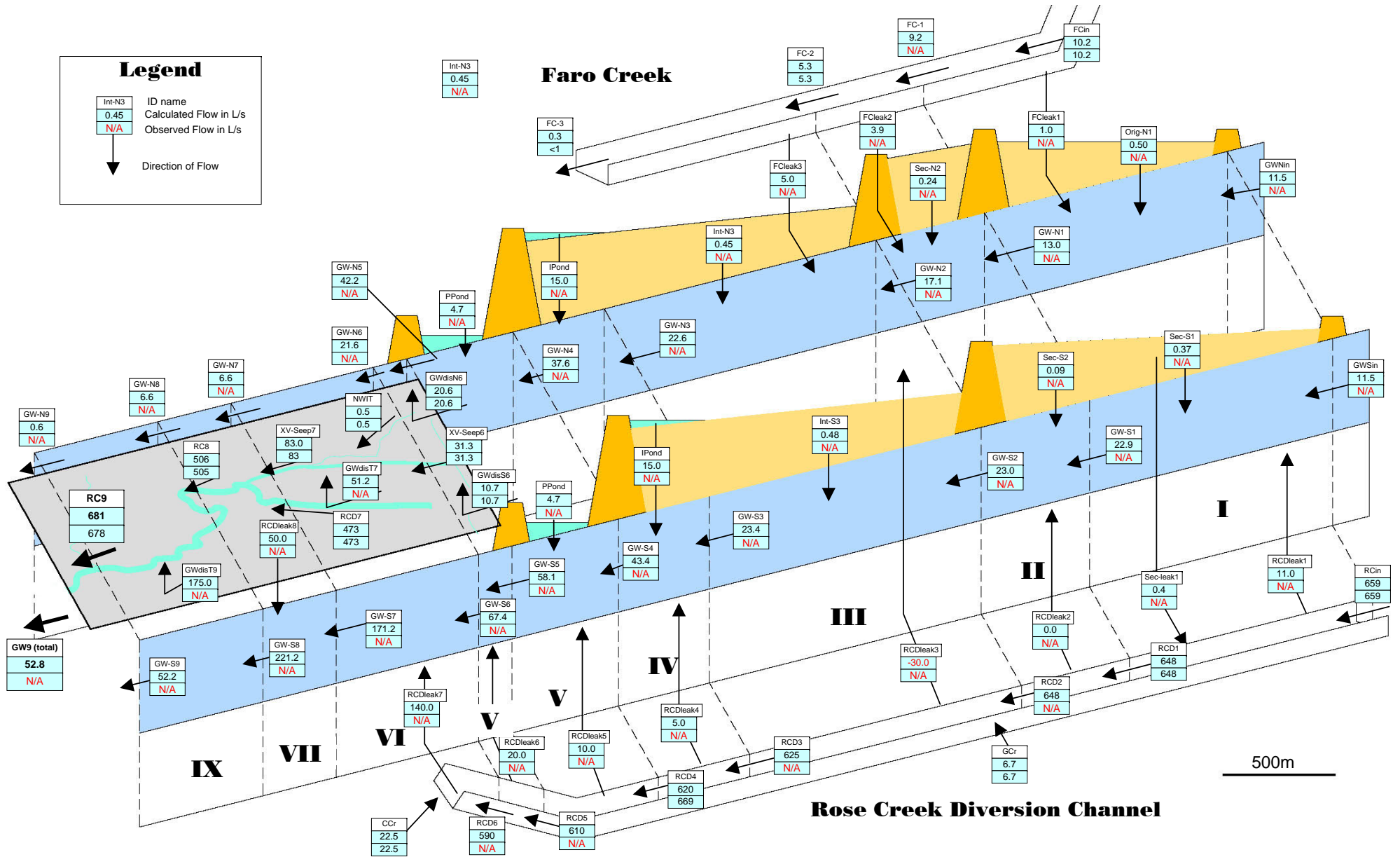
Figure 4.2 Water Balance for Rose Creek Valley - Scenario C2.
