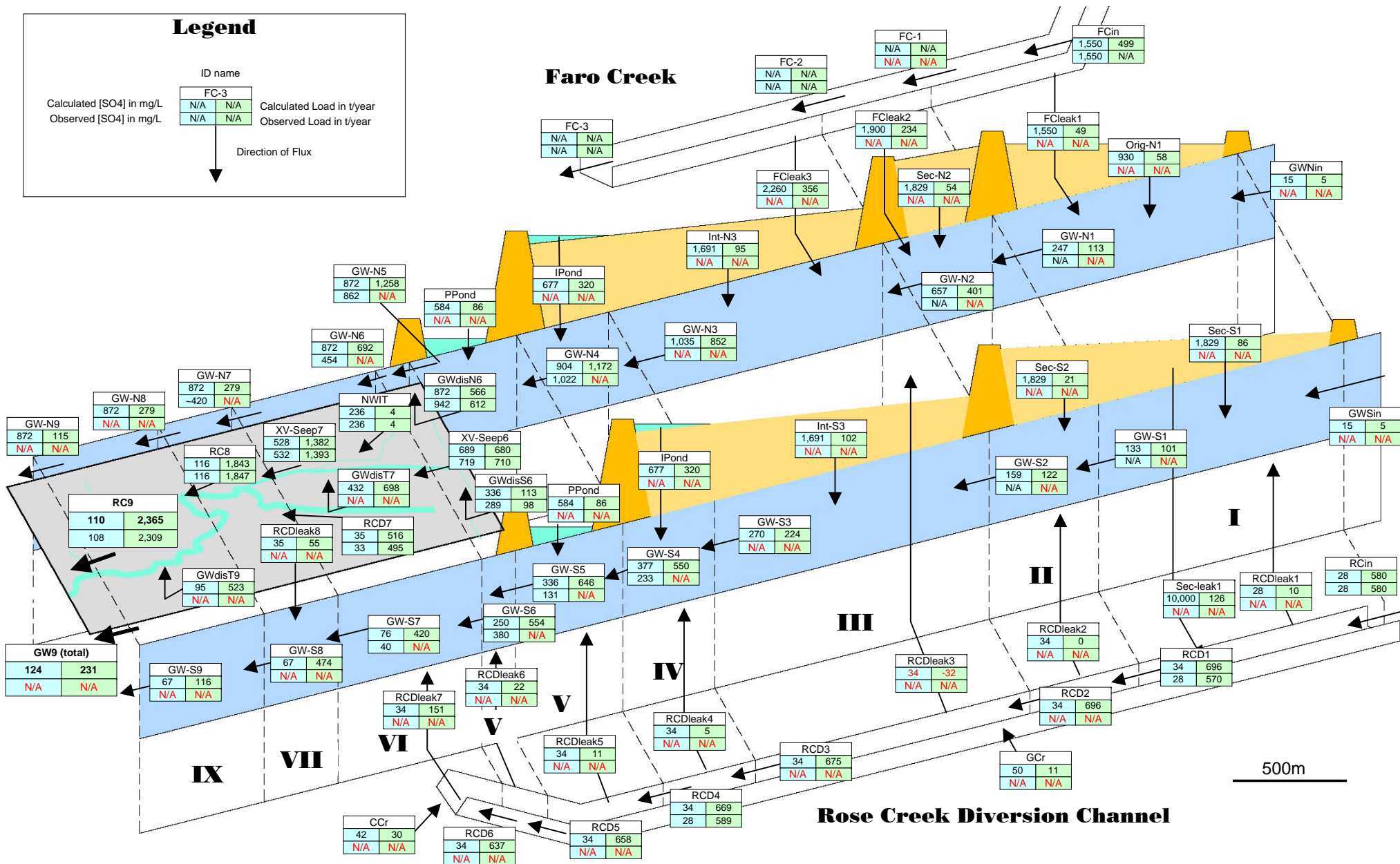
Figure 4.5 Sulphate Load Balance for Rose Creek Valley - Scenario C1.
