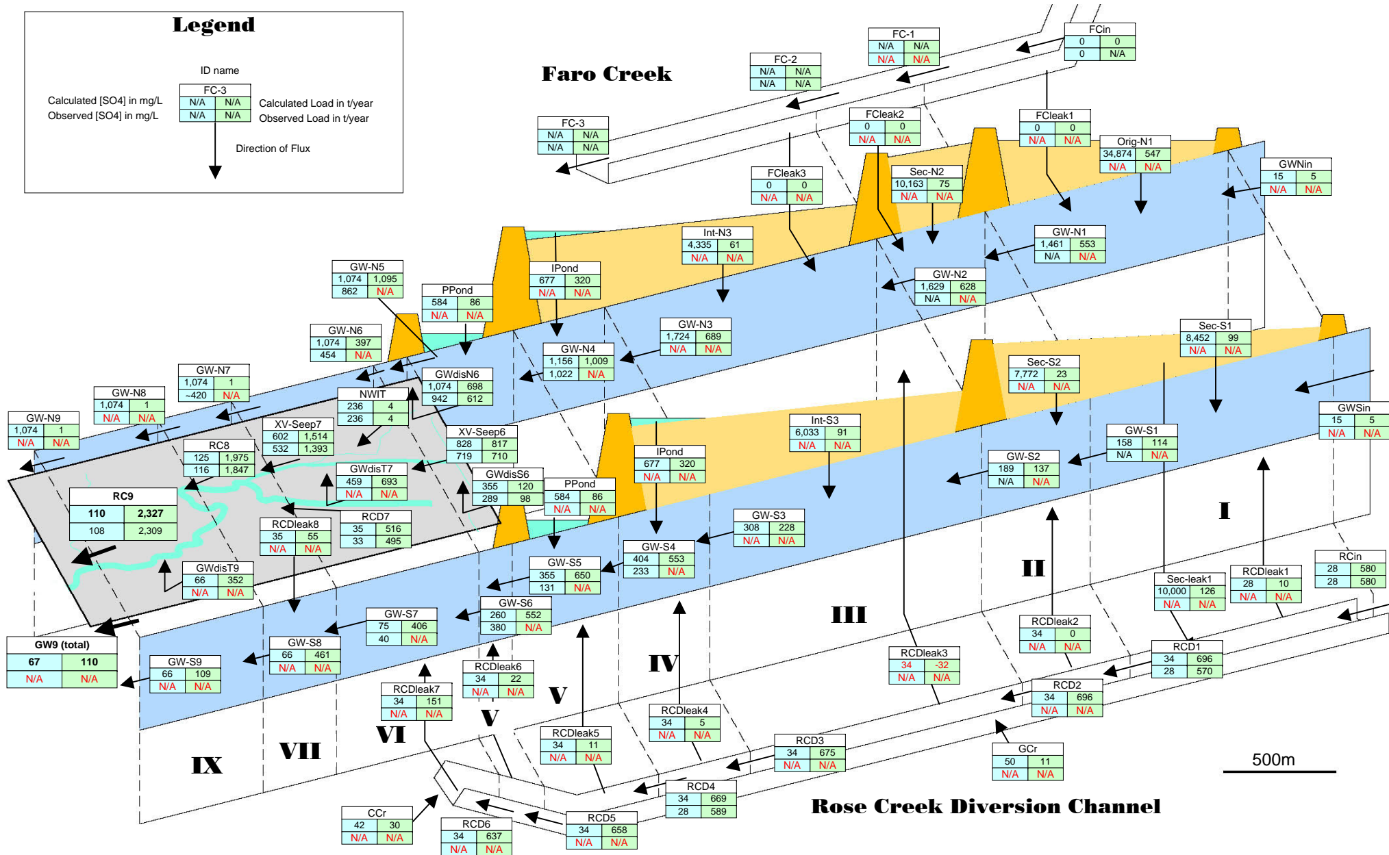
Figure 4.8 Sulphate Load Balance for Rose Creek Valley - Scenario C4.
