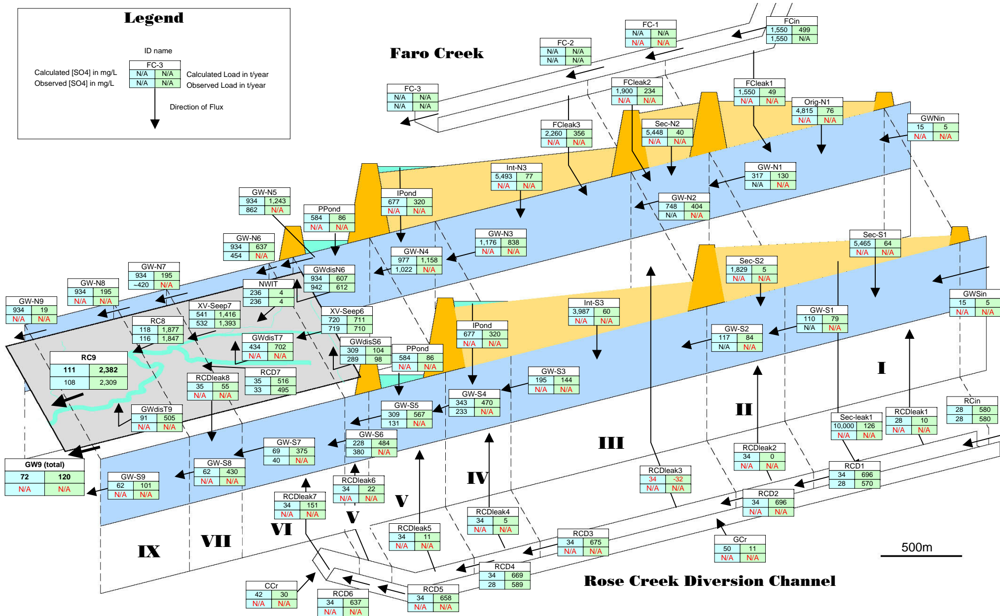
Figure 4.6 Sulphate Load Balance for Rose Creek Valley - Scenario C2.
