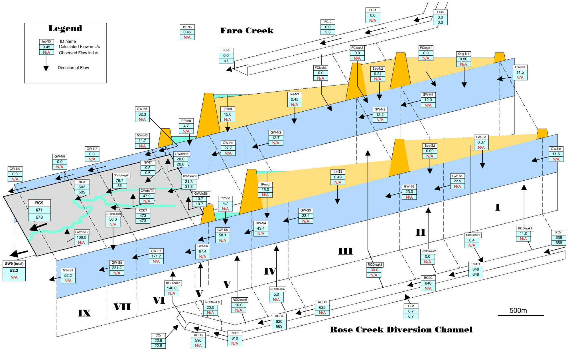
Figure 4.4 Water Balance for Rose Creek Valley - Scenario C4.
