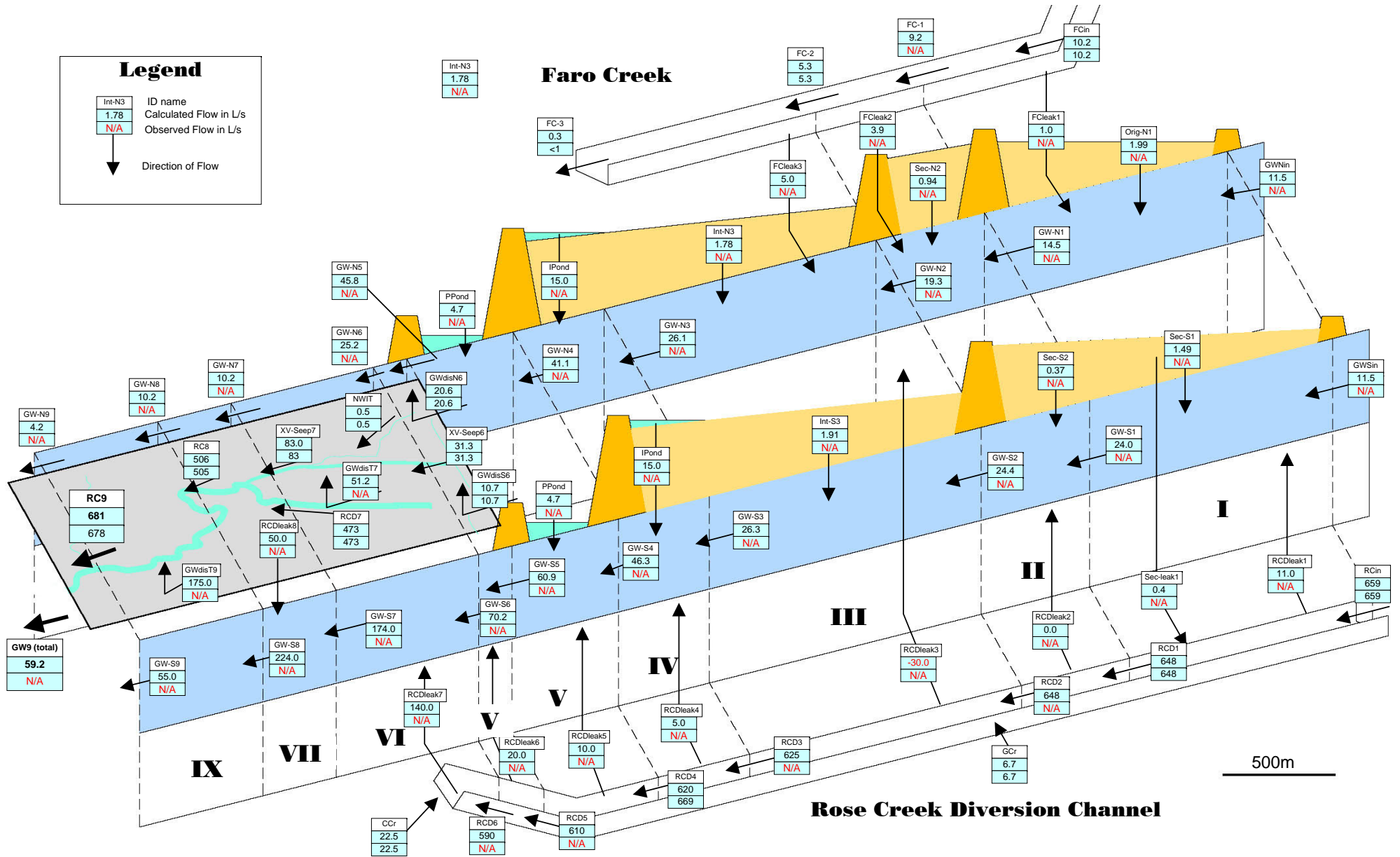
Figure 4.1 Water Balance for Rose Creek Valley - Scenario C1.
