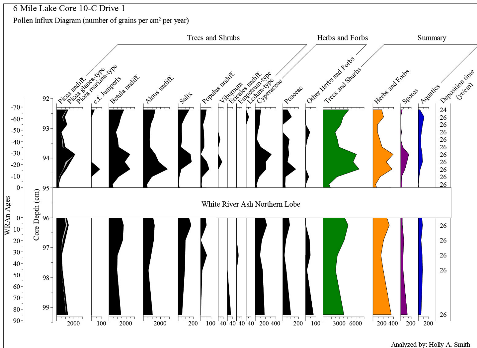
Figure 5.3 Pollen influx (grains/cm 2 /yr) at 6-Mile Lake.
