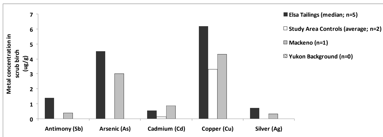
Figure 8. Median antimony, arsenic, cadmium, copper and silver concentrations in scrub birch collected from August 12–14, 2008 from four areas in the Yukon.
