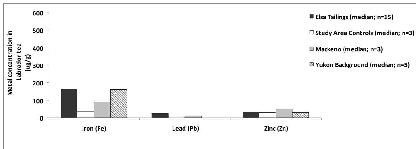
Figure 3. Median iron, lead and zinc concentrations in Labrador tea collected from August 12–14, 2008 from four areas in the Yukon.
