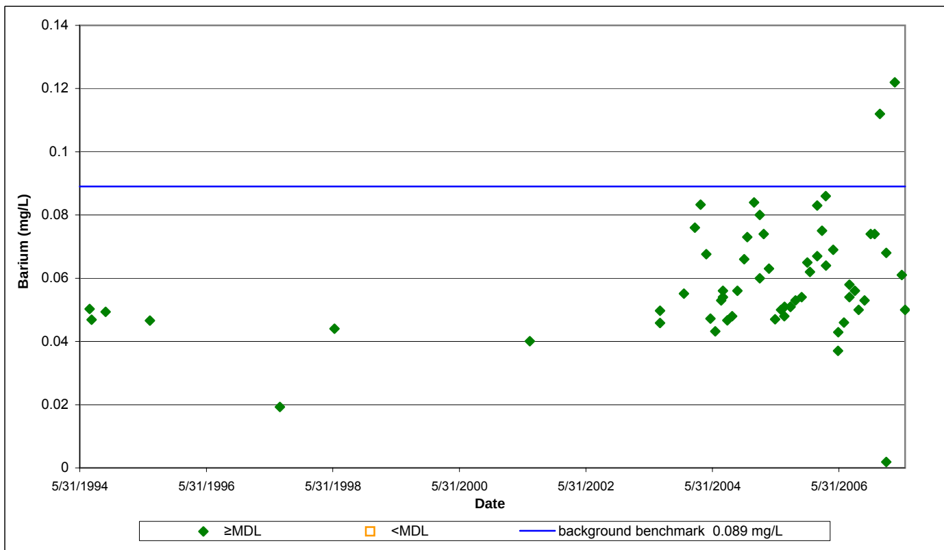
Figure A.54: Scatterplot of barium concentrations over time for background stations KV1 & KV37.
