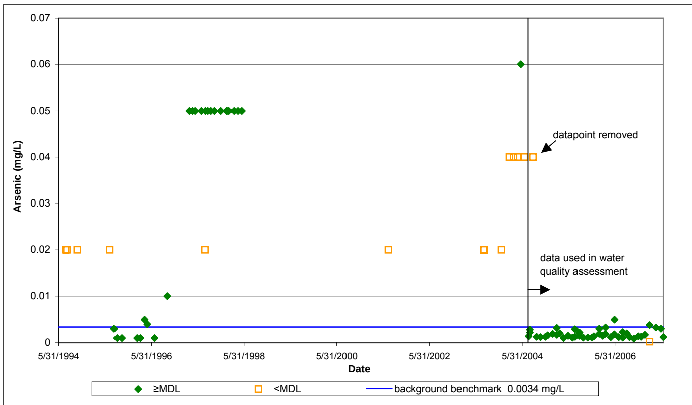
Figure A.53: Scatterplot of arsenic concentrations over time for background stations KV1 & KV37 1 .
