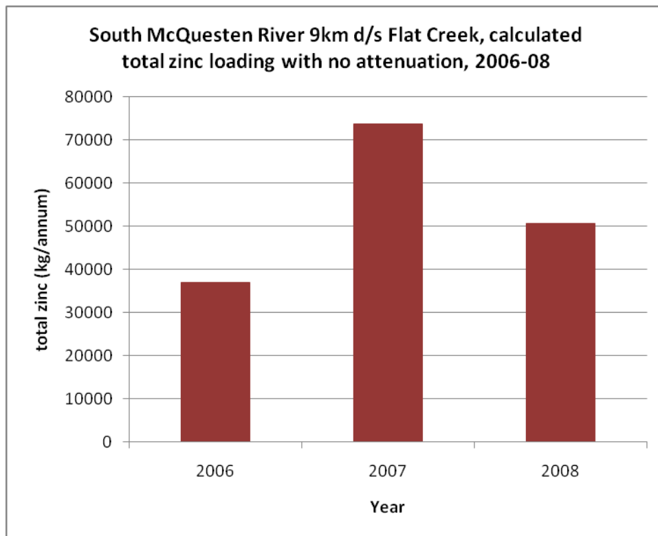
Figure 6 Total Zinc Loading (kg/yr) at the South McQuesten River; All Sources Before Attenuation
