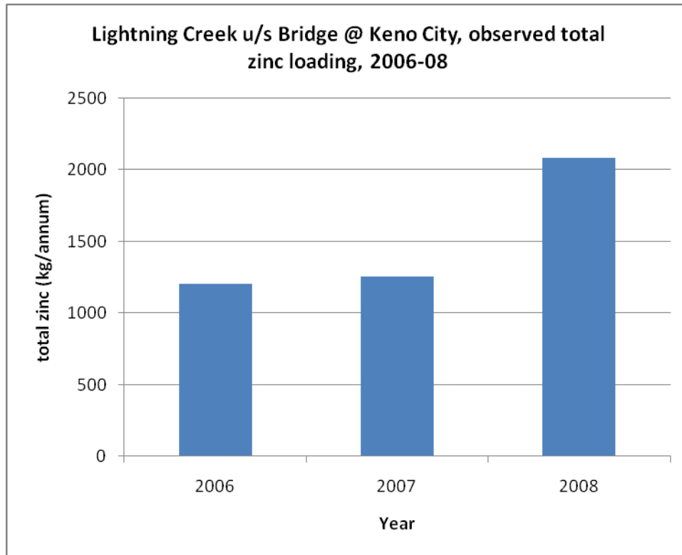
Figure 9 Total Zinc Loading (kg/yr) at Lightning Creek, Observed
