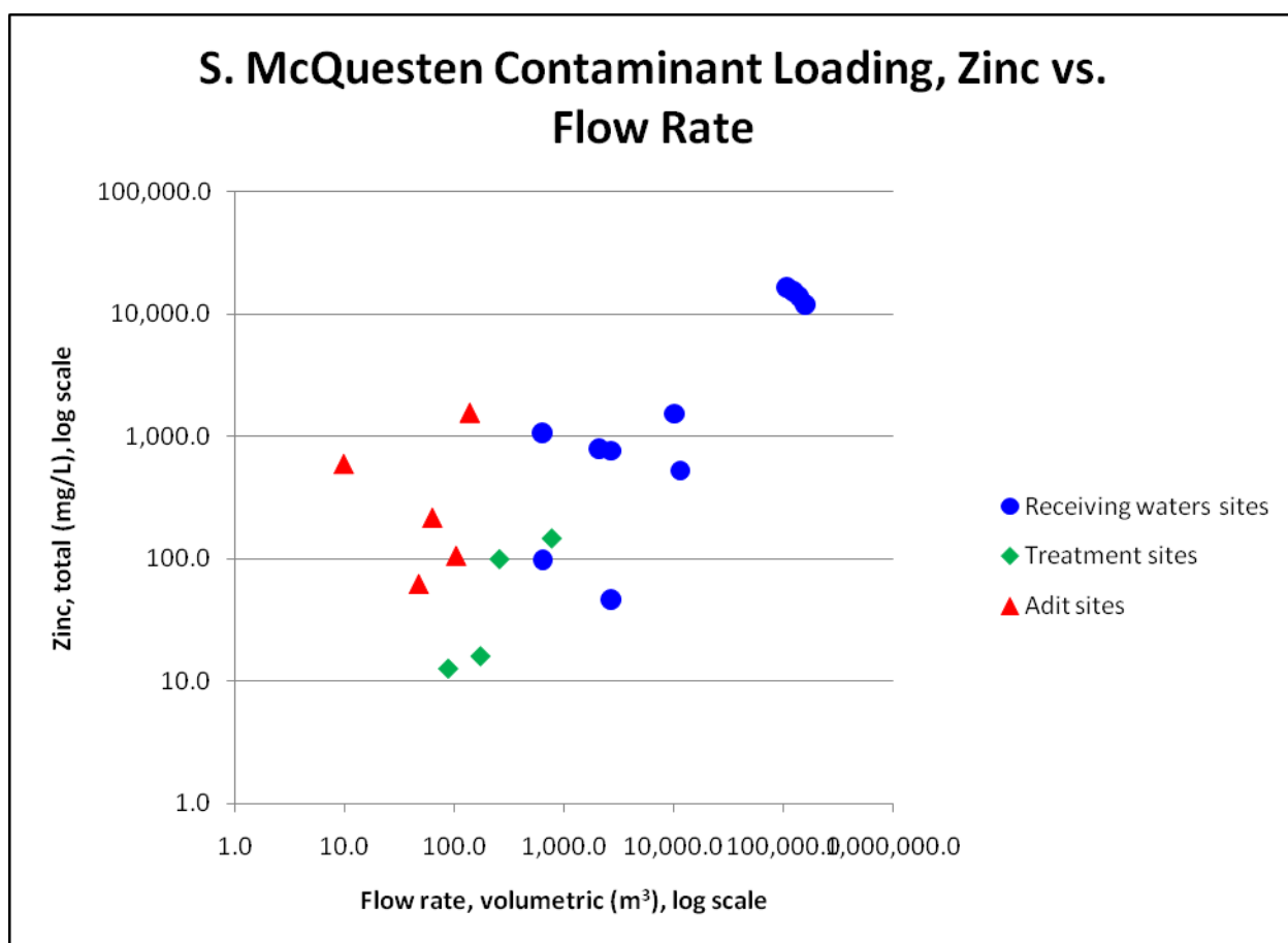
Figure 4 South McQuesten River Cadmium and Zinc Loading versus Annual Volumetric Flow (m³) by Station Type
