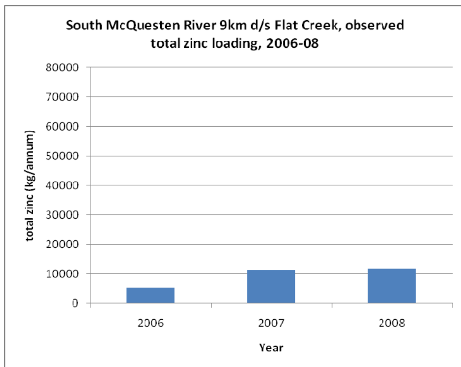
Figure 7 Total Zinc Loading (kg/yr) at the South McQuesten River, Observed
