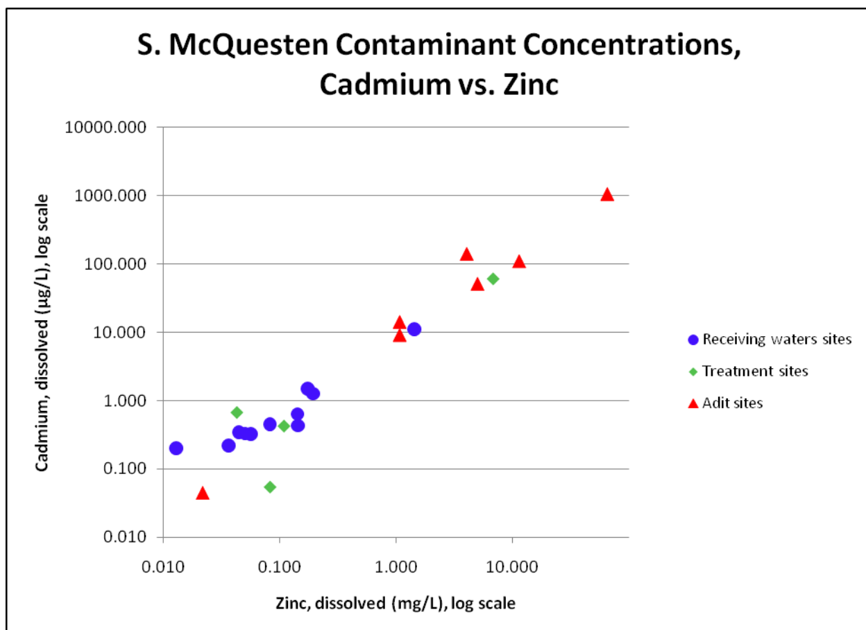
Figure 3 South McQuesten River Cadmium and Zinc Concentrations, by Station Type
