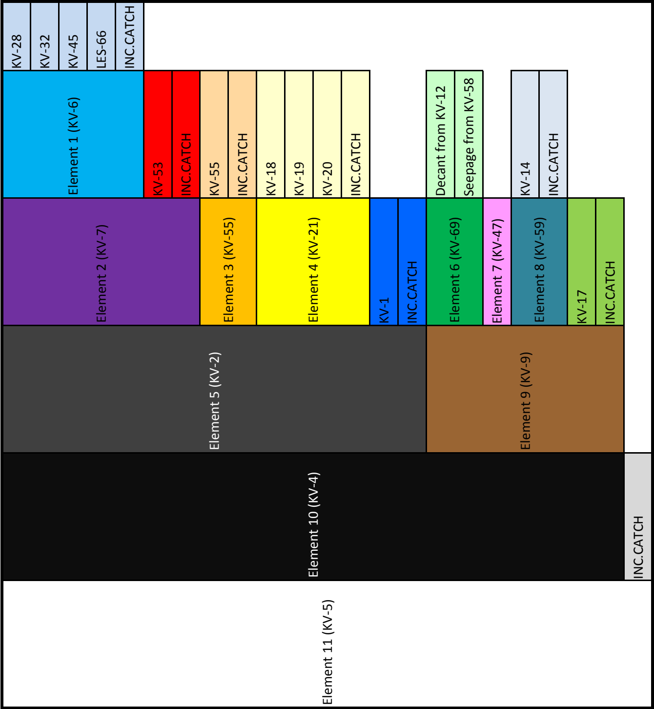
Figure 1 Mass Loading Model Inputs Flow Diagram
