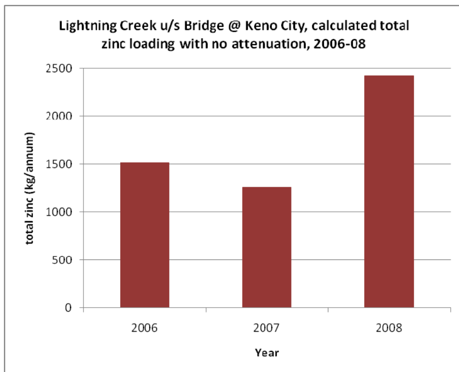
Figure 8 Zinc Loading (kg/yr) at Lightning Creek; All Sources Before Attenuation
