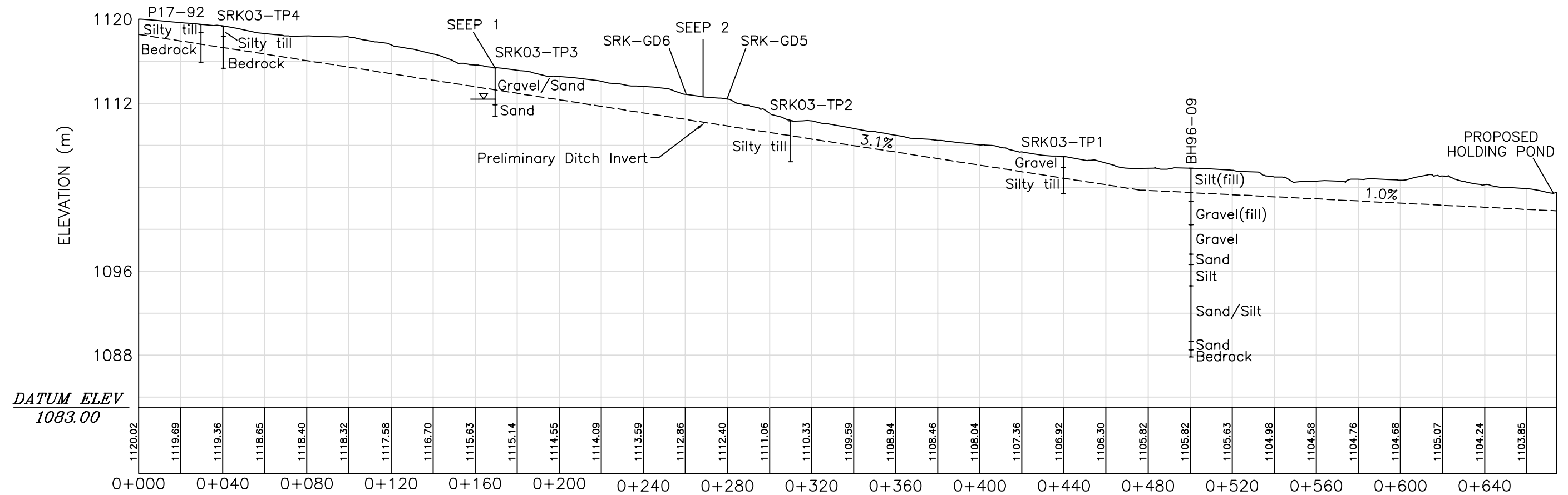
Profile along centerline of Seepage Collection Ditch (metres)
