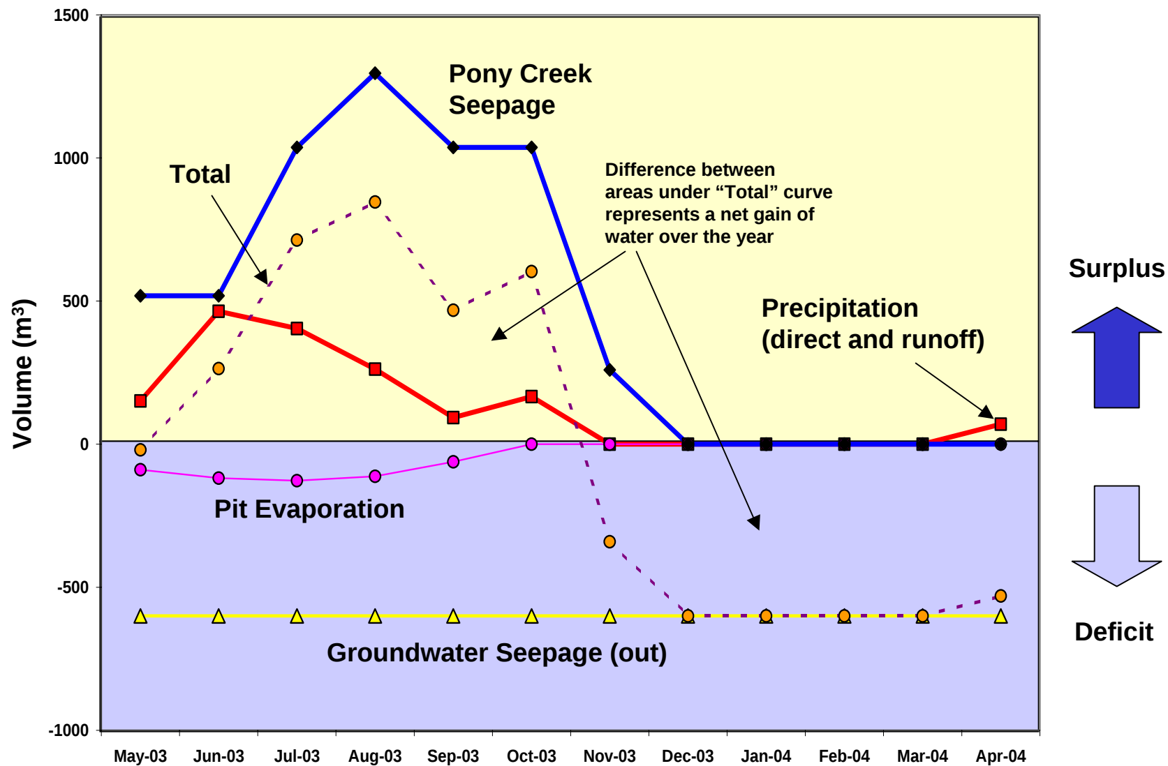
Figure 11. Contribution of Individual Components of Water Balance (based on calibrated model results)
