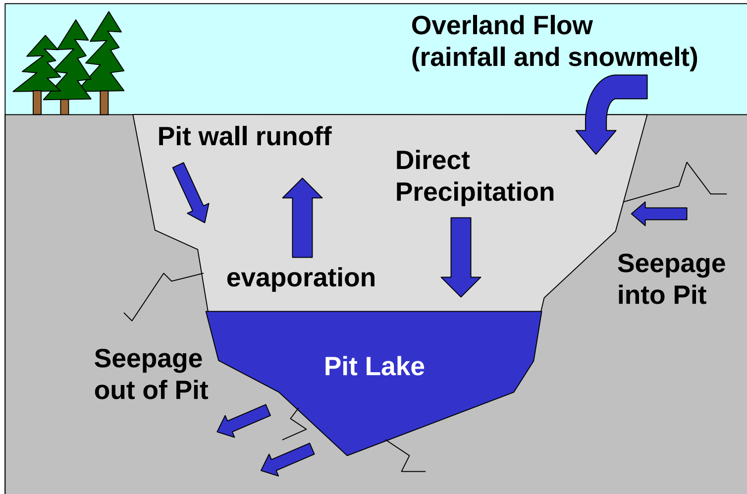
Figure 7. Conceptual Model of Pit Water Balance Components
