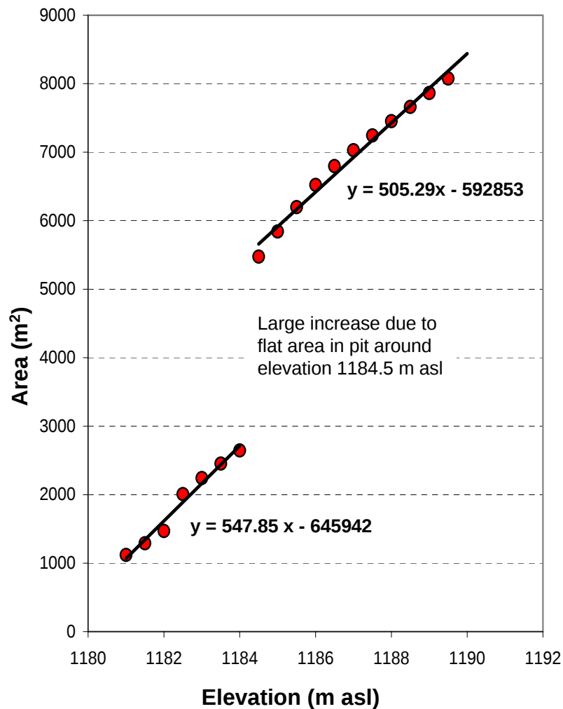
Figure 5. Pit Lake Elevation Volume/Area Curves and functions Used for Water Balance (based on detailed pit survey, 2004)
