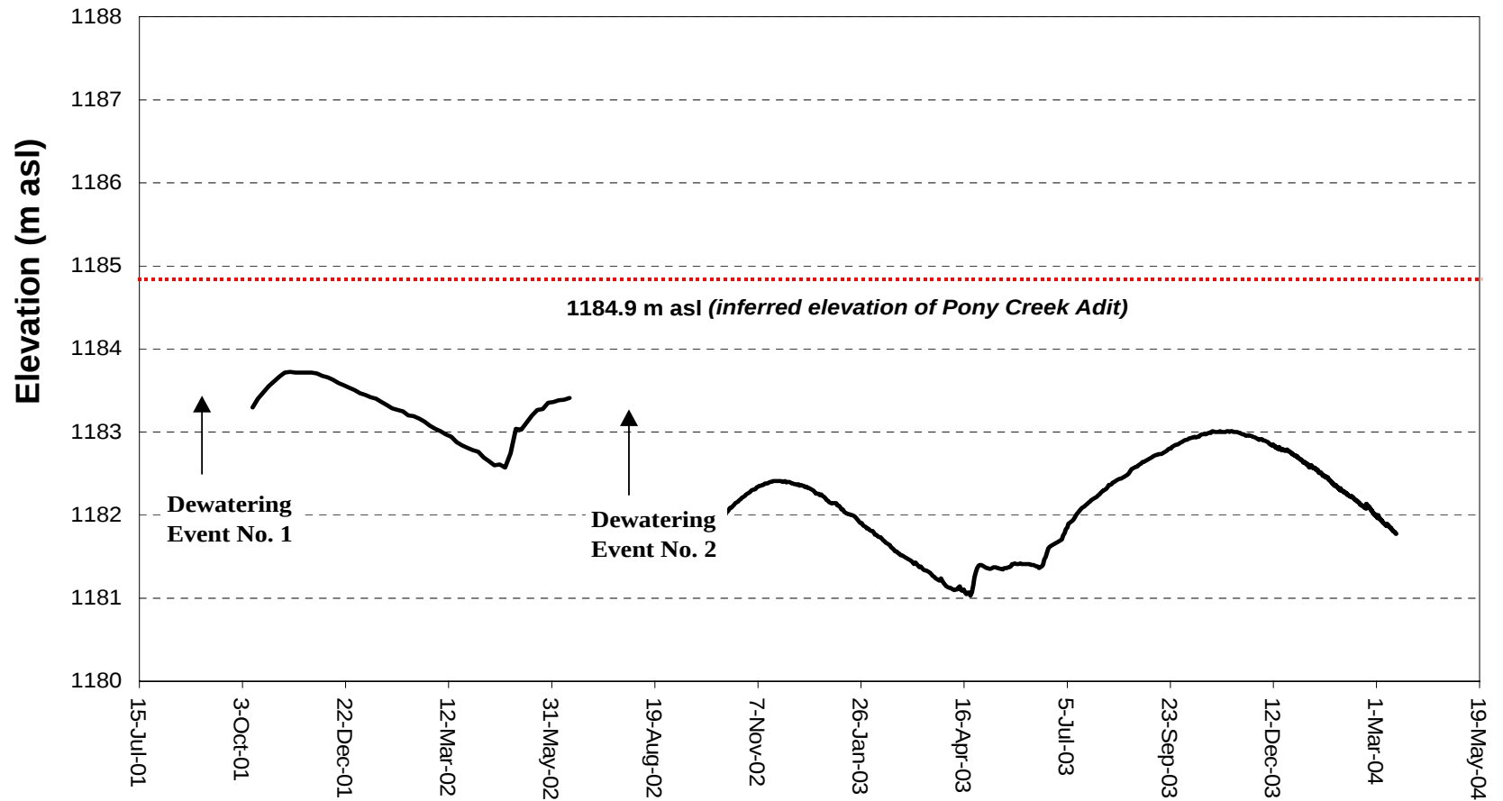
Figure 3. Post-operational Pit Water Level Fluctuations (2001-2004)
