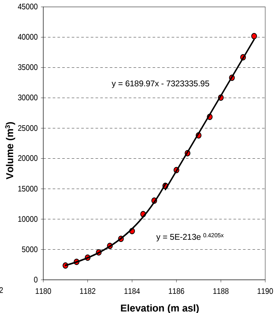
Figure 5. Pit Lake Elevation Volume/Area Curves and functions Used for Water Balance (based on detailed pit survey, 2004)
