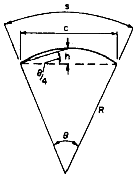
Figure A1. Assumed pipeline configuration.
