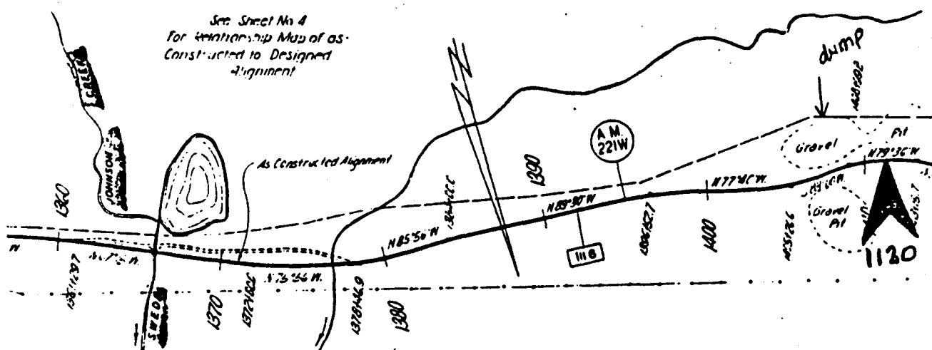
FIGURE 35: Swede Johnson Creek Oil Spill at MP1119.3 - Dump Site at MP1120
