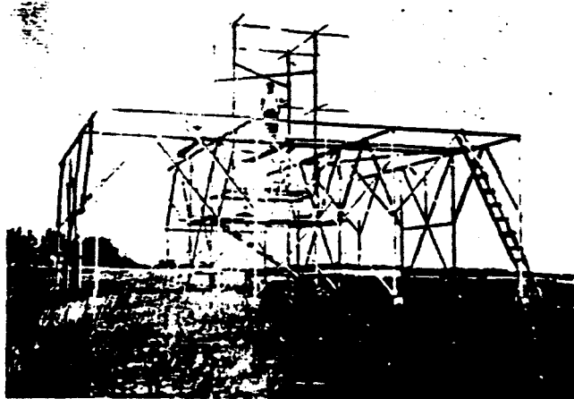
A typical "Cone of Silence" Marker Antenna above counterpoise at all Radio Range Stations
