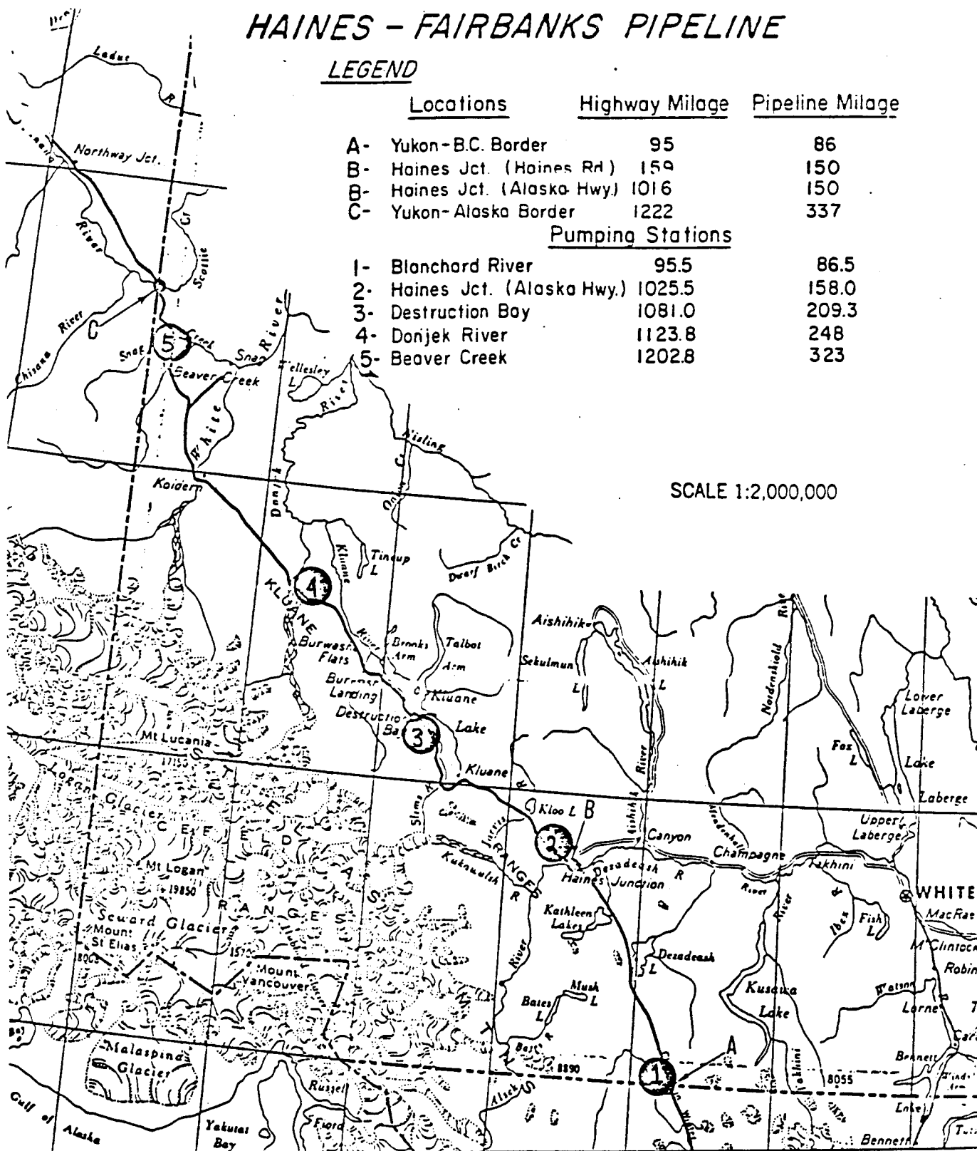
FIGURE 5: Haines -Fairbanks Pipeline with Mileages
