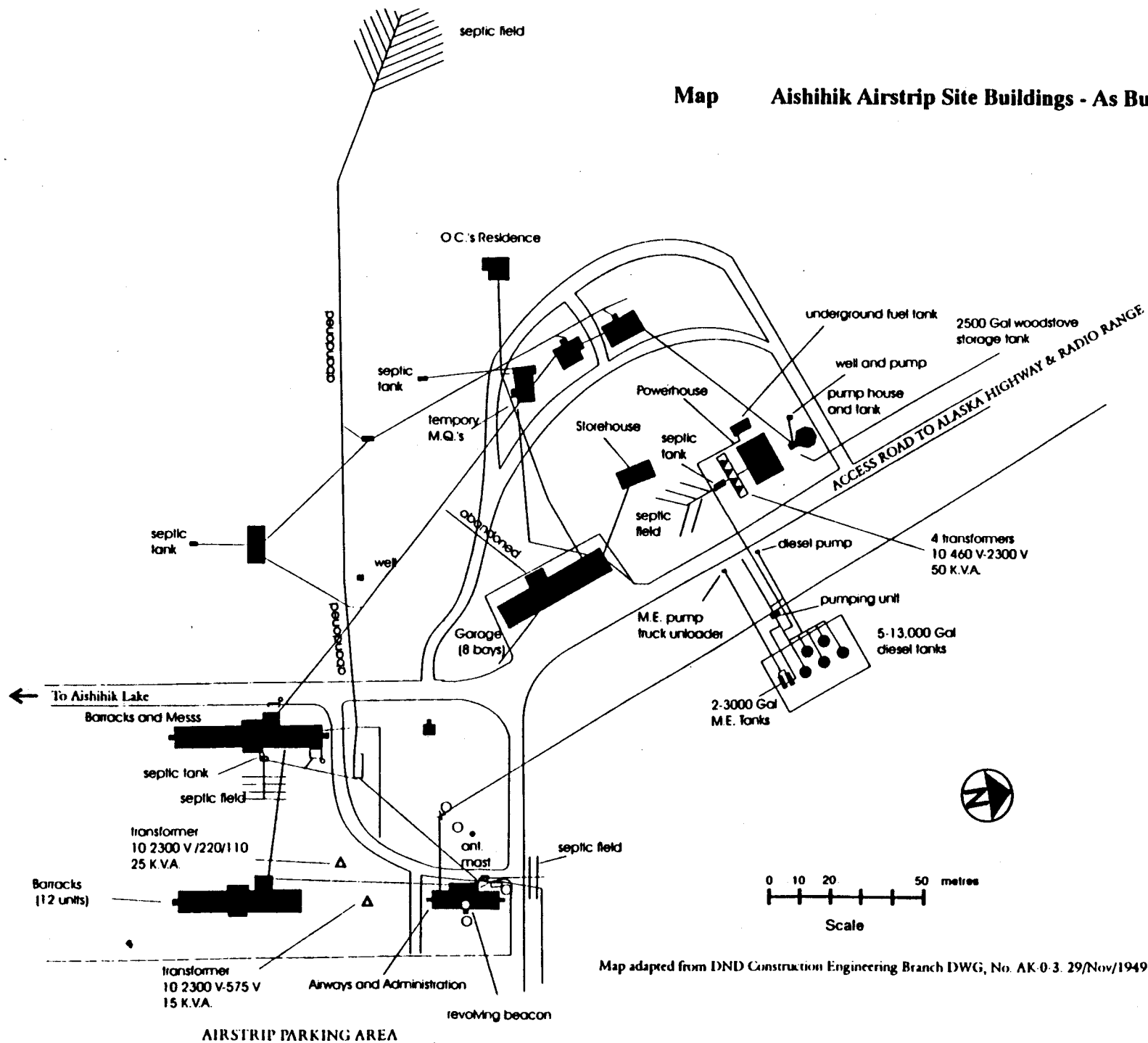
FIGURE 22: Aishihik Airport & Buildings - 1949
