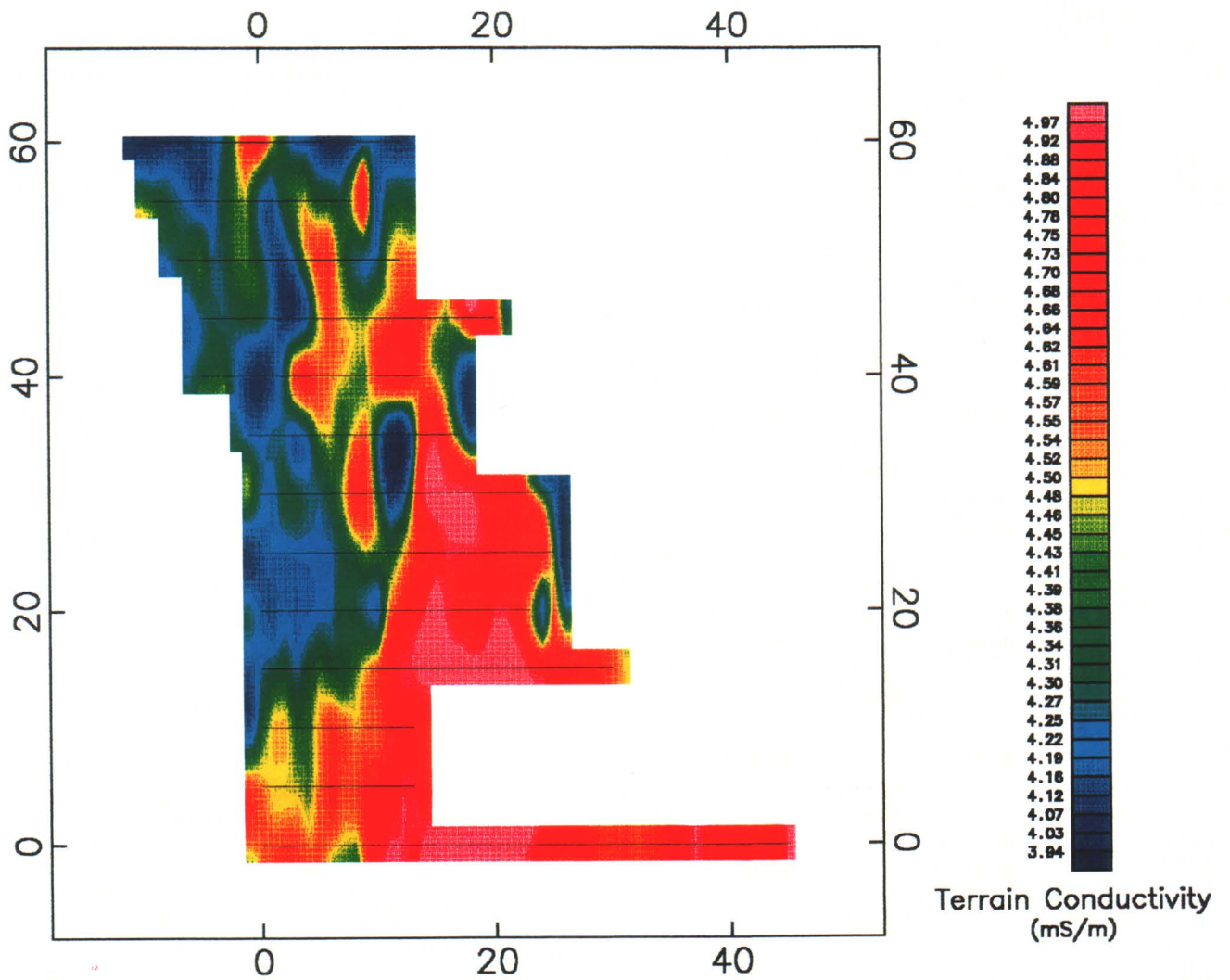
Figure 3a: Canyon Site MDA-3A Terrain Conductivity
