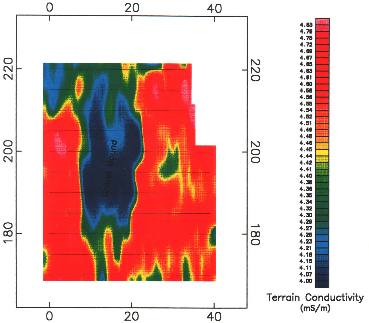
Figure 2a: Canyon Site MDA-1B Terrain Conductivity
