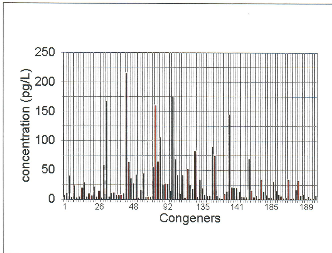
Figure 11: Volume weighted PCB congener concentration of snow samples collected at Wolf Creek, 1997-98
