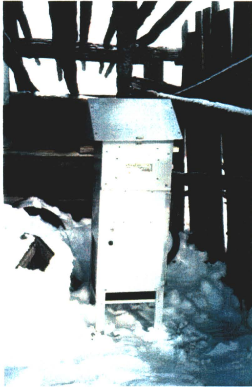
Figure 8: High volume air sampler positioned inside the smoke house prior to lighting of fires and covering with tarpaulins – i.e. background air sample
