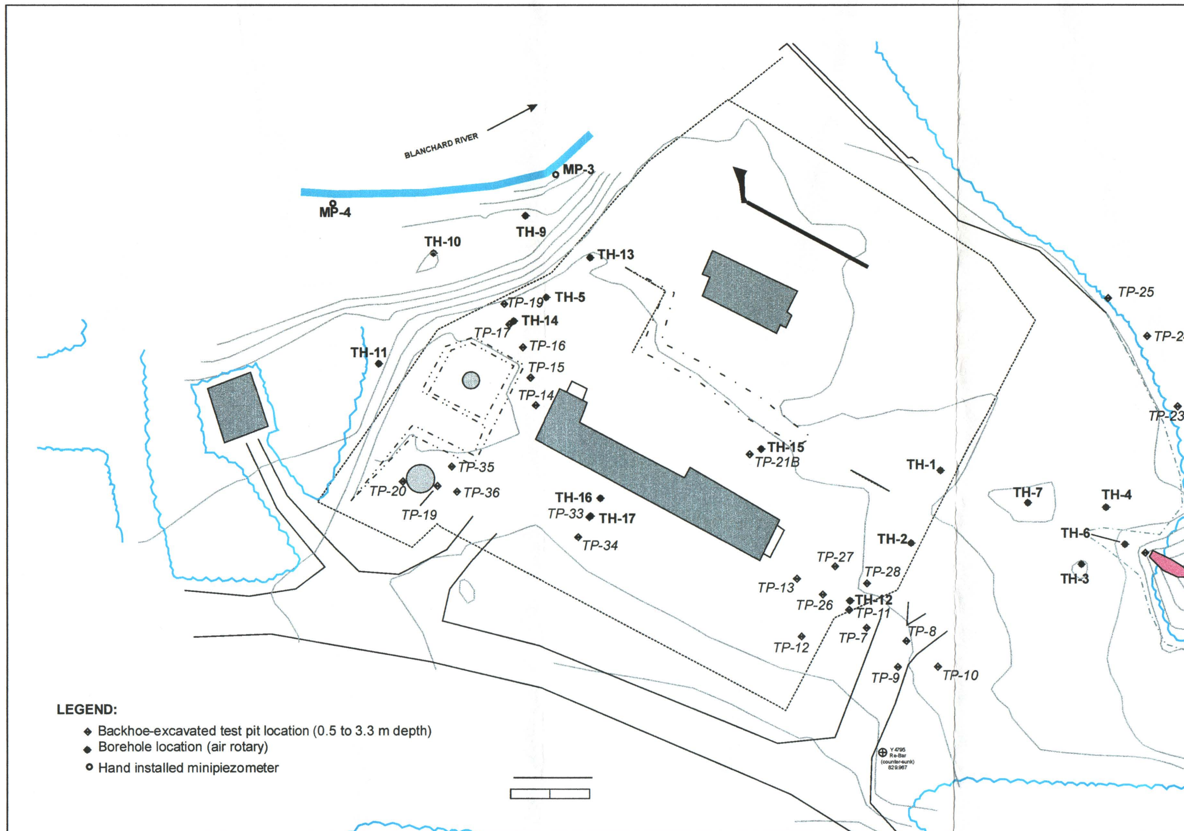
MAP 2.1: BLANCHARD RIVER STATION - SITE LAYOUT Including sampling locations, 1995 preliminary site investigation and 1999 detailed site investigation
