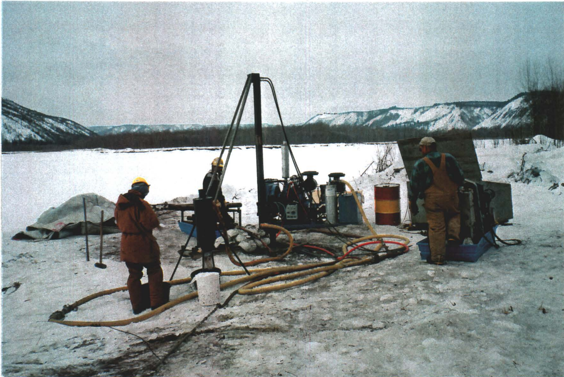
Photograph 2.3: Drilling with the air rotary system on the upper bench
