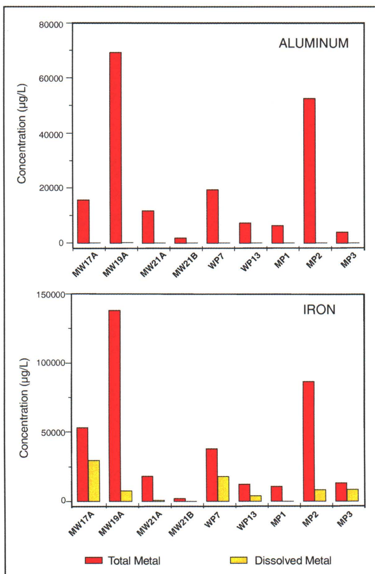
Figure 4.7: Comparison of Total Metal to Dissolved Metal Concentrations in Groundwater Samples Collected from Rainy Hollow in 1998
