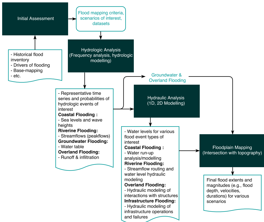
Figure 19. Summary of a typical hydrotechnical approach to flood hazard mapping (Adapted from: FEMA 2009; Wicks and Lovell 2011; Silander et al. 2012; Bowering et al. 2013; MMM Group 2014; Burrell et al. 2015; Naslund-Landenmark 2015; Patrick et al. 2015)
