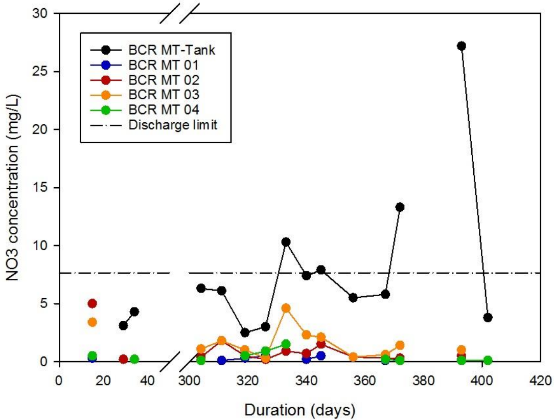
Figure 8. NO 3 concentrations in influent and effluent of the four bioreactors (BCR-MT-01 to -04) between August 20 th 2014 and September 26 th 2015 (Discharge Limit of 7.65).
