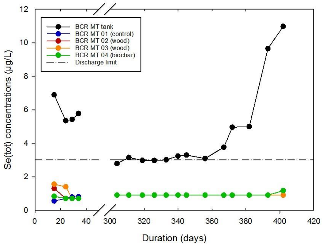
Figure 5. Selenium concentration in influent and effluent of the four bioreactors (BCR-MT-01 to -04) between August 20 th 2014 and September 26 th 2015 (Discharge Limit of 0.003 mg/L).
