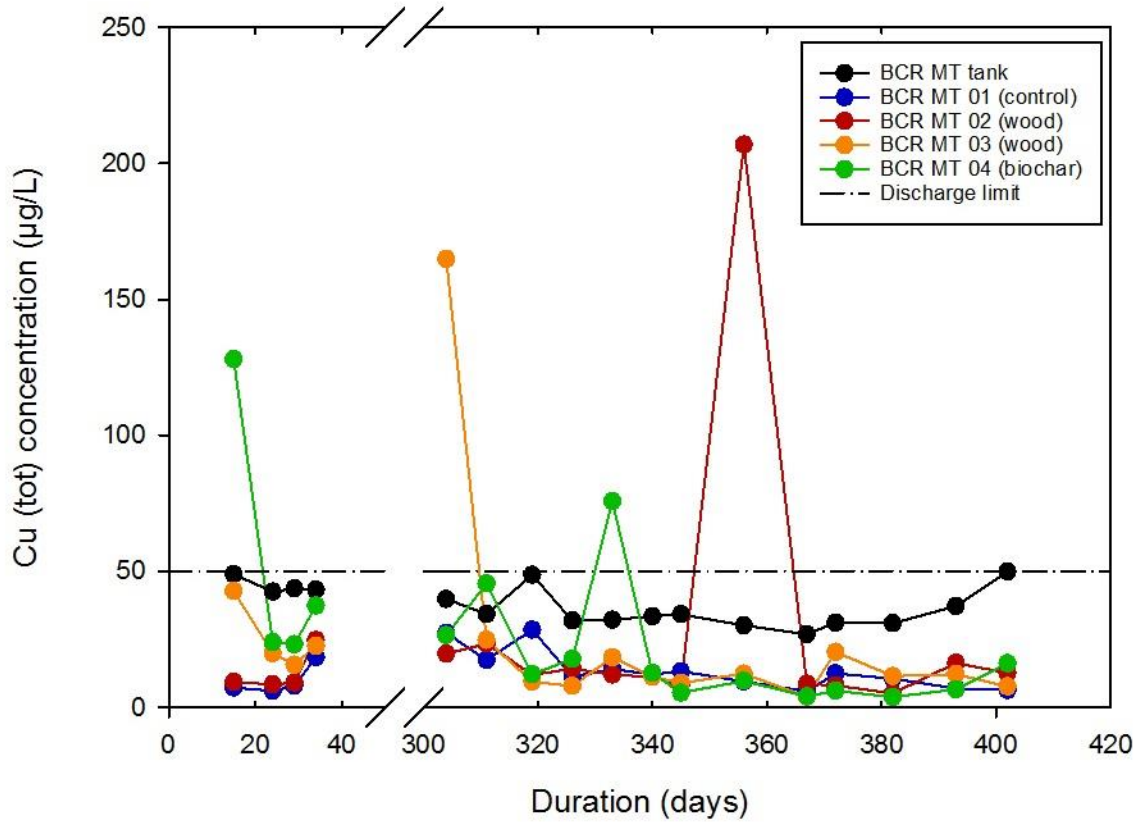
Figure 2. Copper concentrations in influent and effluent of the four bioreactors (BCR-MT-01 to -04) between August 20 th 2014 and September 26 th 2015 (Discharge Limit of 0.050 mg/L).
