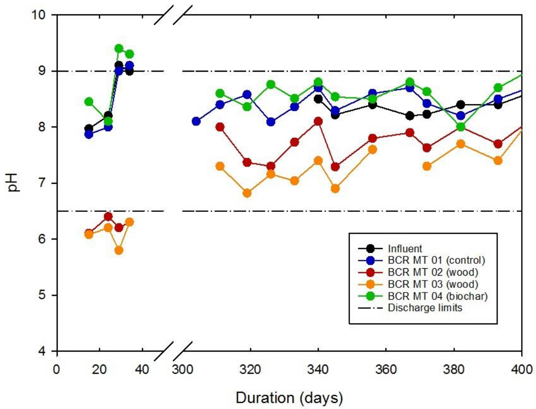
Figure 7. pH in influent and effluent of the four bioreactors (BCR-MT-01 to -04) between August 20 th 2014 to September 26 th 2015 (Discharge Limit Range: 6.5 to 9).
