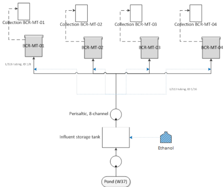
Figure 2. Bioreactors influent feed setup.
