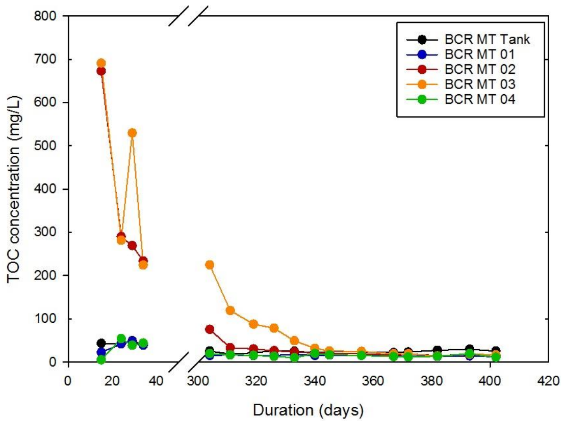
Figure 9. Total Organic Carbon in influent and effluent from the four bioreactors (BCR-MT-01 to -04) between August 20 th 2014 and September 26 th 2015.
