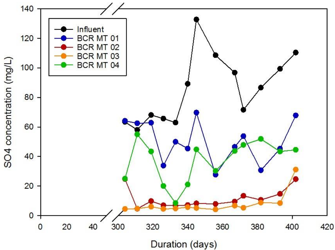
Figure 30. Total Sulfate in influent and effluent from the four bioreactors (BCR-MT-01 to -04) between August 20 th 2014 to September 26 th 2015.
