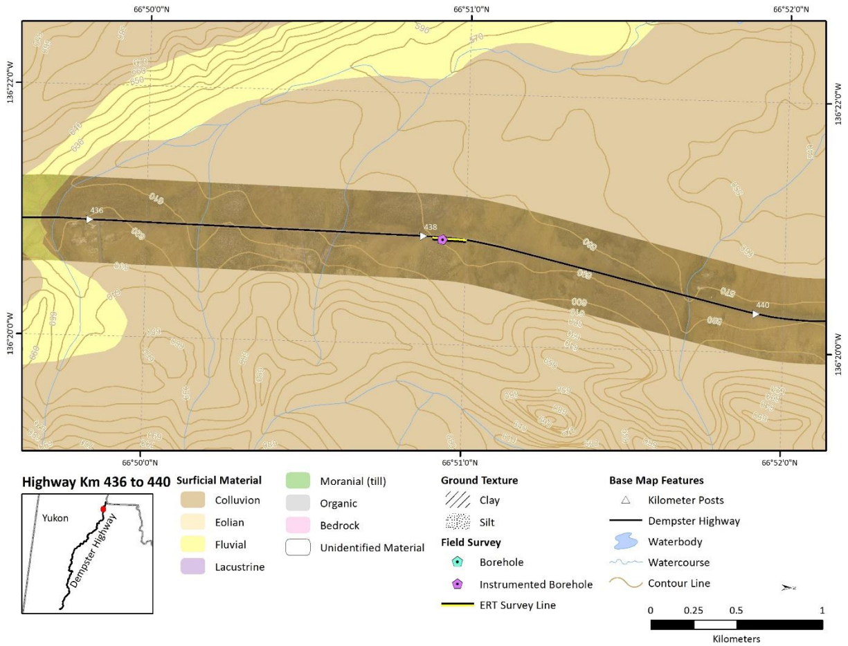
Figure 3.13.2 Surficial geology map of Site 13 DH438 area.
