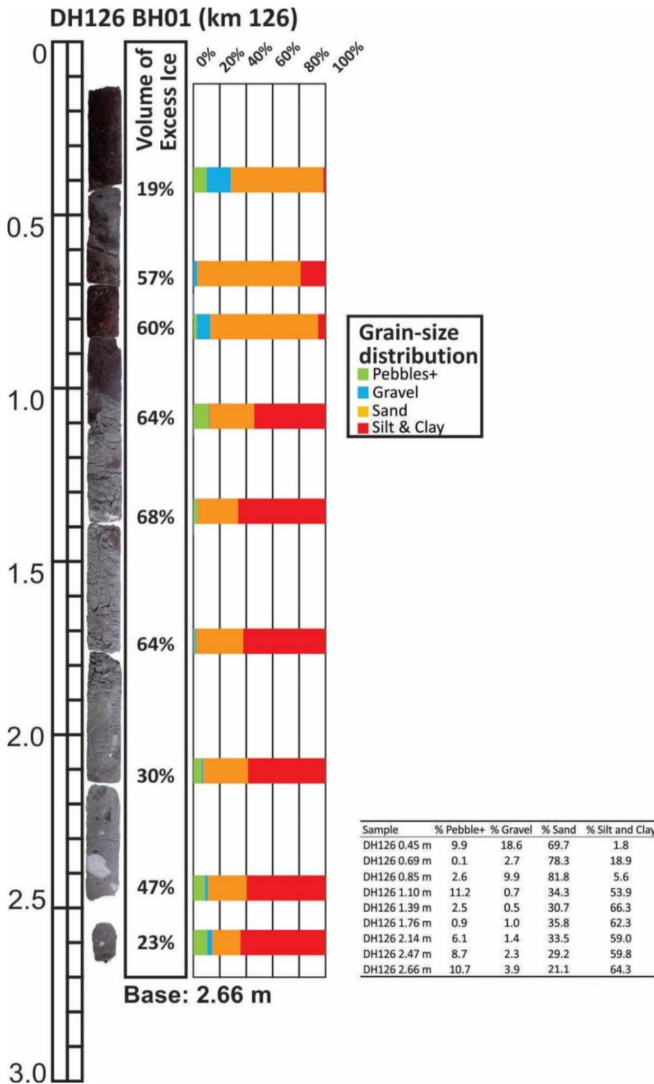
Figure 3.7.4 Log of DH126 BH1, in Field.
