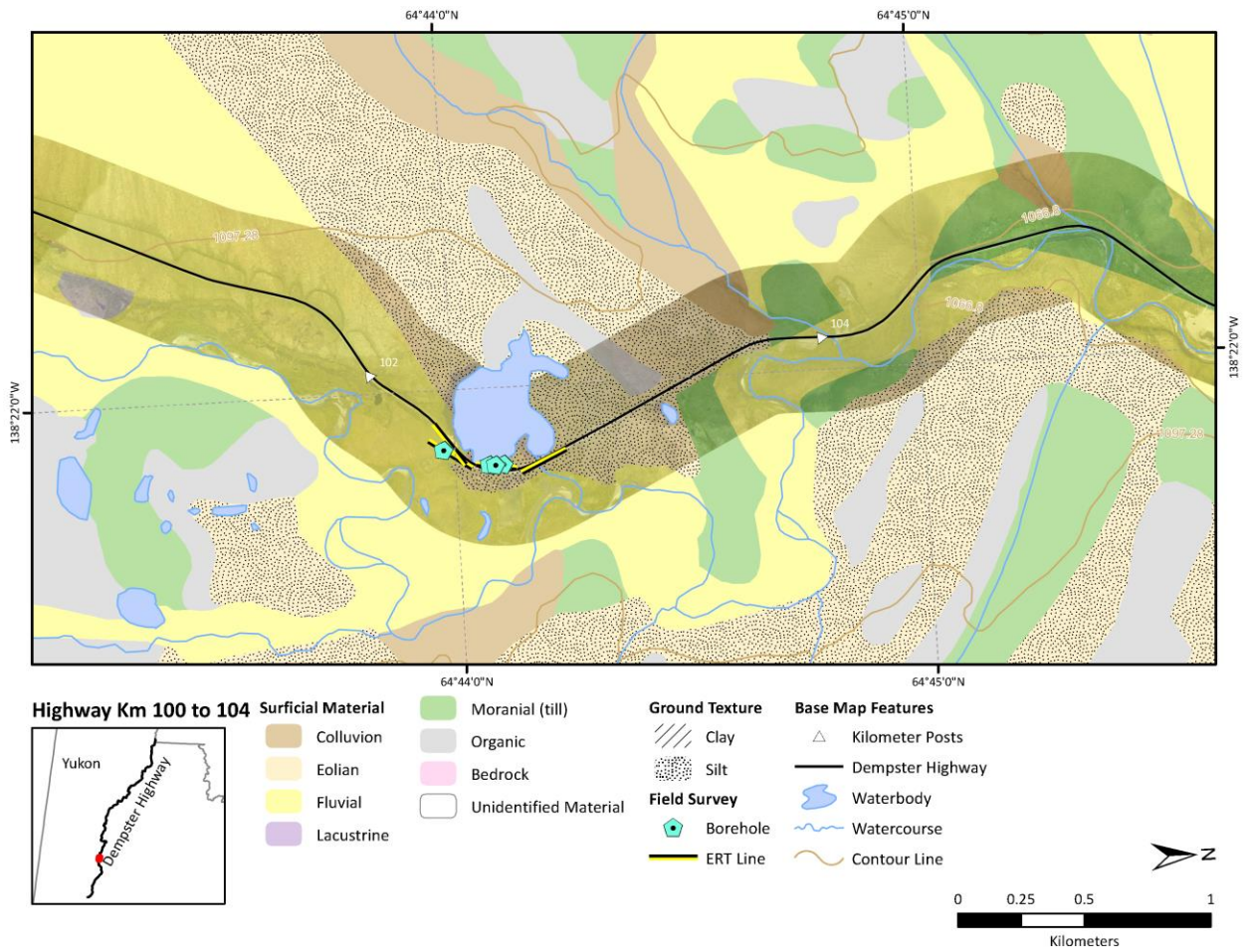
Figure 3.3.1 Surficial geology map of the site 3 DH102 area
