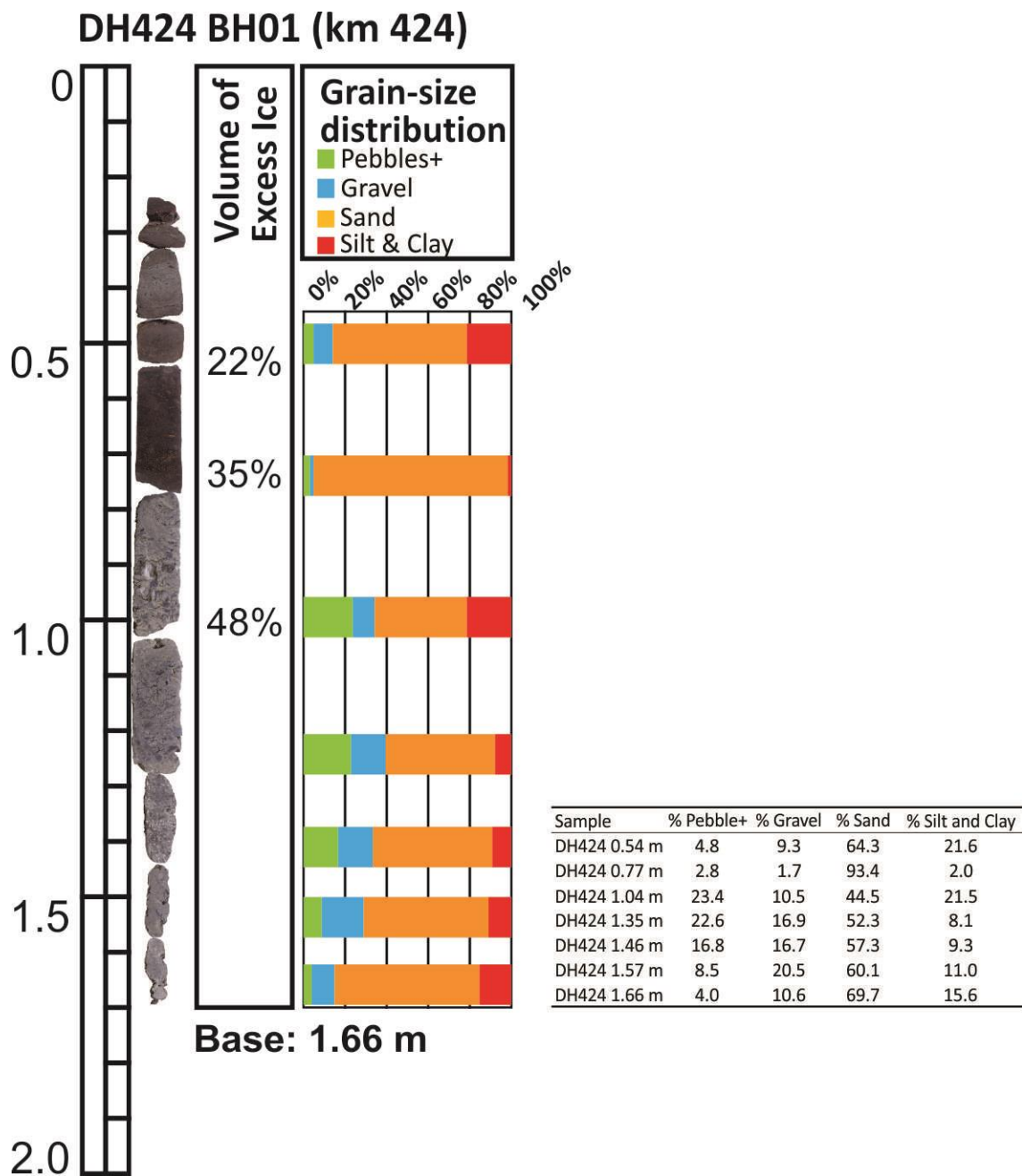
Figure 3.12.4 Log of borehole DH424 BH1 Field.
