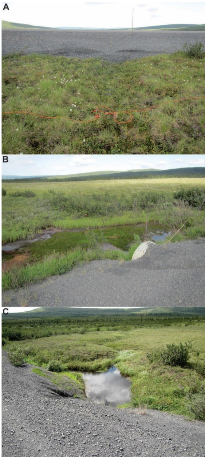
Figure 3.11.1 Degradations observed at site DH421: A- cracks on shoulder of the embankment at right-hand side; B- Settlement and water ponding at a culvert at right-hand side; C- a thermokarst pond and ice wedges degrading at left-hand side.
