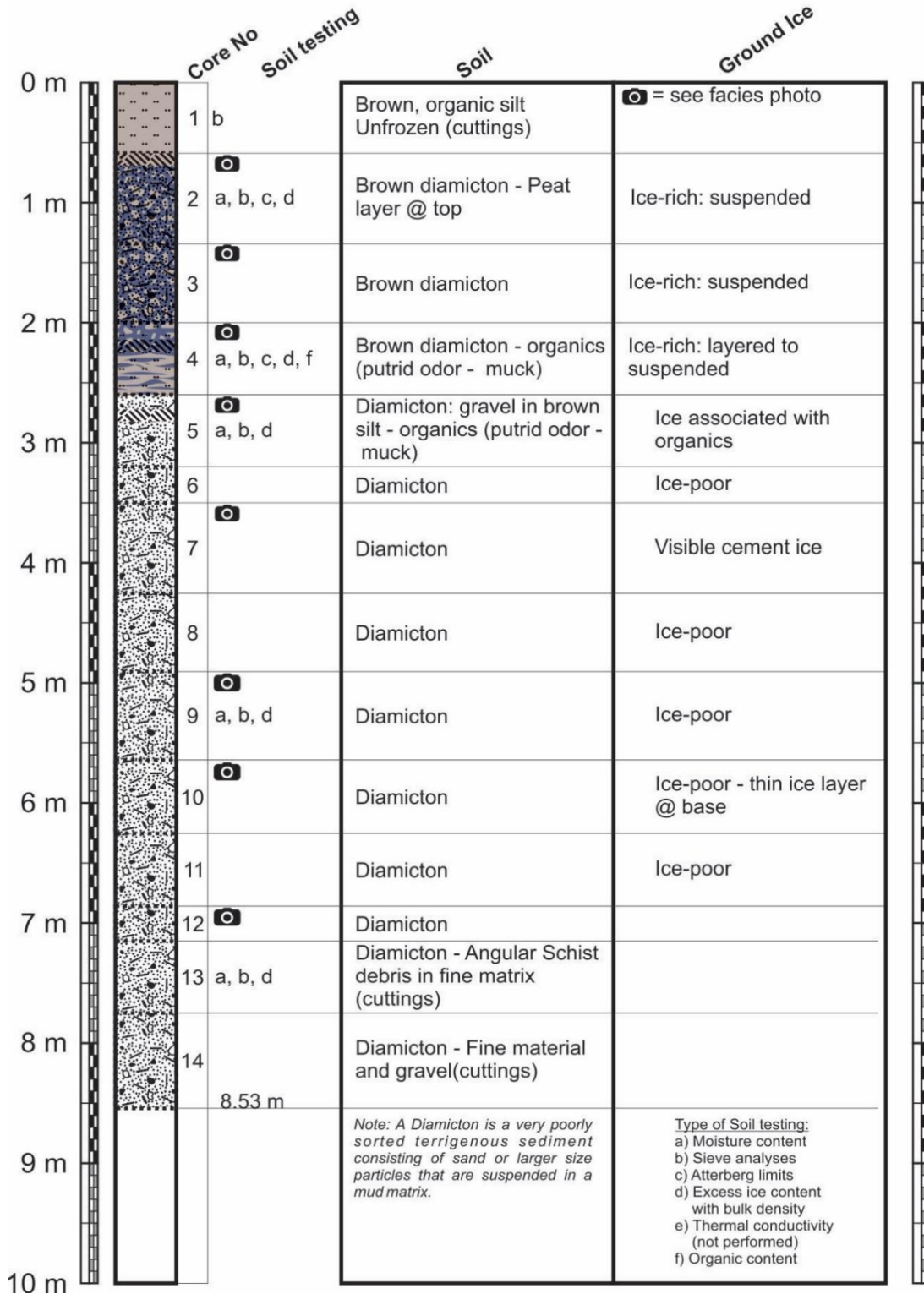
Figure 3.11.4 Log of borehole DH421 BH1 Field.
