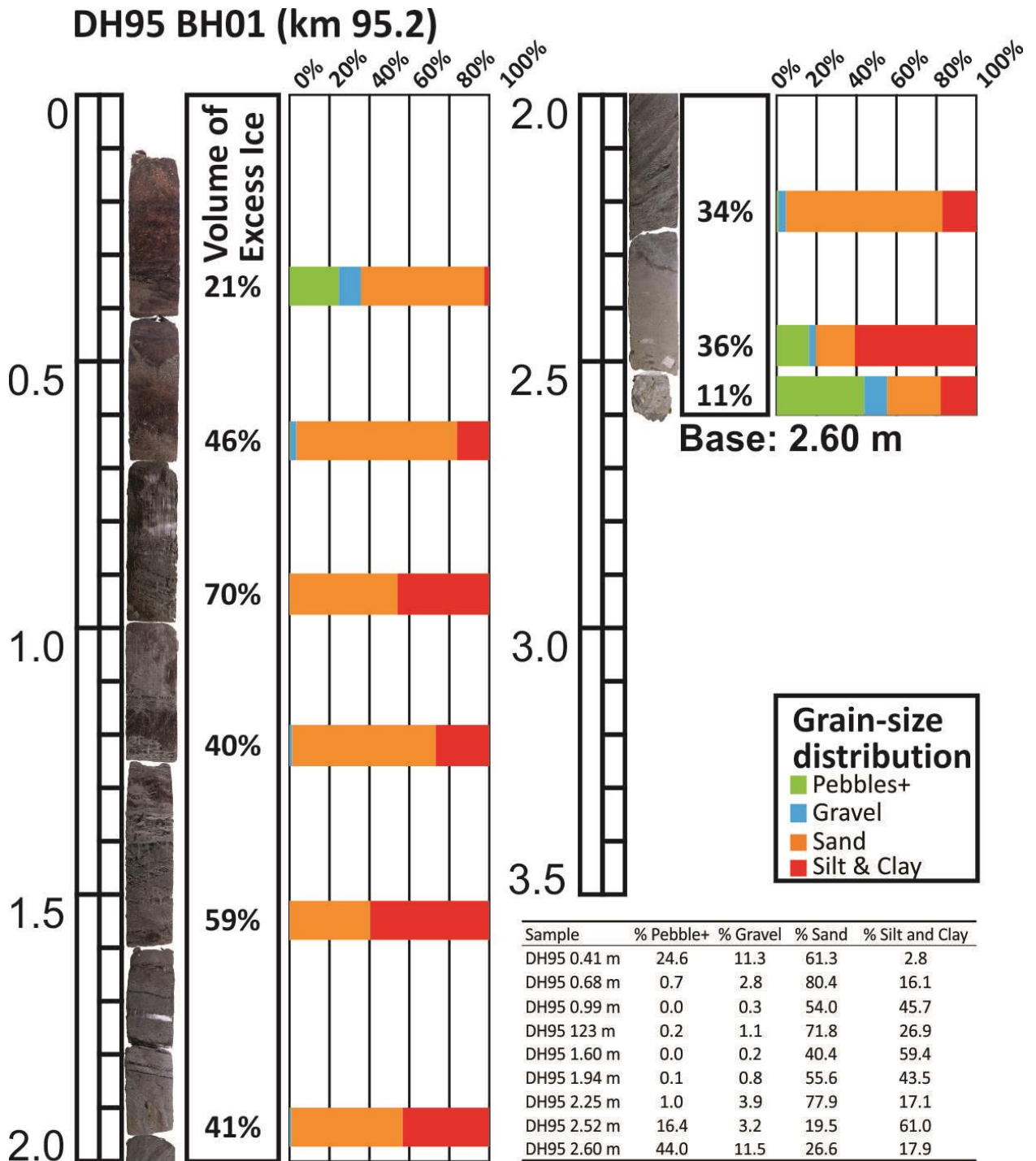
Figure 3.2.3 Logs of borehole DH95 BH1, with volumetric excess ice content and grain size distribution.
