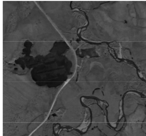
Figure 8. Thermokarst expansion of Two Moose Lake has brought it to the highway embankment. Image from Google Earth.
