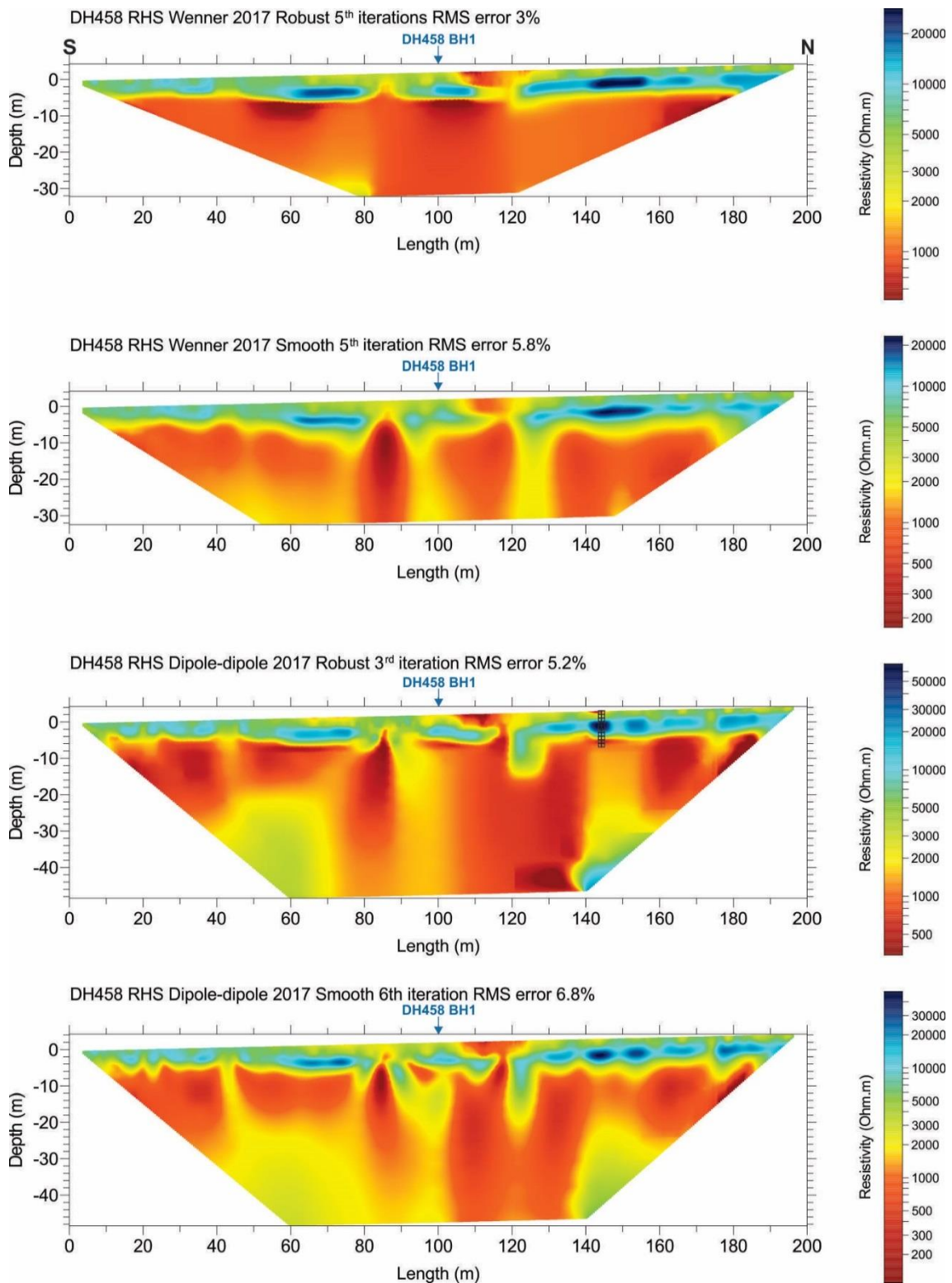
Figure 3.17.6 Wenner and dipole-dipole ERT surveys at site DH458, right-hand side (RHS), using robust and smoothed inversion processes.
