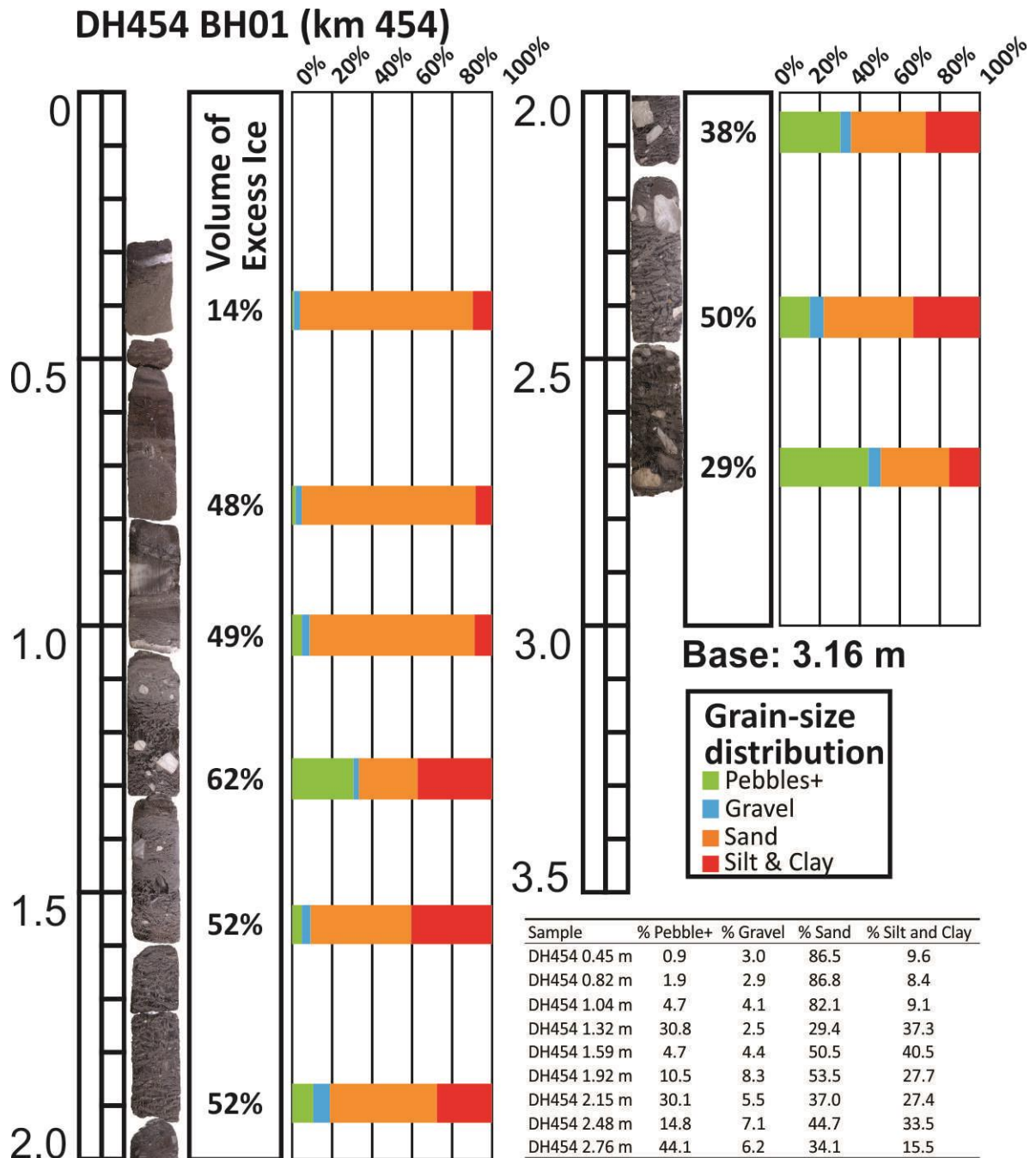
Figure 3.16.4 Logs of borehole DH454 BH1, with volumetric excess ice content and grain size distribution.
