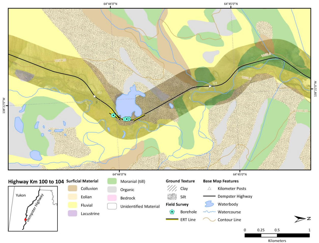
Figure 3.4.2 Surficial geology map of the site 4 DH103 area (same as DH102)
