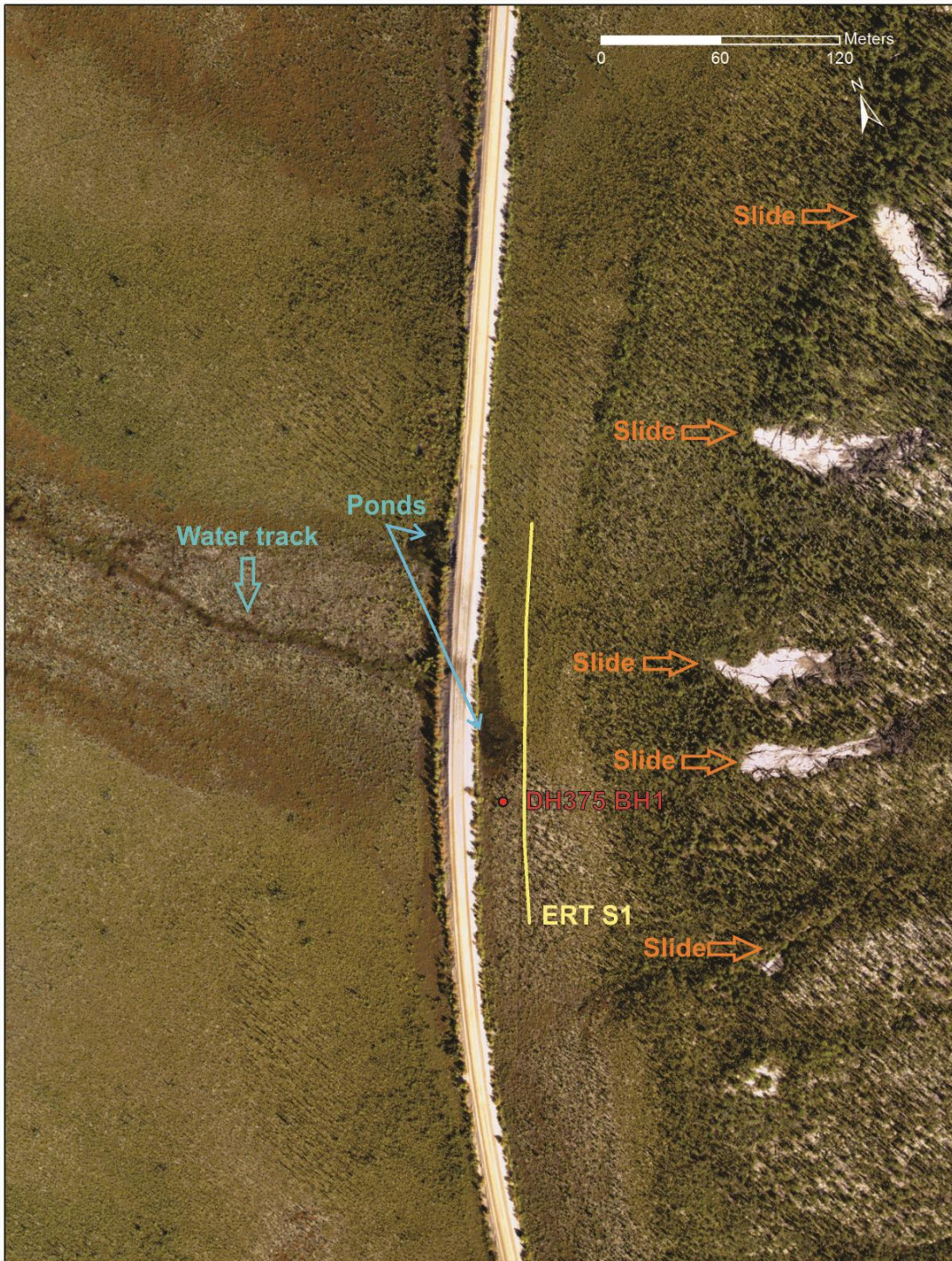
Figure 3.9.3 Aerial view of site DH375
