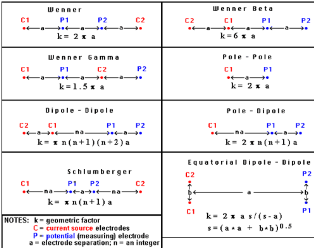
Figure 2.2.2 Survey configurations or “arrays” for ERT surveying.
