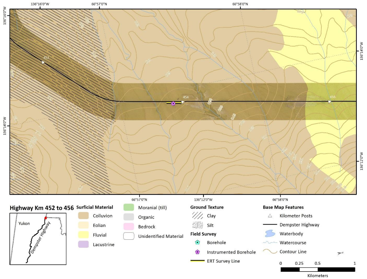
Figure 3.16.2 Surficial geology map of the site 16 DH454 area.
