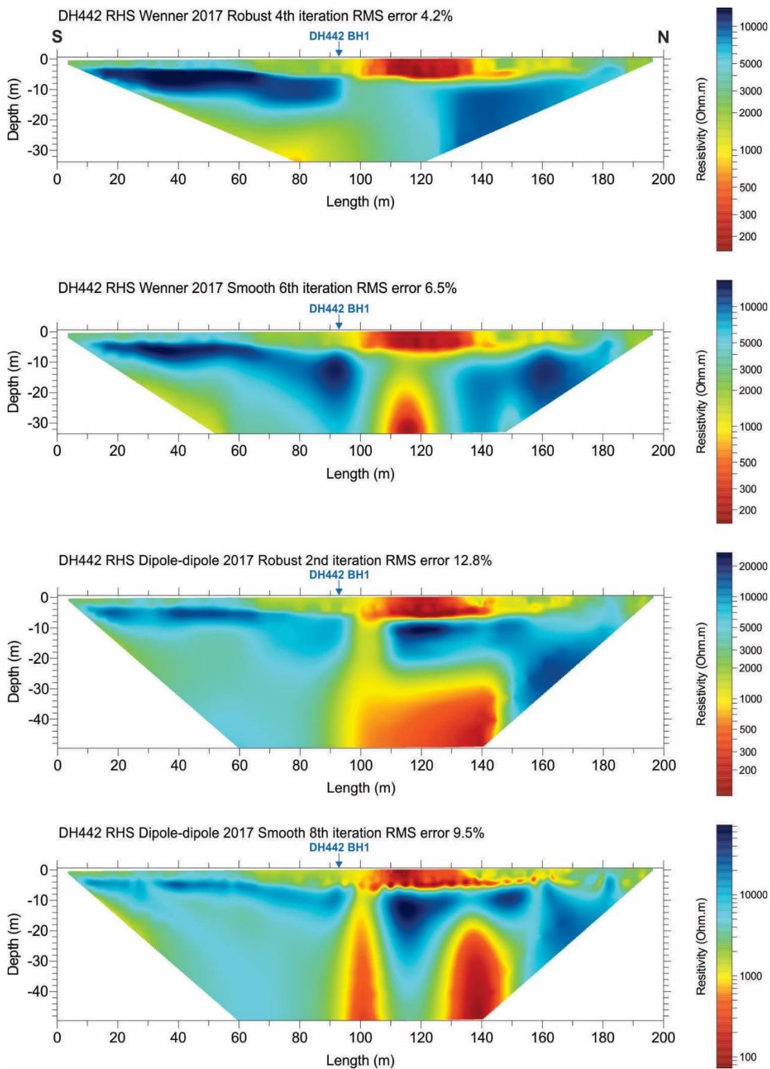
Figure 3.14.5 Wenner and dipole-dipole ERT surveys at site DH442, right-hand side (RHS), using robust and smoothed inversion processes.
