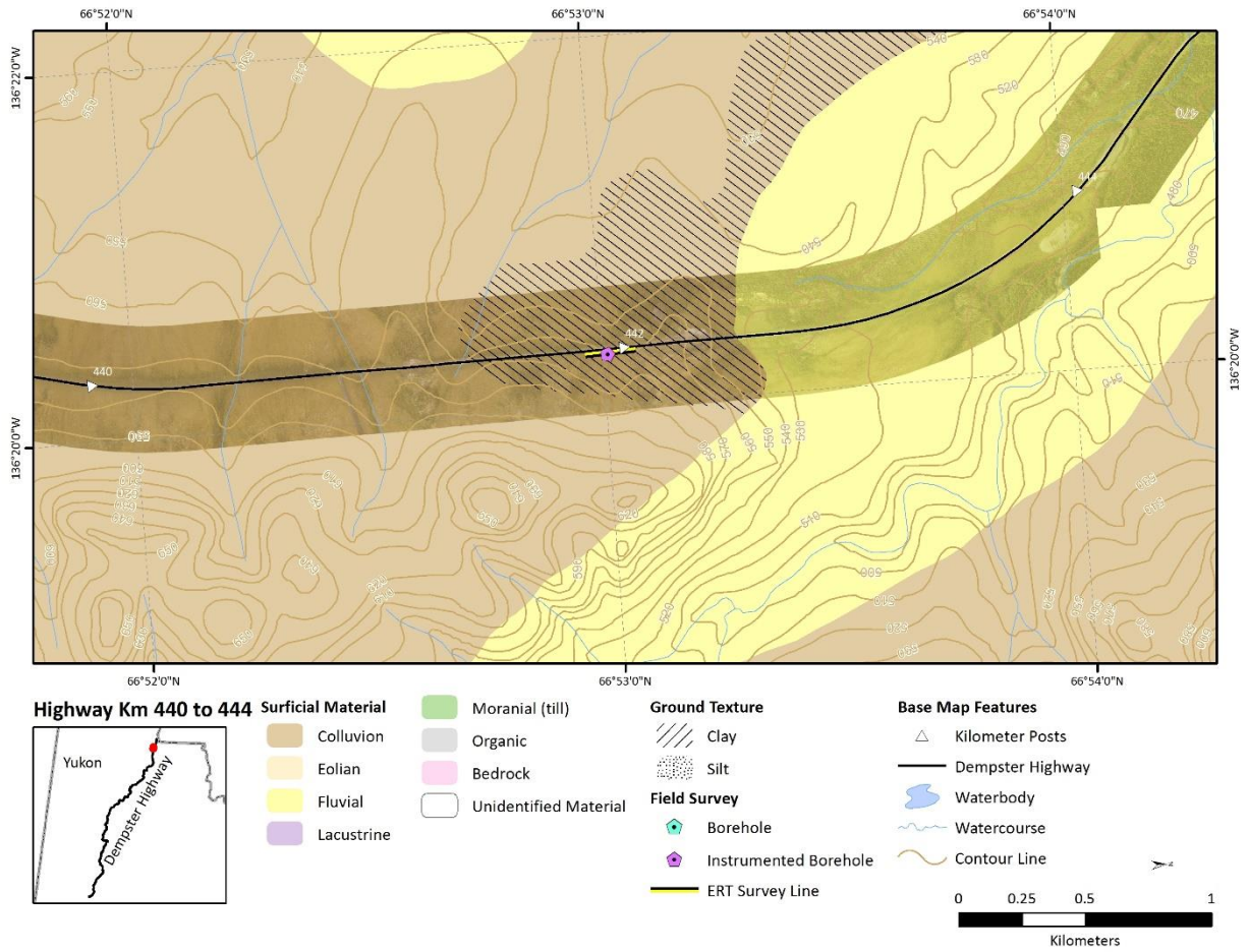
Figure 3.14.1 Surficial geology map of Site 14 DH442 area.
