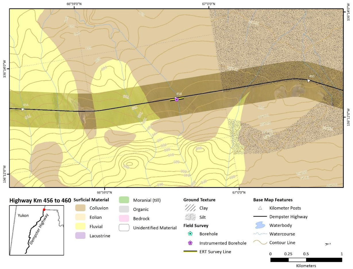
Figure 3.17.2 Surficial geology map of Site 17 DH458 area.
