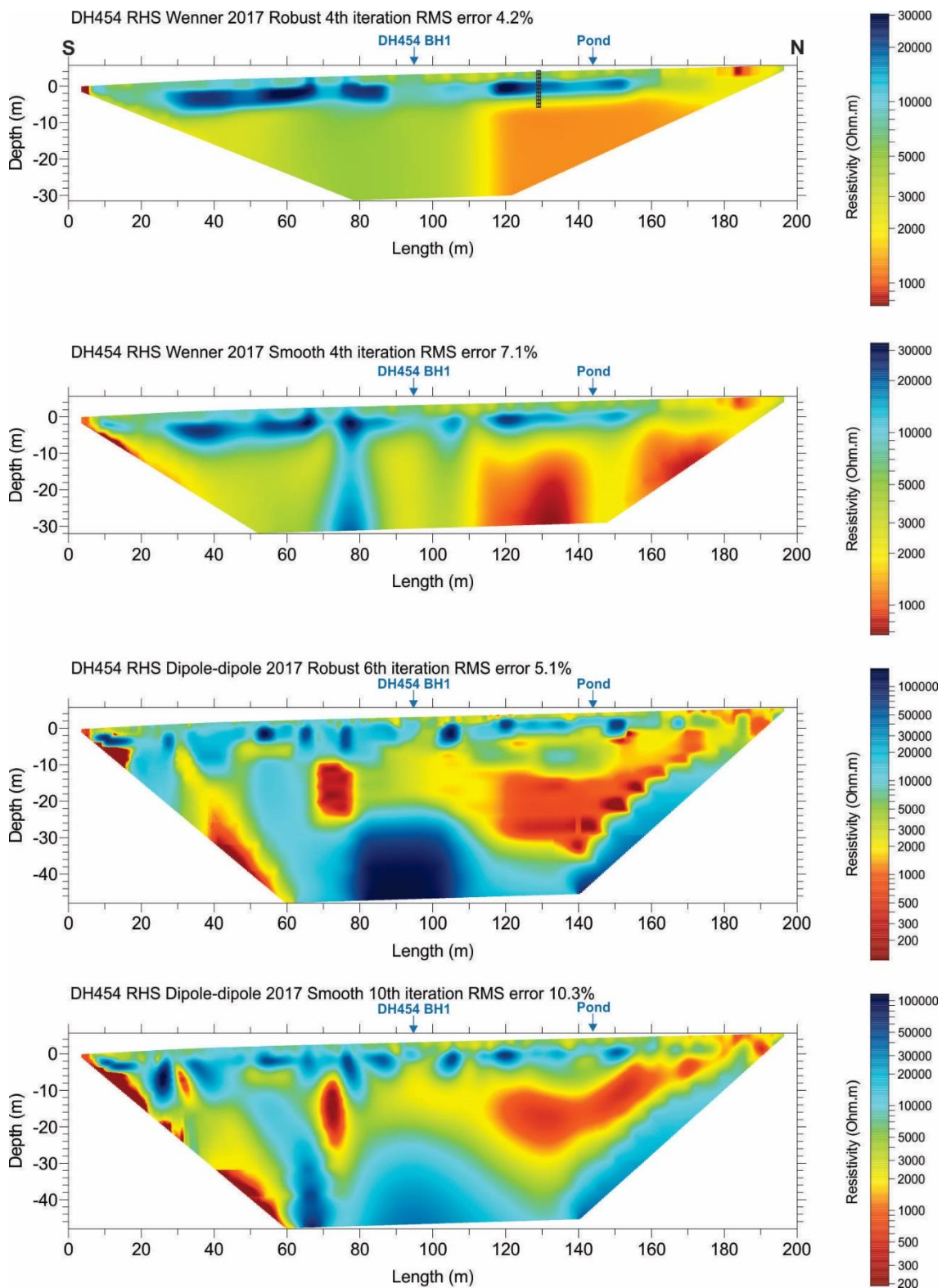
Figure 3.16.6 Wenner and dipole-dipole ERT surveys at site DH454, right-hand side (RHS), using robust and smoothed inversion processes.
