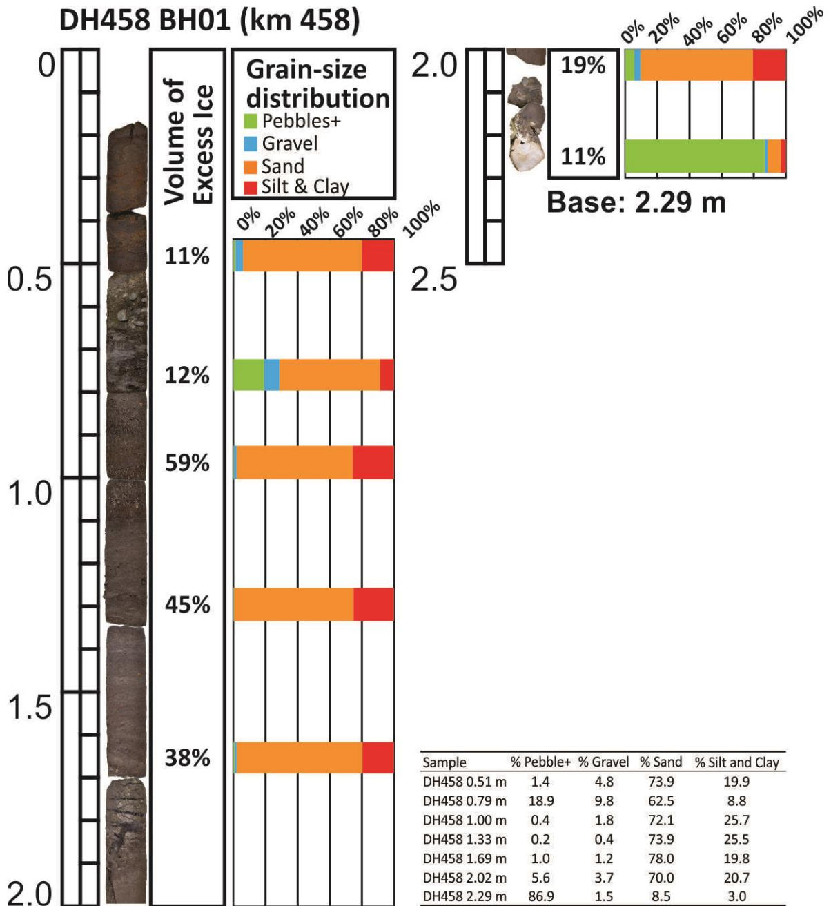
Figure 3.17.4 Logs of borehole DH458 BH1, with volumetric excess ice content and grain size distribution.
