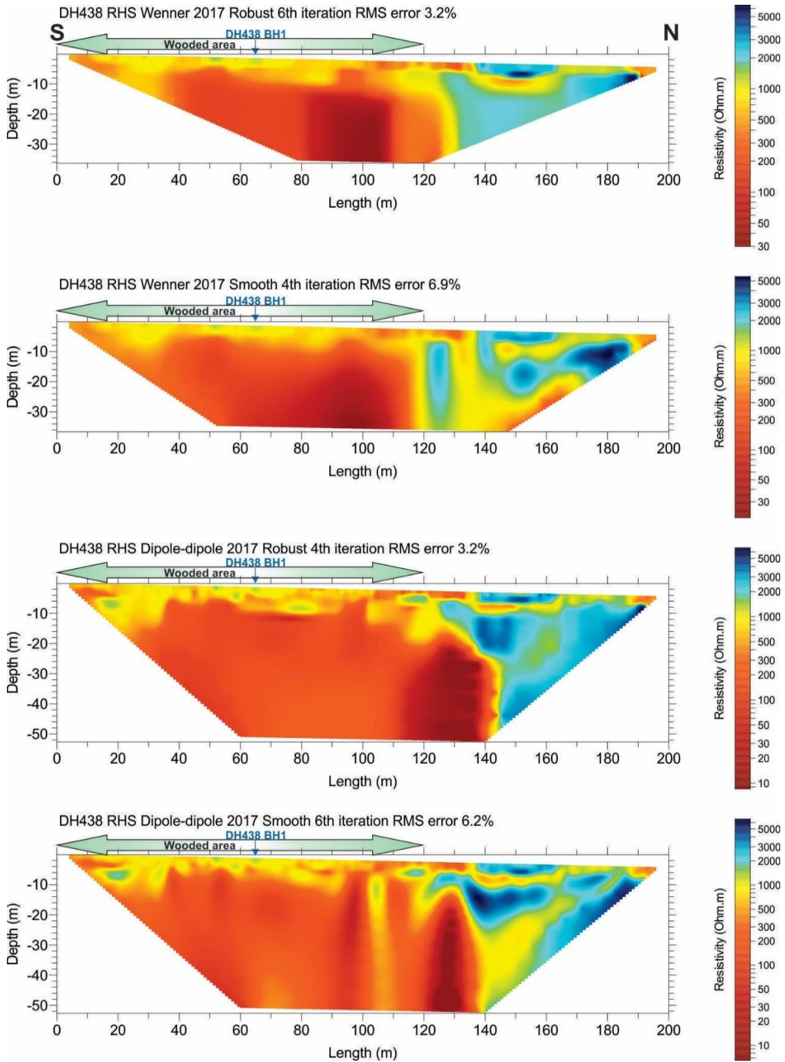
Figure 3.13.6 Wenner and dipole-dipole ERT surveys at site DH438, right-hand side (RHS), wooded and unwooded areas, using robust and smoothed inversion processes.
