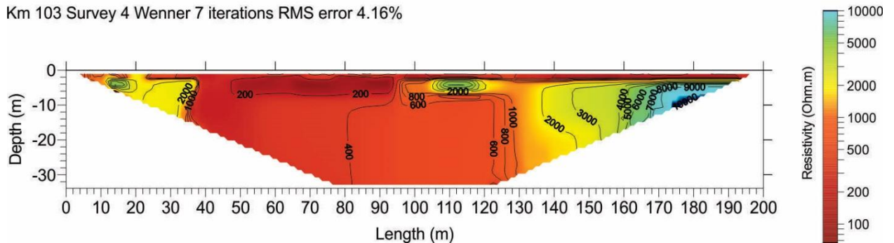
Figure 3.4.6 Wenner ERT surveys at site DH103.
