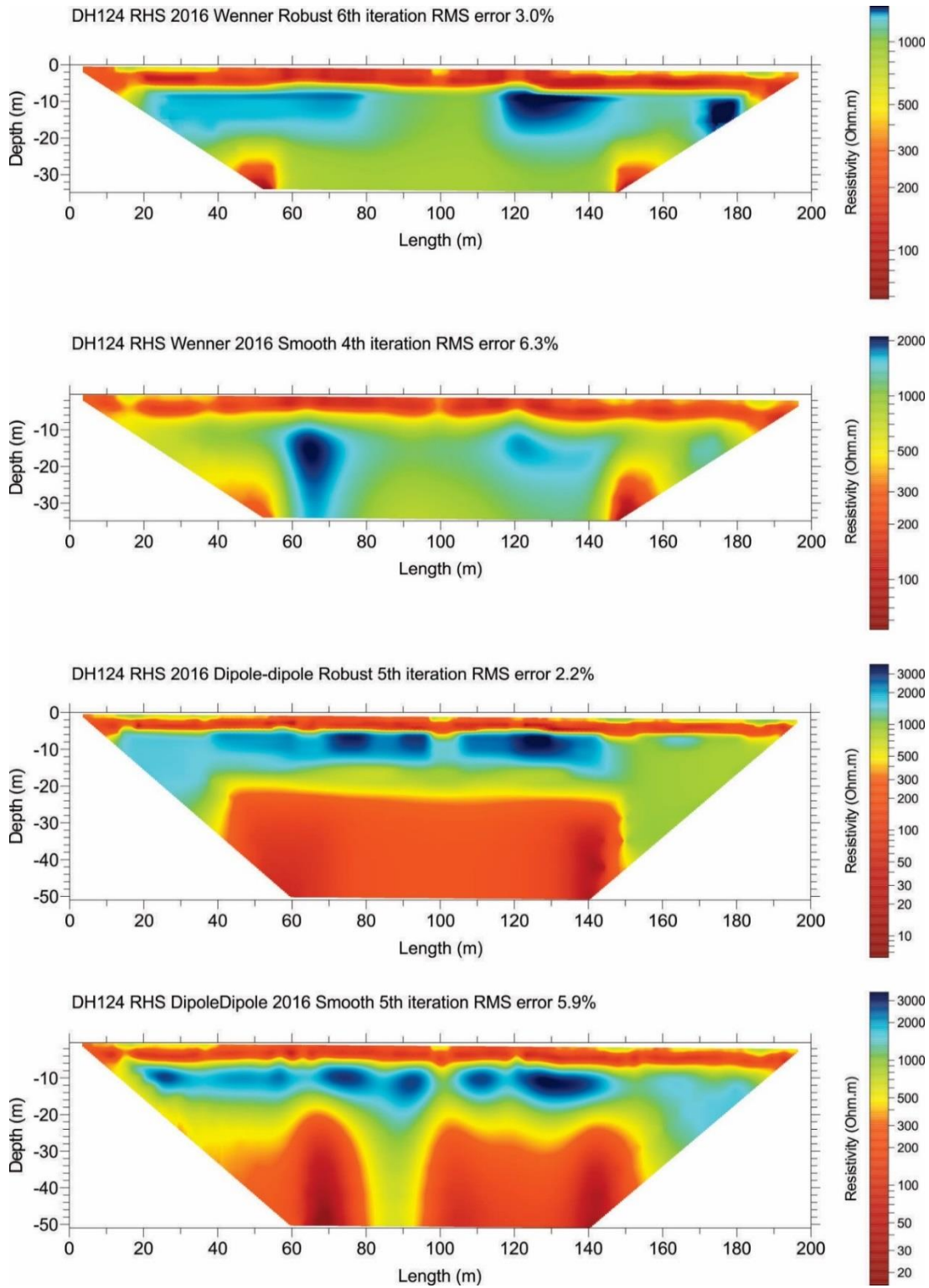
Figure 3.6.9 Wenner and dipole-dipole ERT surveys at site DH124, right-hand side (RHS), using robust and smoothed inversion processes.
