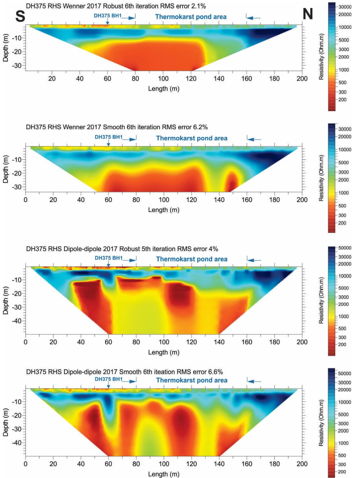
Figure 3.9.6 Wenner and dipole-dipole ERT surveys at site DH375.
