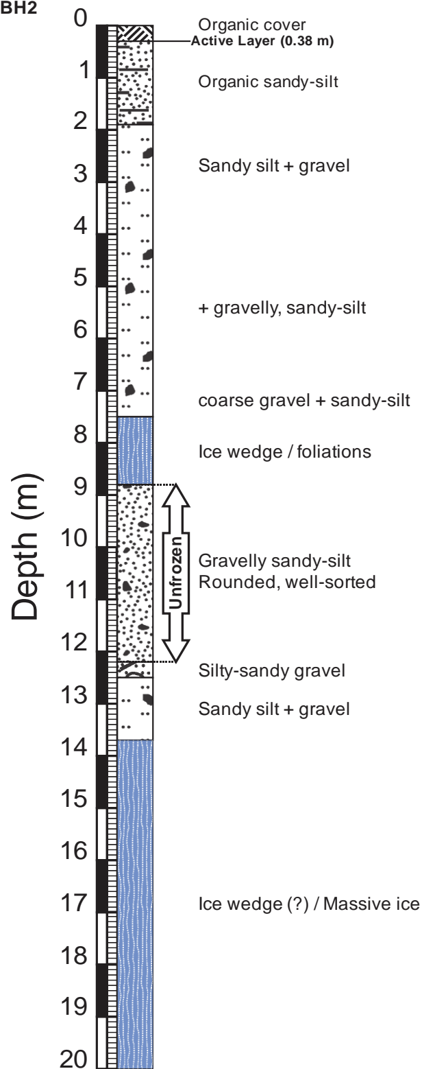
Figure 3.5.6 Preliminary log of borehole DH116 BH2 (BH5566).
