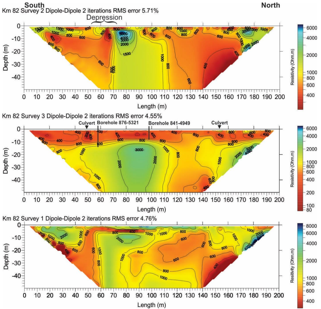
Figure 3.1.7 Dipole-dipole ERT surveys at site DH82
