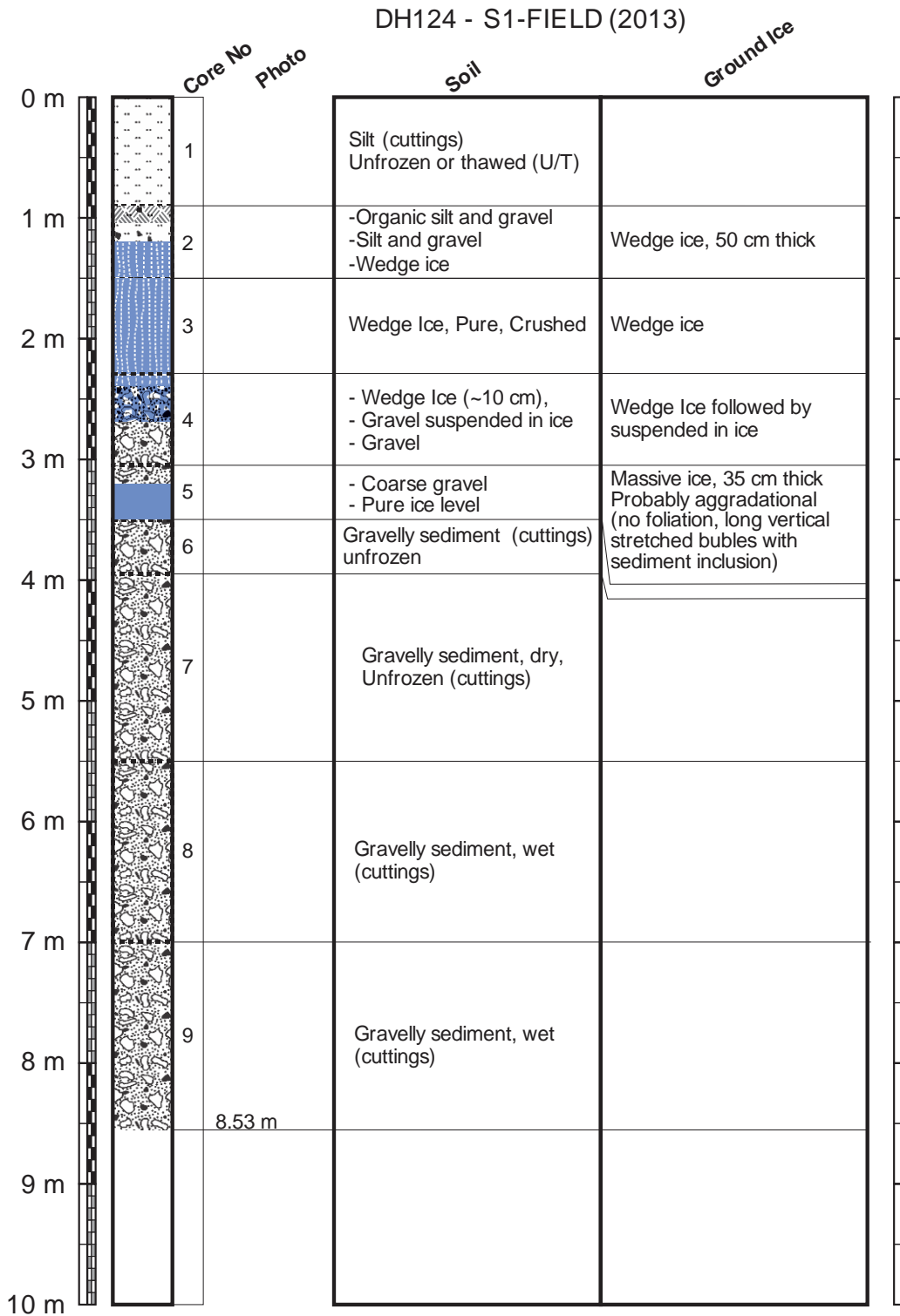
Figure 3.6.4 Log of borehole DH124 BH Field.
