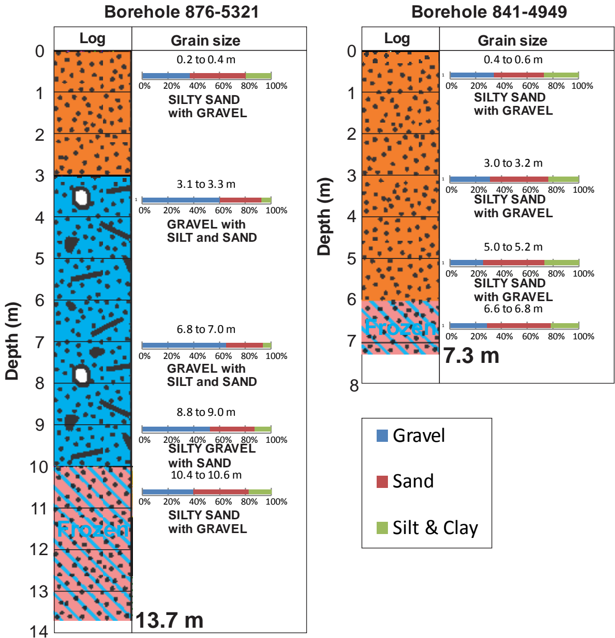
Figure 3.1.4 Logs of boreholes BH 876-5321 and BH 841-4949
