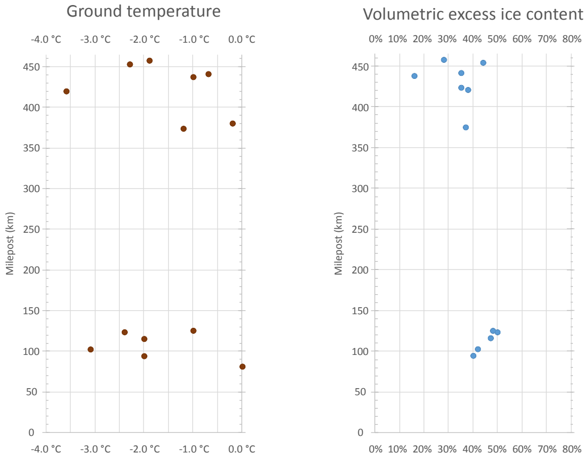
Figure 4.5.2 Ground temperature and ground ice conditions at investigated sites
