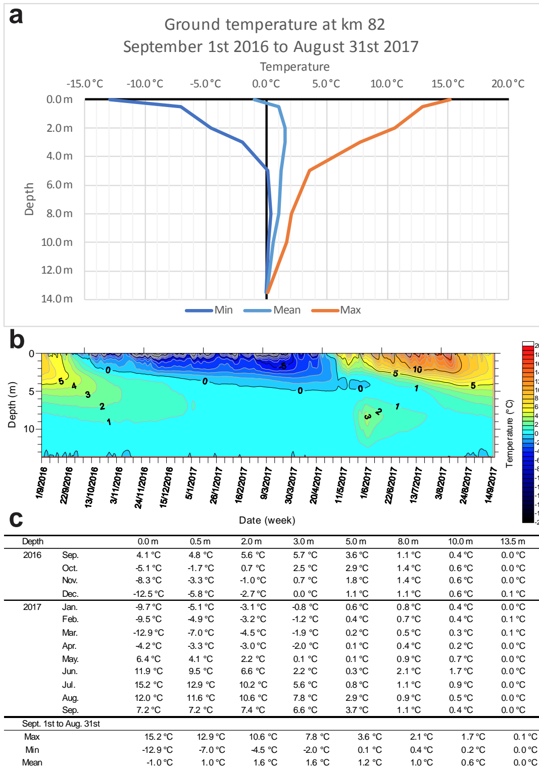
Figure 3.1.5 Ground temperature at site DH82. a- trumpet diagram; b- depth vs. time temperature diagram; c- monthly mean ground temperature
