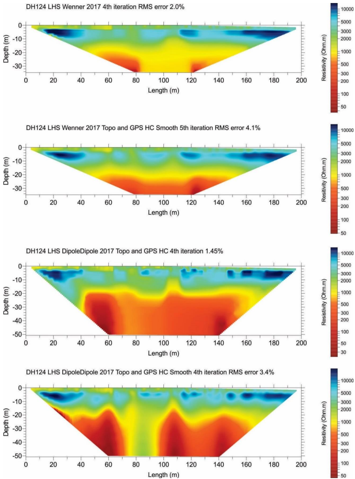
Figure 3.6.8 Wenner and dipole-dipole ERT surveys at site DH124, left-hand side (LHS), using robust and smoothed inversion processes.
