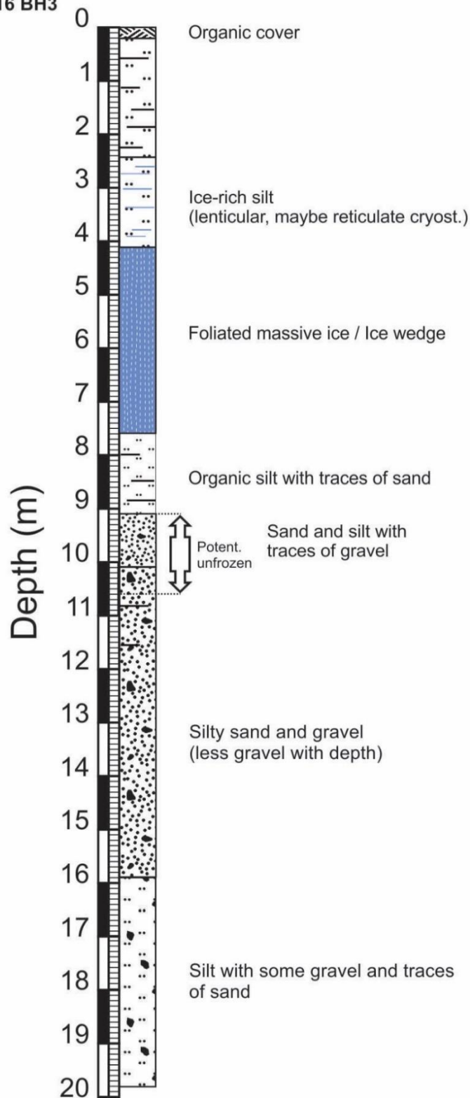
Figure 3.5.7 Preliminary log of borehole DH116 BH3 (BH5567).
