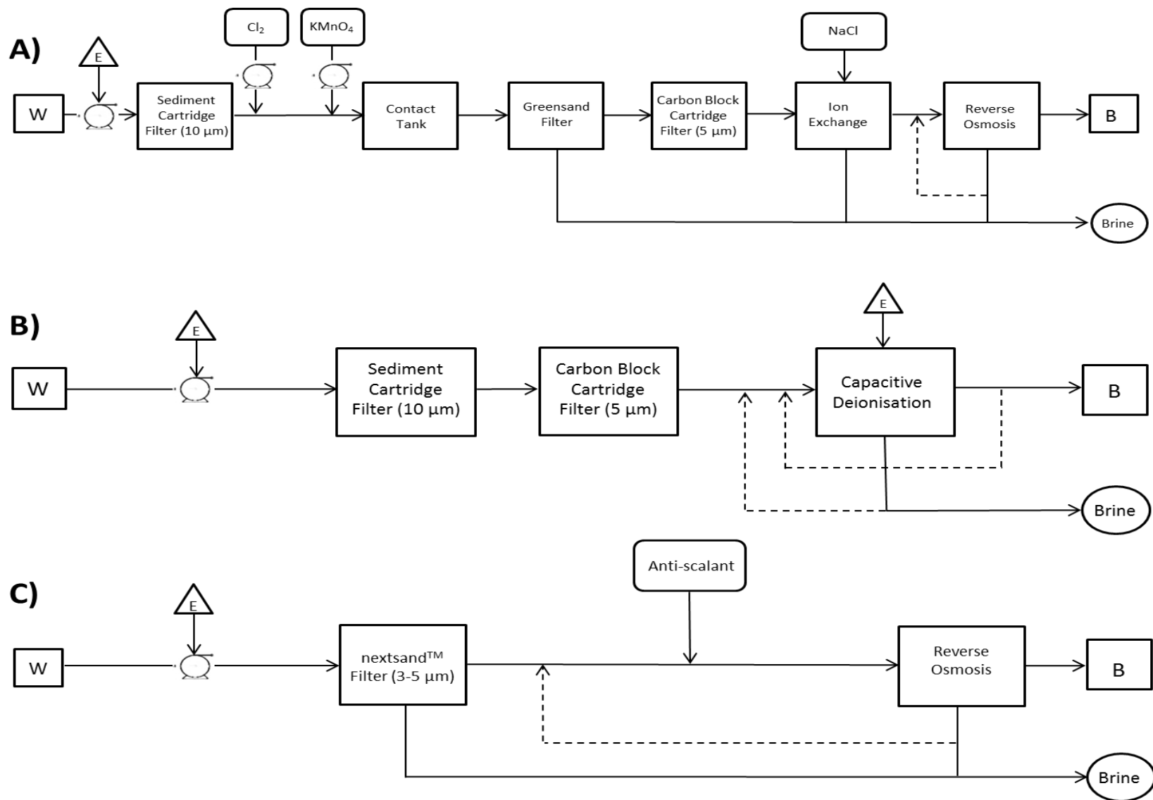
Figure 4: Layout of the three treatment trains that were compared in this study.
