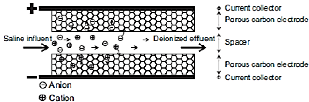
Figure 3: Capacitive Deionization principle. Adapted from nmnuclear (2014)
