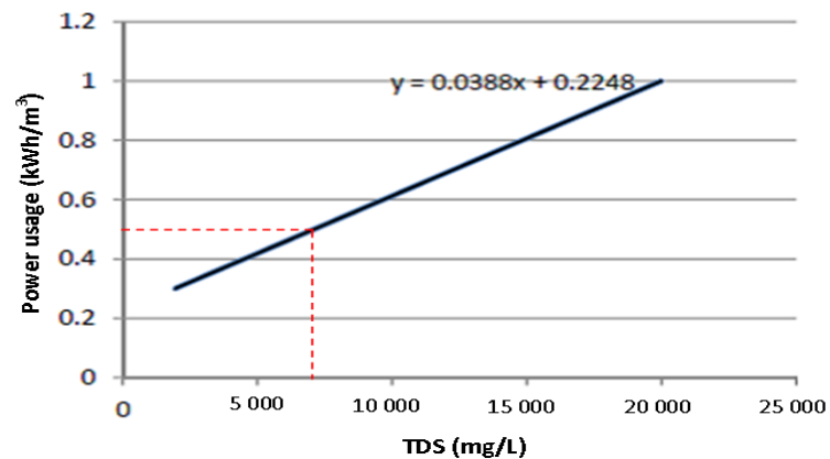
Figure 11: Power usage of one Prestige full-scale unit. The dashed lines represent the power usage (0.50 kWh/m 3 ) at a feed water content of 7 200 mg/L TDS. (adapted from EWP, 2014a)
