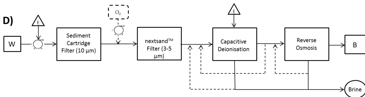
Figure 15: Recommended composite treatment train for provision of drinking water from brackish groundwater available at Northern Cross' base camp in Eagle Plains (Yukon, Canada).
