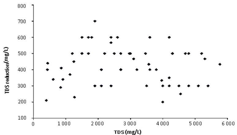
Figure 8: TDS reduction in relation to the feed water TDS content.
