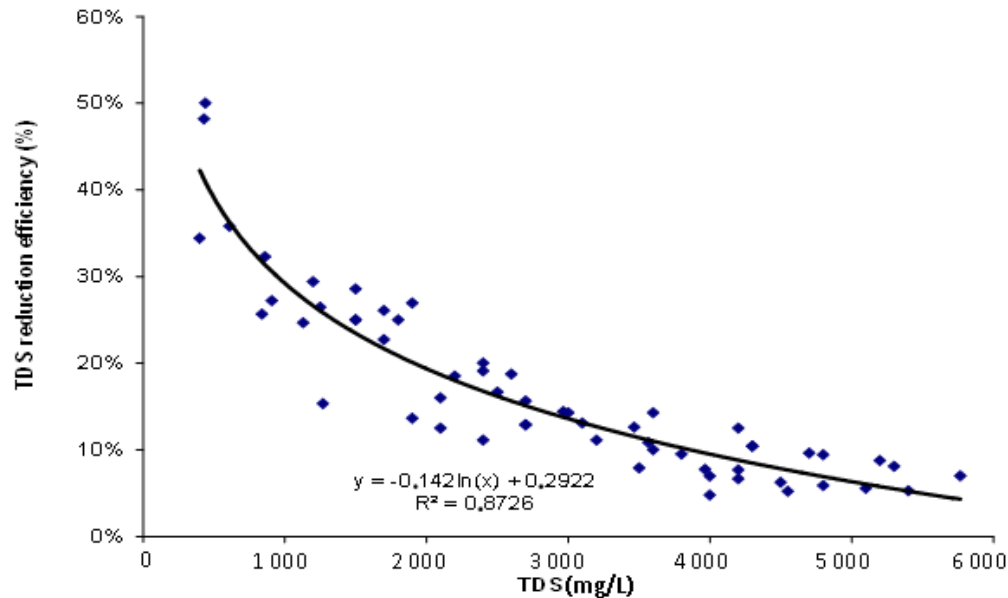
Figure 7: TDS reduction efficiency (%) of the pilot-scale capacitive deionization unit when treating cartridge-filtrated brackish groundwater.
