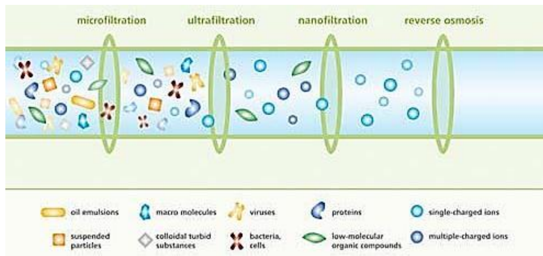
Figure 1: Particle removal capacity of filtration processes in relation to particle size. Adapted from grunbeck (2014).
