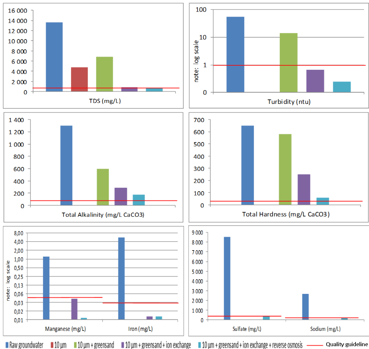
Figure 5: Water quality at the outlet of the different steps of treatment line A.
