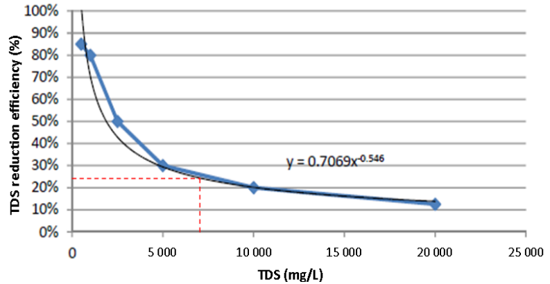
Figure 10: TDS reduction efficiency of one Prestige full-scale unit. The dashed lines represent the efficiency (24%) at a feed water content of 7 200 mg/L TDS. (adapted from EWP, 2014a)
