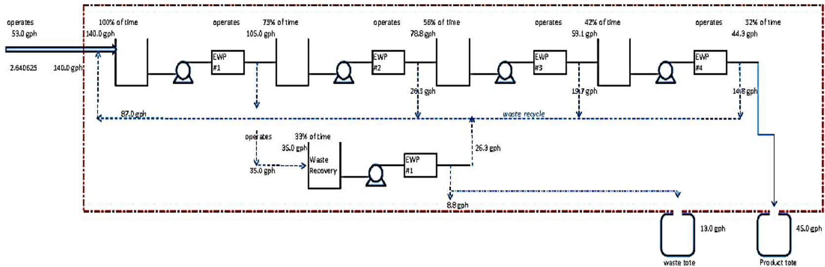
Figure 12: Illustration of a potential layout for a full-scale capacitive deionization water treatment train based on EWP's full scale Prestige units, making use of a series of 5 Prestige units (4 production stages and 1 recovery stage). (adapted from Atlas, B., 2014. pers. comm.)
