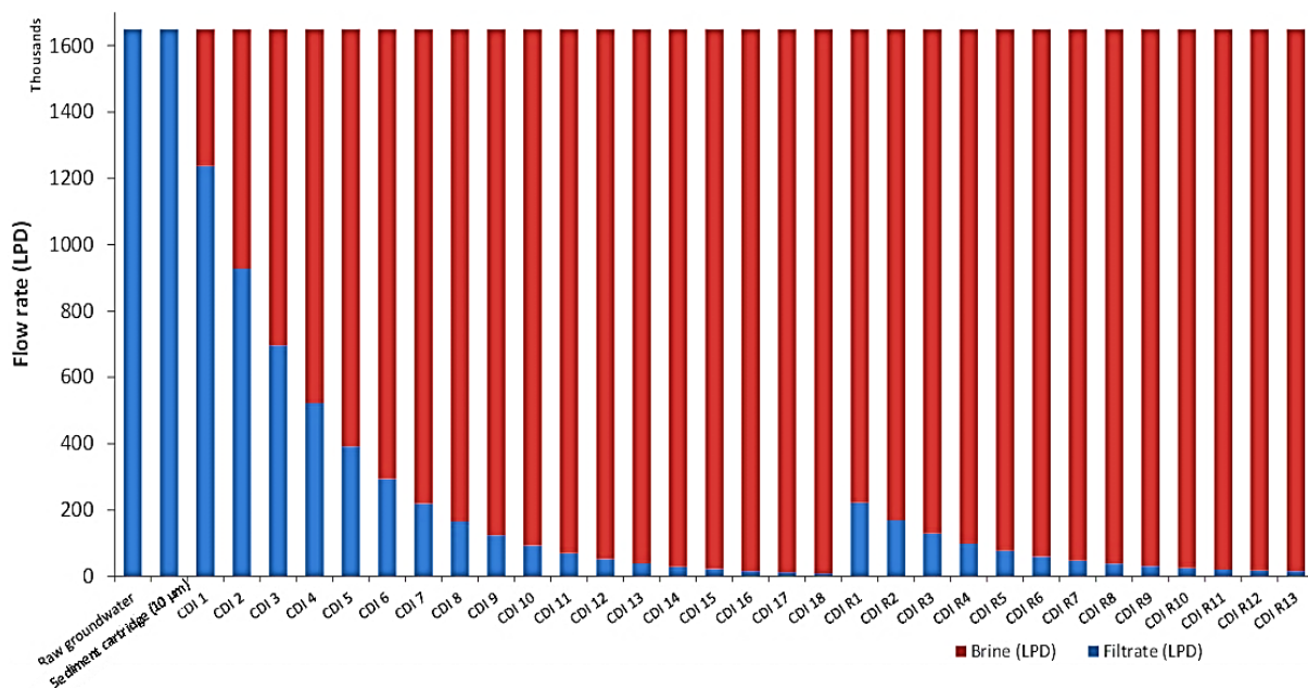
Figure 9: Water recovery observed with treatment train B, which consisted in 1 Sediment cartridge stage, 18 Capacitive deionization production stages (CDI), and 13 Capacitive deionization (CDI) recovery stages (CDI R).
