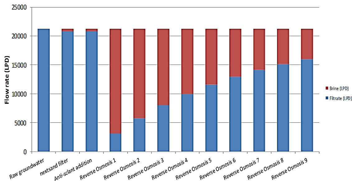
Figure 13: Water recovery observed with treatment train C, which consisted in 1 nextsand TM stage, and 9 Reverse osmosis stages.
