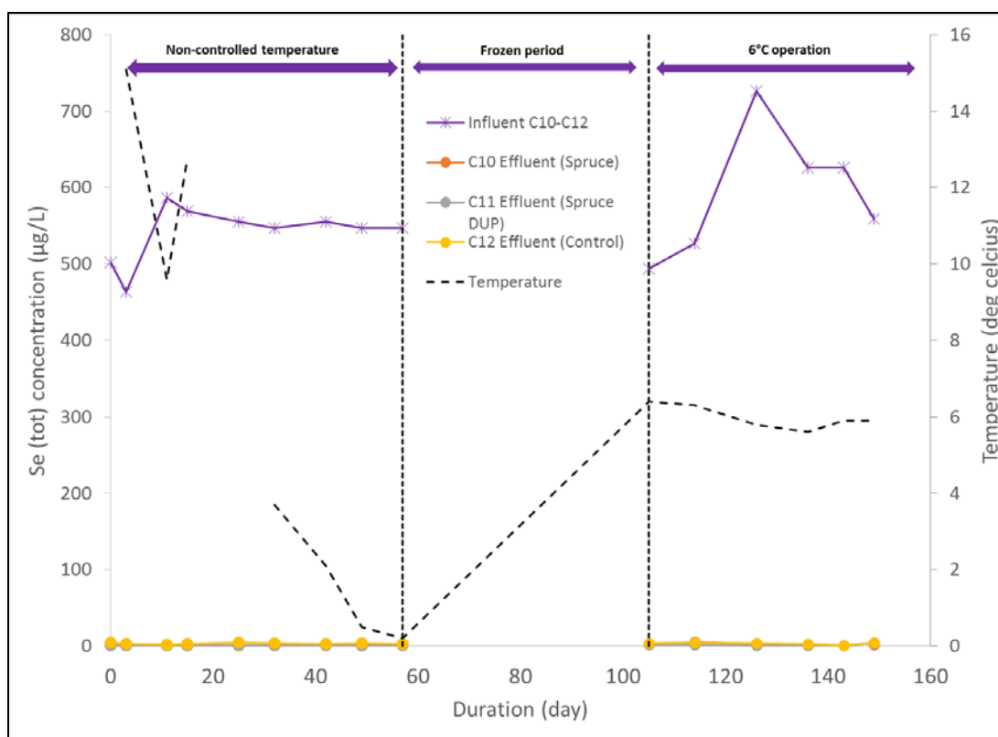
Figure 16. Se concentration in the influent and effluents from the C10-12 reactors (Phases 1-3; quantification limit is 0.7 µg/L, value below the limits are reported as 0.7)
