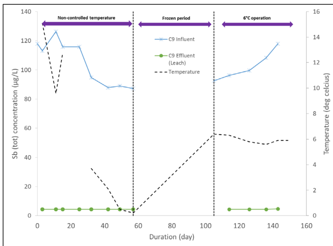
Figure 10. Sb concentrations in influent and effluents from the C9 reactor (Phases 1-3; quantification limit is 4.3 µg/L, value below the limits are reported as 4.3)
