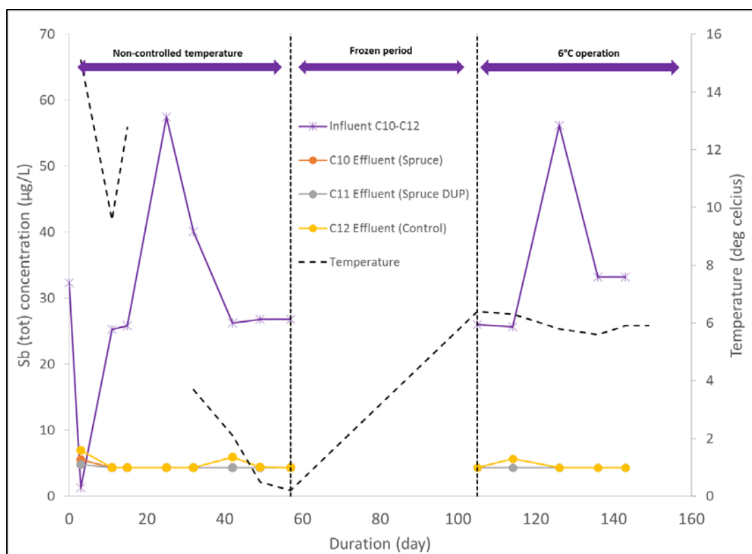
Figure 15. Sb concentrations in influent and effluents from the C10-12 reactors (Phases 1-3; quantification limit is 4.3 µg/L, value below the limits are reported as 4.3)
