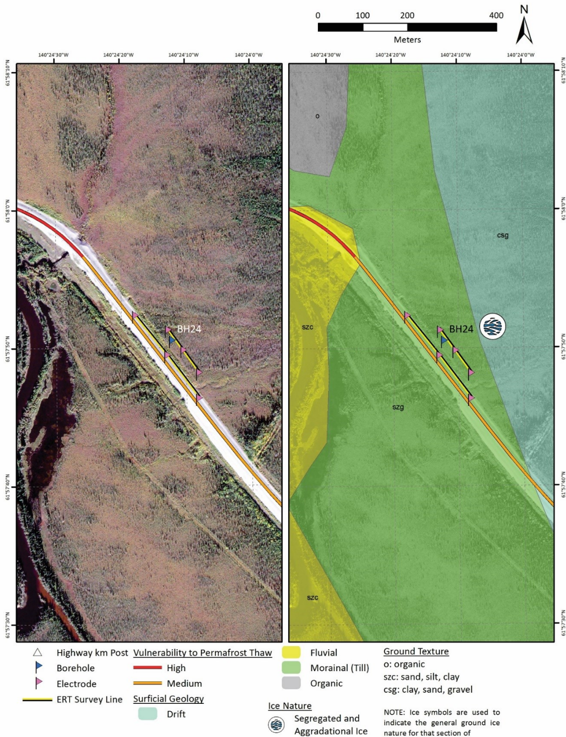
Figure 4.1.1. Vulnerability maps of Site 1 (satellite imagery and surficial geology)
