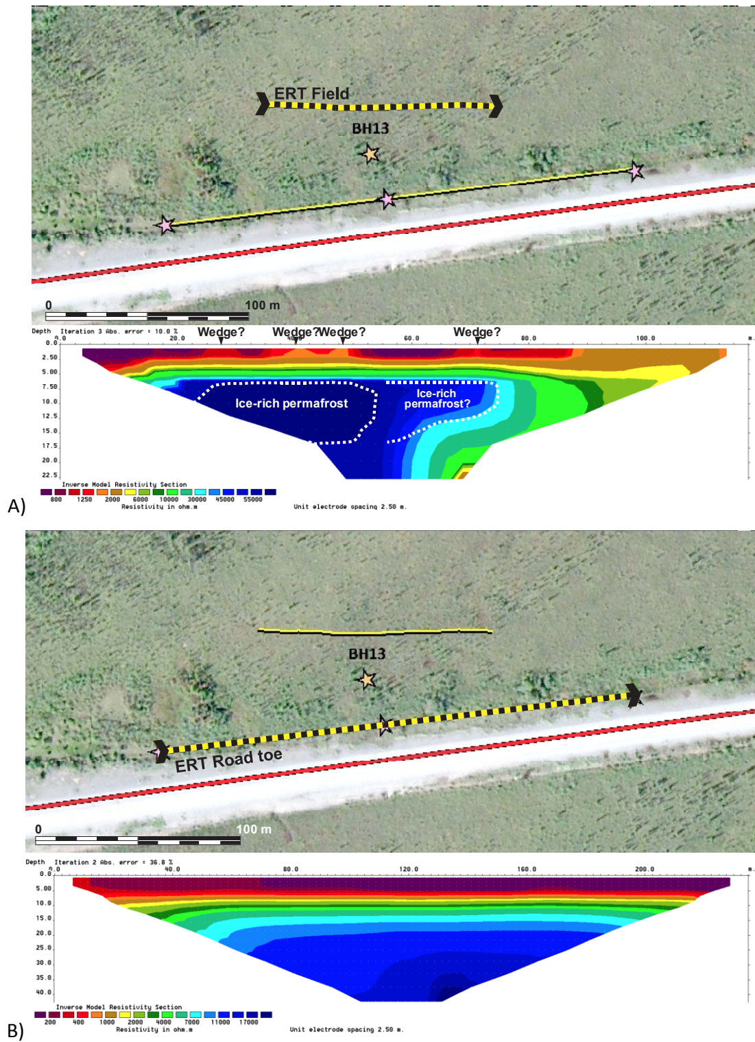
Figure 4.4.6. ERT Surveys performed at borehole BH13 for A) the field west of the BH13; and B) the toe of the highway embankment.
