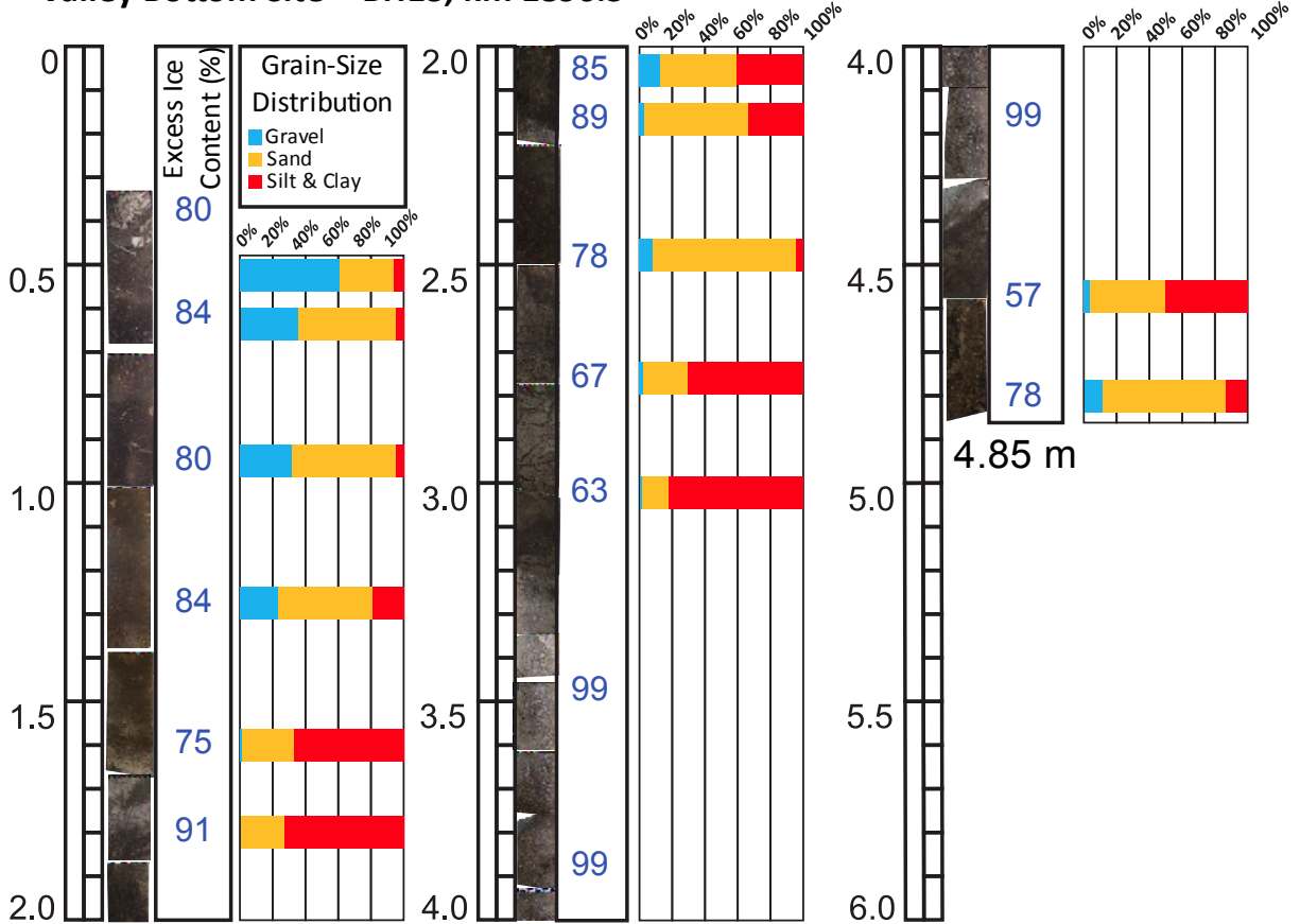
Figure 4.4.2. Log of borehole BH13.
