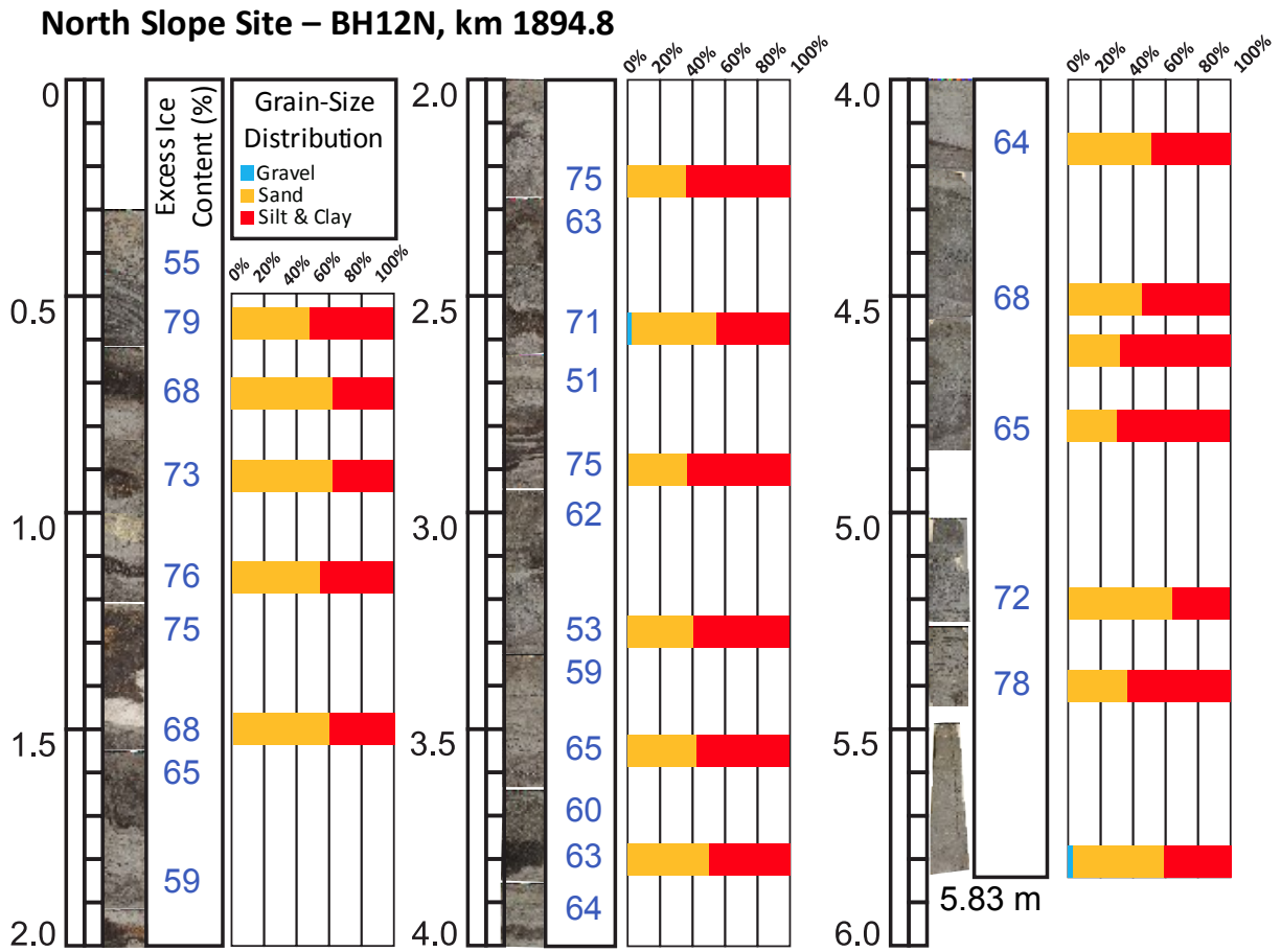
Figure 4.6.4. Log of borehole BH12N.
