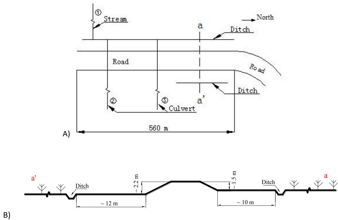
Figure 4.6.9. Schematic illustration of the North of Beaver Creek adaptation site for A) Localisation of proposed embankment cross section in transverse profile; and B) a-a' embankment cross section, km 1894.8
