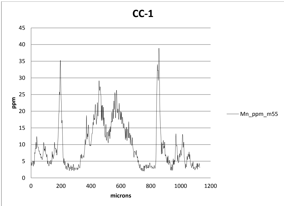
Figure 23 Manganese profile of the sculpin CC-1
