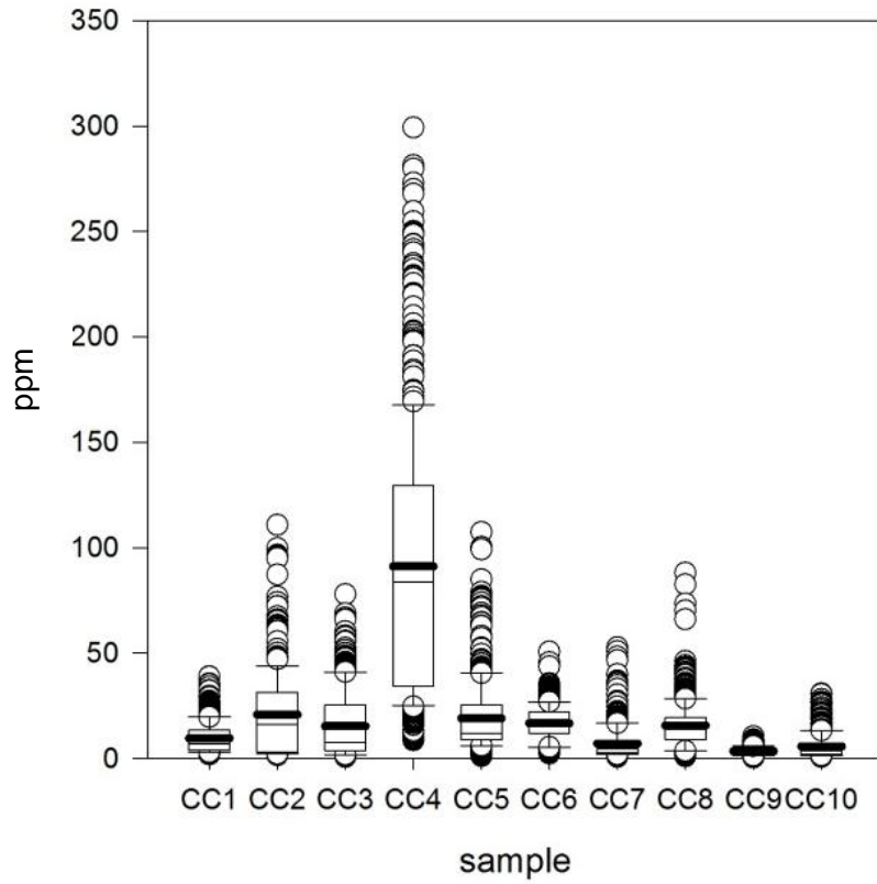
Figure 39 Plots showing Mn data for the sculpin from Christal Creek. Individual sample plots show data range, the boxes 25 th and 75 th percentile of the data, whiskers 10 th and 90 th percentile, and median (thin line) and mean (thick line).
