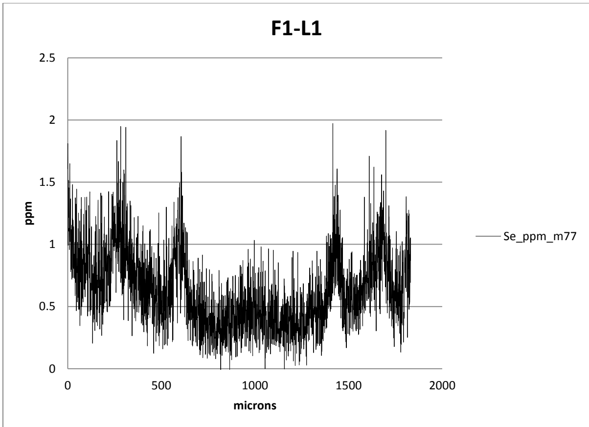
Figure 17 Selenium profile of the F1-L1 grayling individual
