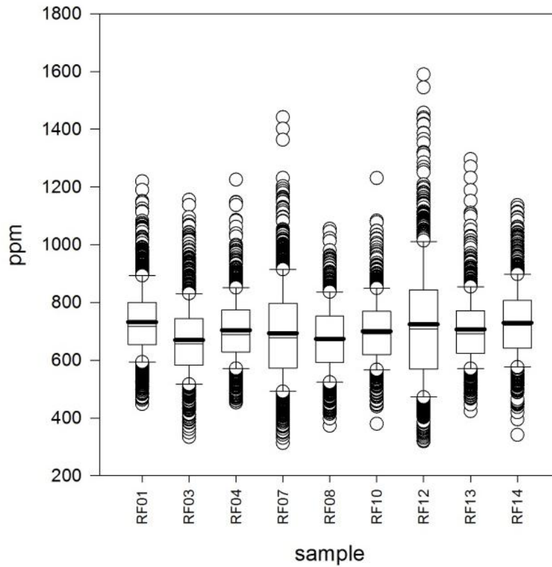
Figure 30 Plots showing Sr data for the grayling from Moose Creek. Individual sample plots show data range, the boxes 25 th and 75 th percentile of the data, whiskers 10 th and 90 th percentile, and median (thin line) and mean (thick line).
