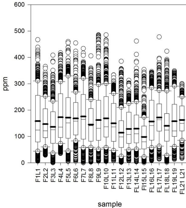
Figure 35 Plots showing Zn data for the grayling from Christal Creek. Individual sample plots show data range, the boxes 25 th and 75 th percentile of the data, whiskers 10 th and 90 th percentile, and median (thin line) and mean (thick line).
