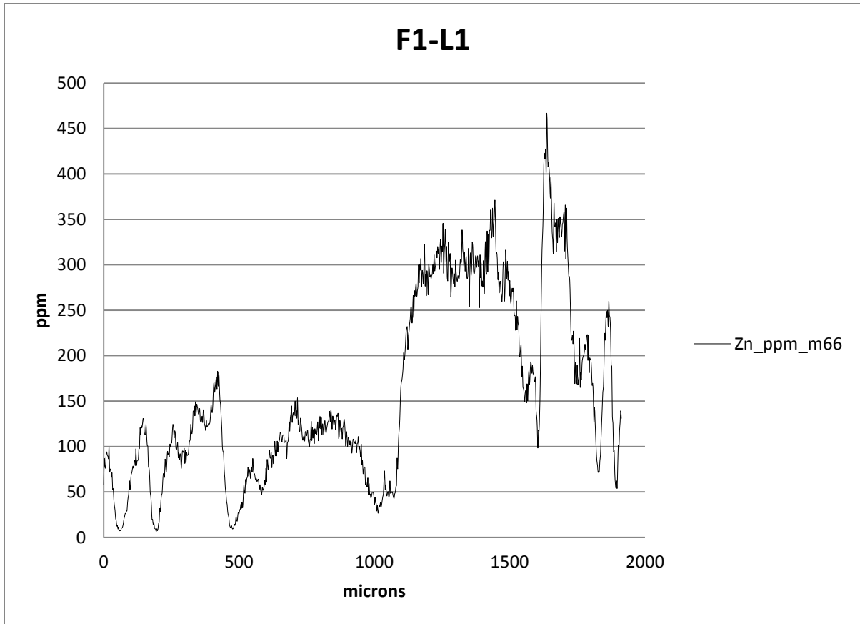
Figure 14 Zinc profile of the F1-L1 grayling individual
