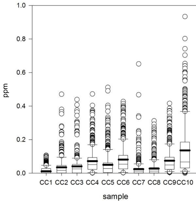
Figure 37 Plots showing Pb data for the sculpin from Christal Creek. Individual sample plots show data range, the boxes 25 th and 75 th percentile of the data, whiskers 10 th and 90 th percentile, and median (thin line) and mean (thick line).
