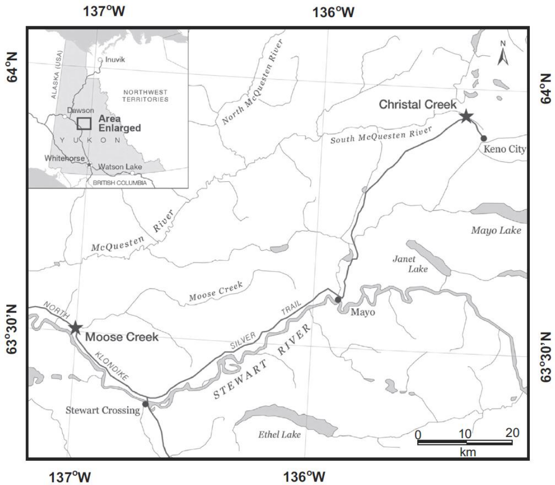
Figure 5 Moose Creek near Stewart Crossing and Christal Creek, near Keno, are indicated by stars (figure from Veldhoen et al 2014)
