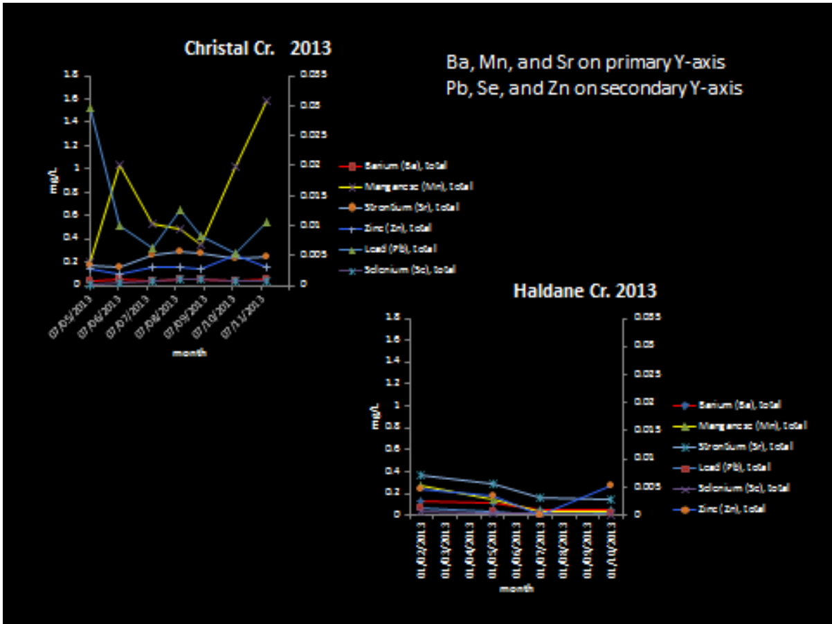
Figure 29 Comparison of water quality data from Christal and Haldane Creeks for 2013. Trace element concentrations are lower in Haldane Creek and Mn and Pb in particular are higher in Christal Creek
