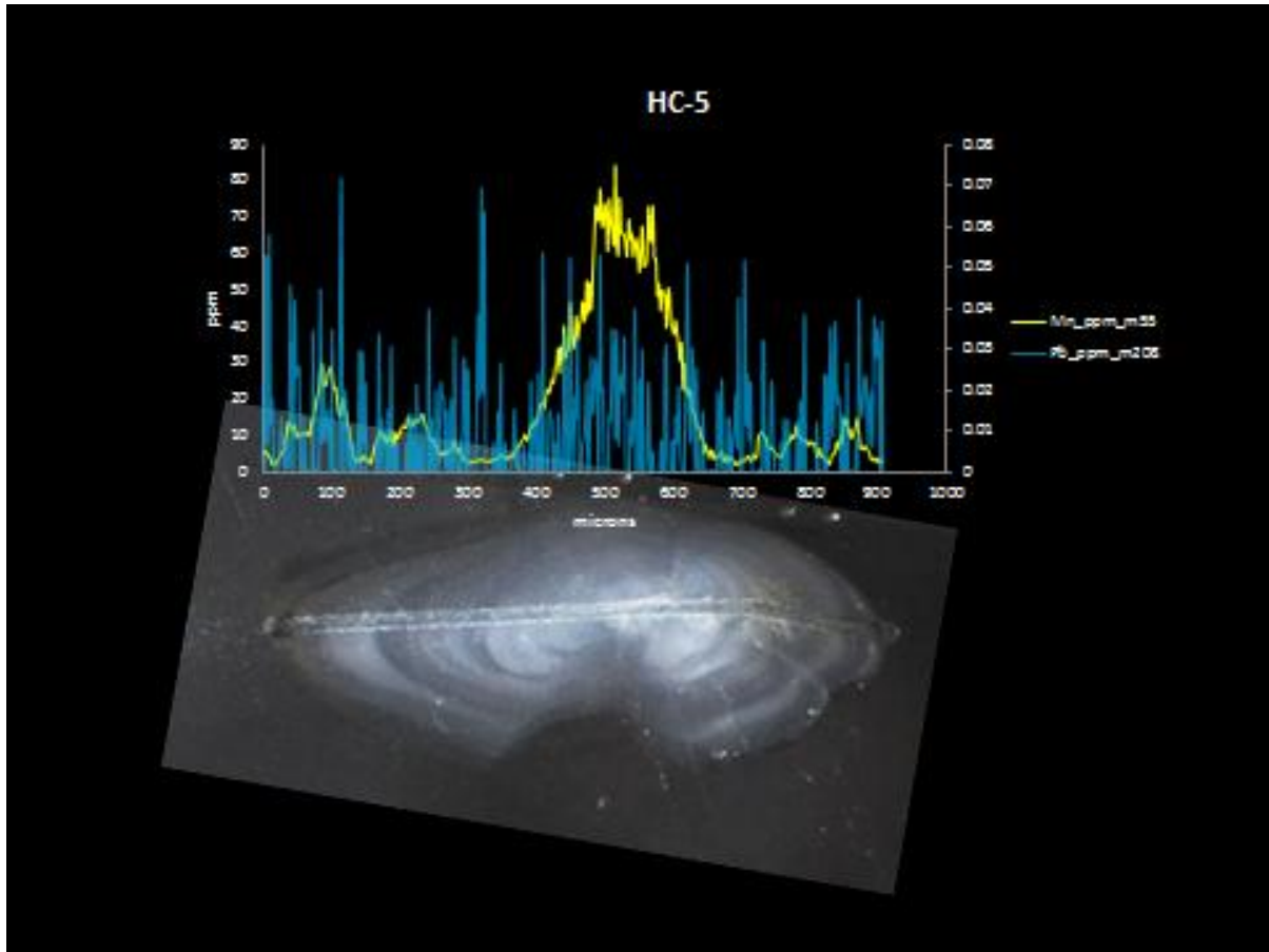
Figure 27 LA-ICP-MS linescan data for Mn (yellow), and Pb (blue) overlaid on a reflected light optical image of a 3 year old sculpin otolith from Haldane Creek. In comparison to Christal Creek the Pb concentrations are very low approaching what might be background levels. Mn is typically elevated in the primordial region for the Haldane Creeksamples with periodic increases also showing up in later annuli, but at a level lower than the primordium (note: metal values are expressed in ppm).
