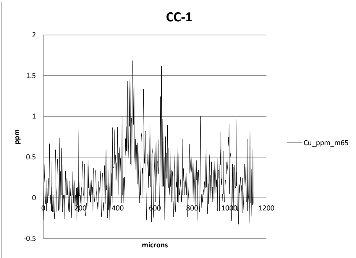
Figure 25 Copper profile of the sculpin CC-1
