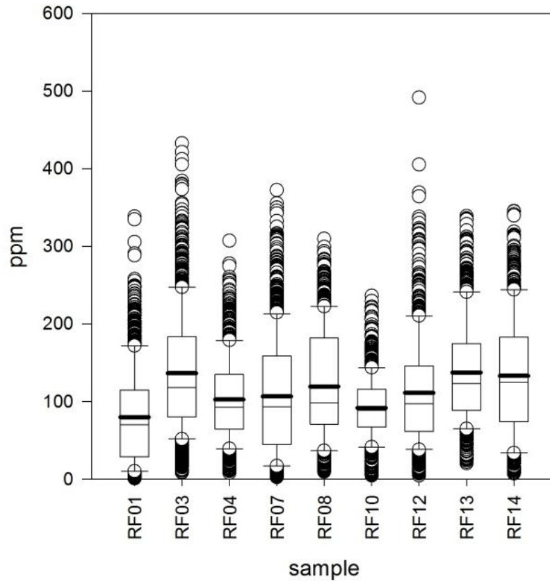
Figure 34 Plots showing Zn data for the grayling from Moose Creek. Individual sample plots show data range, the boxes 25 th and 75 th percentile of the data, whiskers 10 th and 90 th percentile, and median (thin line) and mean (thick line).
