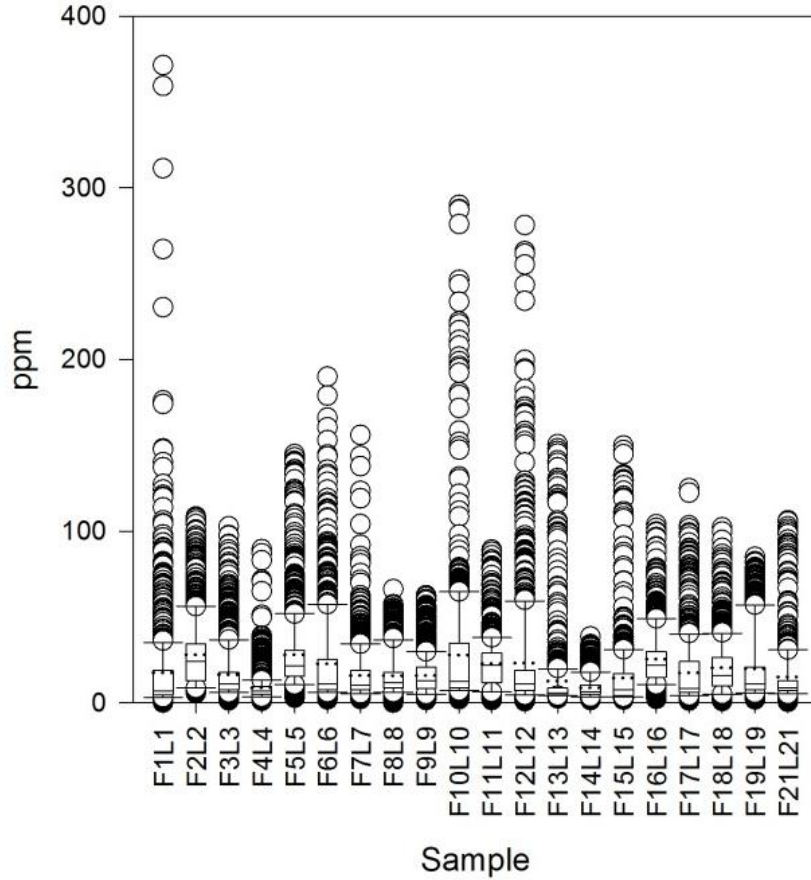
Figure 33 Plots showing Mn data for the grayling from Christal Creek. Individual sample plots show data range, the boxes 25 th and 75 th percentile of the data, whiskers 10 th and 90 th percentile, and median (thin line) and mean (dotted line).
