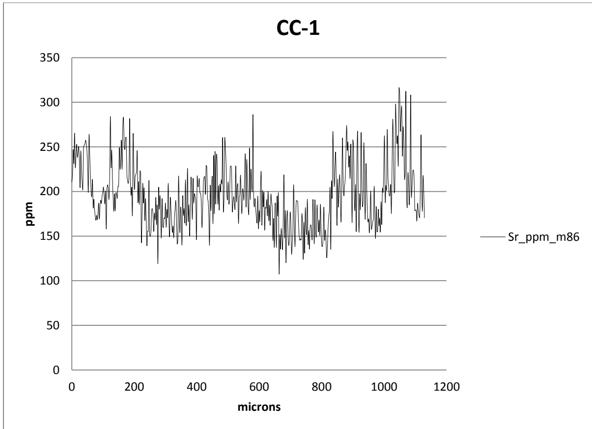
Figure 22 Strontium profile of the sculpin CC-1
