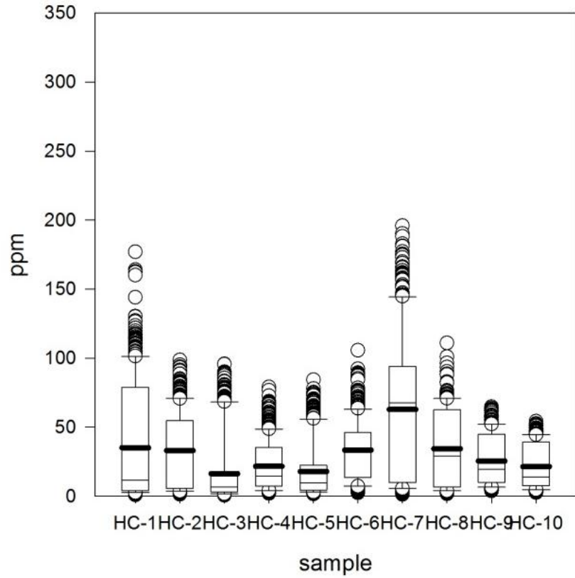
Figure 38 Plots showing Mn data for the sculpin from Haldane Creek. Individual sample plots show data range, the boxes 25 th and 75 th percentile of the data, whiskers 10 th and 90 th percentile, and median (thin line) and mean (thick line).
