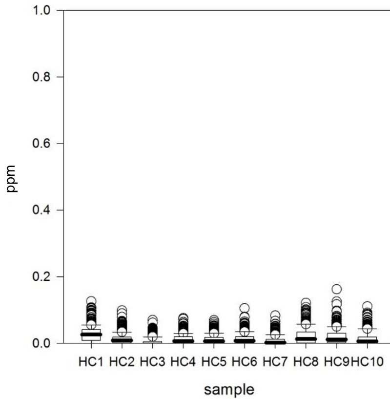
Figure 36 Plots showing Pb data for the sculpin from Haldane Creek. Individual sample plots show data range, the boxes 25 th and 75 th percentile of the data, whiskers 10 th and 90 th percentile, and median (thin line) and mean (thick line).
