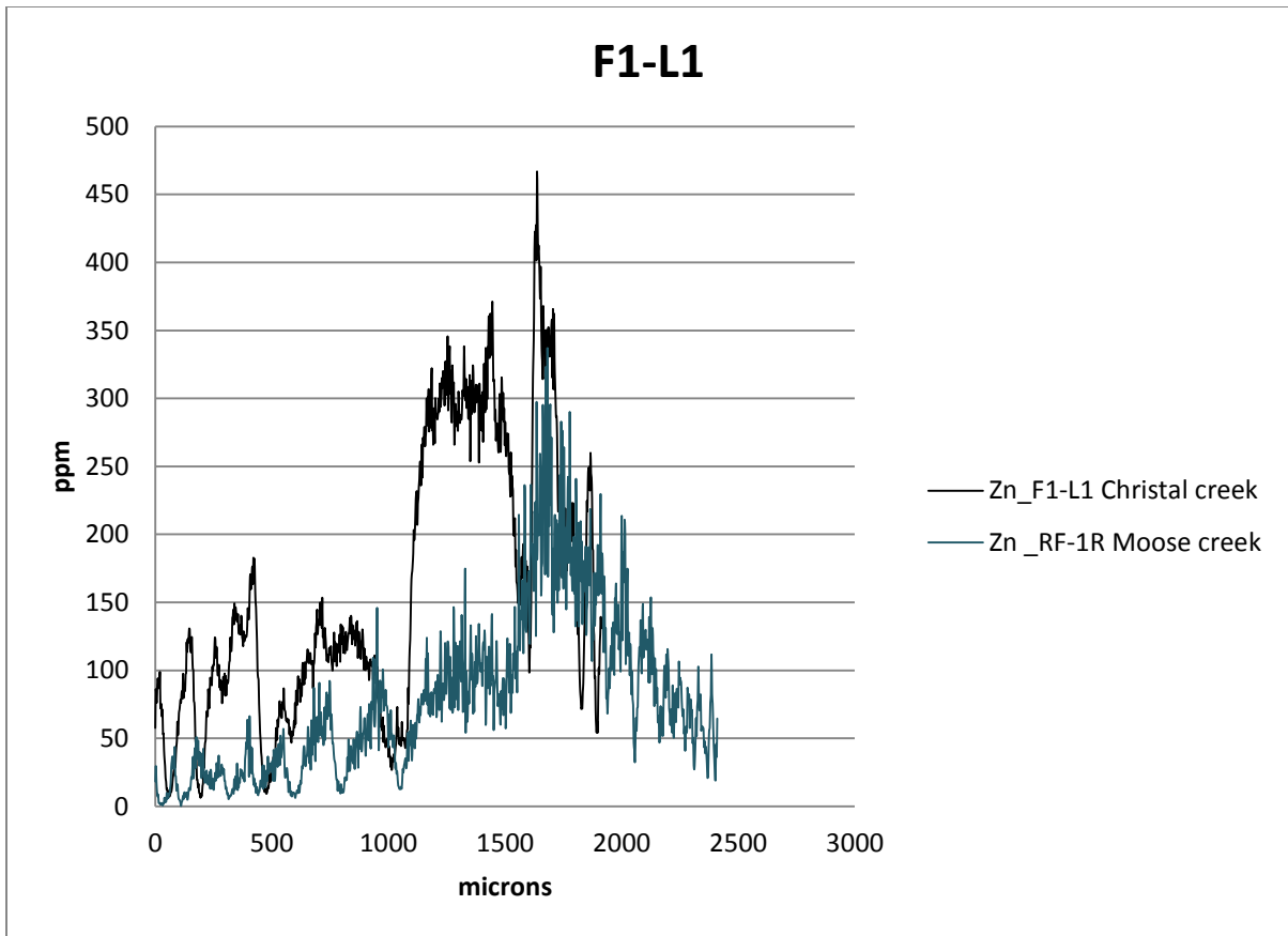
Figure 18 Zinc profiles for two individuals from Christal Creek and Moose Creek (F1-L1 and RF-1R)
