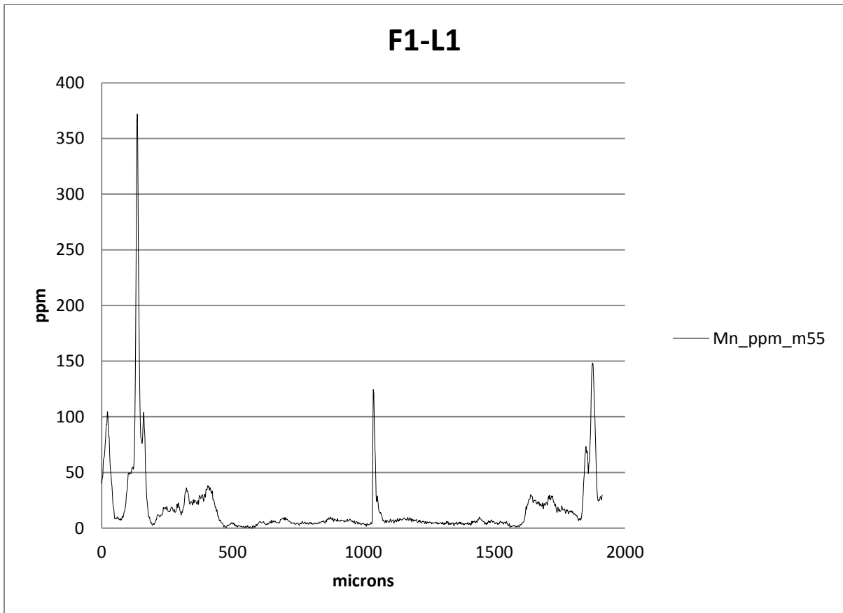
Figure 16 Manganese profile of the F1-L1 grayling individual
