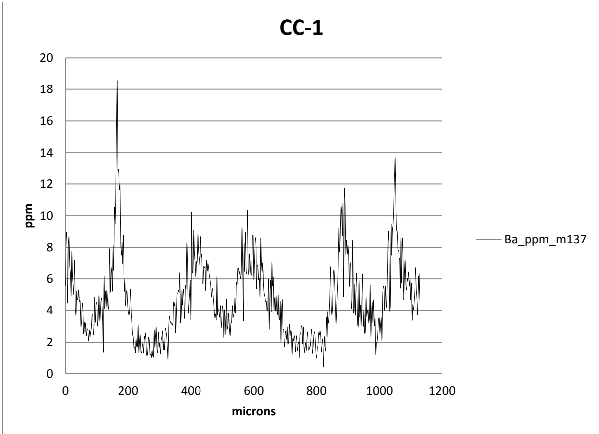
Figure 24 Barium profile of the sculpin CC-1
