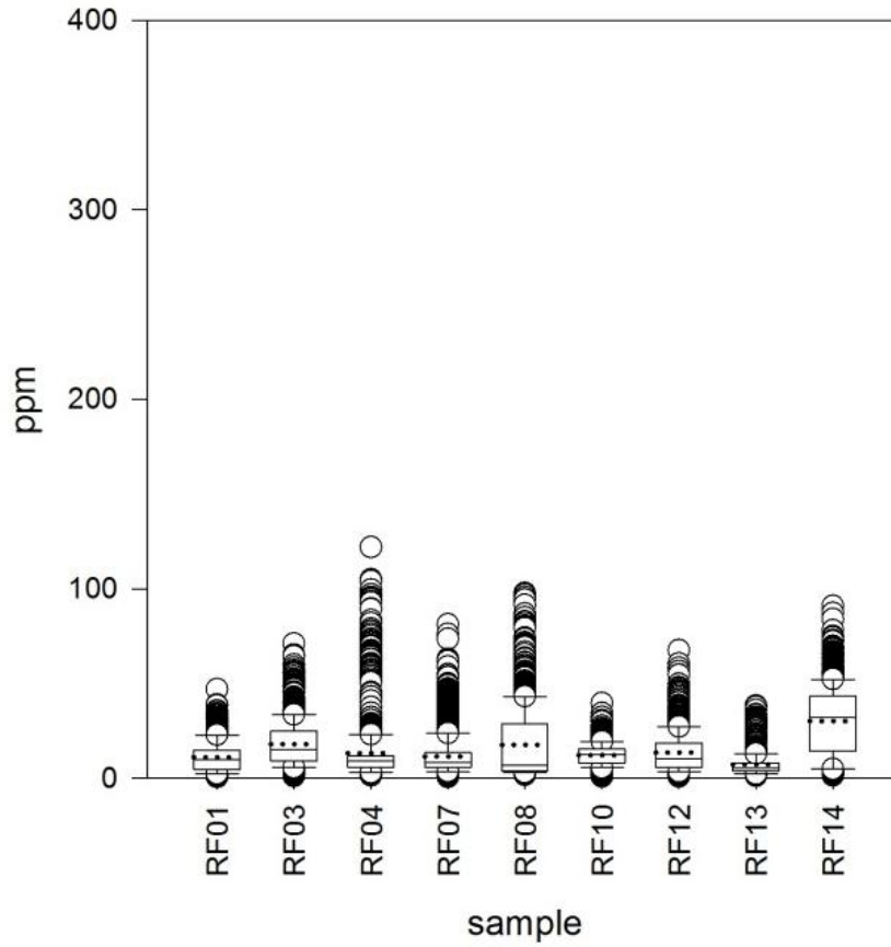
Figure 32 Plots showing Mn data for the grayling from Moose Creek. Individual sample plots show data range, the boxes 25 th and 75 th percentile of the data, whiskers 10 th and 90 th percentile, and median (thin line) and mean (dotted line).
