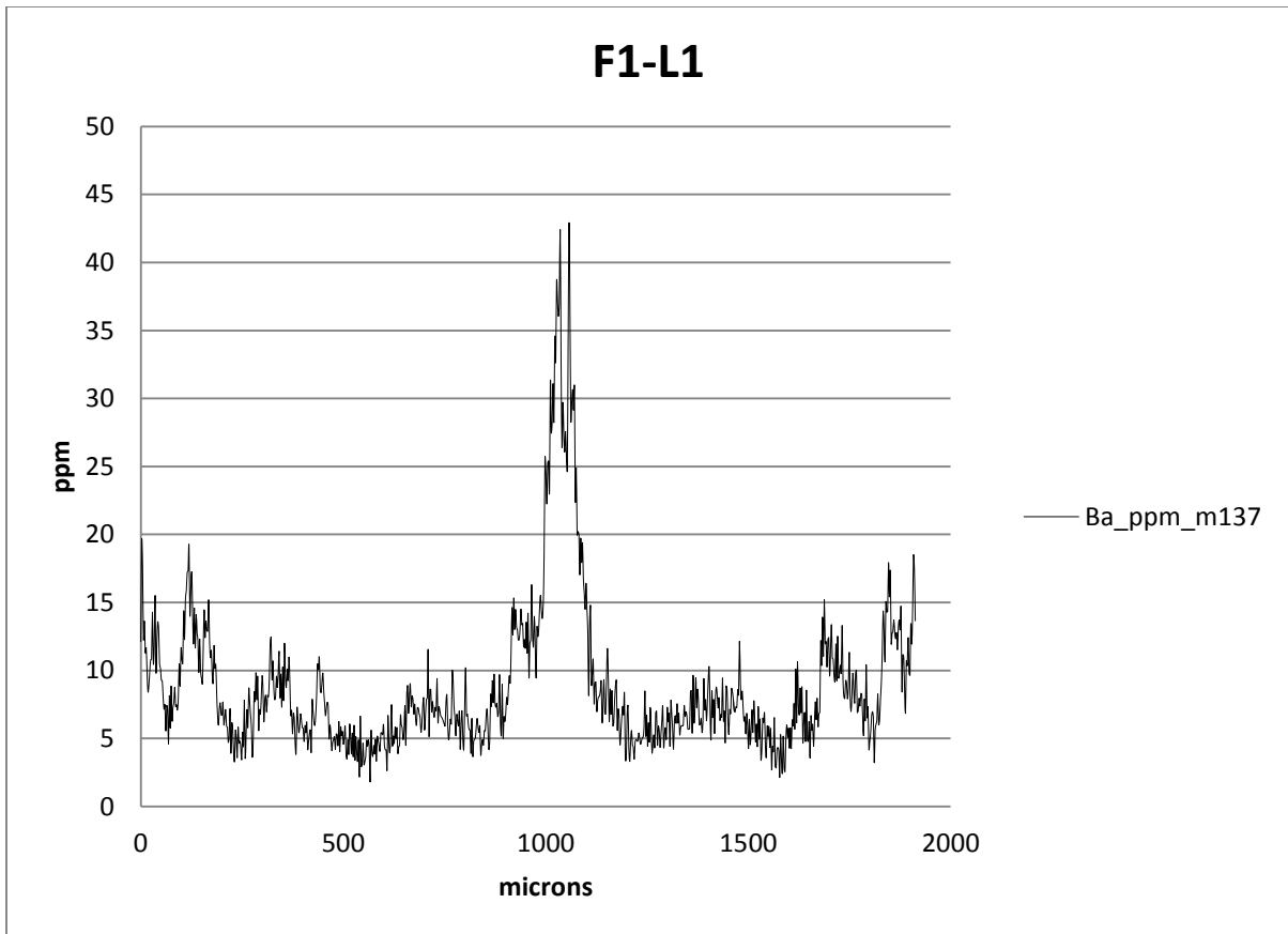
Figure 15 Barium profile of the F1-L1 grayling individual
