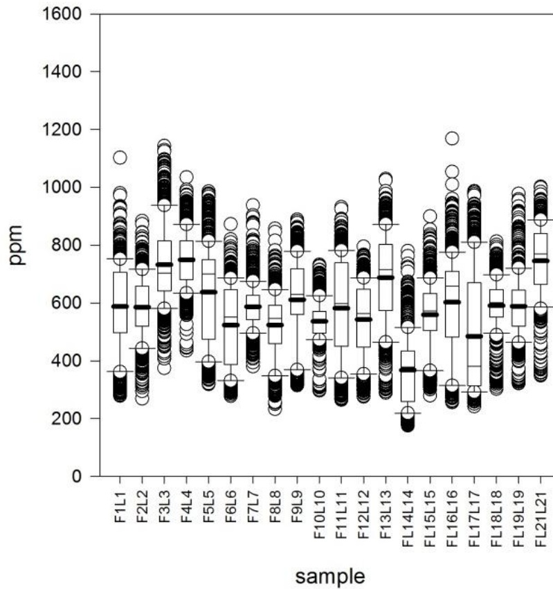
Figure 31 Plots showing Sr data for the grayling from Christal Creek. Individual sample plots show data range, the boxes 25 th and 75 th percentile of the data, whiskers 10 th and 90 th percentile, and median (thin line) and mean (thick line).
