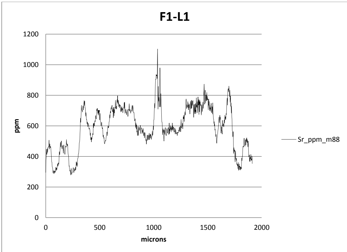
Figure 13 Strontium profile of the F1-L1 grayling individual
