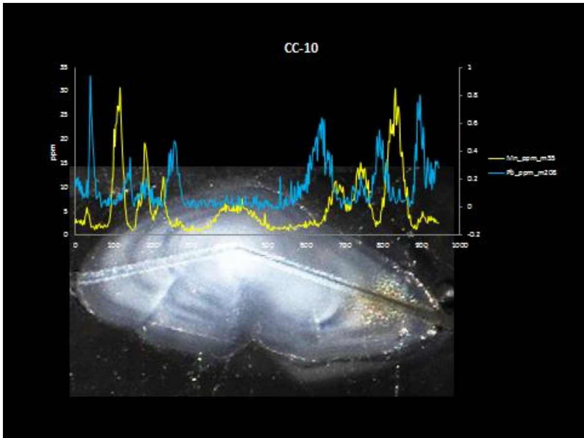
Figure 26 LA-ICP-MS linescan data for Mn (yellow), and Pb (blue) overlaid on a reflected light optical image of a 3 year old sculpin otolith from Christal Creek. The higher Pb concentrations correspond to narrow dark winter bands and the elevated Mn concentrations correlate with summer growth (note: metal values are expressed in ppm).
