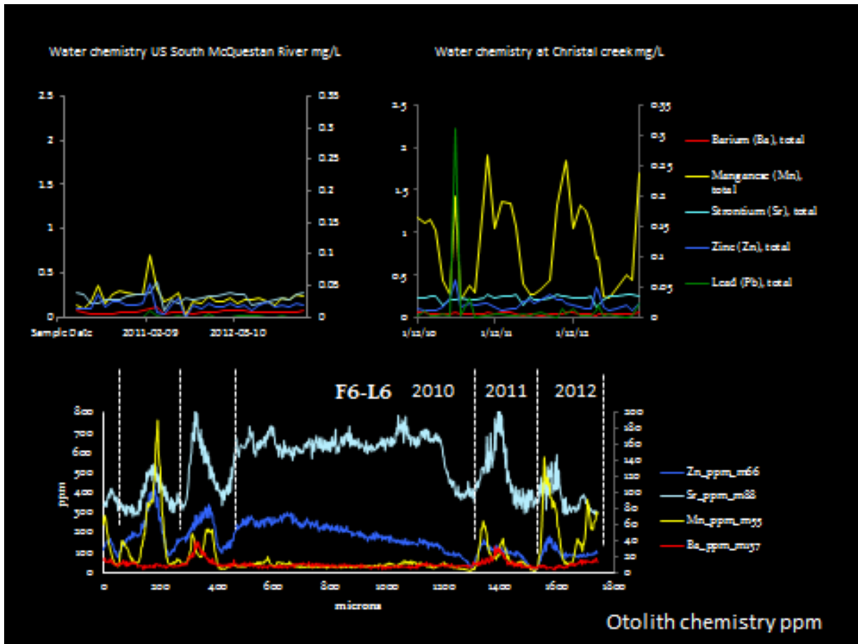
Figure 28 Line scan data for Zn, Sr, Mn and Ba in ppm from Figure 20 corresponding to the time period 2010 to 2013. Also shown are two graphs with the water quality data in mg/L from South McQuesten River and Christal Creek for the same period. A shared feature of the two data sets from the Christal Creek otolith and water quality data are the prominent double Mn peaks in 2011 and 2012.
