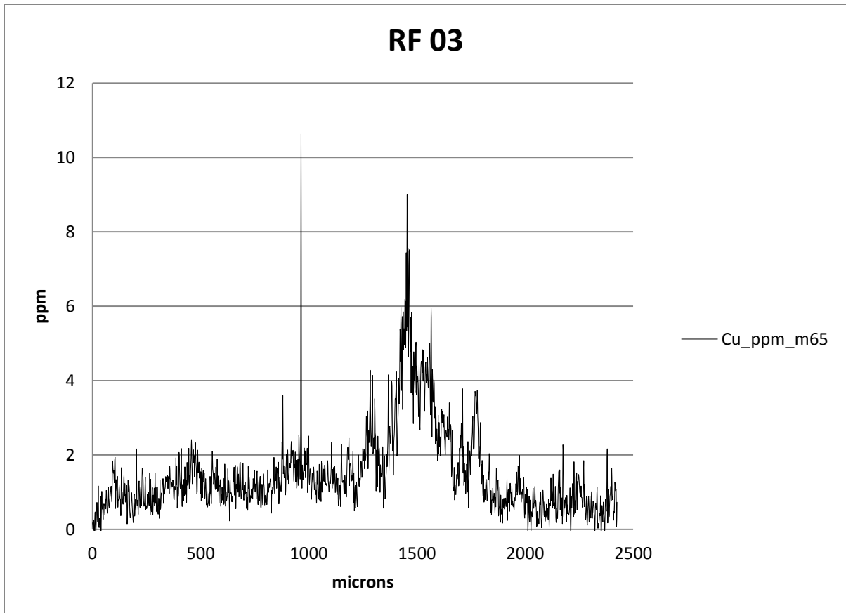
Figure 19 Copper profile of the F1-L1 grayling individual
