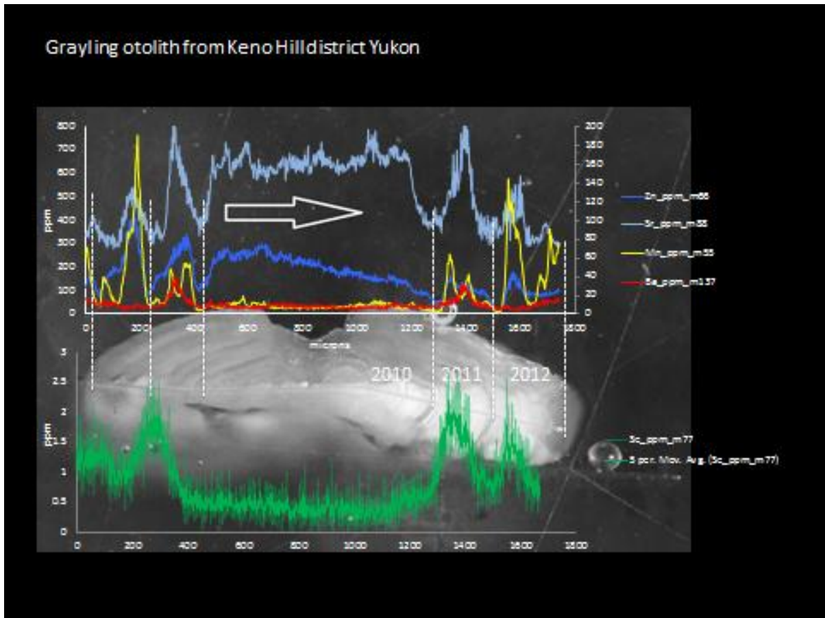
Figure 20 LA-ICP-MS linescan data for Zn (dark blue), Sr (light blue), Mn (yellow), Ba (red), and Se (green) overlaid on a reflected light optical image of a grayling otolith. The annular structure, narrow dark bands indicating slow winter growth and lighter thicker bands indicating faster summer growth, indicate the fish went through its larval stage in 2010 and was caught in 2013 (note: metal values are expressed in ppm)
