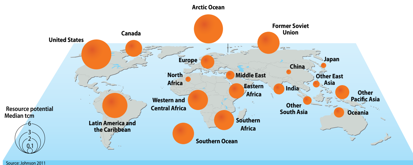
Figure 2.4-a: Gas hydrates resource potential by global regions. This figure includes only that subset of global in-place gas hydrates that appear to occur at high concentrations in sand-rich reservoirs, the most likely candidates for development. Source: Johnson 2011.
