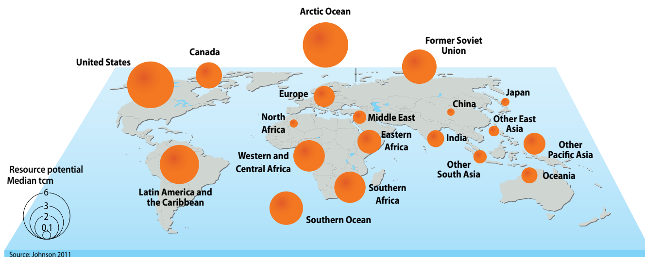
Figure 1.1: Gas hydrates resource potential by global regions. This figure includes only that subset of global in-place gas hydrates that appear to occur at high concentrations in sand-rich reservoirs, the most likely candidates for development. Source: Johnson 2011.
