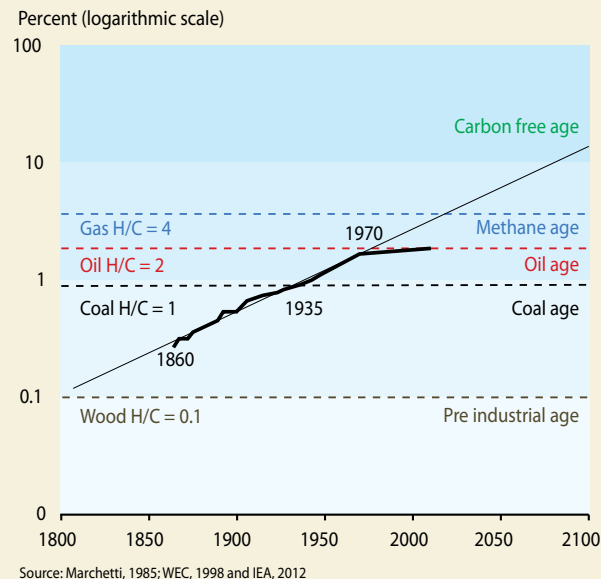
Figure 1.4: Hydrogen to carbon ratio of global primary energy, 1860-2009. The ratio is expressed in fractional shares of hydrogen and carbon in average primary energy consumed. Source: Marchetti (1985), WEC (1998), IEA (2012).
