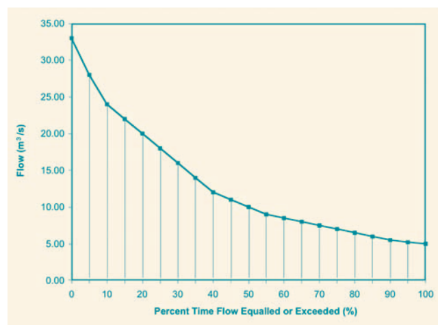
Figure 6b. Flow duration curve for river with more steady flow
