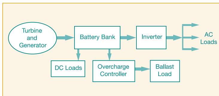
Figure 24. Balance of system for a battery-based system
