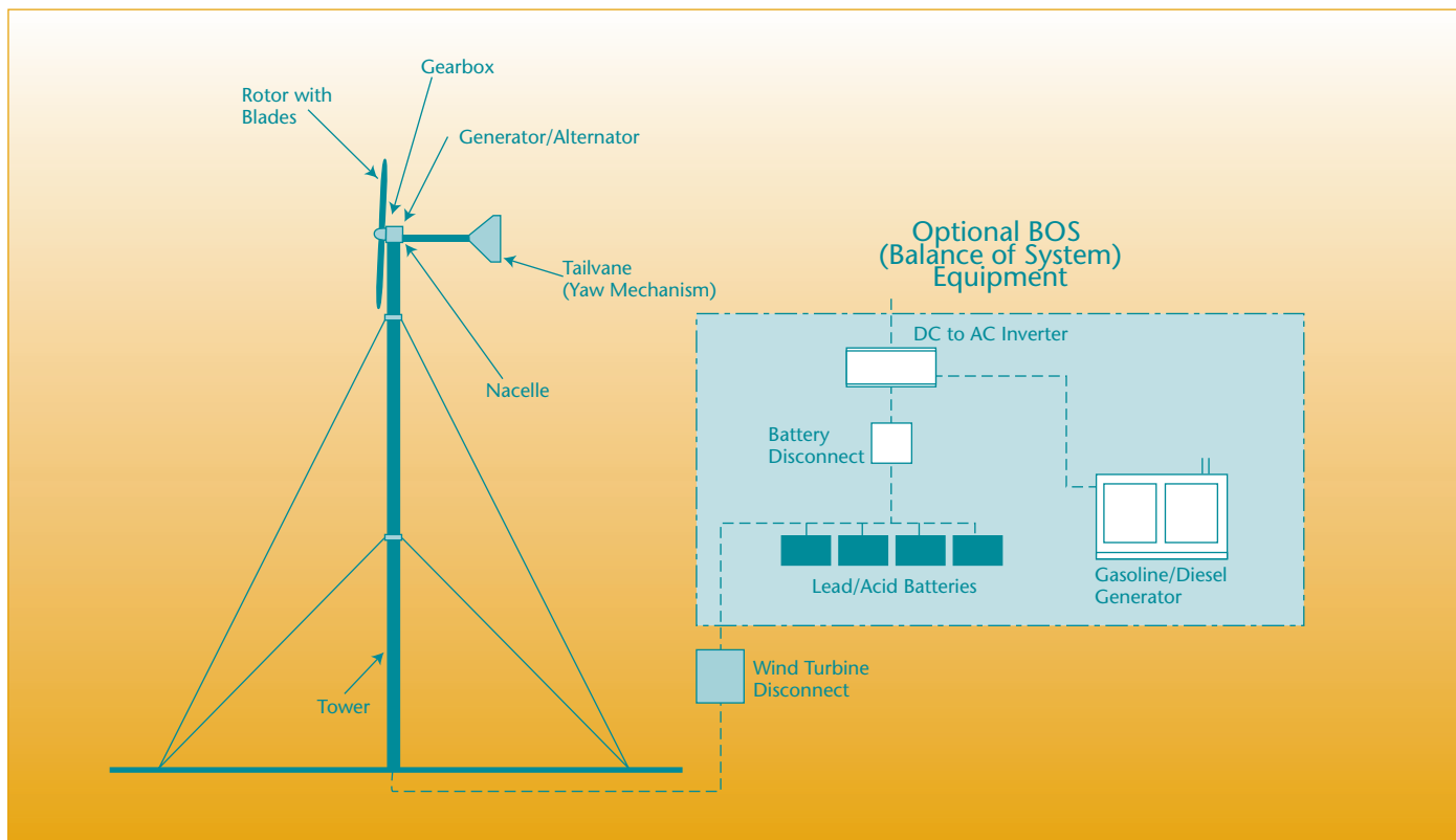
▲ Figure 6. Wind energy system components.
