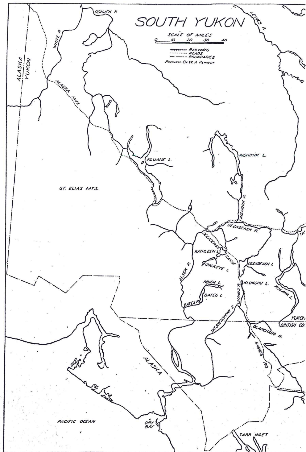
FIGURE 2. Southern Yukon.
