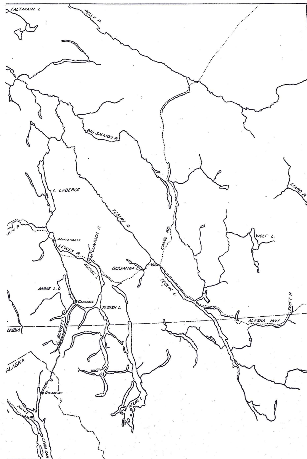
FIGURE 2. Southern Yukon
