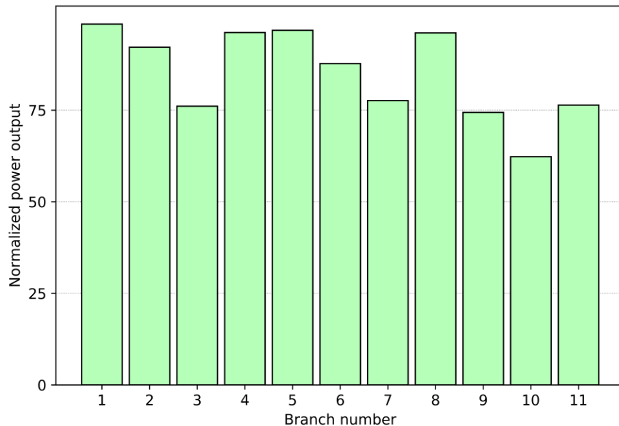
Figure 7 : Average normalized branch power output during two summer months
