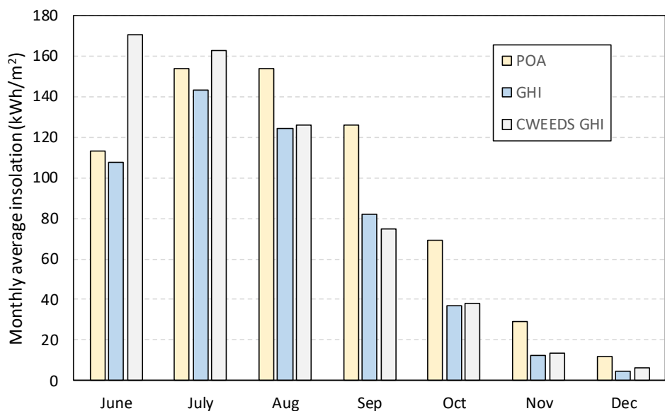
Figure 4 : Comparison between measured Apogee SP 510 insolation and monthly CWEEDS averages
