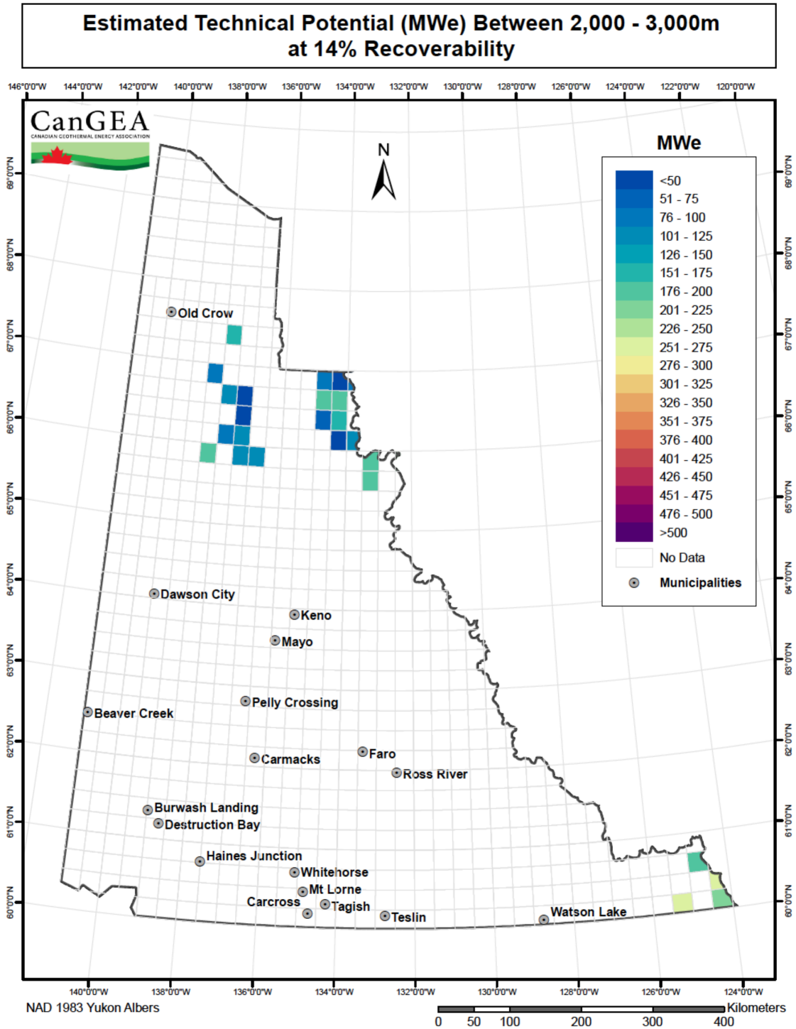
Figure 34: Technical potential between 2,000m and 3,000m at 14% recoverability
