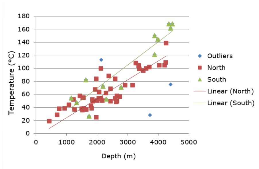
Figure 19: Temperature vs. depth profile of selected boreholes.
