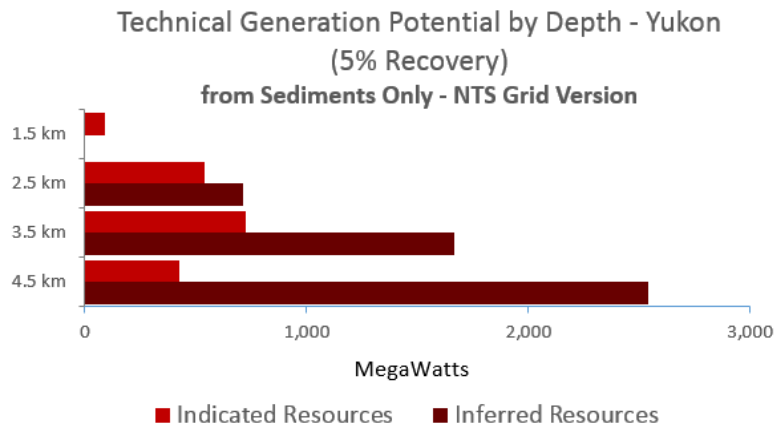
Figure 27: Indicated vs. inferred resources (5% recovery)
