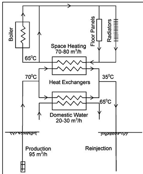
Figure 15: Example of a Melun I-Almont (Paris) doublet heating system
