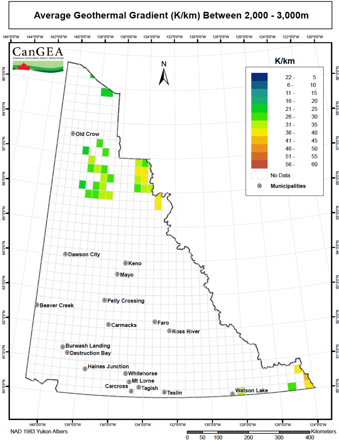
Figure 52: Average geothermal gradient – 2,000m – 3,000m
