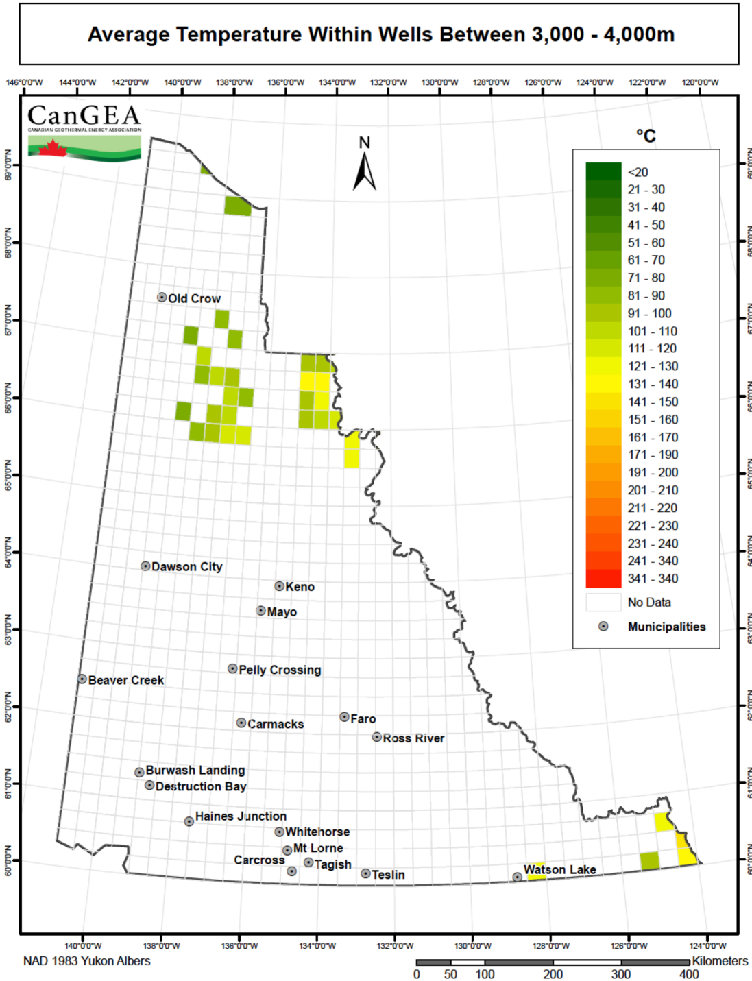
Figure 25: Average temperature within wells – 3,000m – 4,000m
