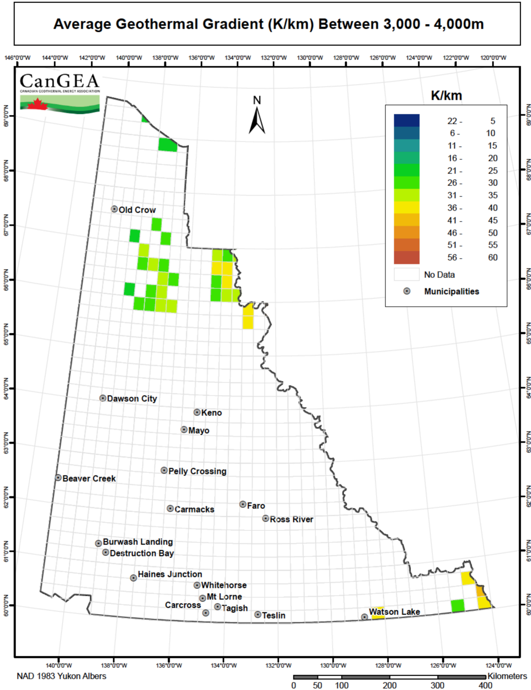
Figure 53: Average geothermal gradient – 3,000m – 4,000m
