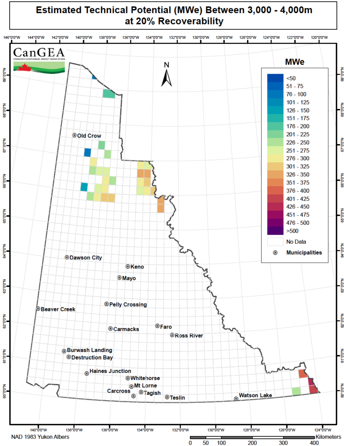
Figure 39: Technical potential between 3,000m and 4,000m at 20% recoverability
