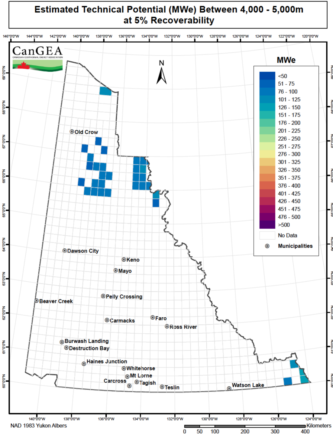
Figure 32: Technical potential between 4,000m and 5,000m at 5% recoverability
