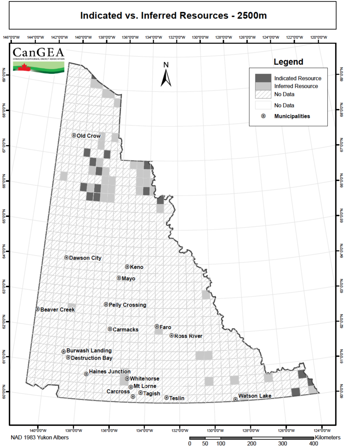
Figure 48: Map of indicated vs. inferred resources – 2,500m
