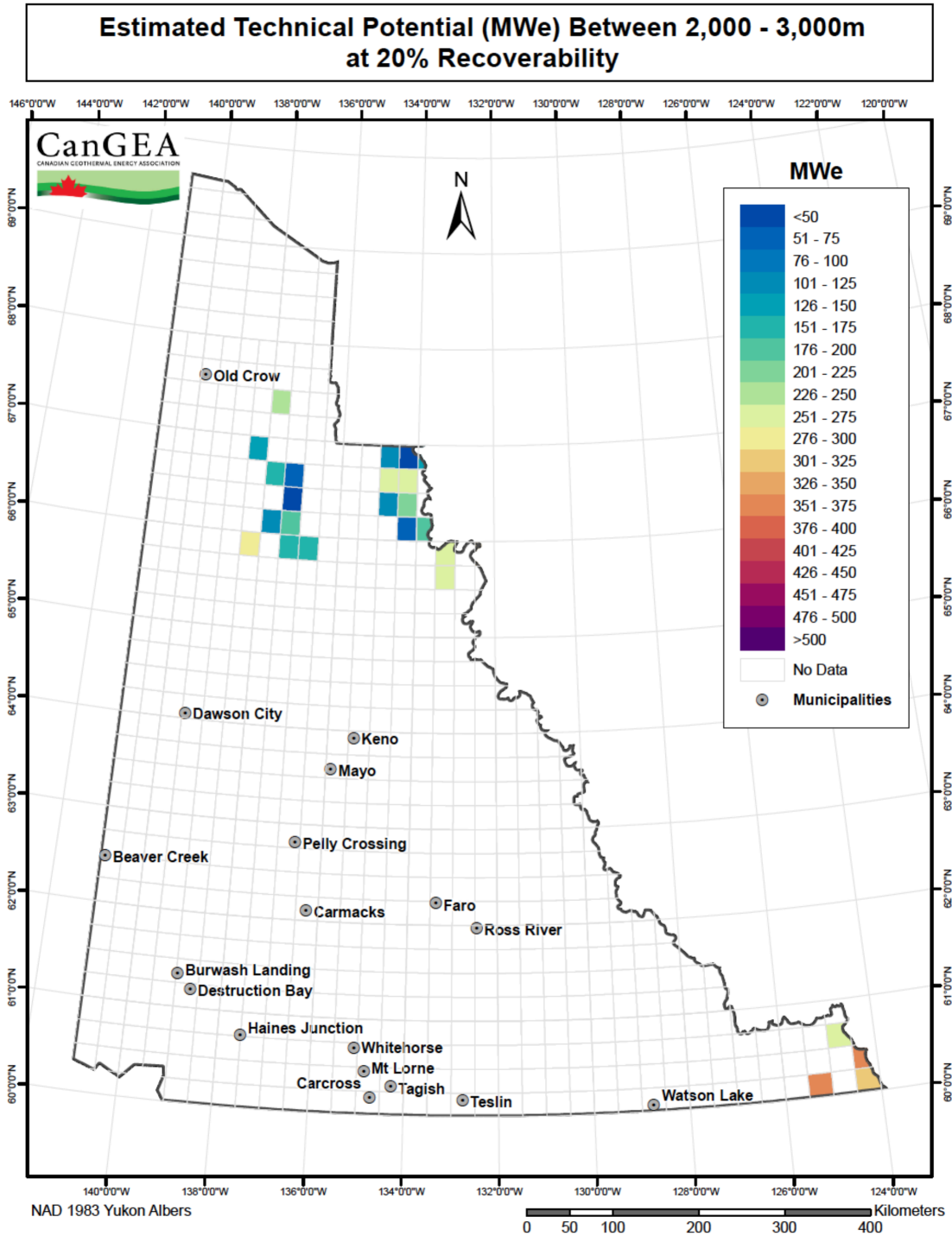
Figure 38: Technical potential between 2,000m and 3,000m at 20% recoverability
