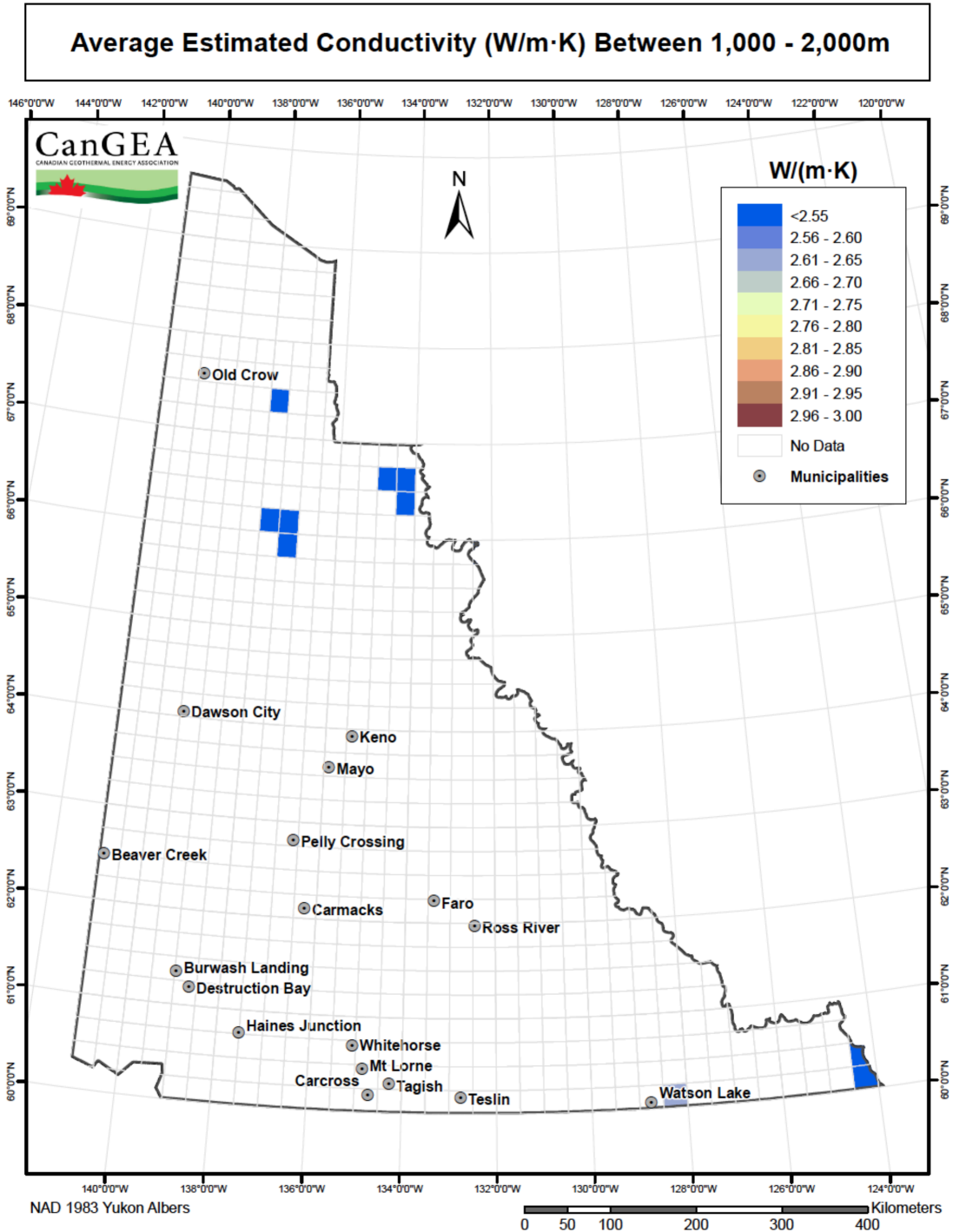
Figure 56: Average estimated conductivity – 1,000m – 2,000m
