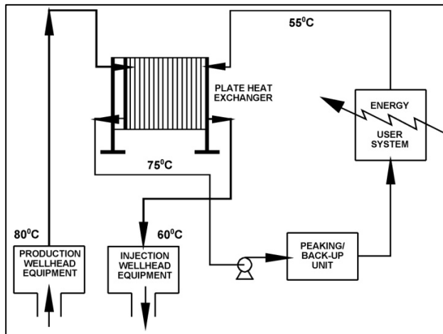
Figure 12: Geothermal direct-utilization system using a heat exchanger
