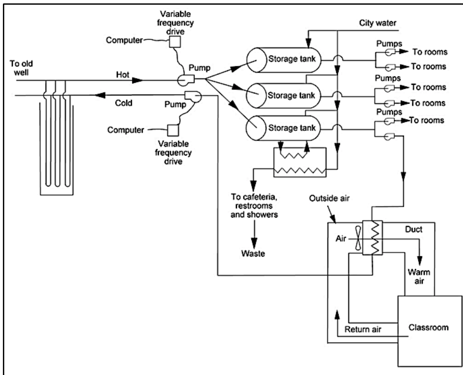
Figure 11: Down hole heat exchanger system at Ponderosa Middle School, Klamath Falls, Oregon
