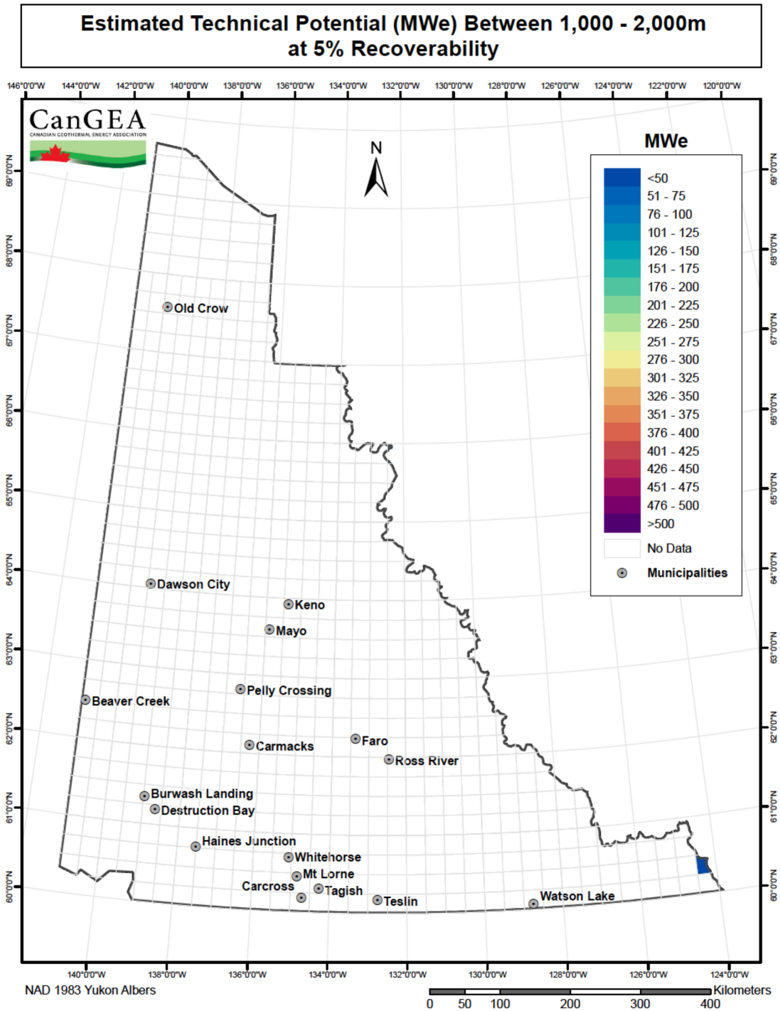
Figure 29: Technical potential between 1,000m and 2,000m at 5% recoverability
