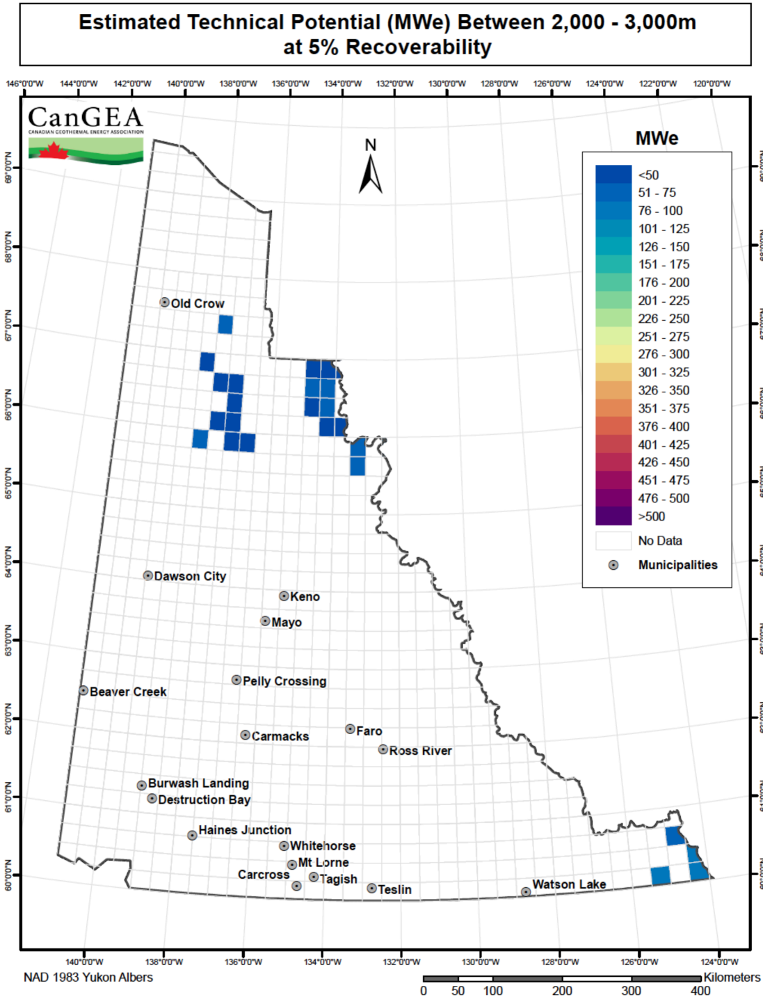
Figure 30: Technical potential between 2,000m and 3,000m at 5% recoverability
