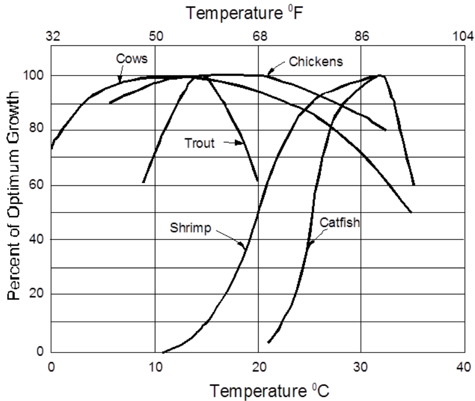
Figure 6: Growth rate of aquatic species compared to land animals
