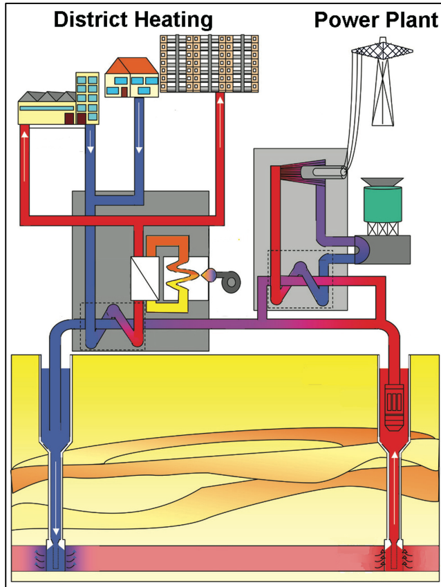
Figure 2: Schematic of combined geothermal heat and power utilization at Neustadt Glewe, Germany
