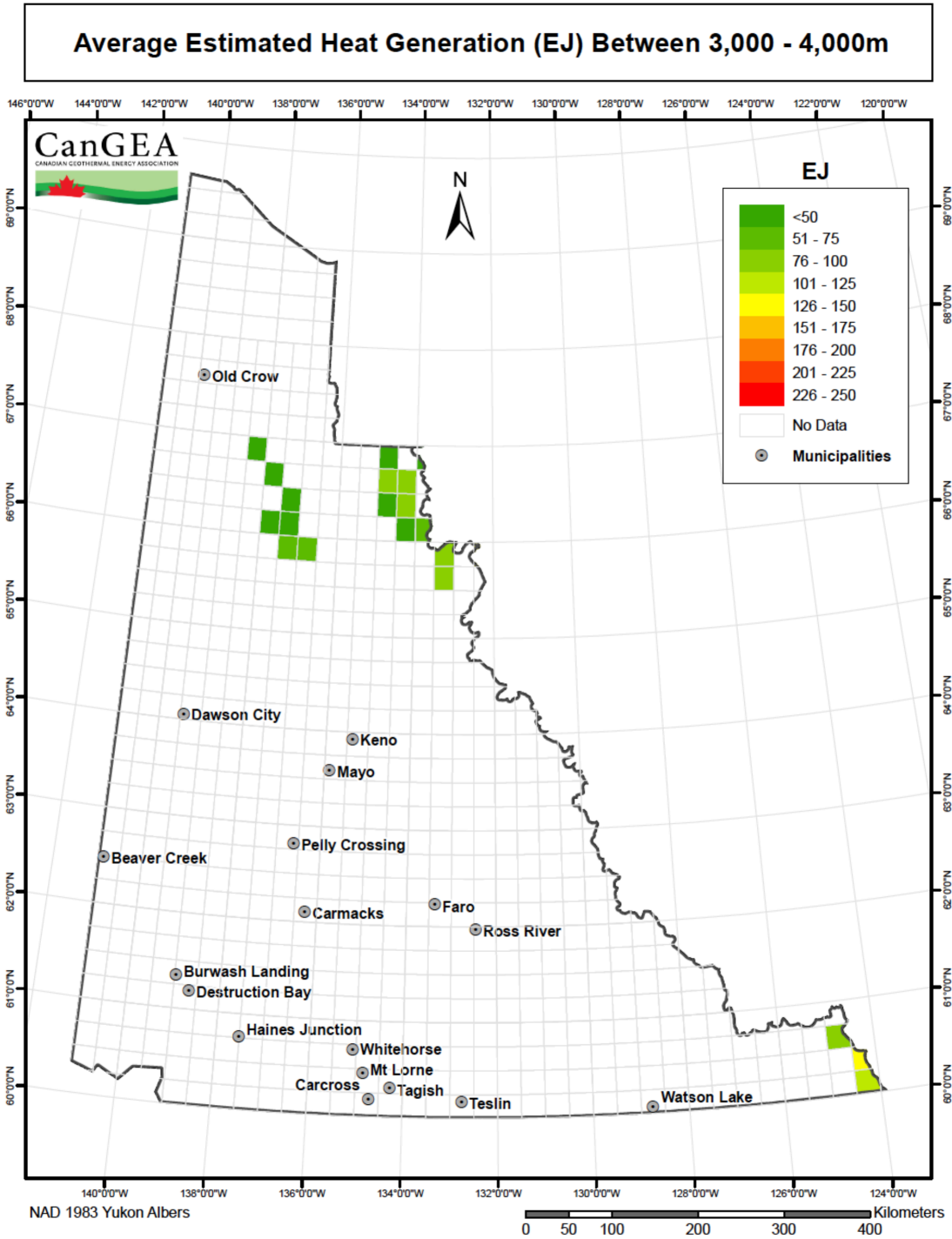
Figure 62: Average estimated heat generation – 3,000m – 4,000m
