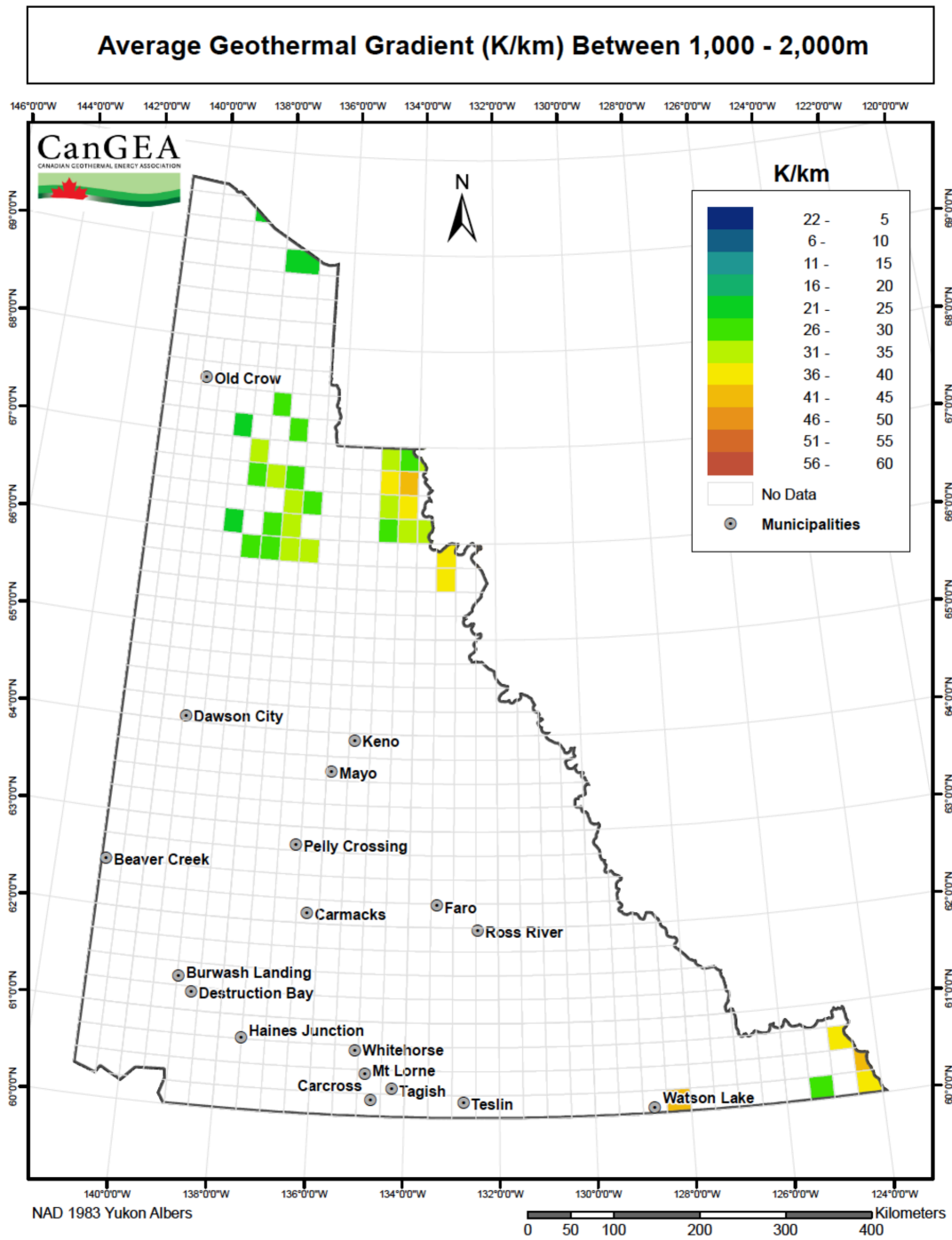
Figure 51: Average geothermal gradient – 1,000m – 2,000m
