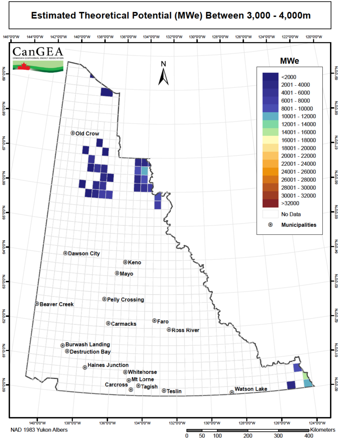
Figure 45: Theoretical potential between 3,000m and 4,000m
