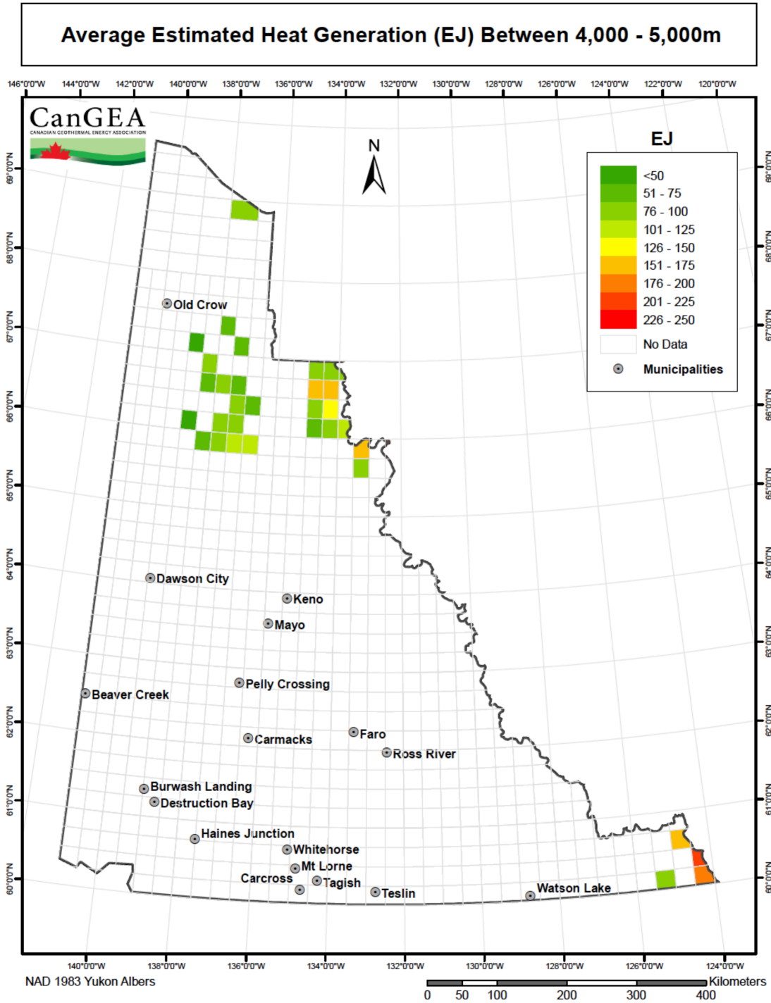
Figure 63: Average estimated heat generation – 4,000m – 5,000m
