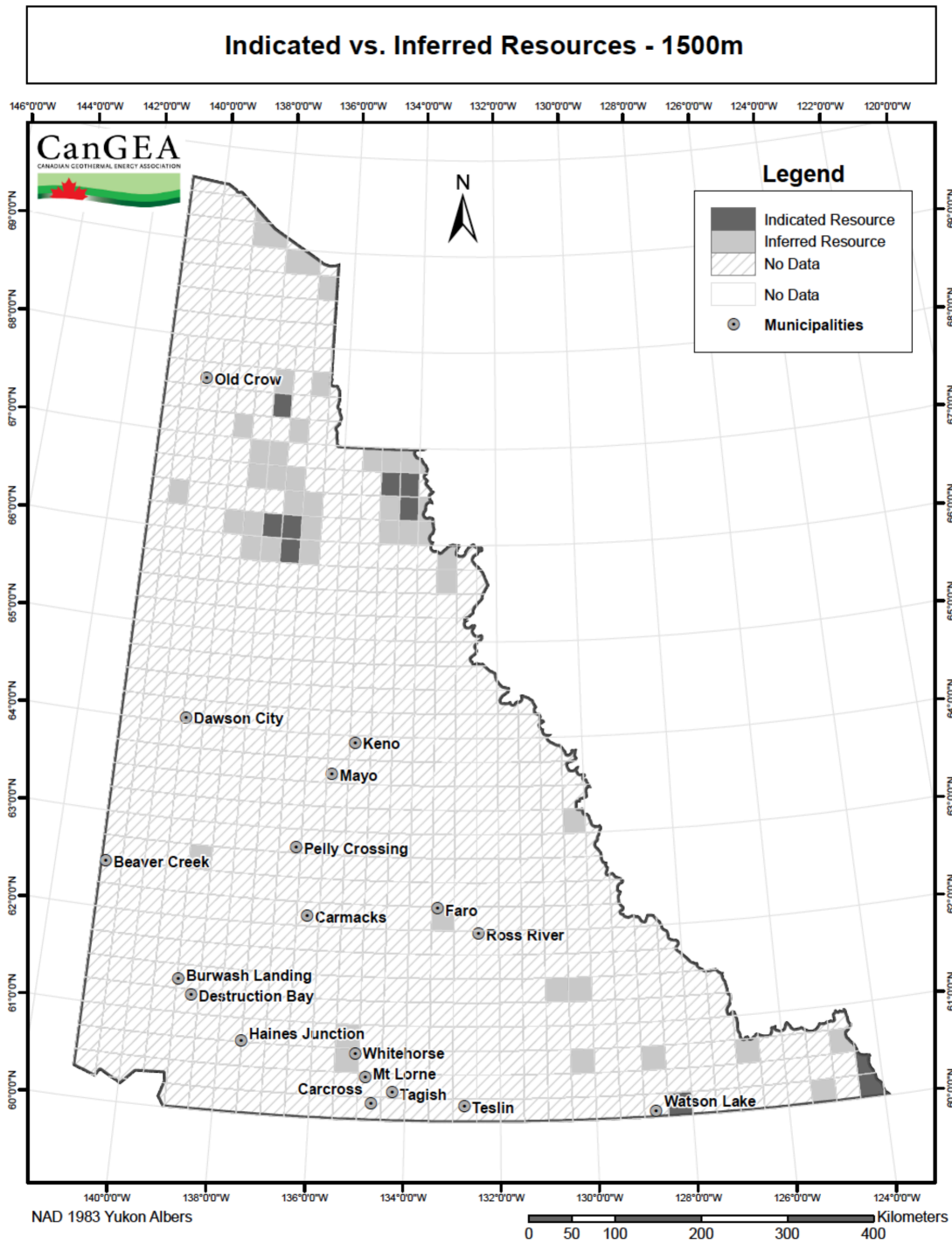
Figure 47: Map of indicated vs. inferred resources – 1,500m
