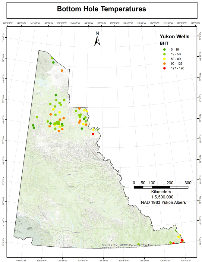
Figure 17: Bottom hole temperatures, Yukon
