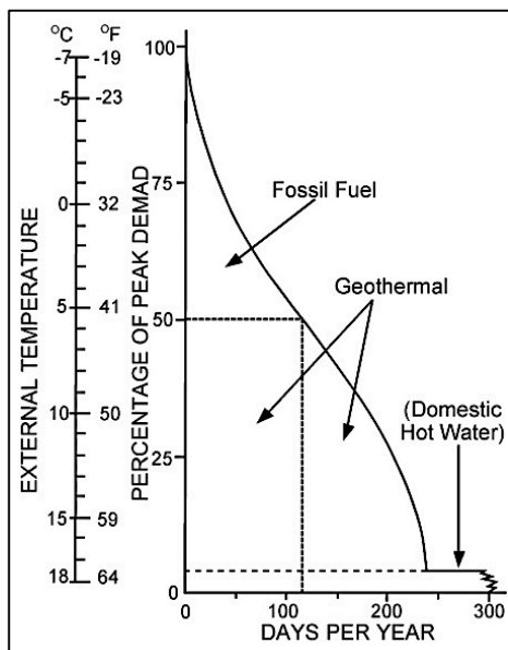
Figure 13: Meeting peak demand with fossil fuel
