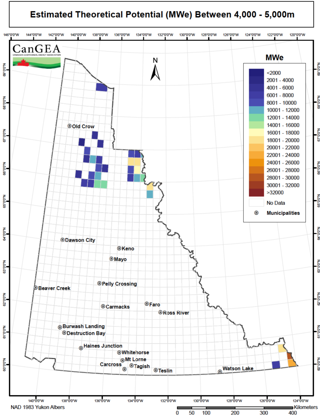
Figure 46: Theoretical potential between 4,000m and 5,000m
