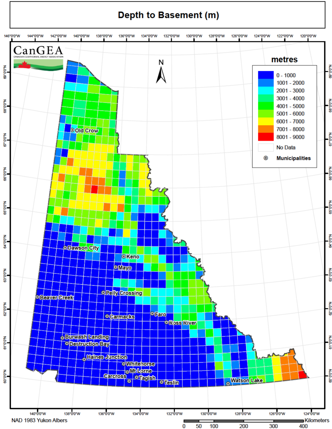
Figure 55: Depth to basement
