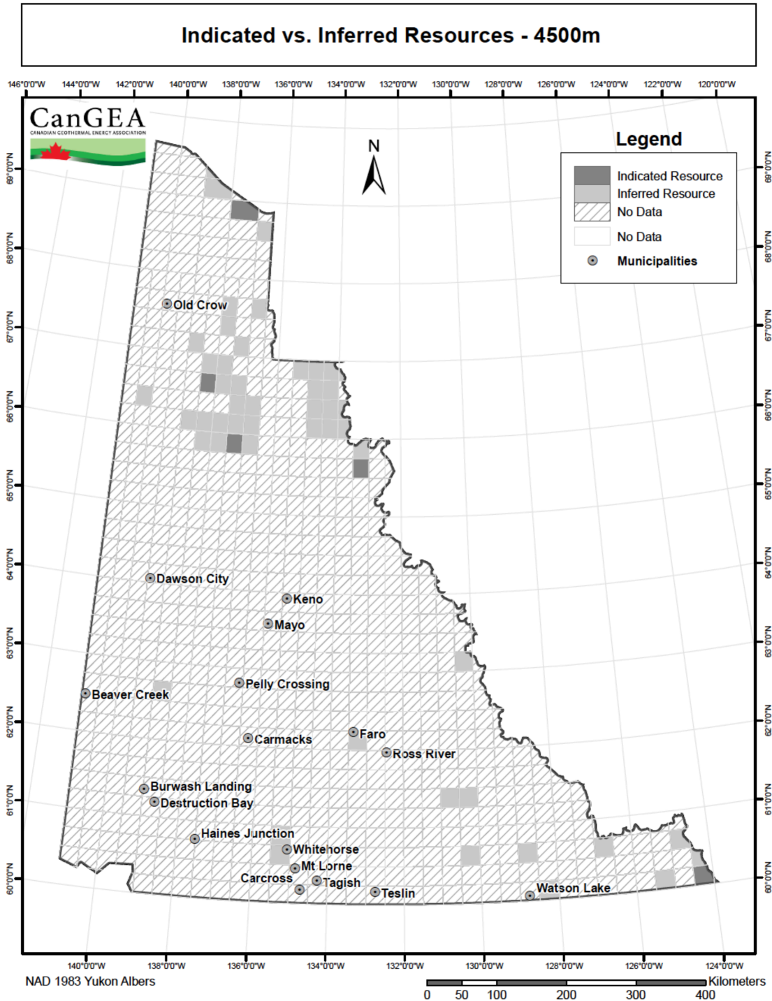
Figure 50: Map of indicated vs. inferred resources – 4,500m
