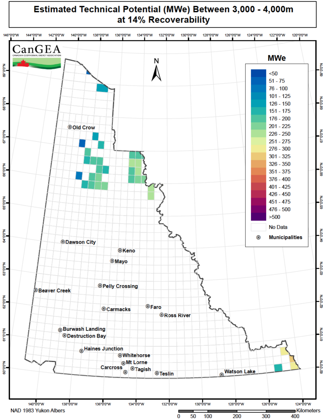
Figure 35: Technical potential between 3,000m and 4,000m at 14% recoverability
