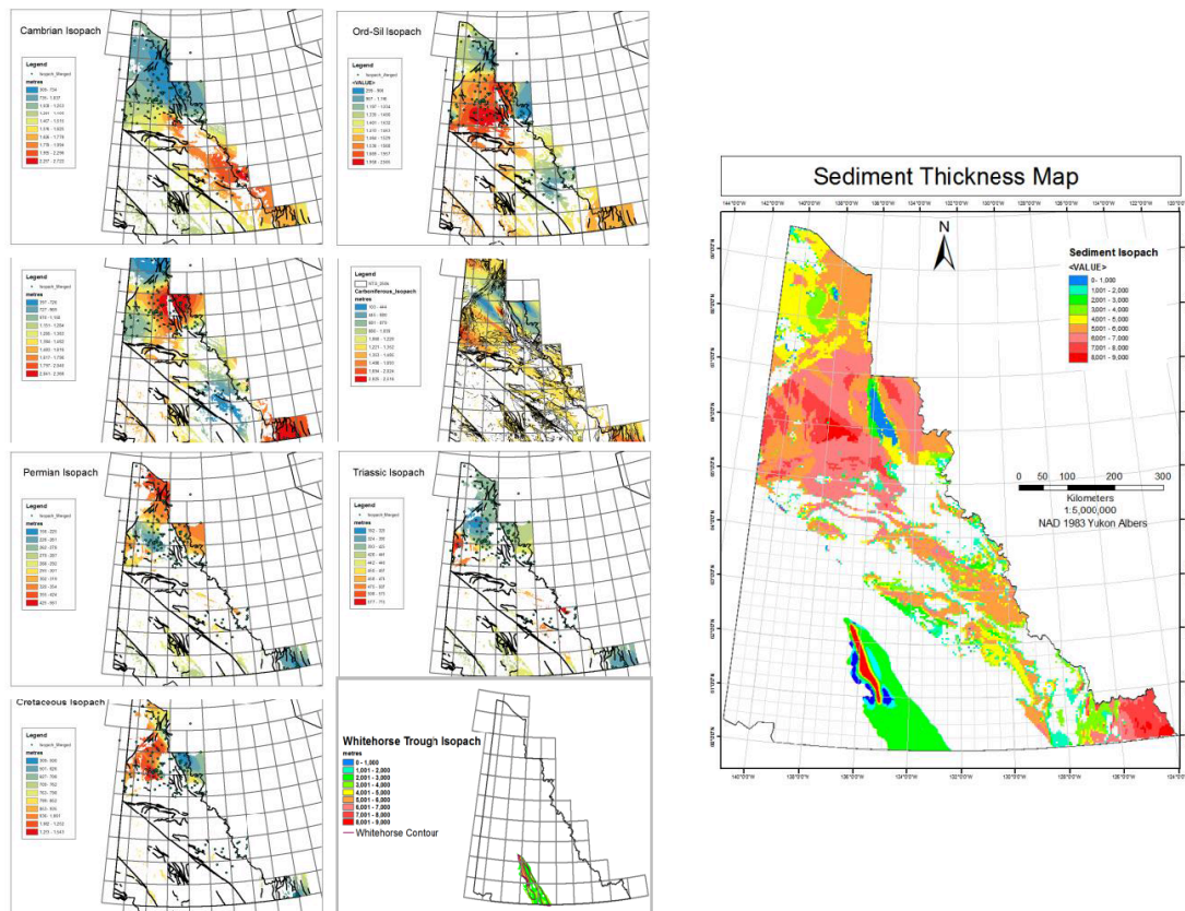
Figure 18: Series of images illustrating how datasets were used in combination to estimate the thickness of the sedimentary cover
