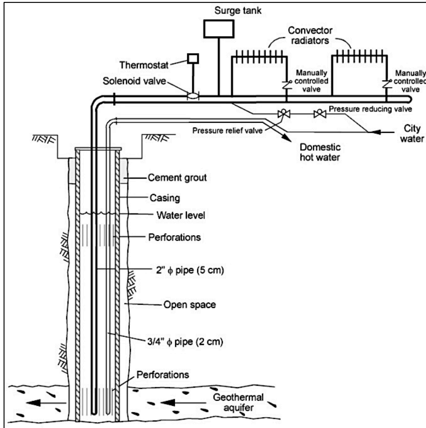
Figure 10: An example of a residential down hole heat exchanger installation
