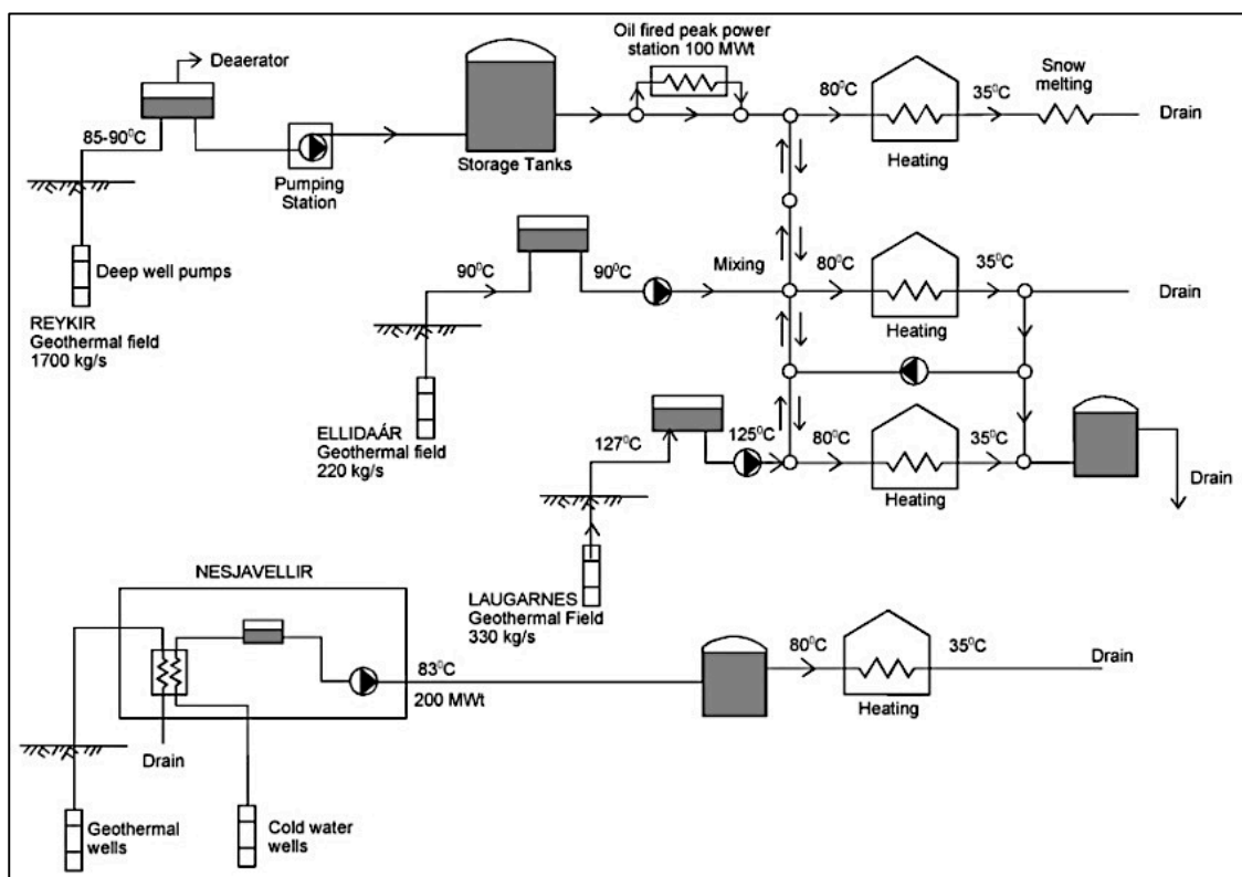
Figure 14: Reykjavik, Iceland district heating system
