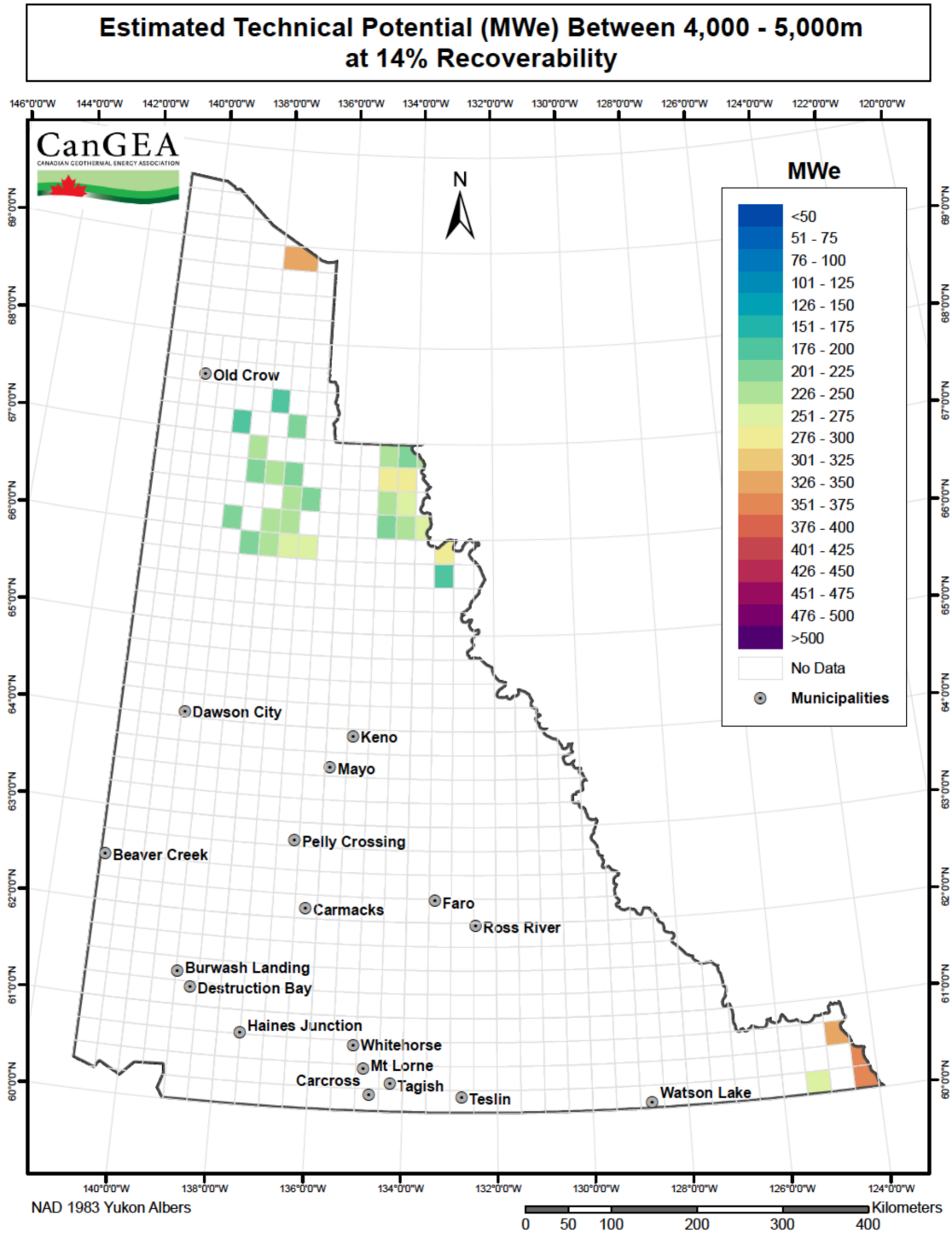
Figure 36: Technical potential between 4,000m and 5,000m at 14% recoverability
