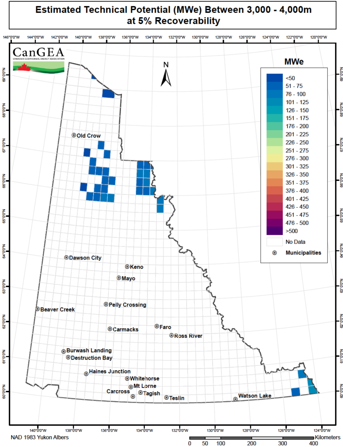
Figure 31: Technical potential between 3,000m and 4,000m at 5% recoverability
