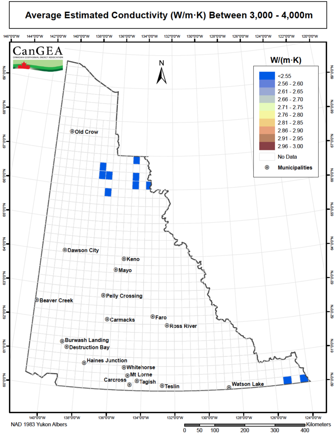
Figure 58: Average estimated conductivity – 3,000m – 4,000m
