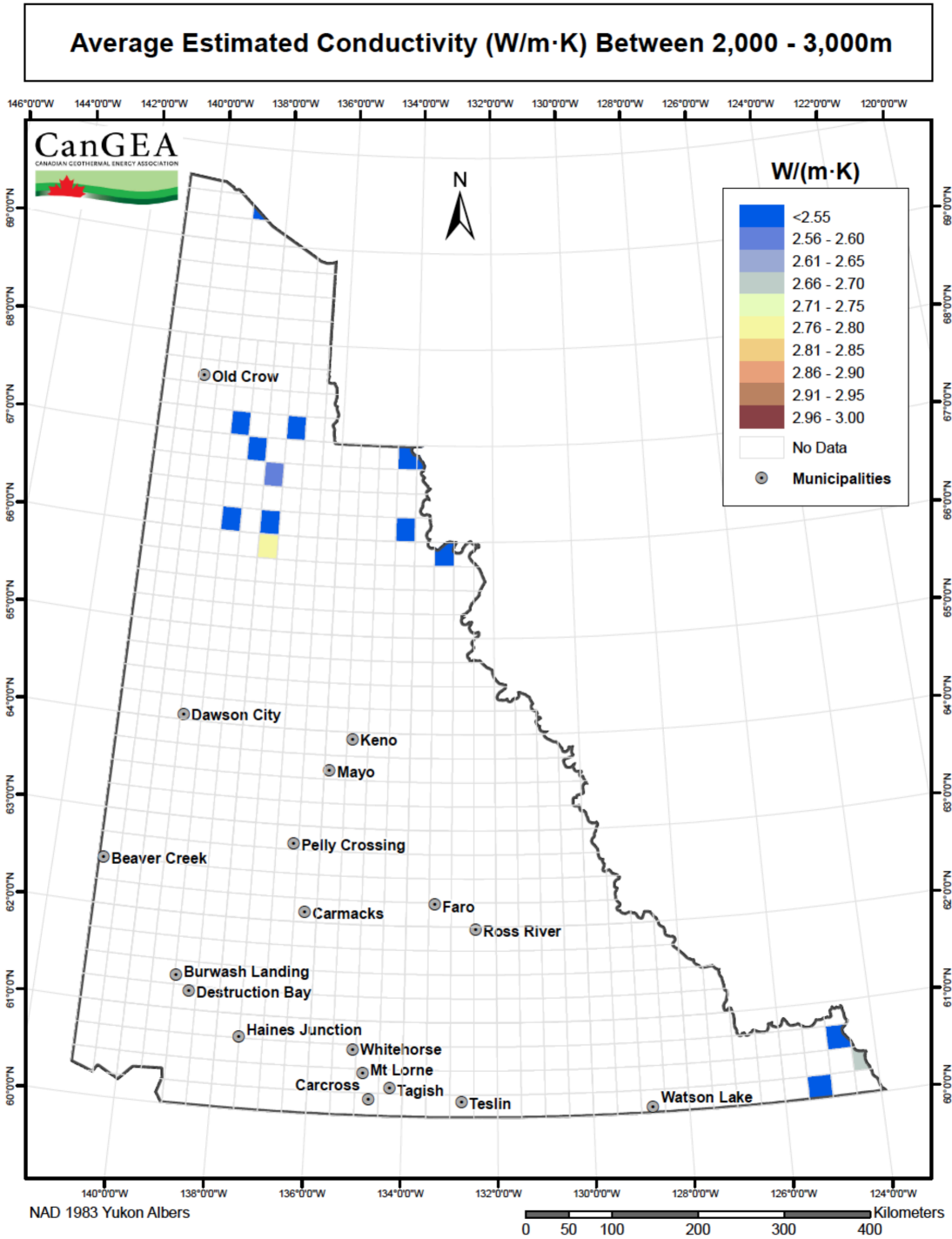
Figure 57: Average estimated conductivity – 2,000m – 3,000m
