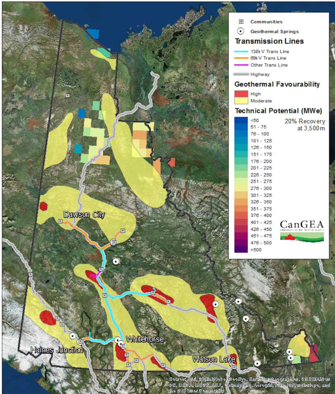
Figure 20: Primary geothermal exploration areas
