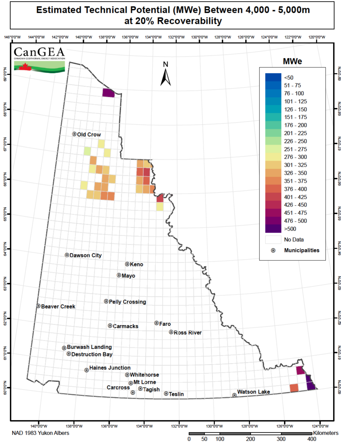
Figure 40: Technical potential between 4,000m and 5,000m at 20% recoverability
