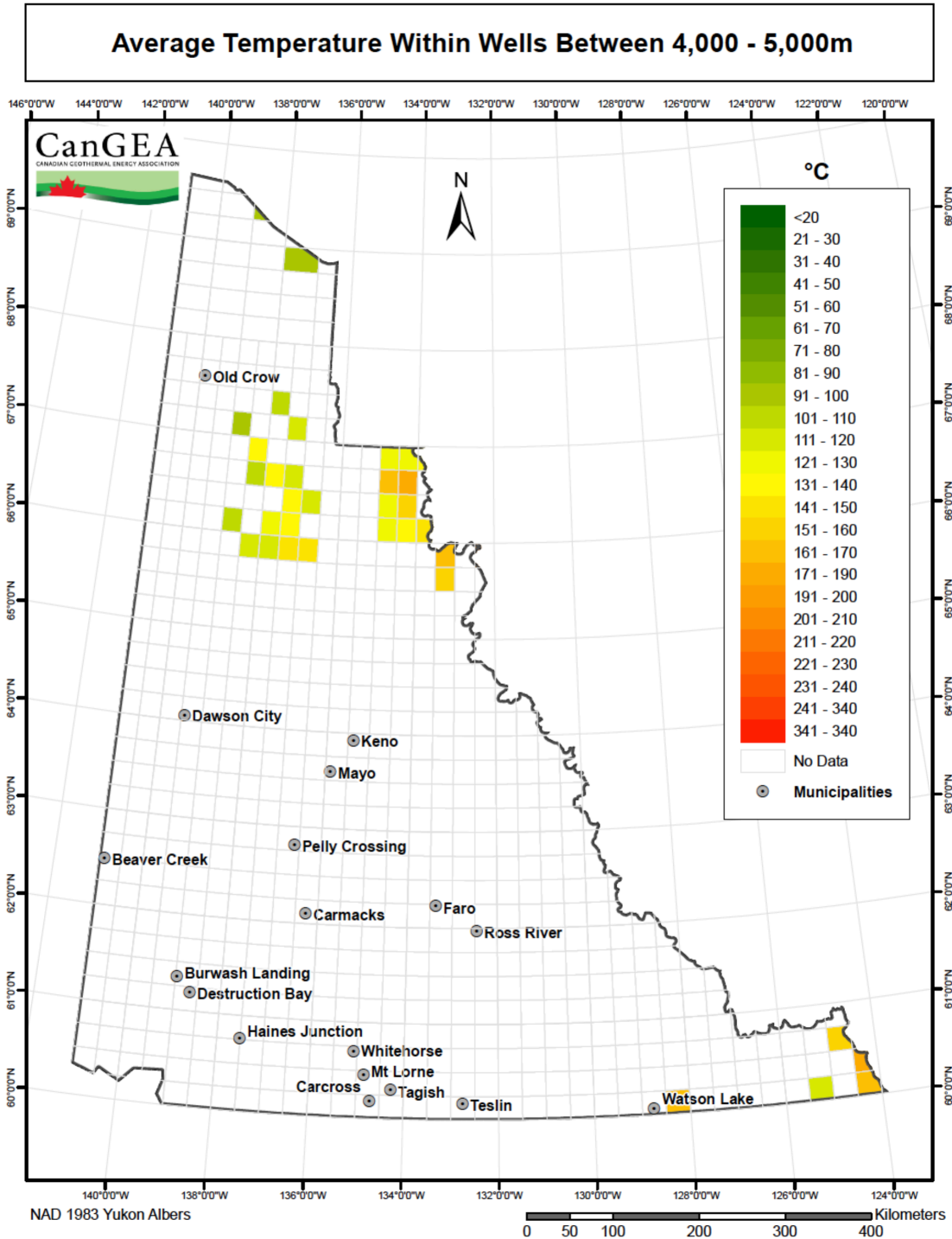
Figure 26: Average temperature within wells – 4,000m – 5,000m
