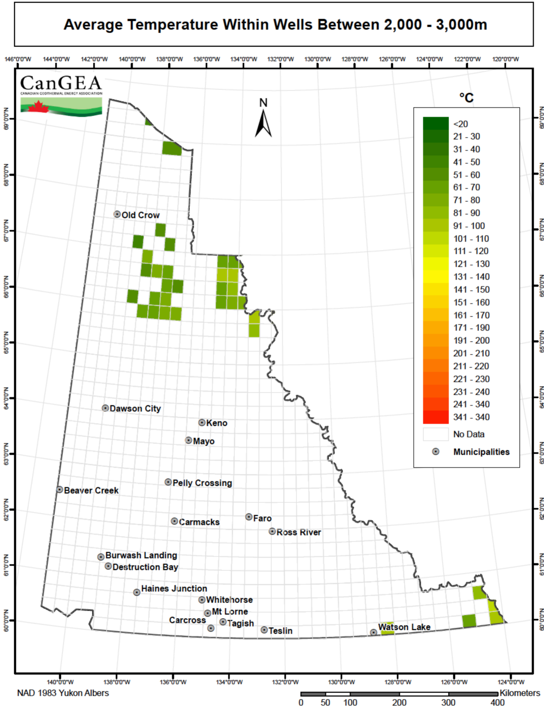
Figure 24: Average temperature within wells – 2,000m – 3,000m
