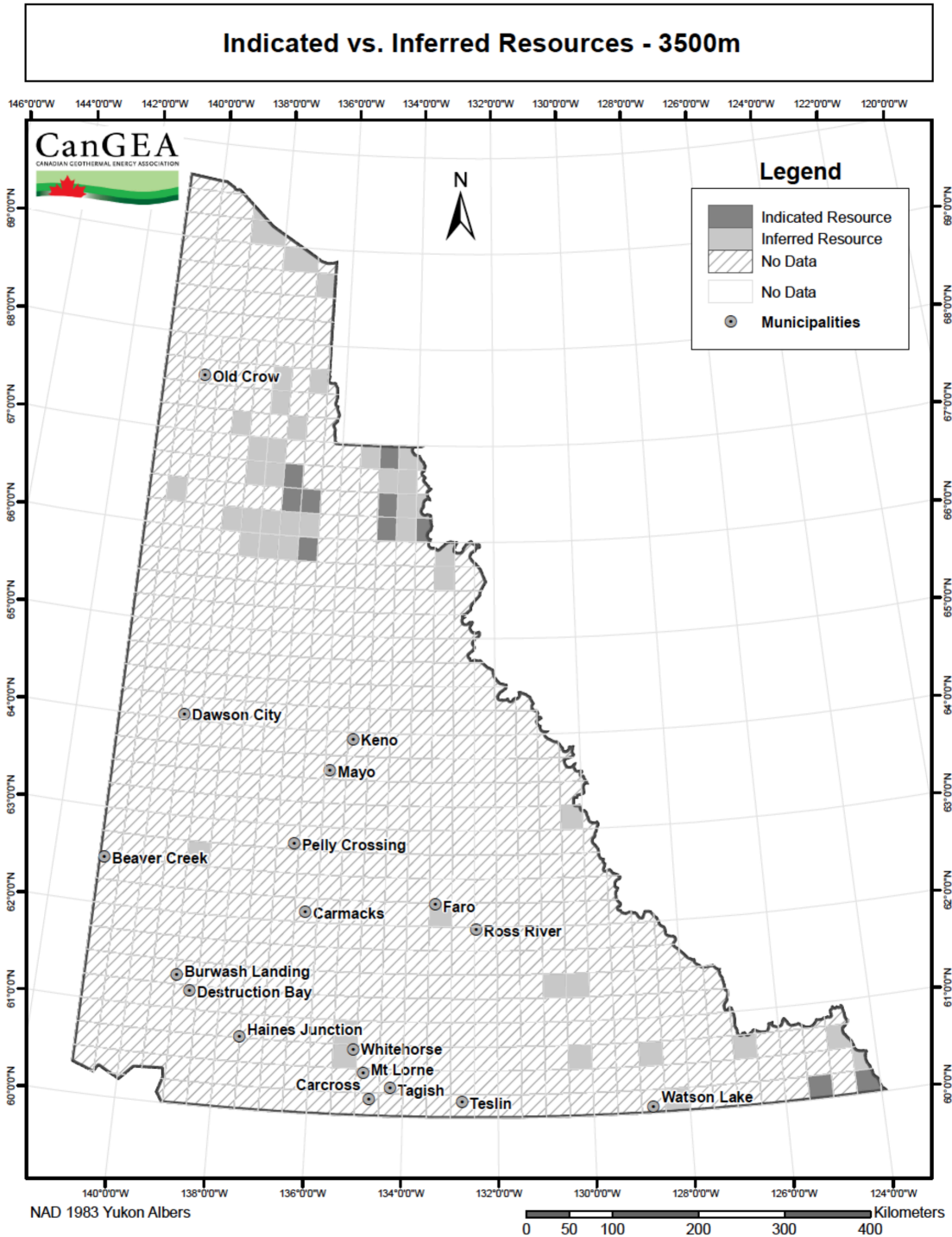
Figure 49: Map of indicated vs. inferred resources – 3,500m
