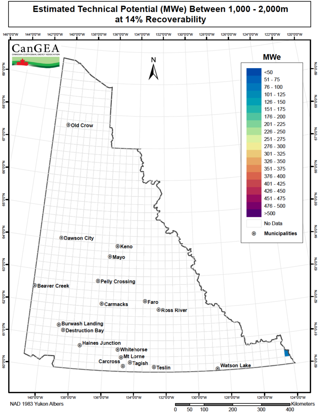
Figure 33: Technical potential between 1,000m and 2,000m at 14% recoverability
