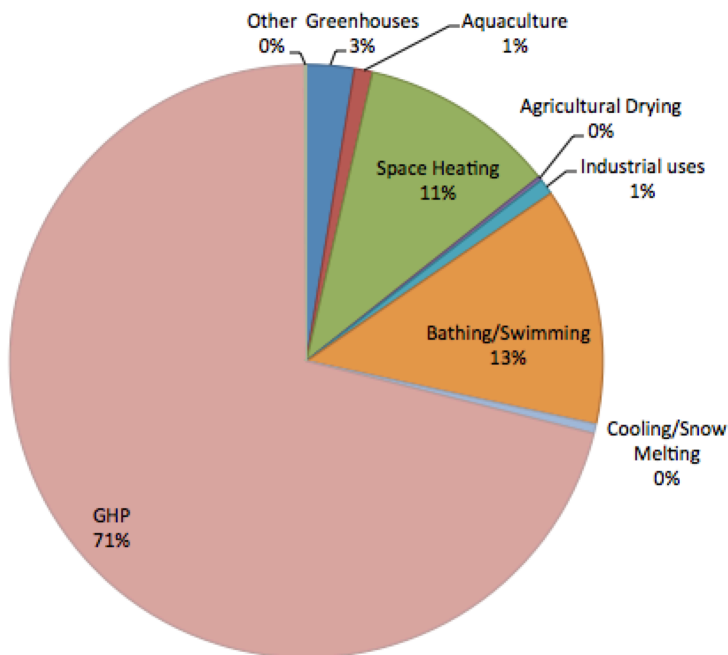
Figure 3: Geothermal direct use applications worldwide in 2010, distributed by percentage of total installed capacity (MWt) 41
