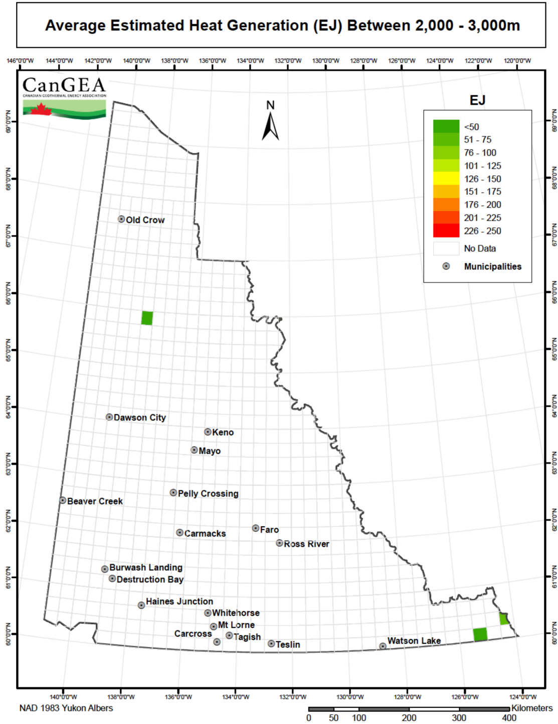
Figure 61: Average estimated heat generation – 2,000m – 3,000m
