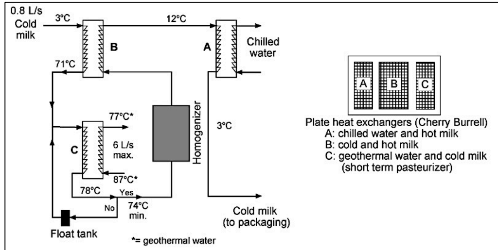
Figure 8: Klamath Falls milk pasteurization flow diagram
