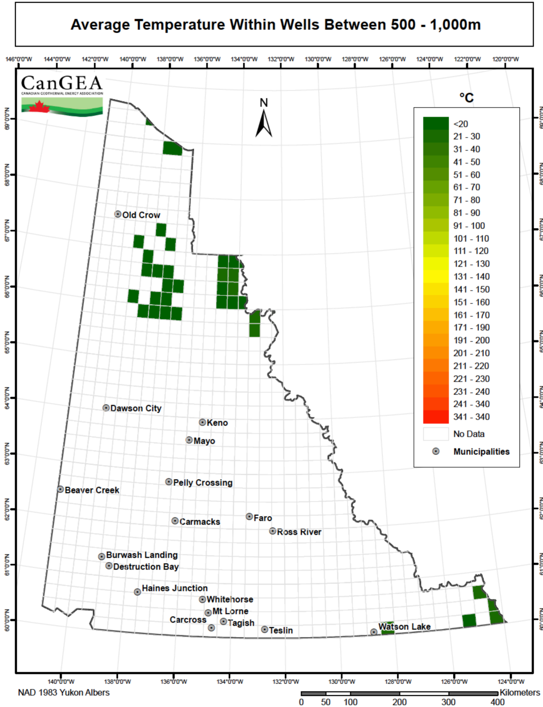
Figure 22: Average temperature within wells – 500m – 1,000m
