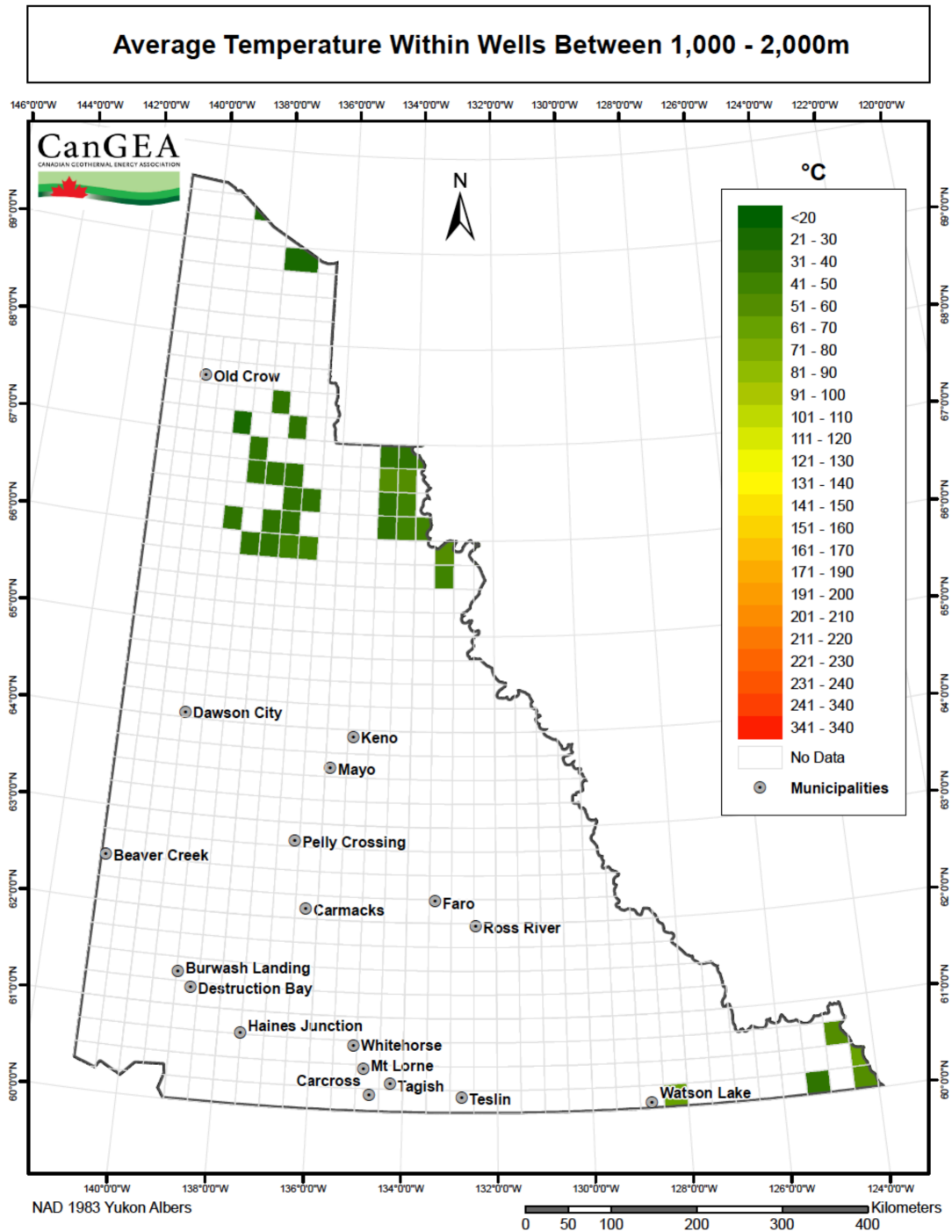
Figure 23: Average temperature within wells – 1,000m – 2,000m
