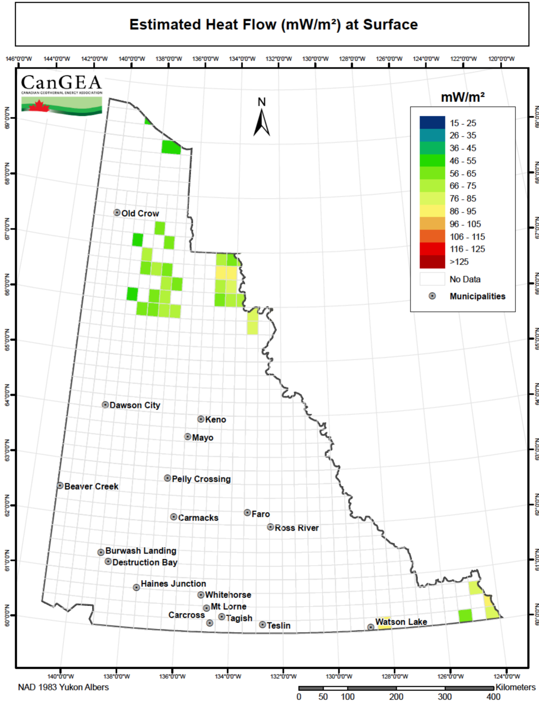
Figure 64: Estimated heat flow at surface
