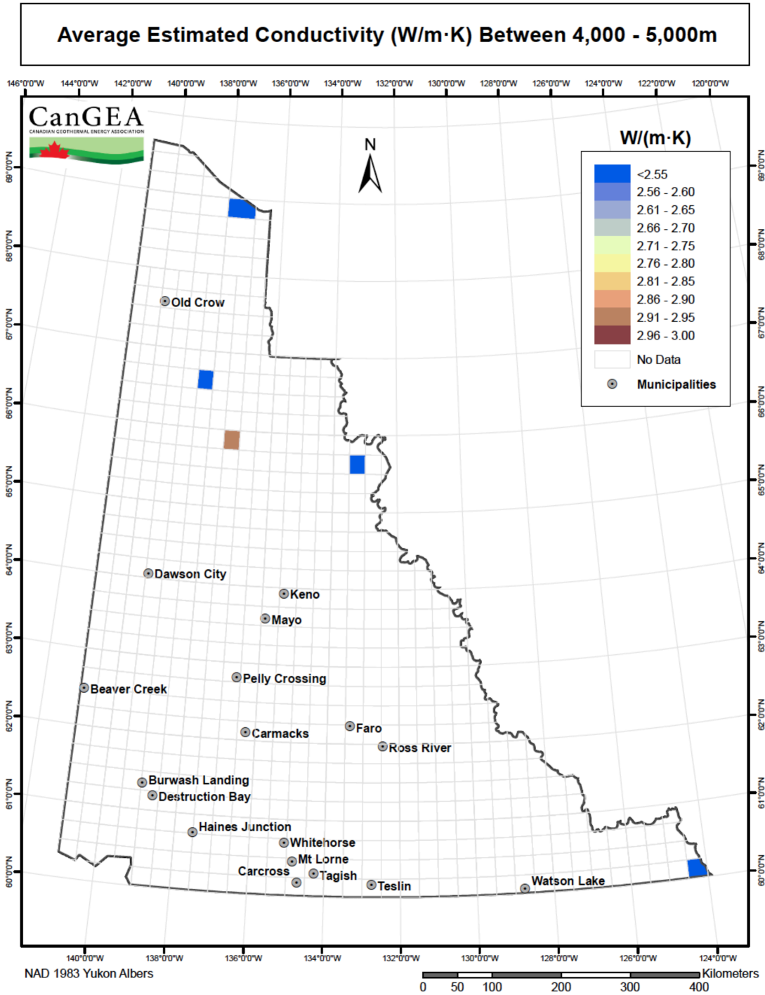
Figure 59: Average estimated conductivity – 4,000m – 5,000m
