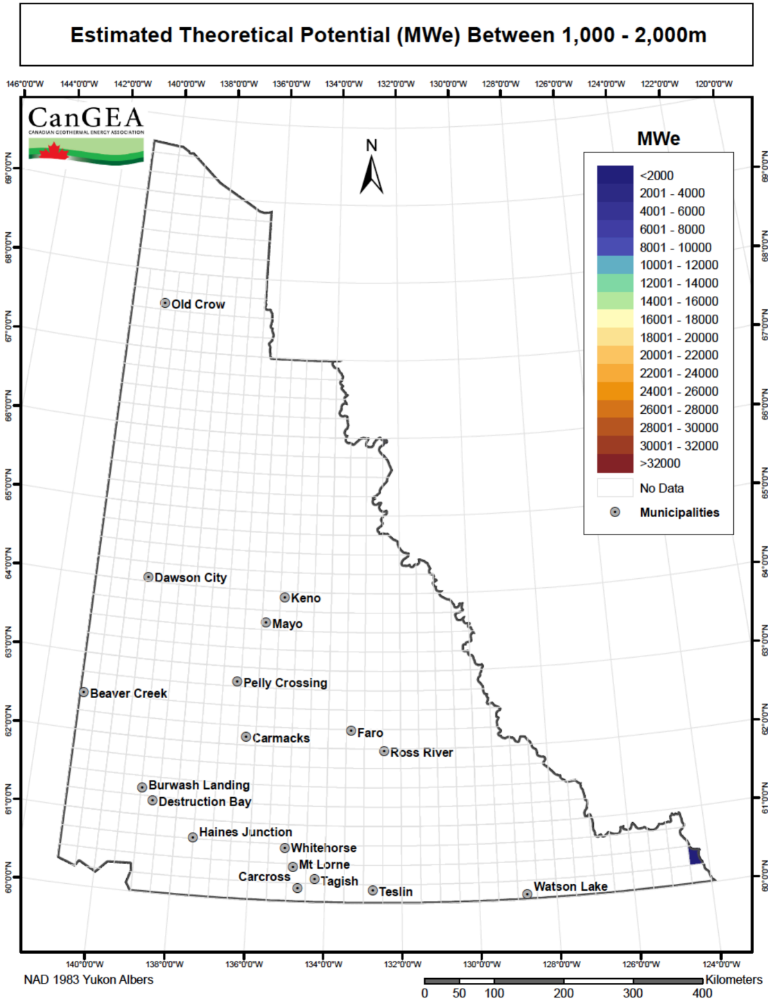
Figure 43: Theoretical potential between 1,000m and 2,000m
