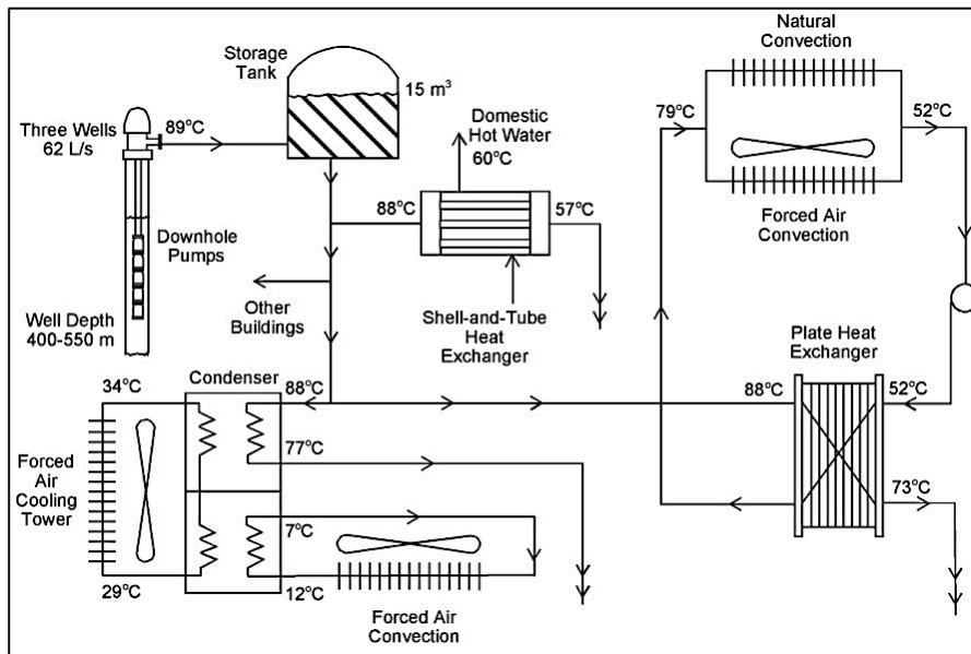
Figure 9: Oregon Institute of Technology heating and cooling system
