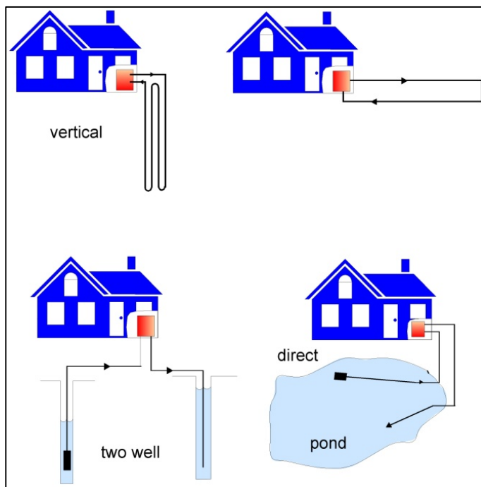
Figure 16: Typical ground-source and groundwater geothermal heat pump installations
