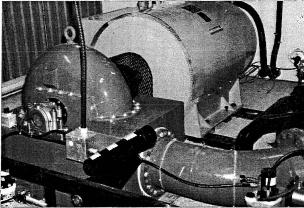
Micro-hydro turbine at Fraser provides power to the Yukon Highways maintenance station. (Photo courtesy of New ERA Corporation)
