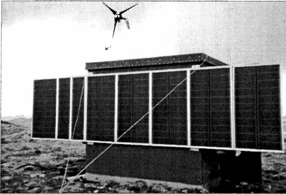
Wind monitoring station on Mount Sumanik, powered by a combination of wind and solar power.
