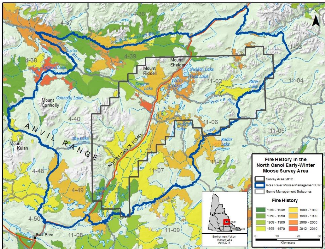
Figure 3. Fire history in the North Canol early-winter moose survey area, southeast Yukon, 2012.
