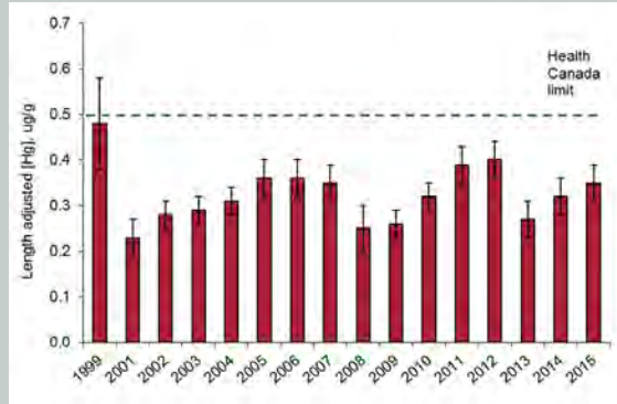
FIGURE 2: Length adjusted mercury concentrations in Kusawa Lake trout (1996-2015).
