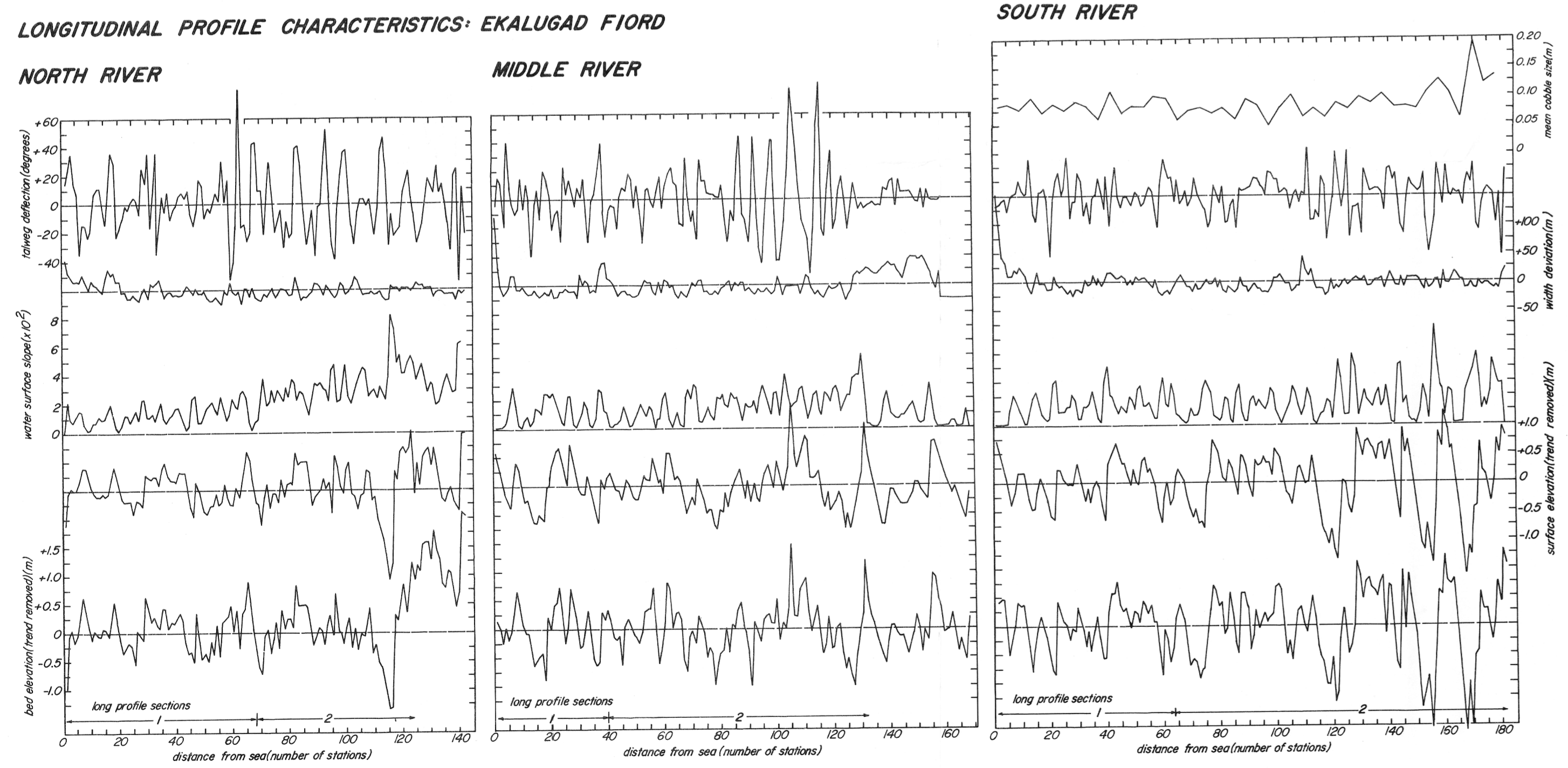
Figure 49. Longitudinal profile characteristics of Ekalugad sandur rivers.
