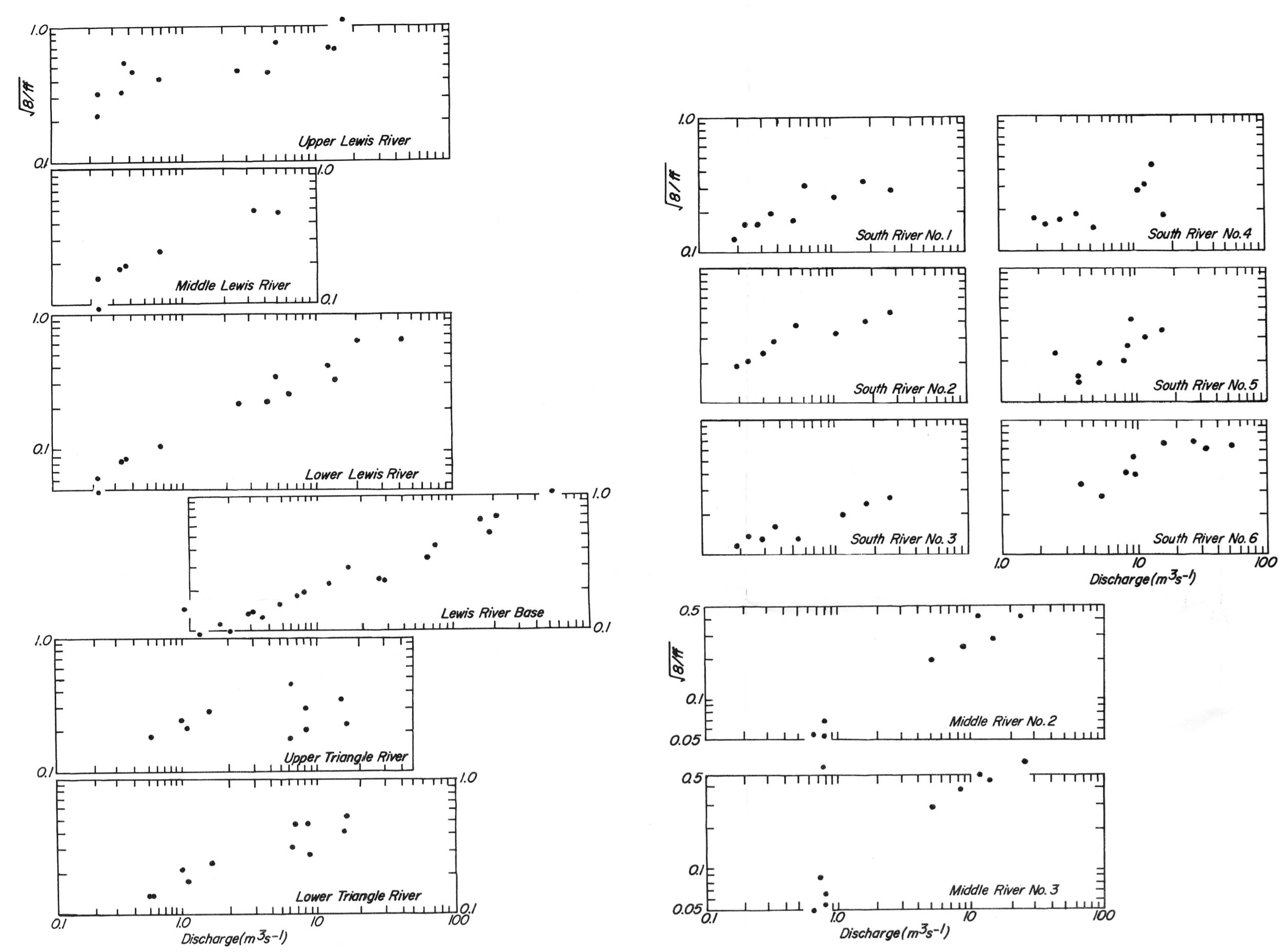
Figure 46. Variation of flow resistance with discharge: A. Lewis River sections B. Ekalugad sandur sections
