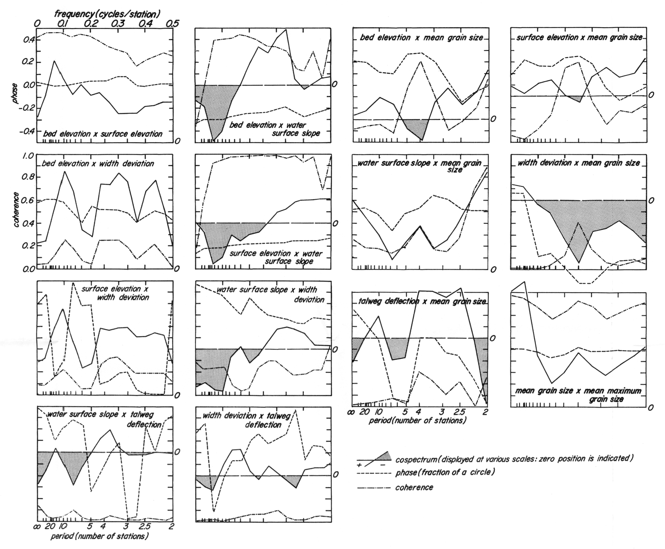
Figure 53. Cross-spectral characteristics in South River, Ekalugad Fjord (including grain size data).
