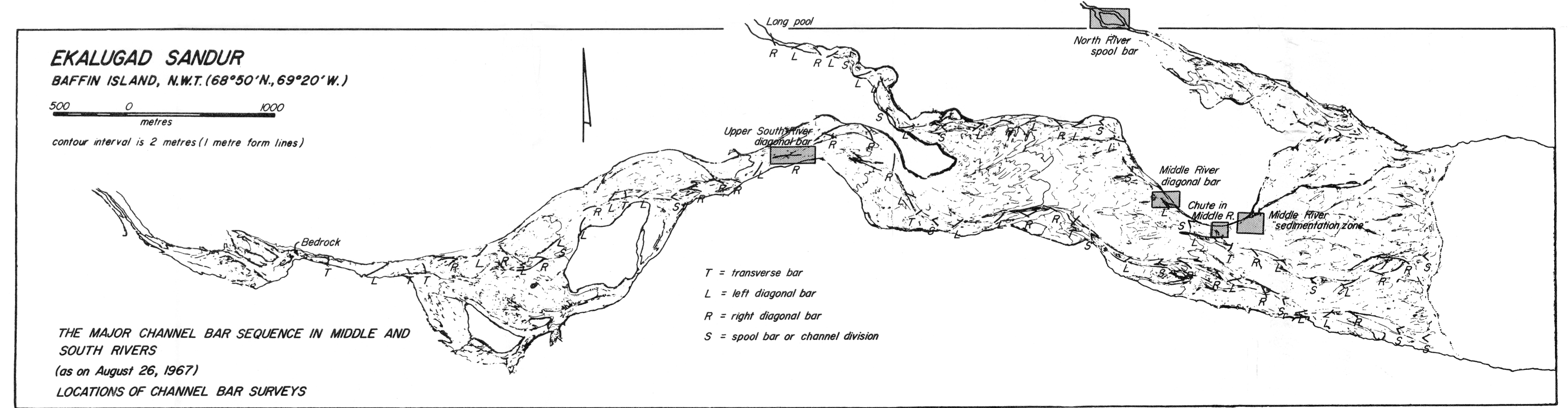
Figure 55. Ekalugad sandur: the major channel bar sequence in Middle and South Rivers and locations of channel bar surveys.
