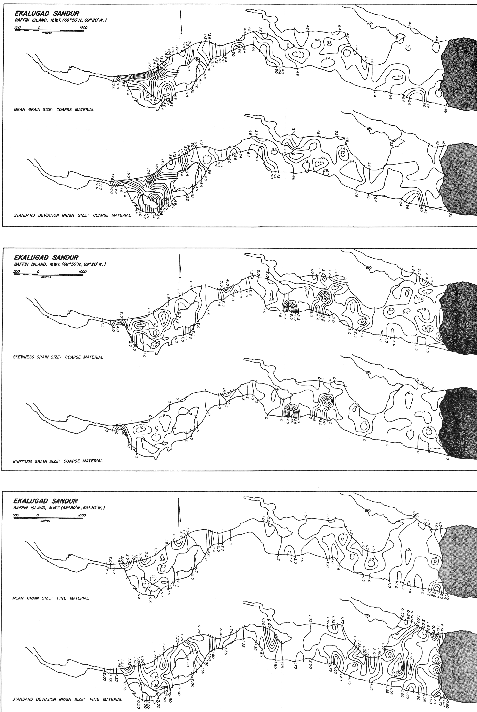
Figure 87. Ekalugad sandur: distribution of materials.
