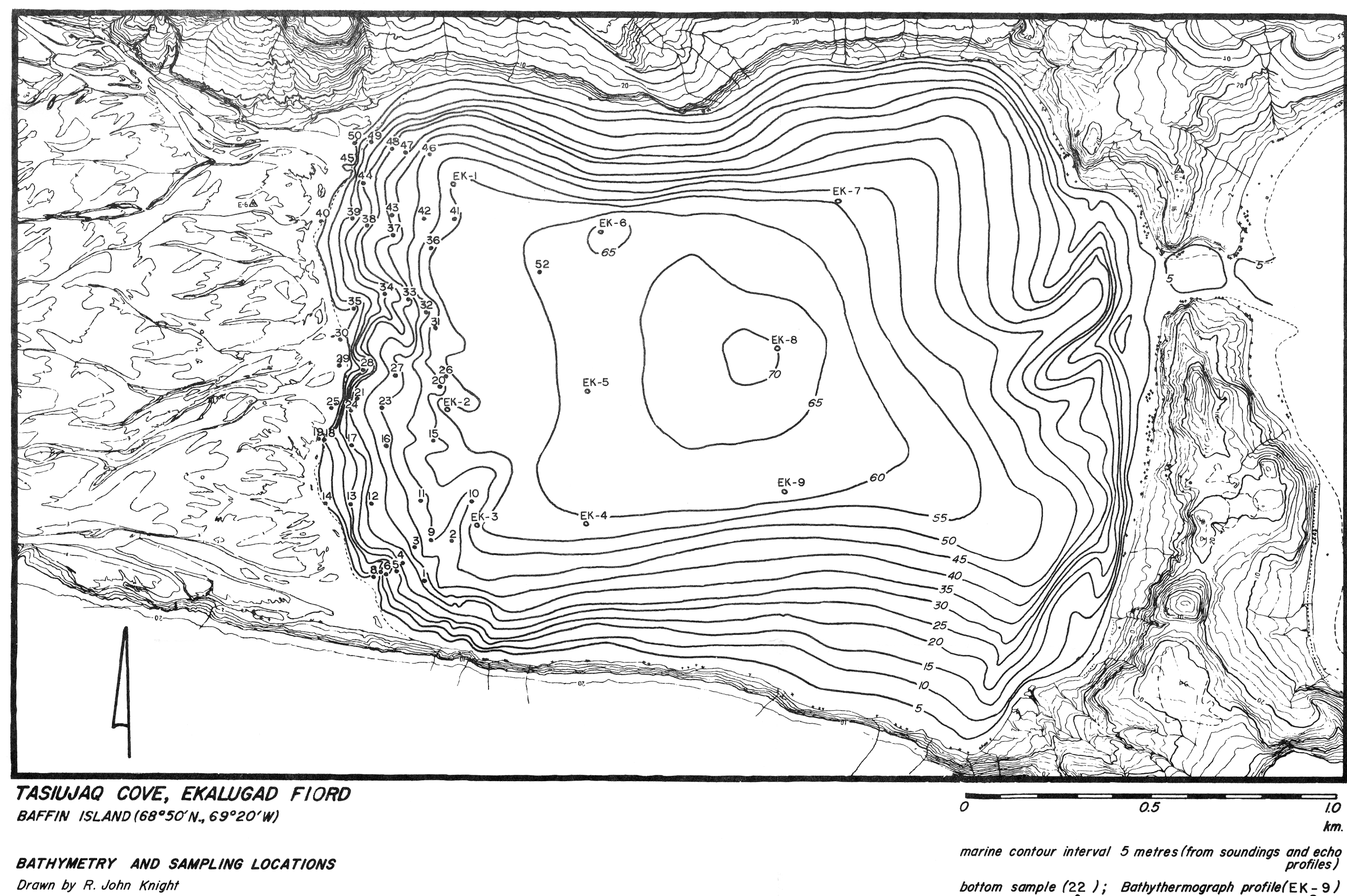
Figure 90. Tasiujaq Cove, Ekalugad Fiord; bathymetry and sampling locations.
