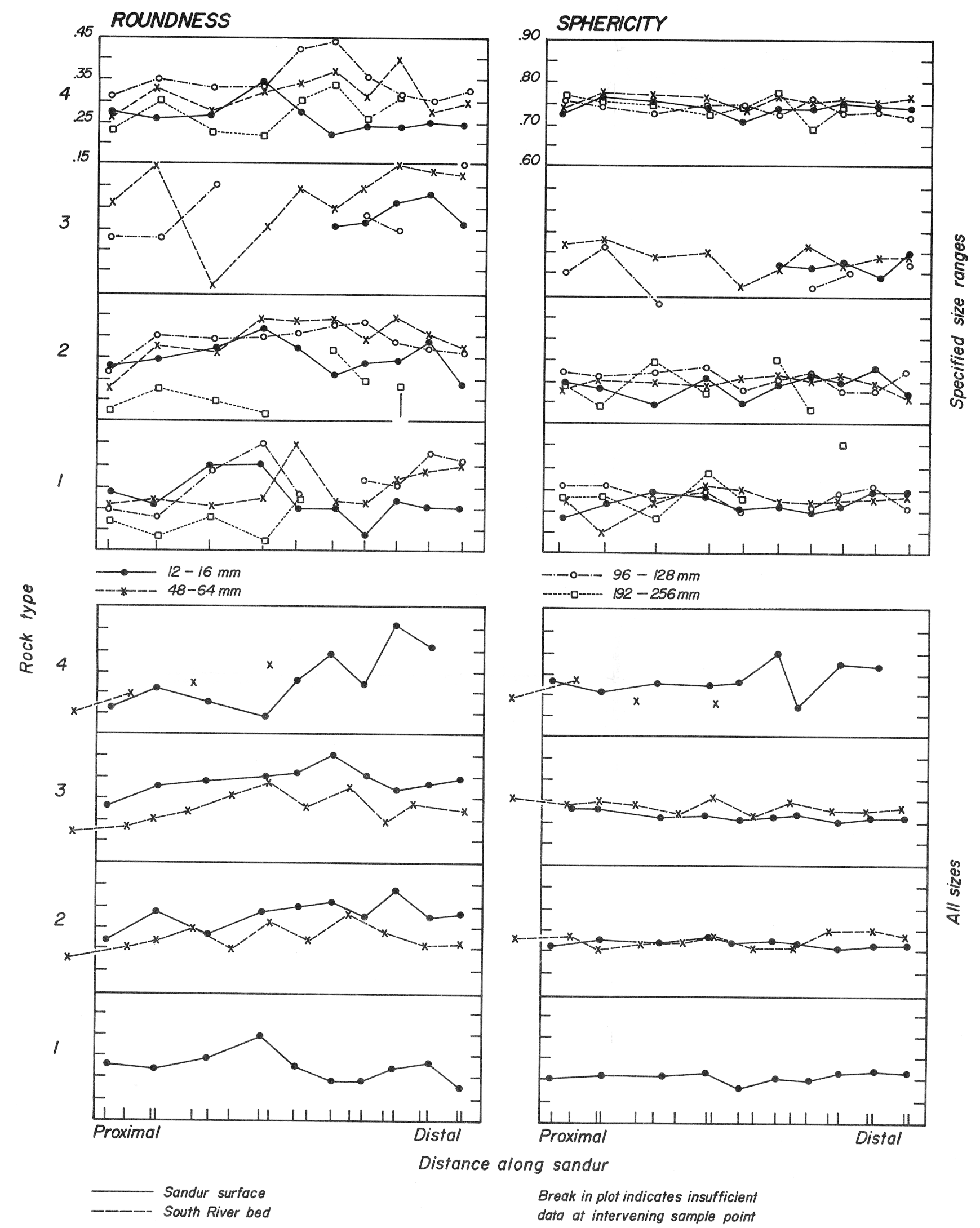
Figure 89. Variation of roundness and sphericity of coarse materials on Ekalugad sandur.
