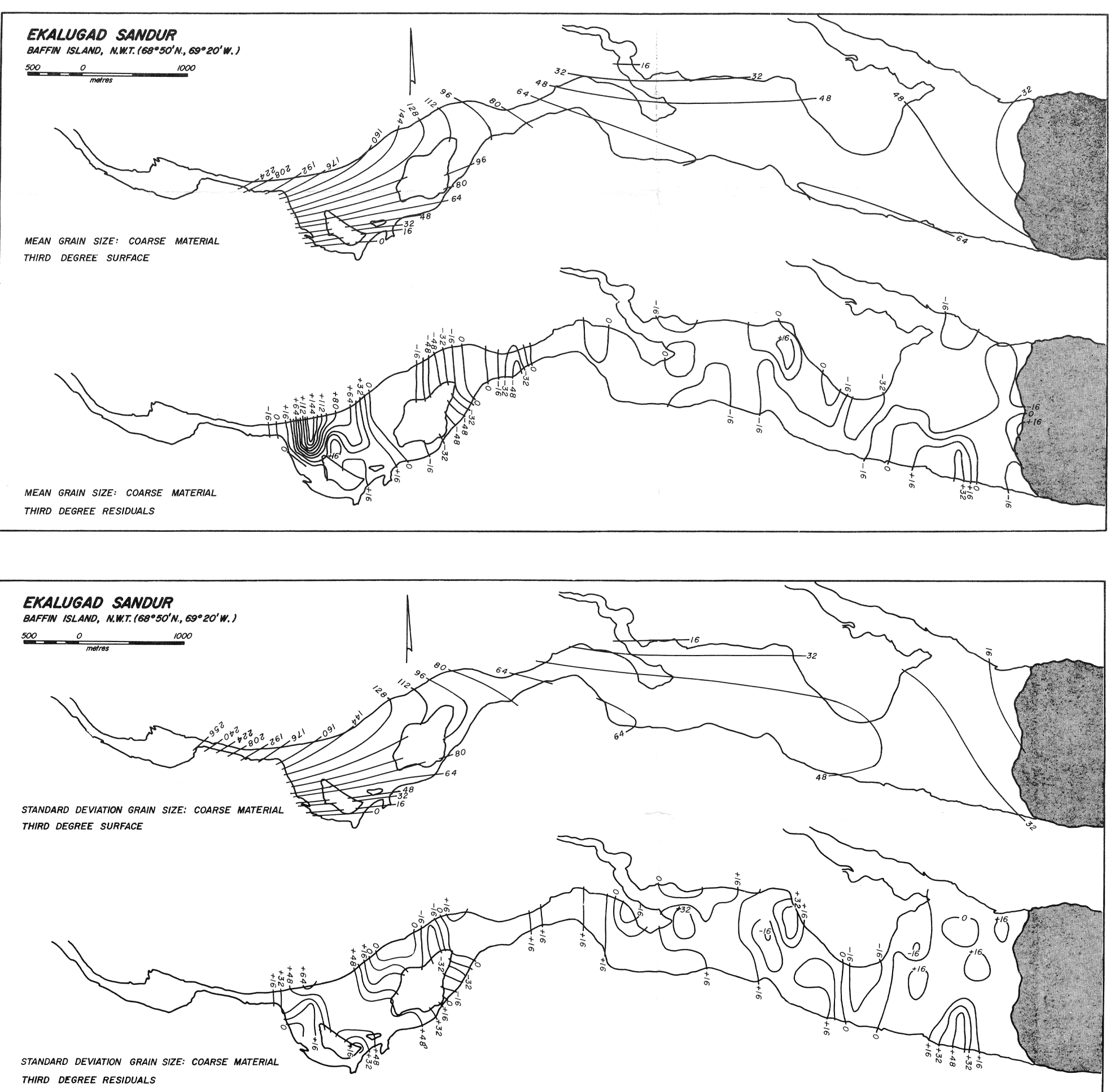
Figure 88. Ekalugad sandur: trend surfaces.
