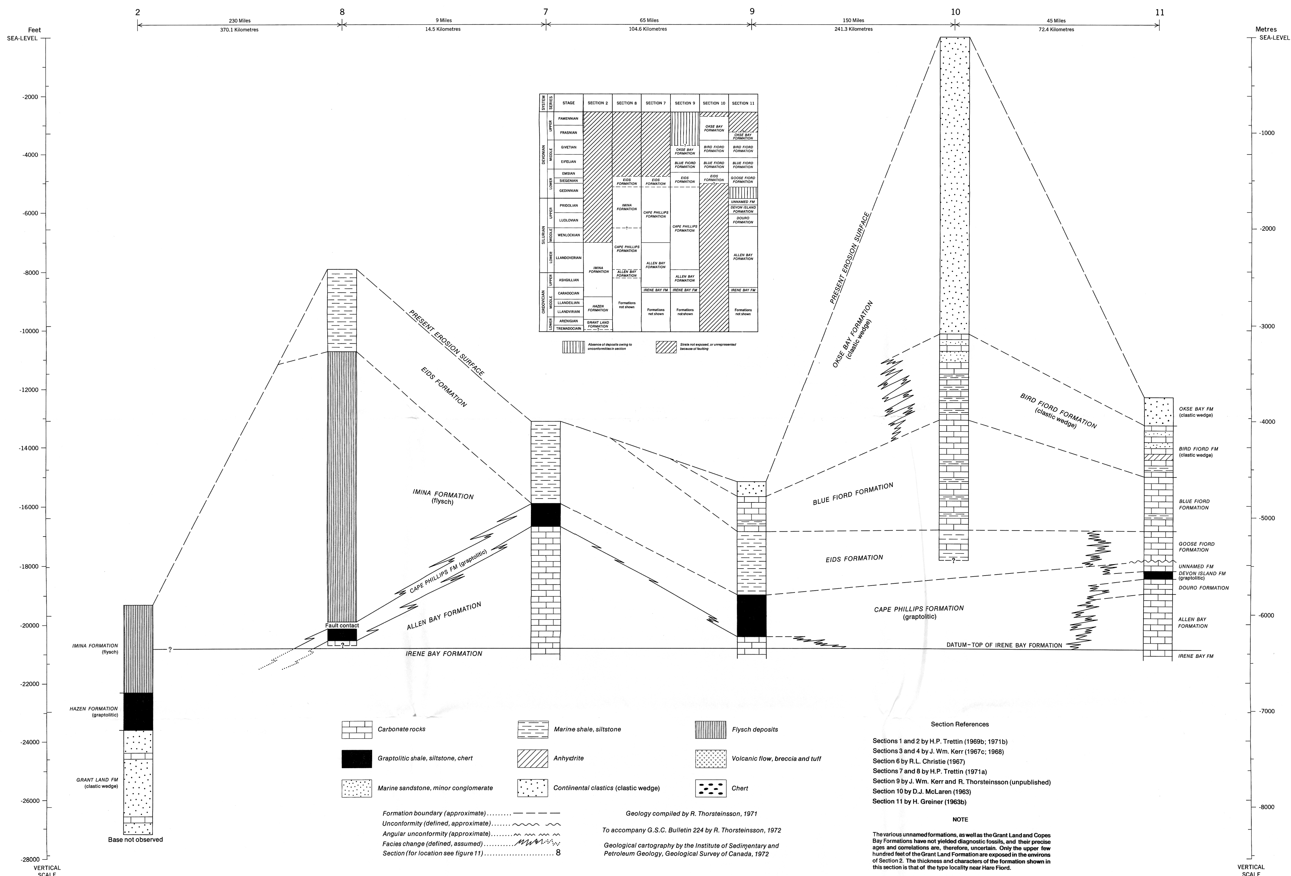
Figure 13. Generalized columnar sections and correlations of Upper Ordovician to Upper Devonian formations from northeast to southwest on Ellesmere Island
