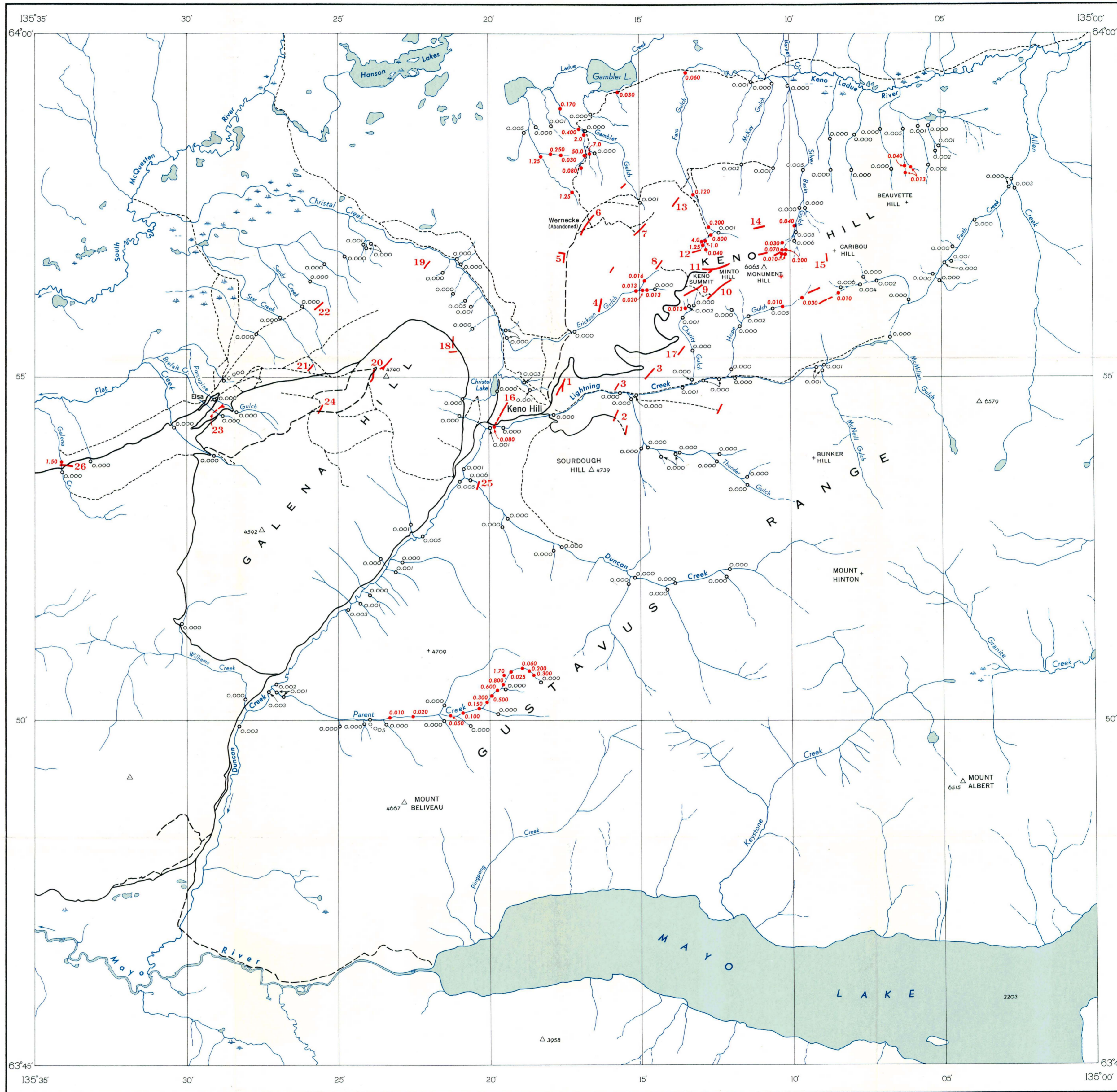
MAP NO. 1 Heavy Metal Content of the Streams in the Keno Hill - Galena Hill Area, Yukon Territory
