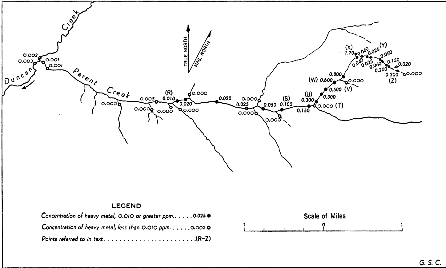
Figure 4. Heavy metal anomalies in the Parent Creek stream system, Yukon Territory.
