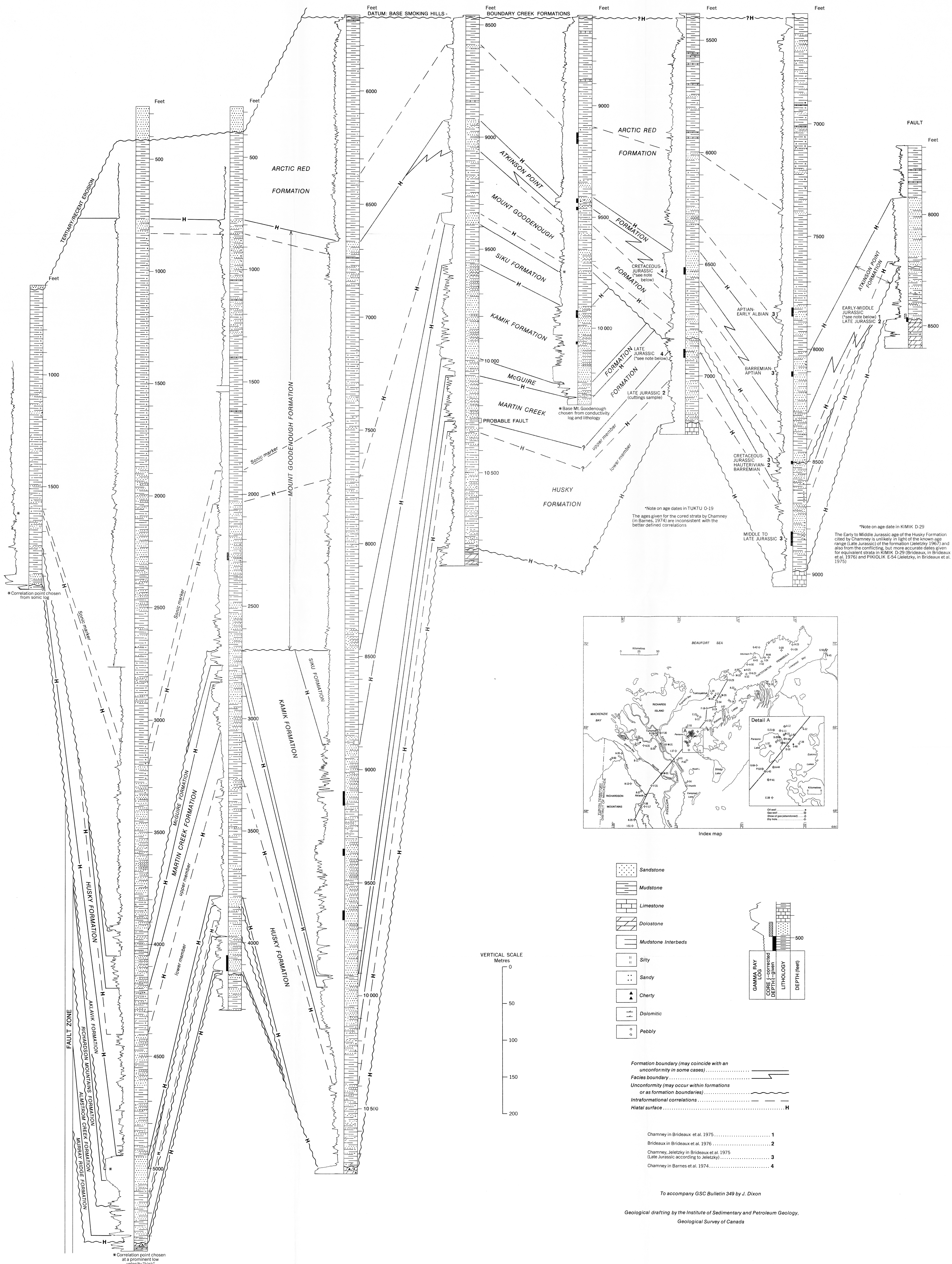
Figure 4. Stratigraphic correlations, Rat Pass A-35 to Kimik D-29
