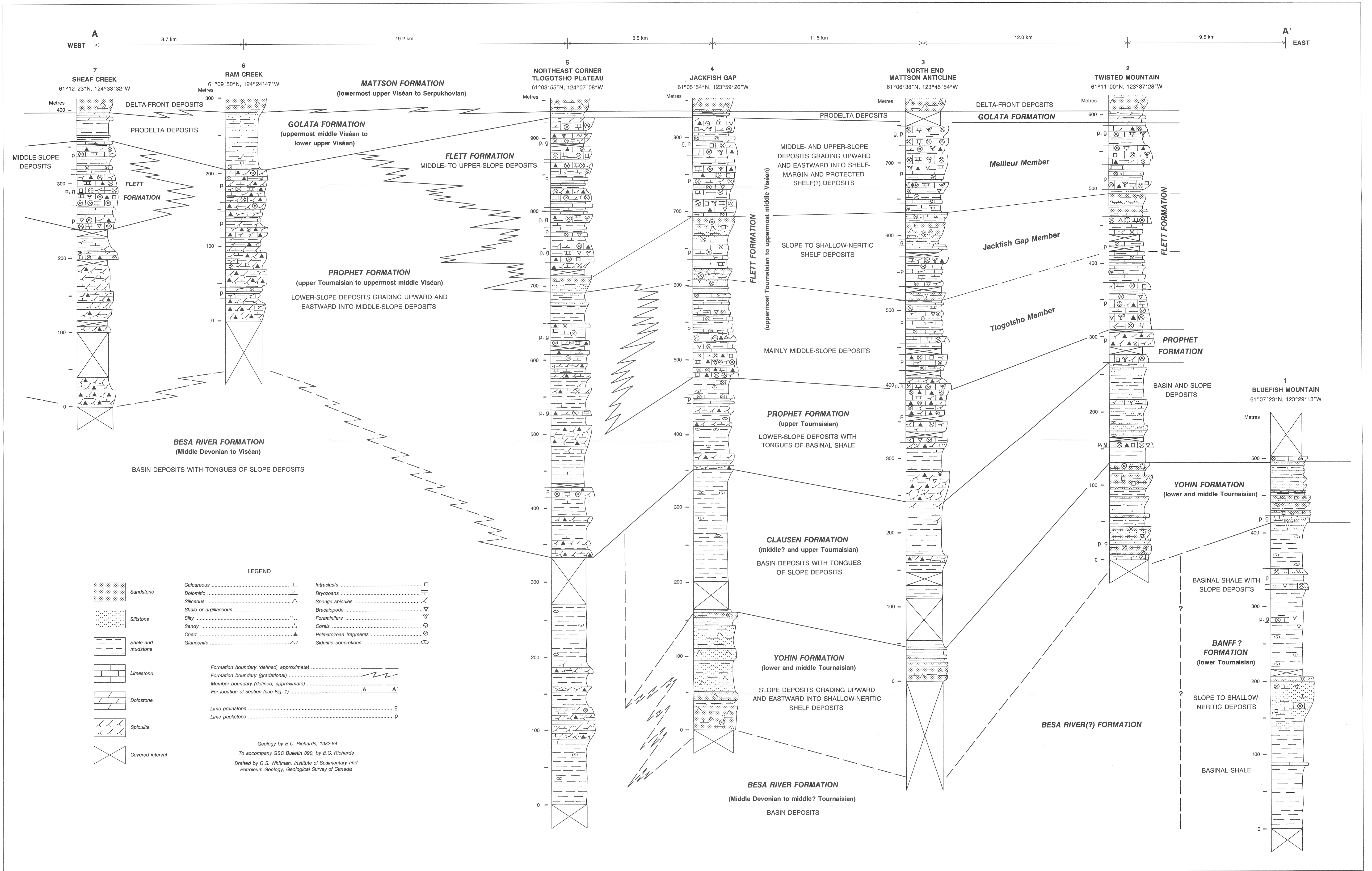
Figure 4. Partially restored cross-section between Bluefish Mountain and Sheaf Creek, southern Mackenzie Fold Belt, southwestern District of Mackenzie.
