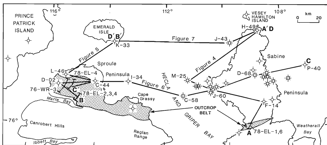
Figure 1. Location of study area showing wells, surface sections, and lines of cross-section for Figures 4, 5, 6, 7. Jurassic outcrop area (stippled) from Tozer and Thorsteinsson (1964).
