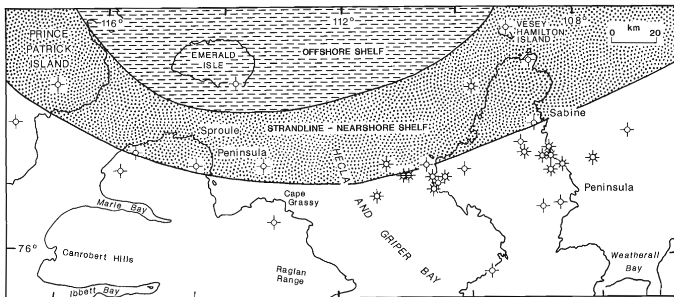
Figure 17. Late Hettangian paleogeography.
