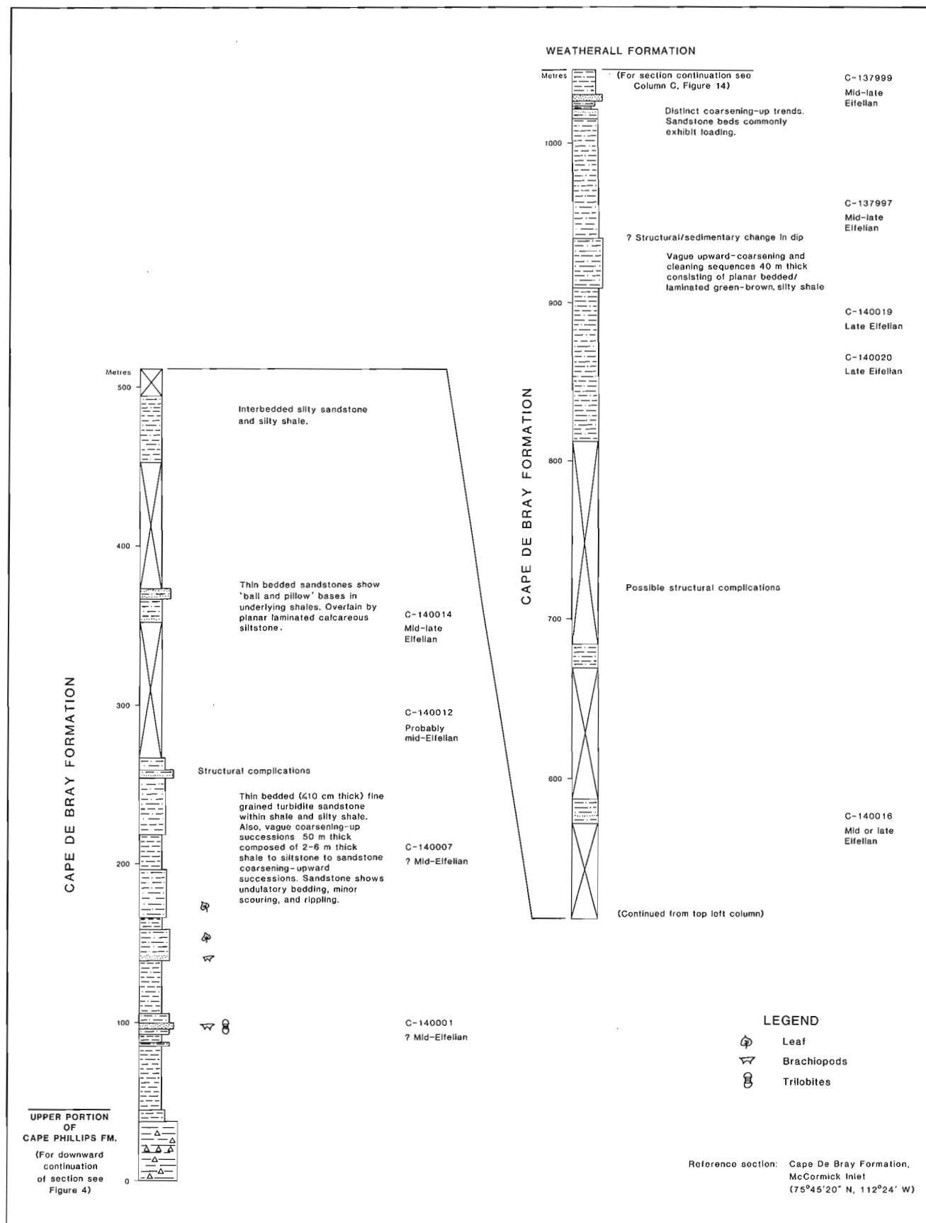
Figure 12. Measured section of the Cape De Bray Formation, 6 km south of McCormick Inlet, central Melville Island. Note the structural complications. Measured by Q. Goodbody. See Figure 4 for legend.
