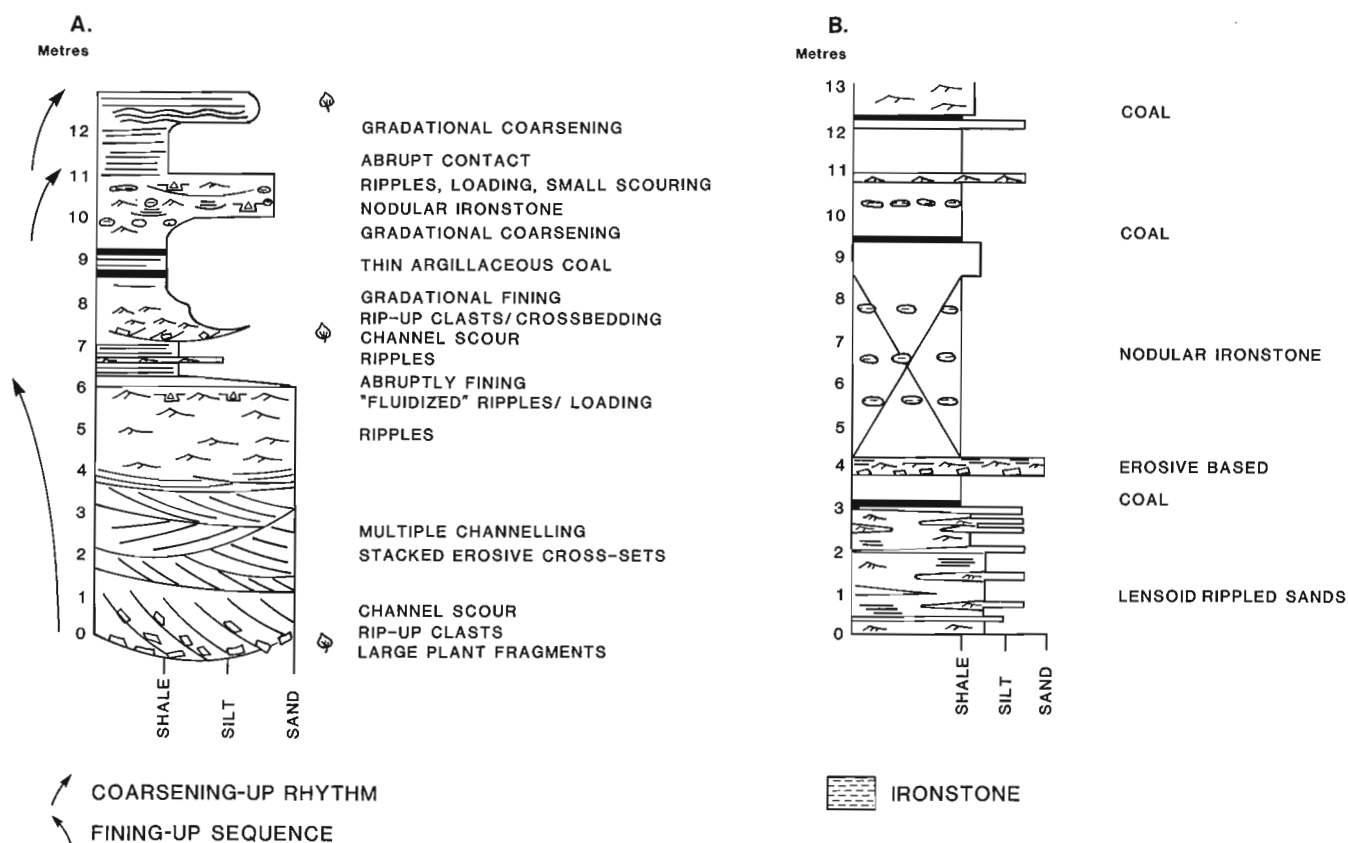
Figure 30. A. Facies association 3, fluvial-meandering to braided. B. Facies association 4, lower delta floodplain, Beverley Inlet Formation.
