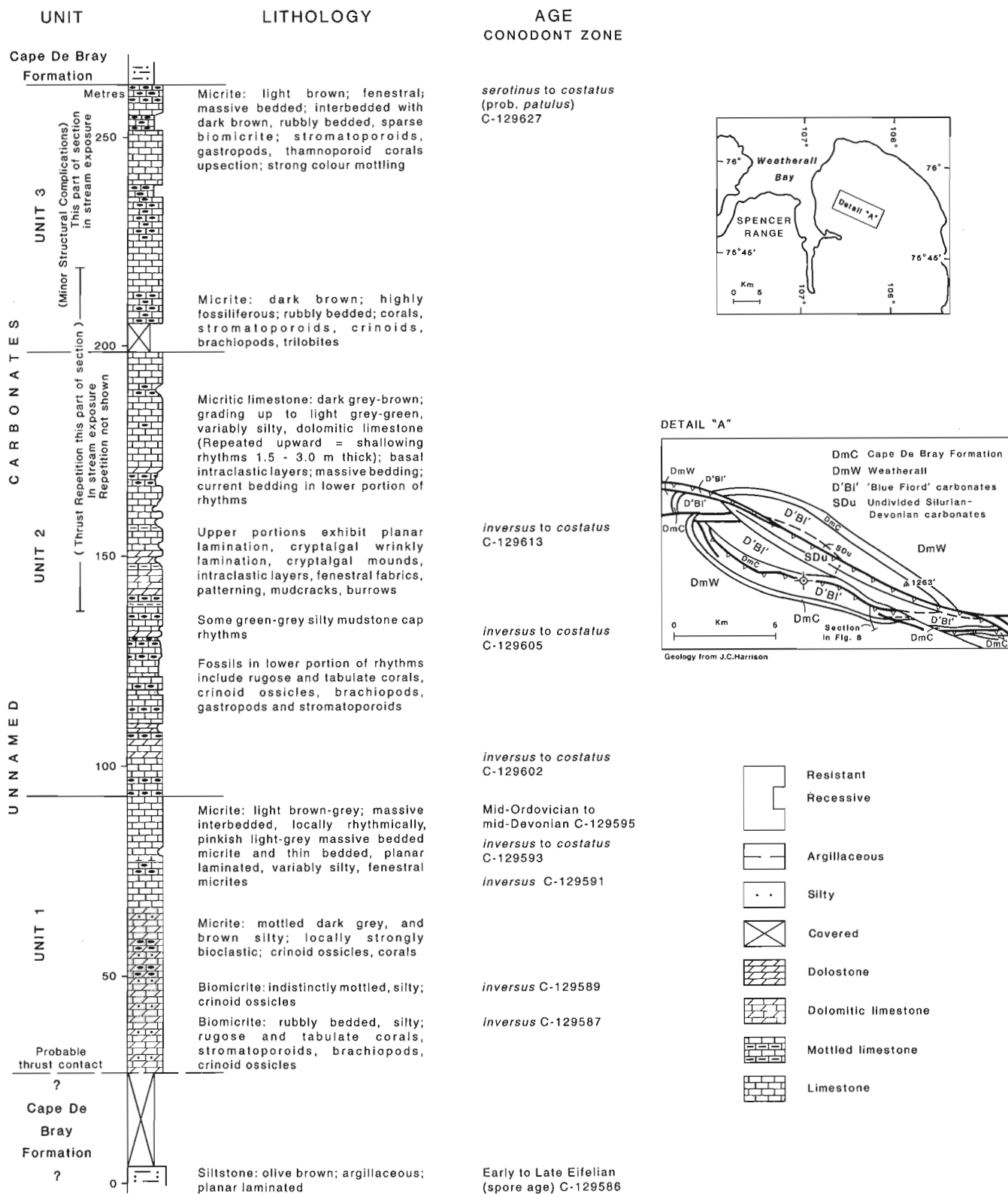
Figure 8. Location and measured section, Towson Point Inlier, eastern Melville Island. Measured by Q. Goodbody.
