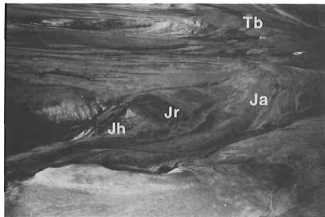
Figure 18. Uppermost Wilkie Point sandstone (Jh; lower slopes, left), overlain by Ringnes Shale (Jr; lower Mould Bay) (centre), which grades up into lower part of the Awingak (Ja; middle Mould Bay) sandstone (right). The rounded noses of the dissected terrace in the upper right portion of the figure are formed by unconsolidated Tertiary (Tb; Beaufort Formation) gravels; ridge north-northeast of Mould Bay weather station, Prince Patrick Island (ISPG photo no. 2578-16).
