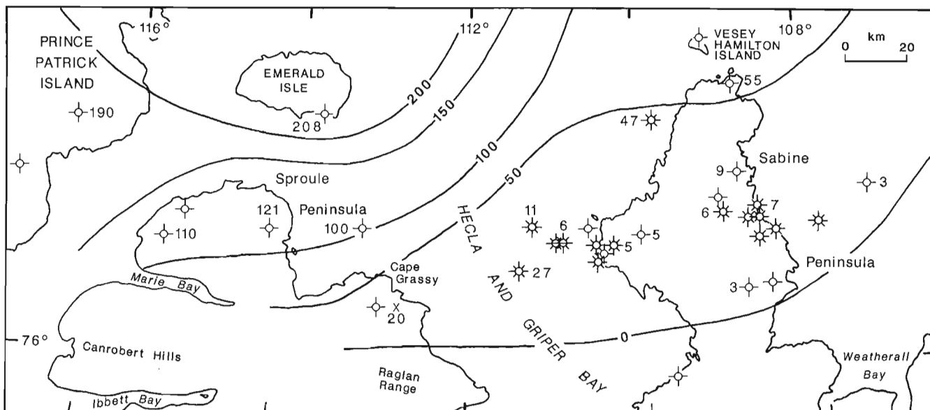
Figure 12. Isopach map, sequence 3, Bajocian-Callovian. Contour interval 50 m.
