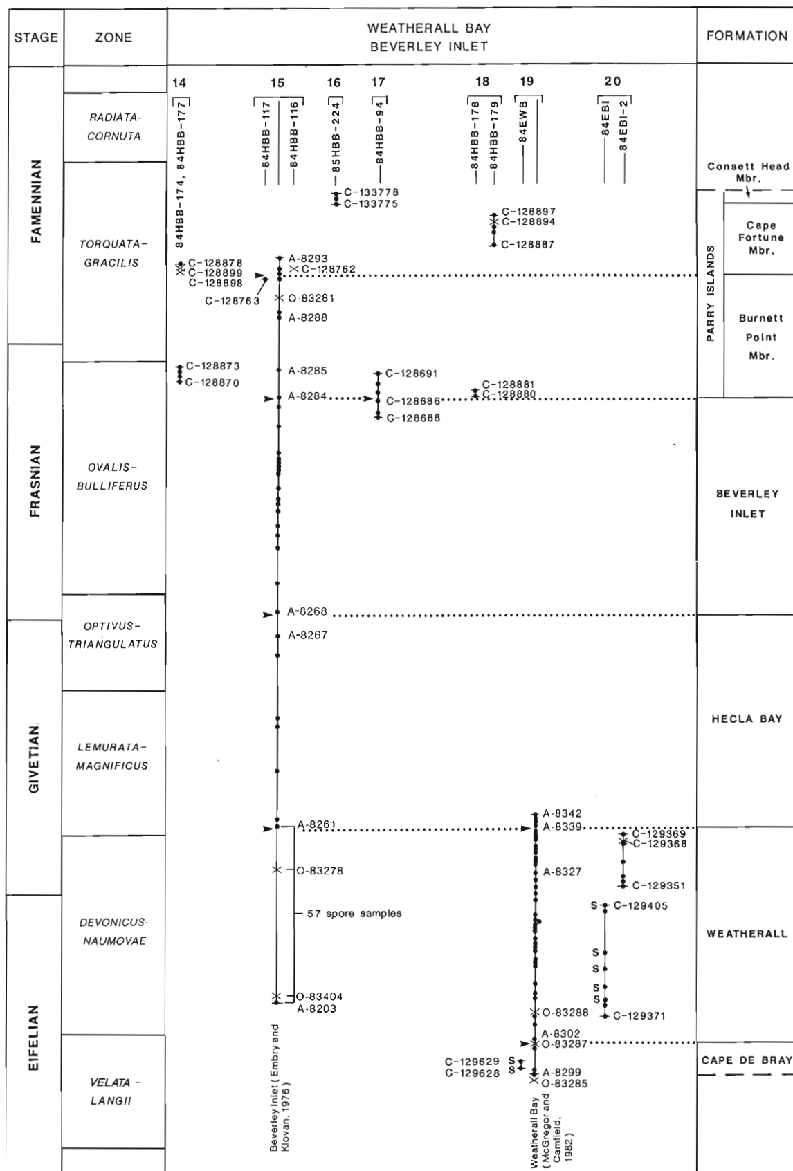
Figure 4. Correlation and age of Middle and Upper Devonian formations of eastern Melville Island, based on spore assemblages. The base of the Hecla Bay Formation according to Embry and Klován (1976) and McGregor and Camfield (1982) is below GSC loc. A-8327 in the Weatherall Bay section (location 19). For further explanation, see caption of Figure 2.
