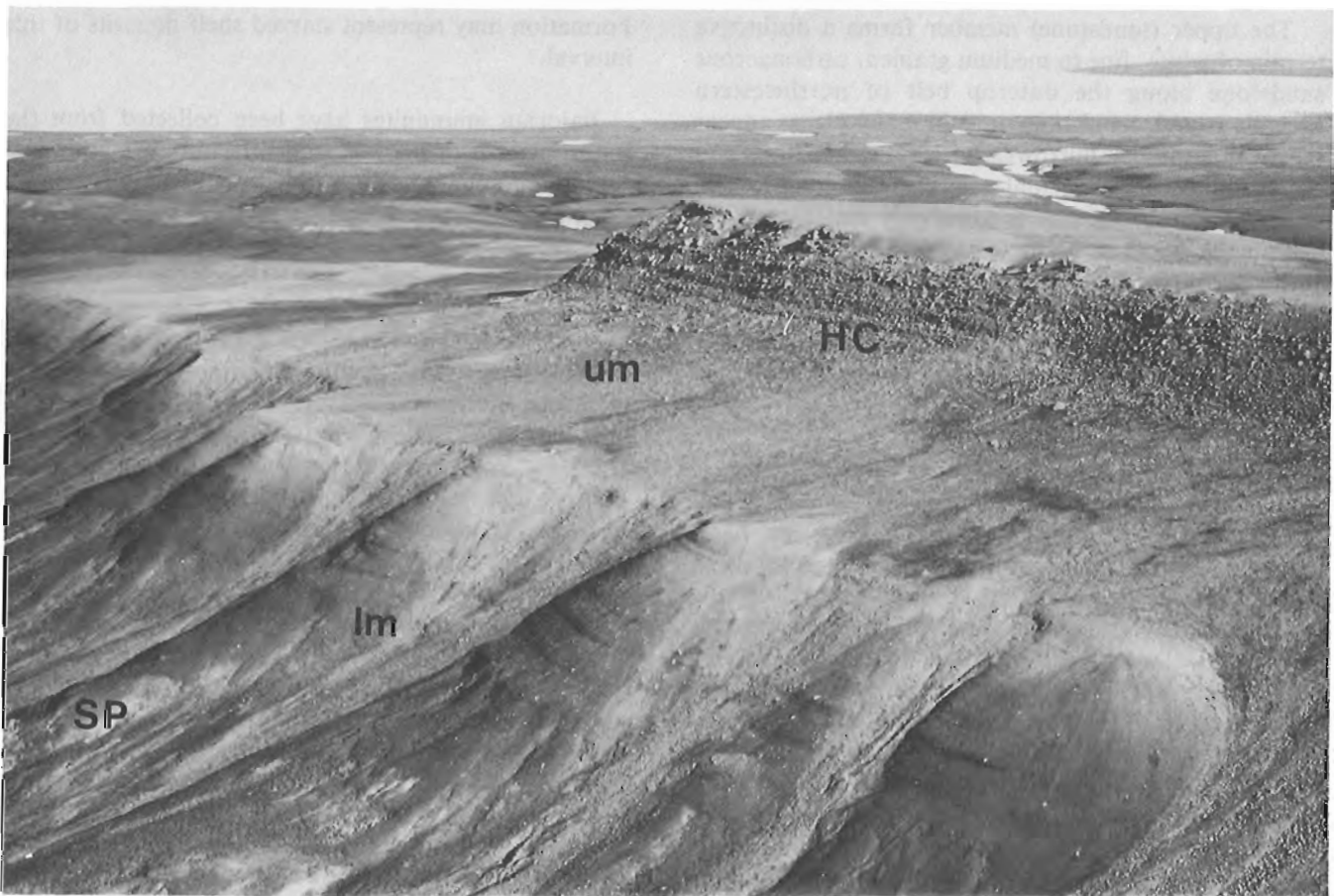
Figure 11. McConnell Island Formation (lm = lower member, um = upper member) unconformably overlying Sandy Point Formation (SP) and conformably overlain by Hiccles Cove Formation (HC), Marie Heights, western Sproule Peninsula. (GSC photo no. 2870-4.)
