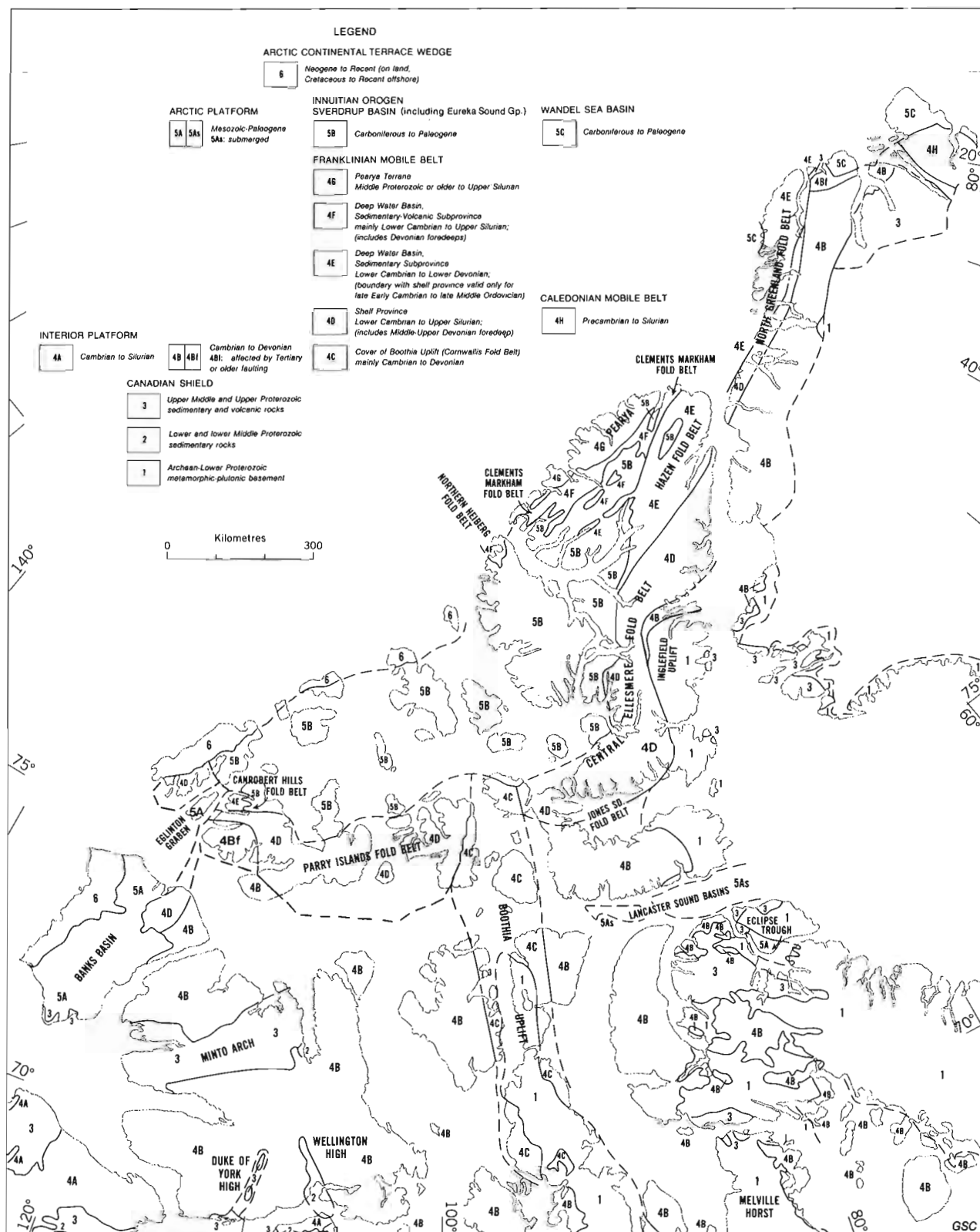
Figure 1. Geological framework of the Arctic islands (modified from Trettin, 1987 and Harrison, 1991a). The Canrobert Hills Fold Belt of northwestern Melville Island was named and first described by Harrison and Bally (1988). In the eastern Arctic, the term "Inglefield Uplift" was first applied by Smith and Okulitch (1987) to a tectonic feature discovered previously by Kerr (1976). Kerr, who called this the Bache Peninsula Arch, believed it was an easterly trending structure of more limited dimension.
