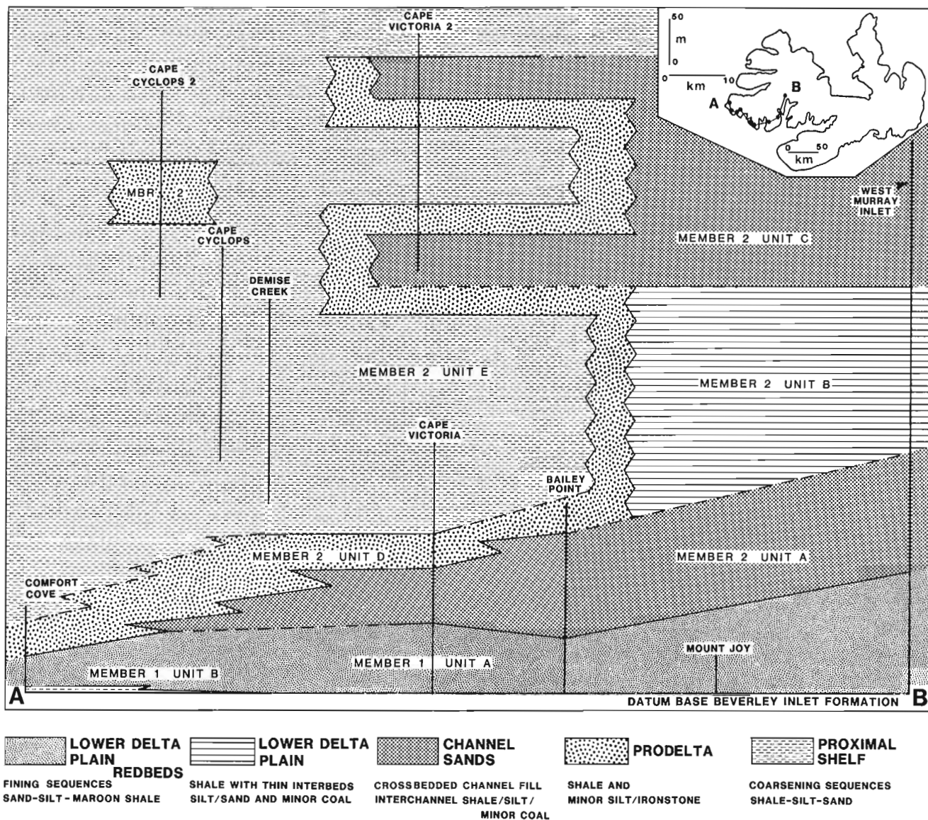
Figure 32. Cross-section, Beverley Inlet Formation, southwestern Melville Island showing relation between measured sections, and distribution of interpreted depositional environments.
