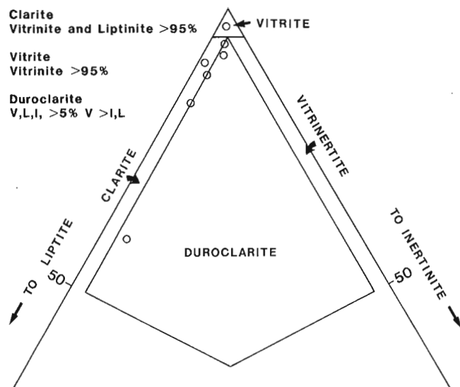
Figure 5. Ternary composition diagram for coal samples from eastern Melville Island.
