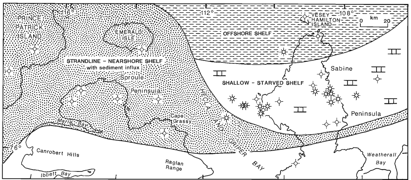
Figure 18. Late Callovian paleogeography.
