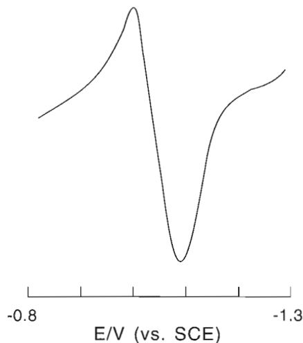
Figure 1. Derivative polarogram. System: 0.9 M \text{H}_2\text{SO}_4 - 2% NaCl - 0.01 \mu\text{g/mL} MBT - 0.5 \mu\text{g} W.
