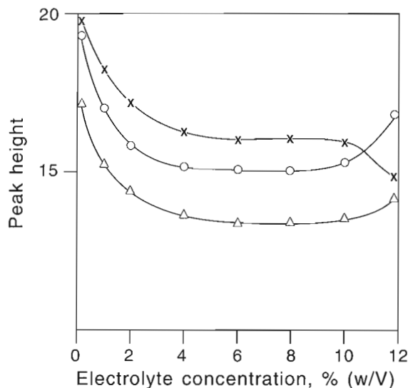
Figure 2. Effect of supporting electrolytes on the peak height. System: 0.9 \text{ M H}_2\text{SO}_4 - 0.01 \mu\text{g/mL MBT} - 0.5 \mu\text{g W} . Electrolyte: \circ NaCl \Delta KCl \times \text{NH}_4\text{Cl} .
