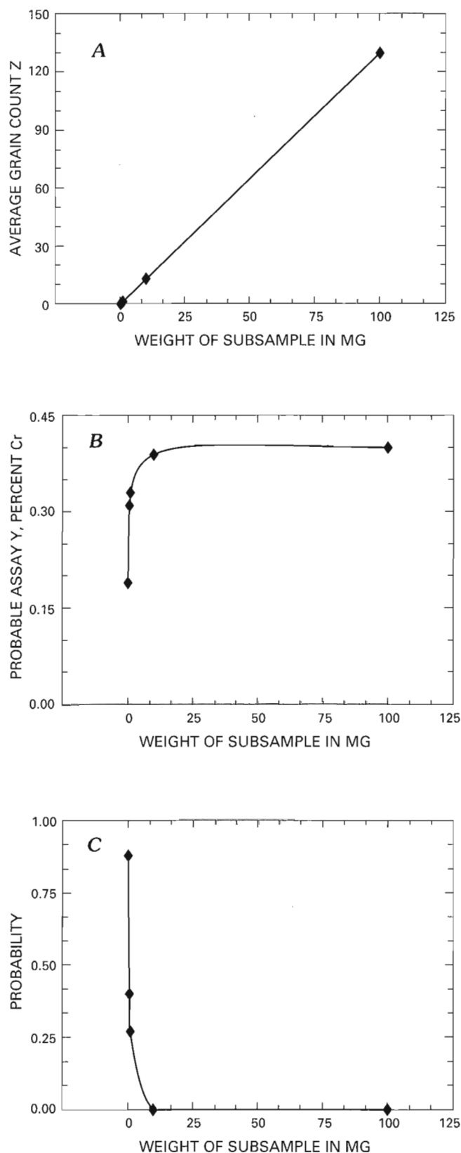
Figure 3. Sampling parameters for chromite in USGS DTS-1 as a function of subsample weight. A. Z, average grain count. B. Y, most probable chromium assay. C. probability that subsample will contain no grains of mineral species.
