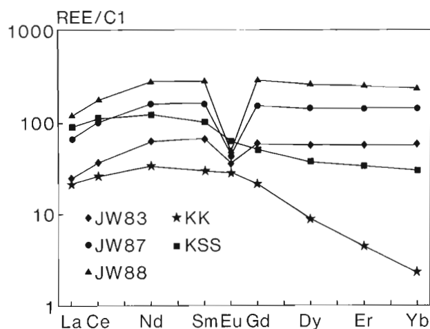
Figure 1. Abundances of REEs in investigated amphiboles, normalized to chondrite values.
