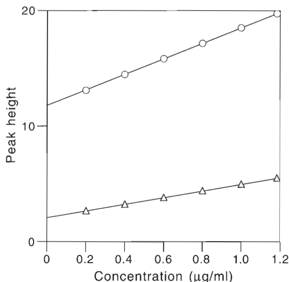
Figure 3. Comparison between W current and MBT background. System: \circ 0.9 \text{ M H}_2\text{SO}_4 - 2\% \text{ NaCl} - 0.01 \mu\text{g/mL MBT} - \text{W} (\times 10^{-1}) . Background: \Delta 0.9 \text{ M H}_2\text{SO}_4 - 2\% \text{ NaCl} - \text{MBT} (\times 10^{-2}) .
