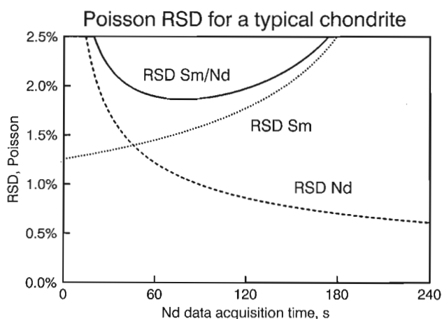
Figure 2. Poisson RSD for the determination of Sm/Nd, Sm, and Nd in a rock having concentrations of a typical chondrite. The RSD is presented as a function of the data acquisition time of Nd from 0 to 240 s, while the total data acquisition time for Sm plus Nd is held constant at 240 s.
