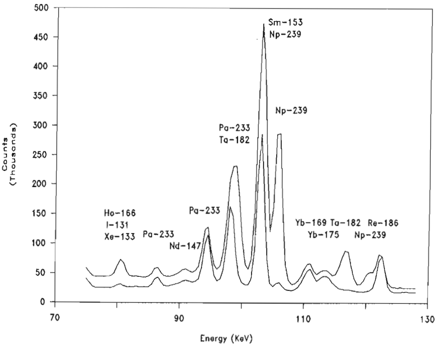
Figure 3. Interference Reduction. Sample: SY-2; Pa-233 is produced by Th; Np-239, I-131 and Xe-133 are produced by U.
