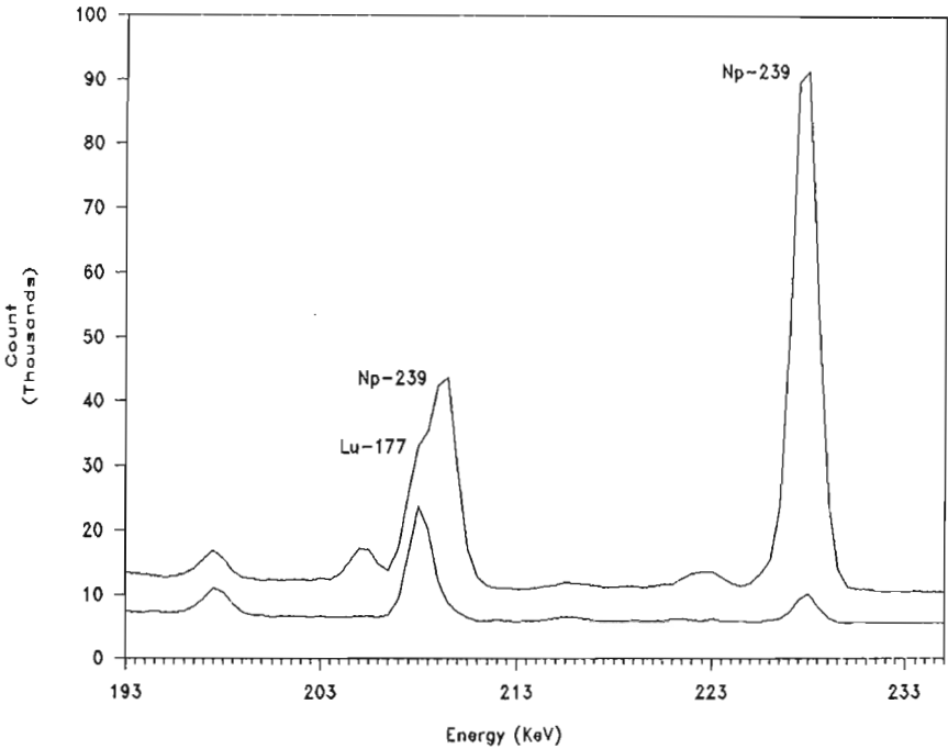
Figure 2. Interference Reduction. Sample: SY-2; Np-239 is produced by U.
