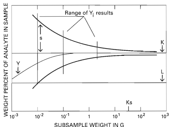
Figure 1. Theoretical sampling diagram; Y, K, Y_i, L as defined by/for equation 2; S as defined by equation 5; K_s as defined by equation 6.
