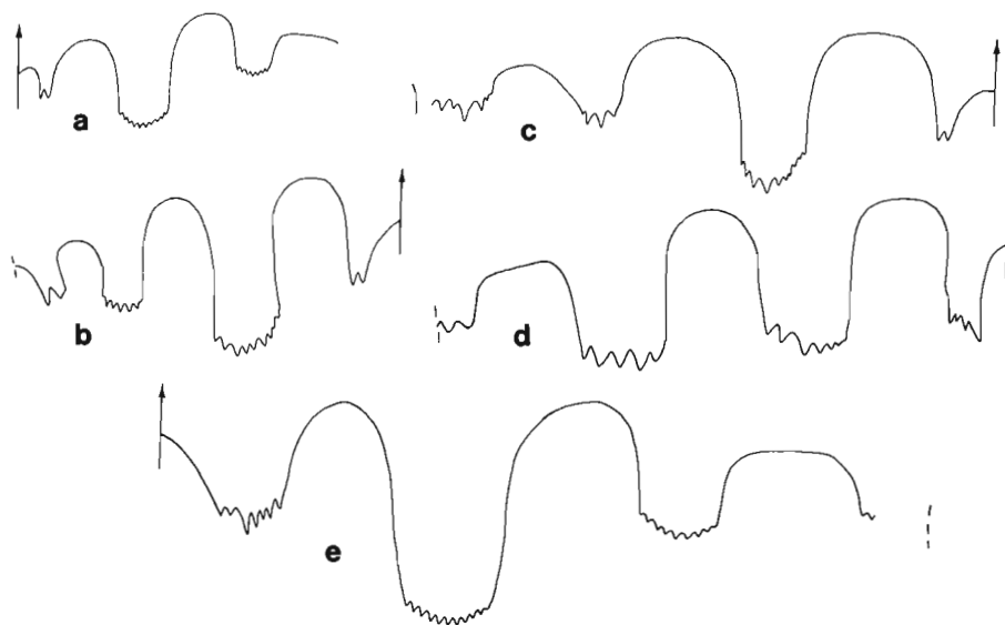
Figure 11. Sutures. a, Pleurogyronites krafftii n. sp., GSC 14269 (Pl. 10, fig. 5) x4; b, Proptychites newelli Tozer, GSC 14270 (Pl. 10, fig. 3) x4; c, Proptychites kummeli Tozer, GSC 14272 (Pl. 10, fig. 4) x4; d, Dunedinites pinguis Tozer, GSC 14287 (Pl. 10, fig. 2) x4; e, Meekophiceras columbianum (Tozer), GSC 14266 (Pl. 10, fig. 1) x4.
