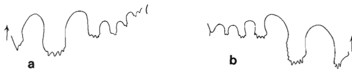
Figure 28. Sutures. a, Groenlandites canadensis n. sp., GSC 28457 (Pl. 40, fig. 12), x4; b, Groenlandites amplus n. sp., GSC 28461 (Pl. 40, fig. 13), x2.
