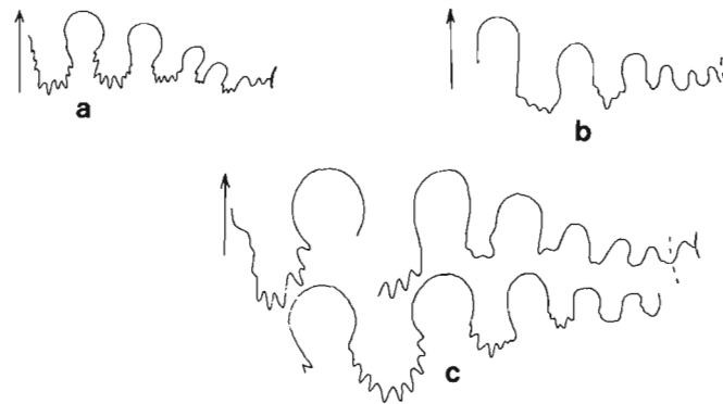
Figure 42. Sutures. a, Stenopopanoceras angulatum n. sp., GSC 28251 (Pl. 57, fig. 1) x3; b, Amphipopanoceras medium (McLearn), GSC 28254 (Pl. 57, fig. 7) x3; c, Stenopopanoceras obesum (McLearn), GSC 28253 (Pl. 57, fig. 5) x3.
