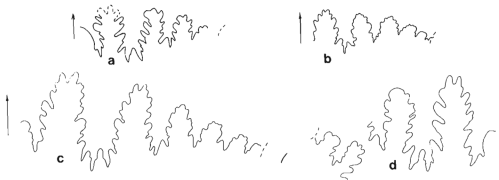
Figure 91. Sutures. a, b. Griesbachites laevis n. sp. a, GSC 32206 (Pl. 114, fig. 5) x2; b, GSC 32207 (Pl. 114, fig. 6) x2; c, Dimorphites pardonetiensis McLearn, GSC 12602 (McLearn, 1960a Pl. 16, figs. 1a–c); d, Gonionotites spiekeri McLearn, GSC 8807 (McLearn, 1960a, Pl. 14, fig. 1) x4.
