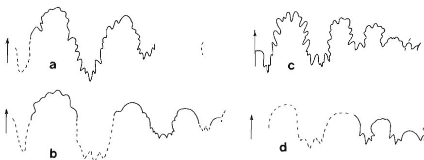
Figure 98. Sutures. a, d. Juvavites concretus McLearn. a, GSC 8818 (McLearn, 1960a, Pl. 9, fig. 2) x2; d, GSC 32248 (Pl. 123, fig. 6) x2; b, Juvavites magnus McLearn, GSC 8837 (McLearn, 1960a, Pl. 9, fig. 1) x2; c, Juvavites levigatus n. sp., GSC 32244 (Pl. 121, fig. 7) x2.
