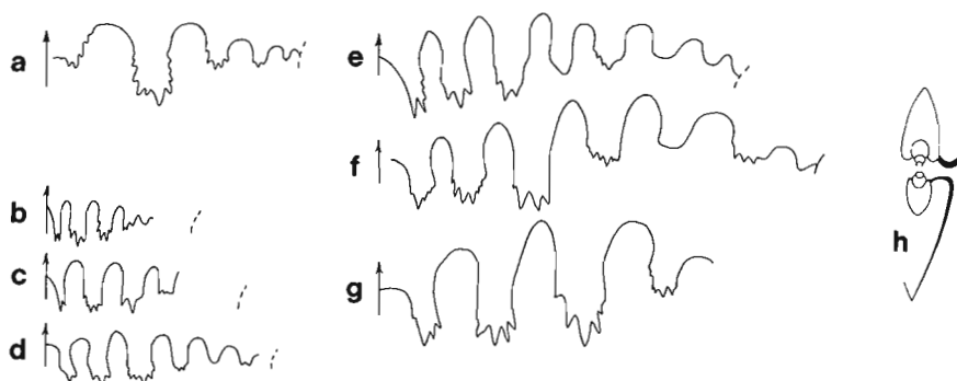
Figure 44. Sutures and section. a, Gymnotoceras smithi n. sp., GSC 28326 (Pl. 59, fig. 13), x2. b–h. Intornites canadensis (McLearn). b, e, GSC 6449 (McLearn, 1969, Pl. 6, fig. 1) x2; c, GSC 28542 (Pl. 59, fig. 3) x2; d, GSC 28547 (Pl. 59, fig. 5) x2; f, GSC 28549 (Pl. 59, fig. 8) x2; g, GSC 28544 (Pl. 59, fig. 9) x2; h, GSC 28548* x1.
