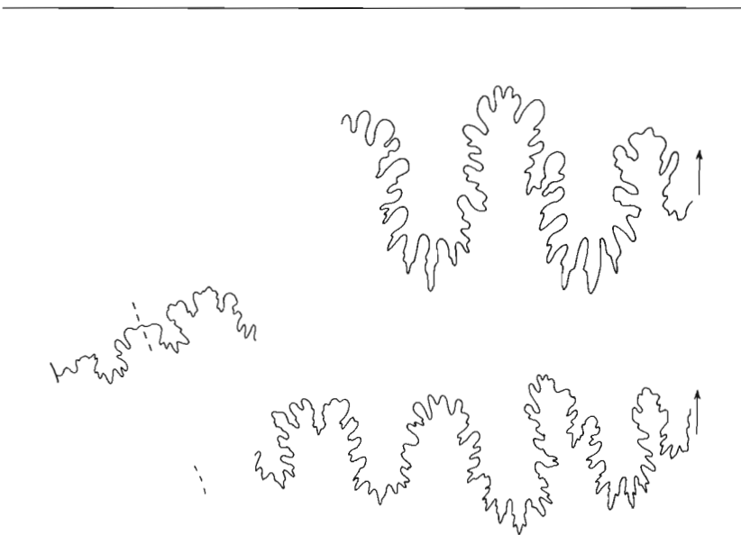
Figure 52. Sutures. Arctoptychites lingulatus n. sp., GSC 28409 (Pl. 69, fig. 5) x4.
