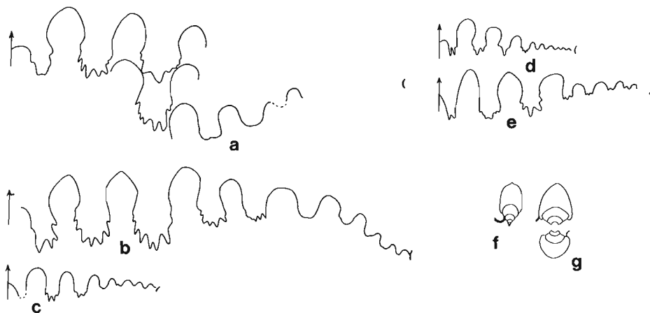
Figure 53. Sutures and sections. a–c, g. Indigirites freboldi n. sp. a, GSC 28576 (Pl. 70, fig. 11) x4; b, GSC 28589 (Pl. 70, fig. 18) x4; c, GSC 28583* x4; g, GSC 28582 x1. d–f. Eonathorstites dieneri n. sp., d, GSC 28571 (Pl. 70, fig. 3) x4; e, GSC 28568 (Pl. 70, fig. 4) x4; f, GSC 28574* x1.
