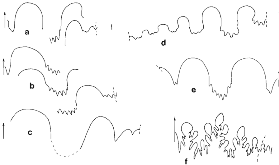
Figure 63. Sutures. a, Asklepioceras exilis n. sp., GSC 28776 (Pl. 80, fig. 3). b, c, Asklepioceras altilis n. sp. b, GSC 28777 (Pl. 80, fig. 5) x4; c, GSC 28779 (Pl. 80, fig. 4) x4; d, Hungarites inermis n. sp., GSC 28368 (Pl. 80, fig. 1) x4; e, Zestoceras nitidum n. sp., GSC 28770 (Pl. 80, fig. 9), x4; f, Monophyllites aonis Mojsisovics, GSC 32348* x2.
