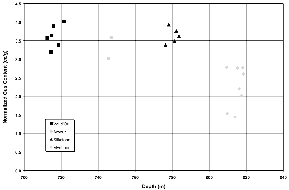
Figure 136. Normalized gas content versus depth of intersection, BHP Peco samples.
