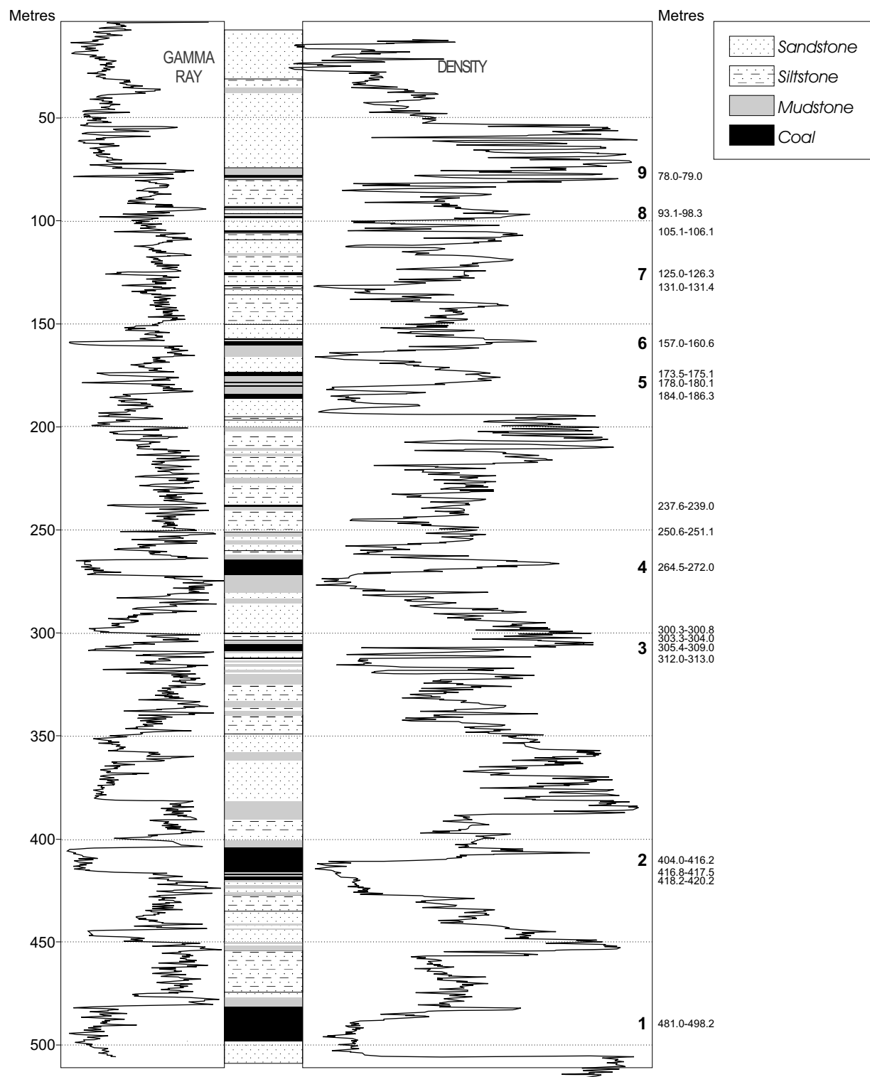
Figure 13. Detailed stratigraphic section of the KPP90-1 borehole.
