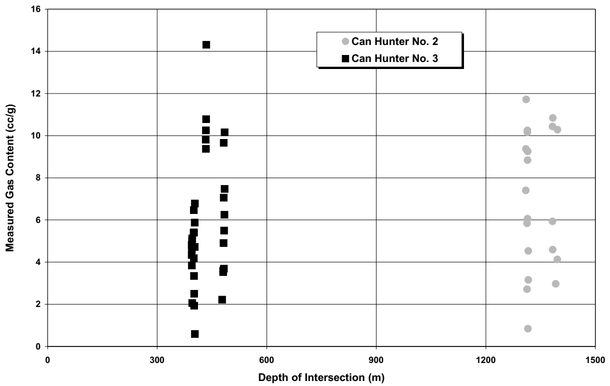
Figure 46. As measured gas content versus depth of intersection, Canadian Hunter Nos. 2 and 3.
