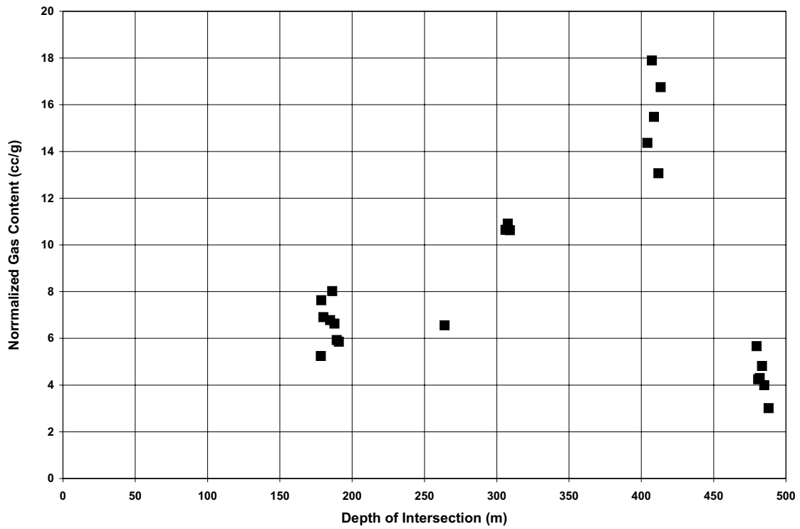
Figure 6. Normalized gas content versus depth of intersection for all coal samples, wellbore a-65-E.
