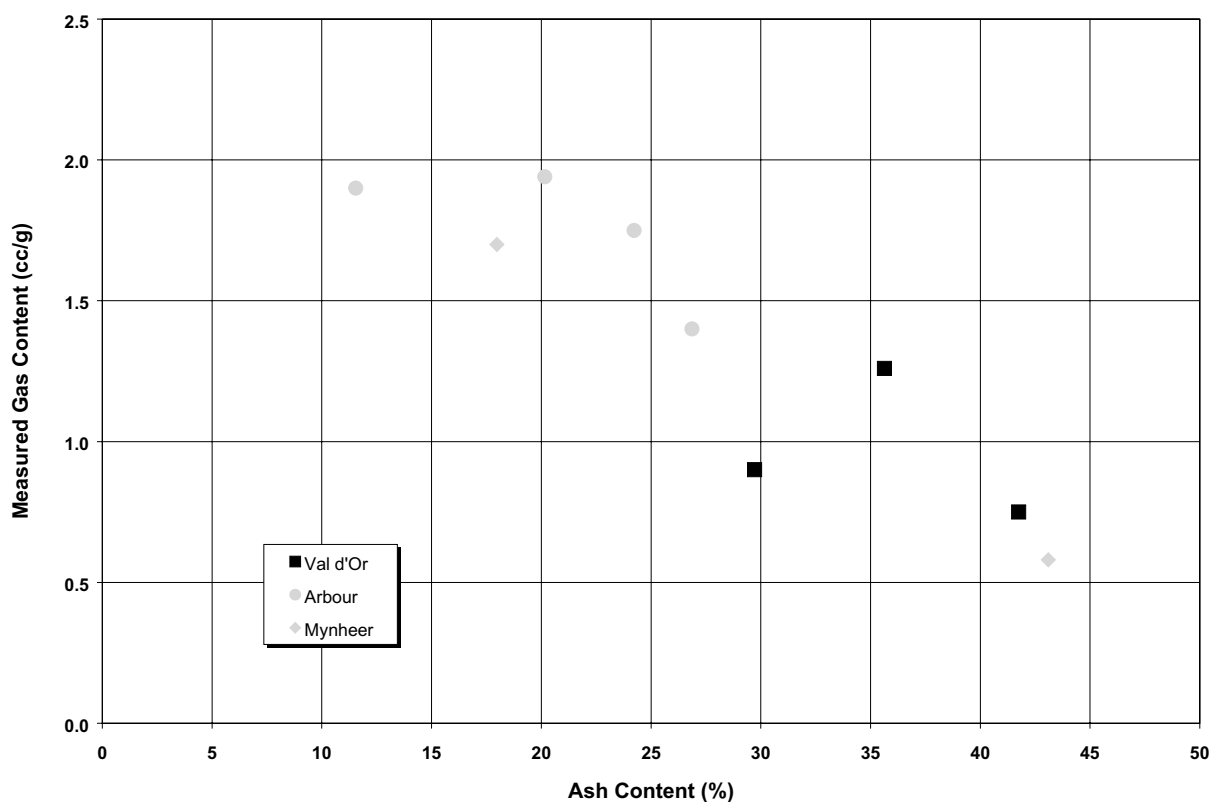
Figure 145. Measured gas content versus ash content (a.d.b.), BHP Embarras samples.
