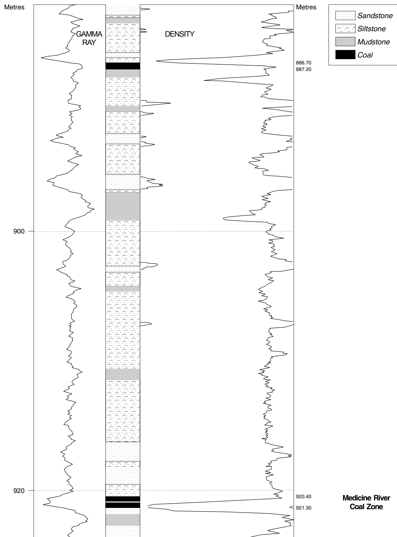
Figure 88. Detailed stratigraphic section of the AEC Jenner borehole.
