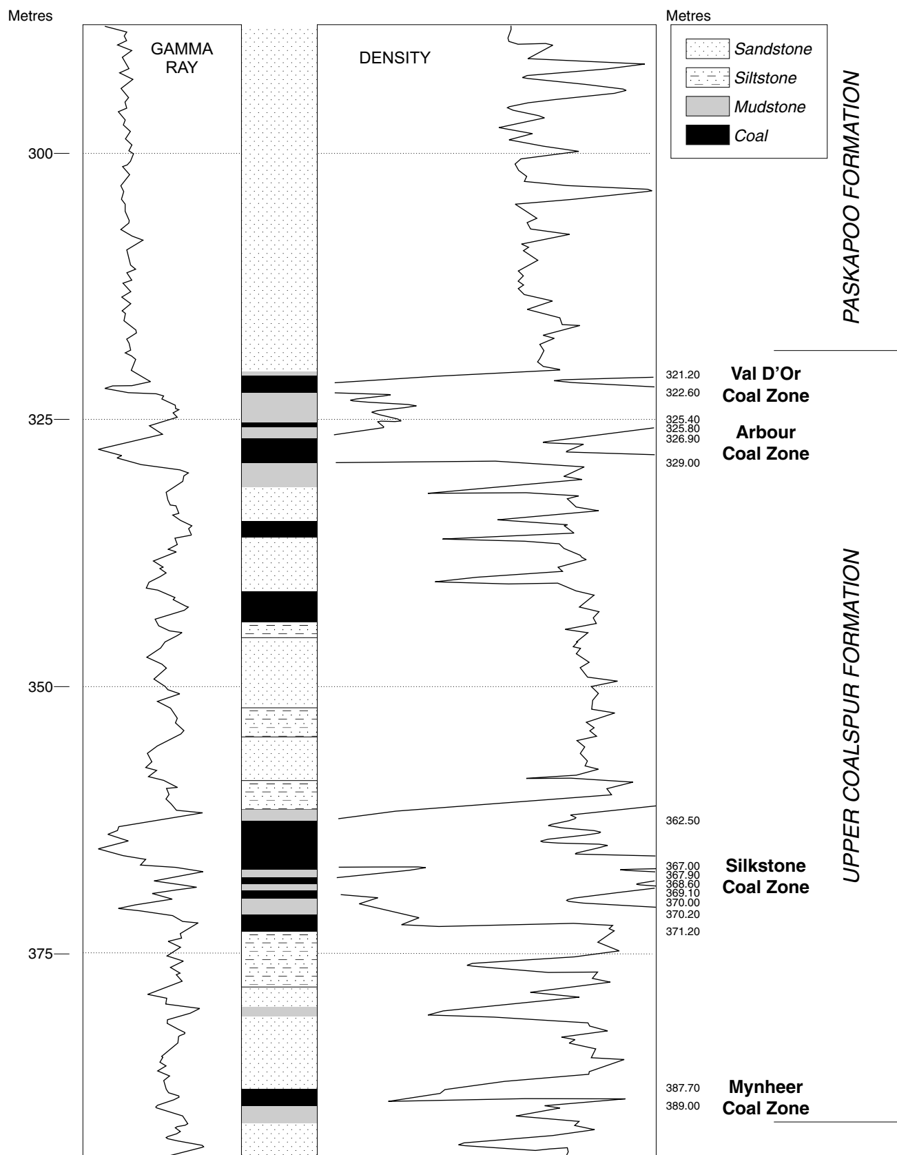
Figure 112. Detailed stratigraphic section of the Norcen Pembina 3-29 borehole.
