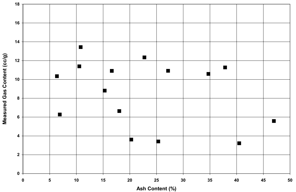
Figure 11. Measured gas content versus ash content for all coal samples, Gulf Fernie c-12-L.
