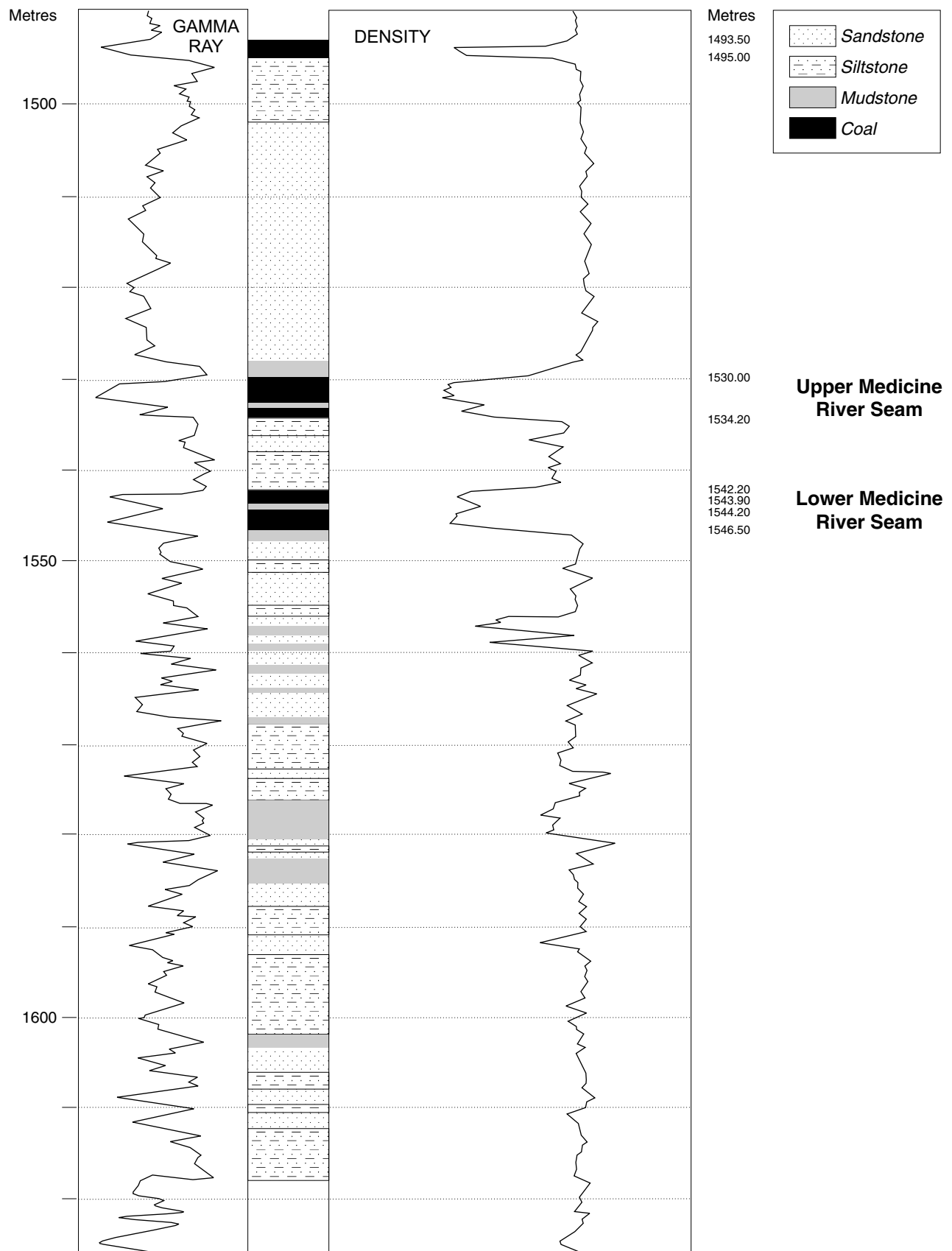
Figure 86. Detailed stratigraphic section of the Medicine River coal zone, Lionheart Attock borehole.
