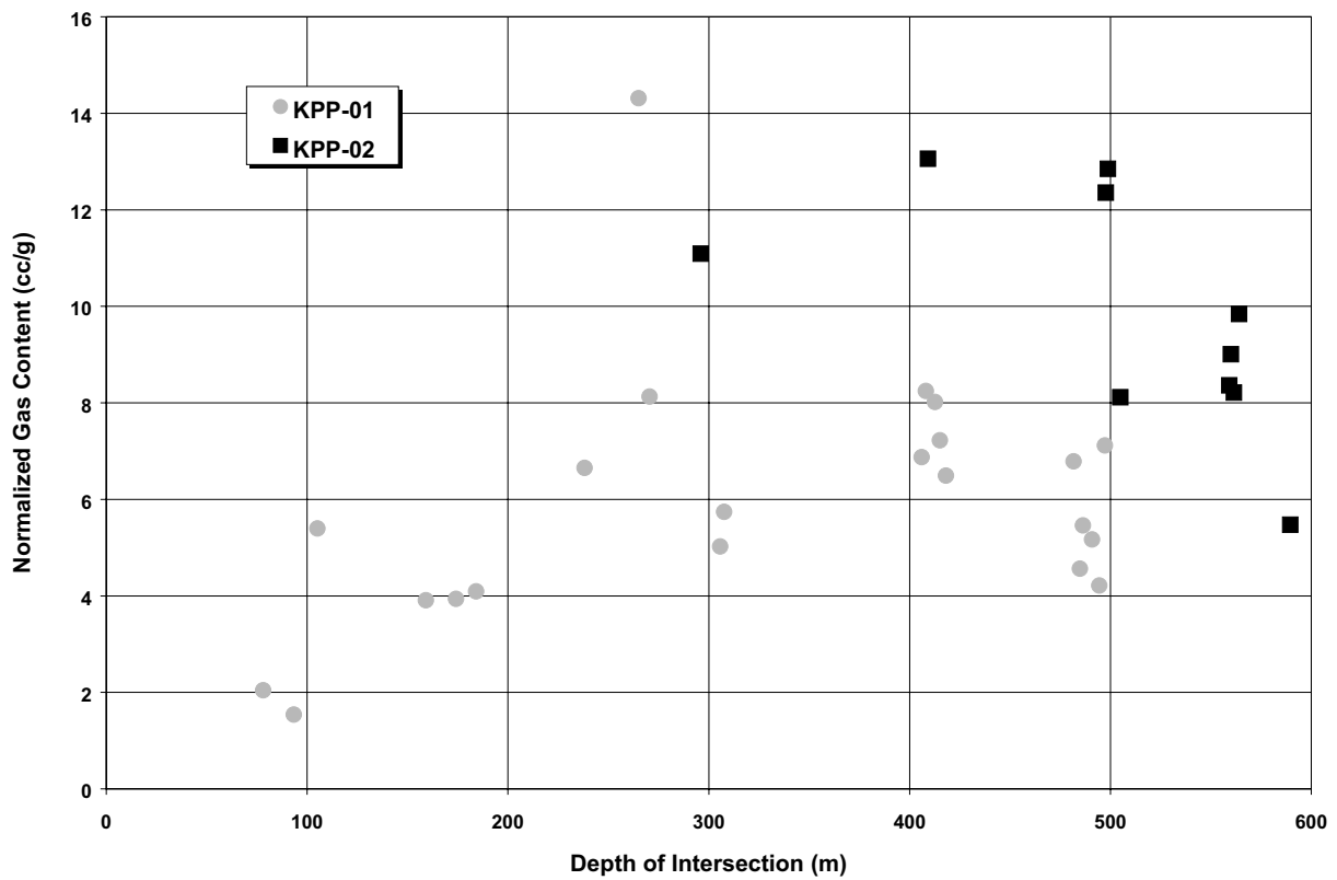
Figure 17. Normalized gas content versus depth of intersection, KPP90-1 and KPP90-2 canister samples.
