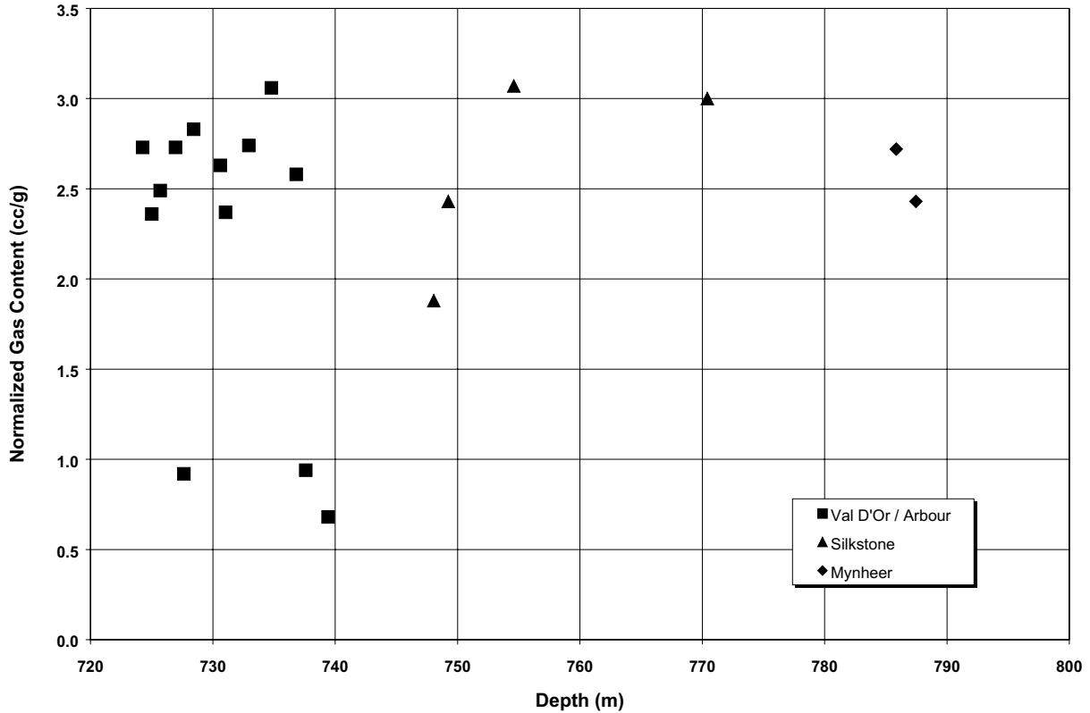
Figure 140. Normalized gas content versus depth of intersection, BHP Pine Creek samples.
