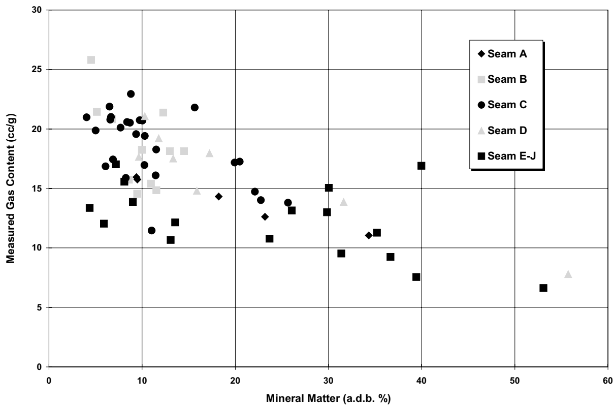
Figure 37. Measured gas content versus mineral matter by seam designation, Phillips Flatbed exploration area.
