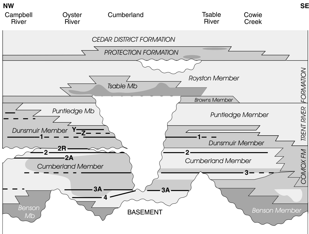
Figure 2. General stratigraphic column of coal-bearing strata in the Tsable River area.
