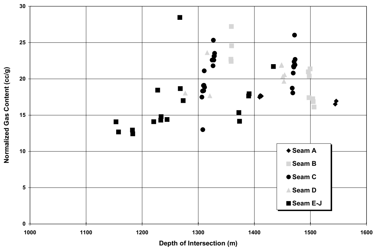
Figure 36. Normalized gas content (d.m.m.f. basis) versus depth of intersection by seam designation, Phillips Flatbed exploration area.
