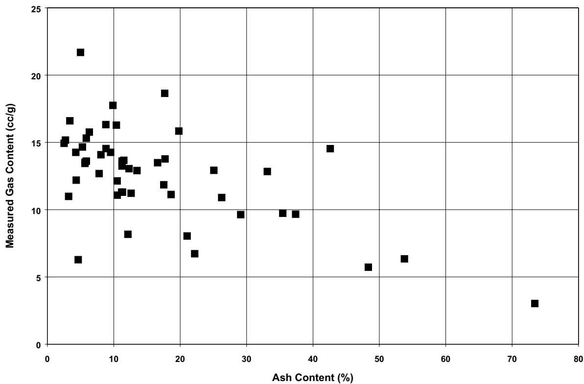
Figure 27. Measured gas content versus ash content for all Elk Valley samples.
