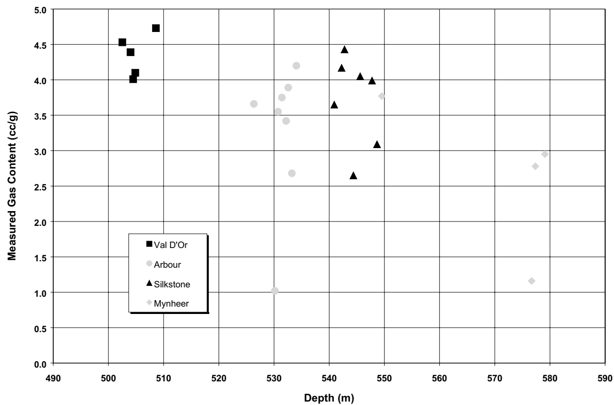
Figure 130. Measured gas content versus depth, BHP Pembina samples.
