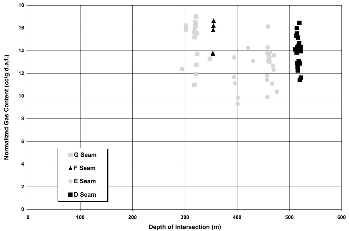
Figure 22. Normalized gas content versus depth of intersection, Fording coal samples.
