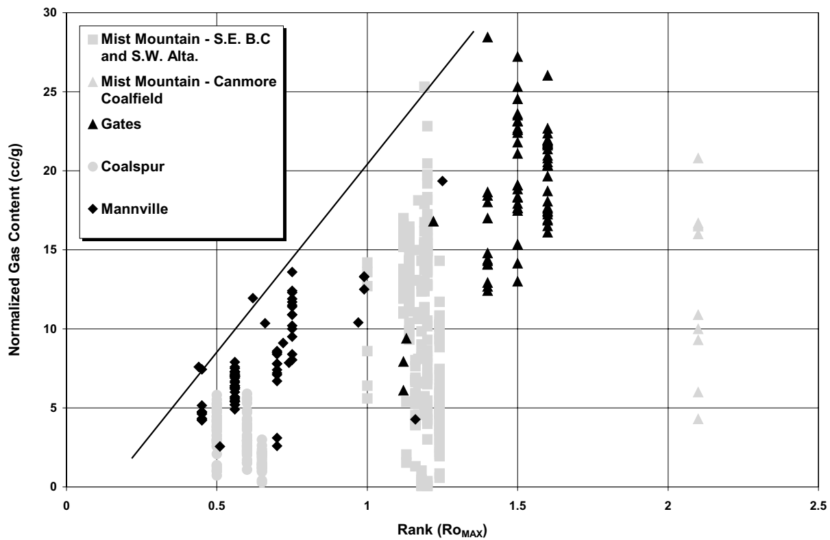
Figure 153. Comparison of normalized gas content versus Ro_{MAX} for all coalbed methane data collected in Western Canada.
