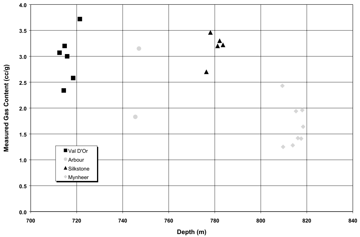
Figure 135. Measured gas content versus depth of intersection, BHP Peco samples.
