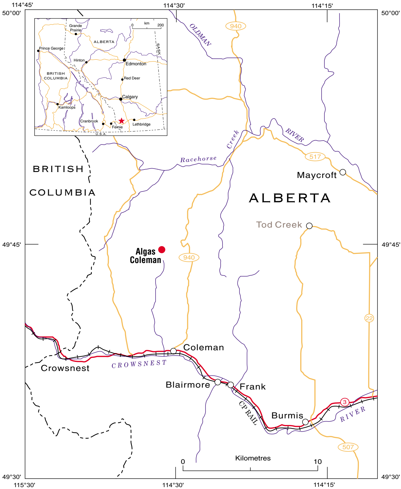
Figure 50. General location map of the Algas Resources Coleman (08-19-09-04W5M) exploration borehole.
