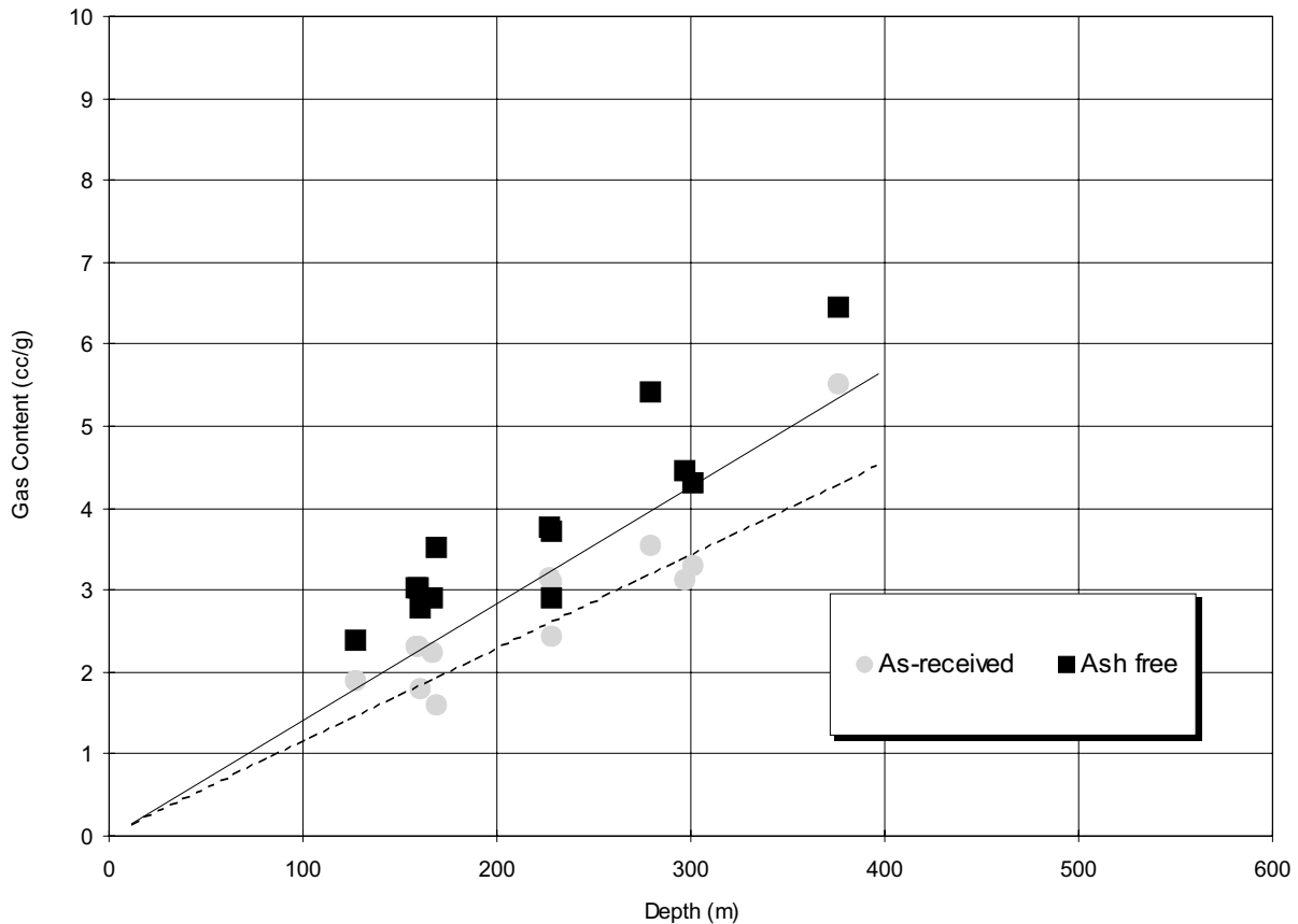
Figure 3. As-received and normalized gas content versus depth, Tsable River area.
