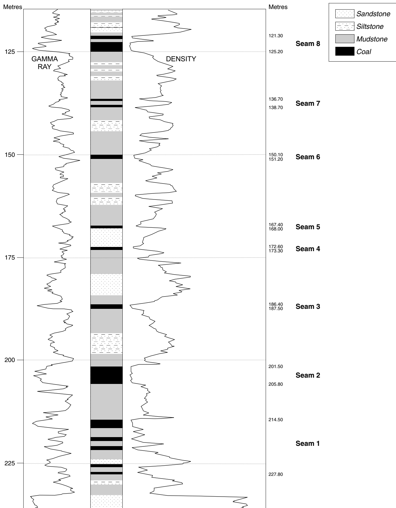
Figure 53. Detailed stratigraphic section of the Mist Mountain Formation for the Sullivan Creek borehole.
