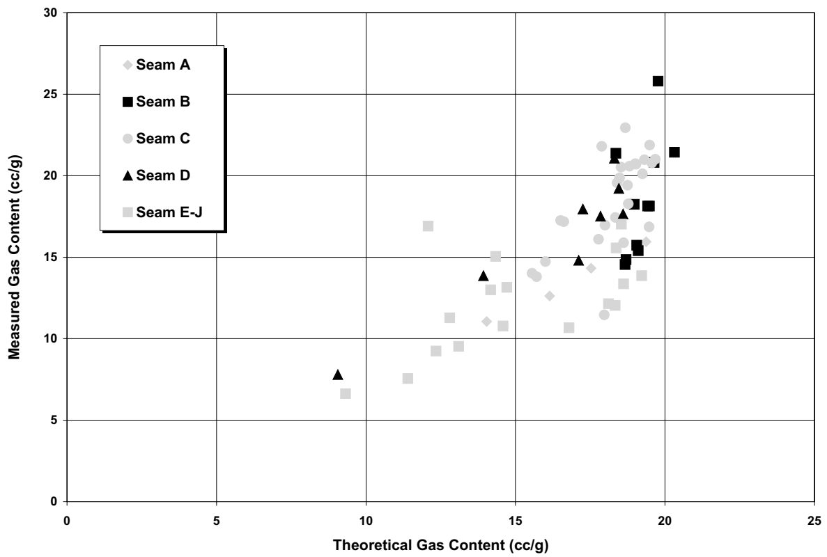
Figure 38. Measured gas content versus theoretical gas content by seam designation, Phillips Flatbed exploration area.
