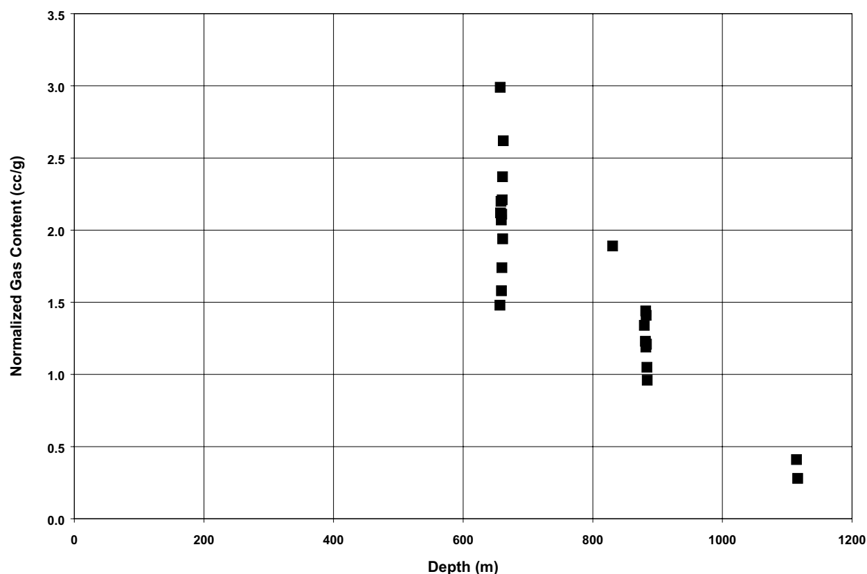
Figure 64. Normalized gas content versus depth for desorption samples collected from the Conoco Hanlan well.
