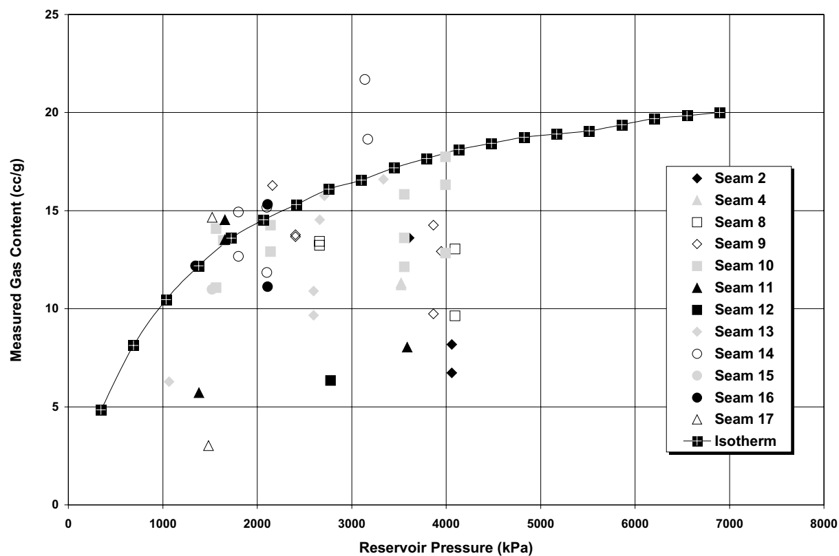
Figure 28. Comparison of measured gas content to adsorption isotherm values of Elk Valley samples.
