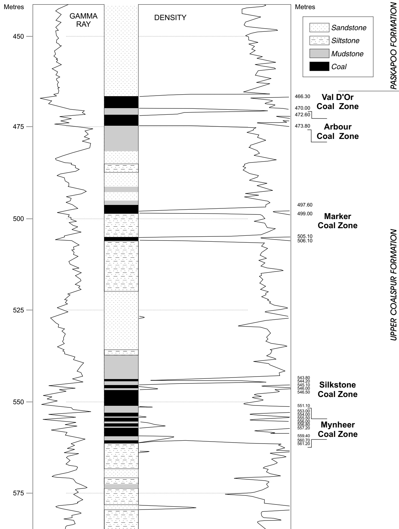
Figure 126. Detailed stratigraphic section of the Coalspur Formation coal measures intersected in the Wascana Brazeau borehole.
