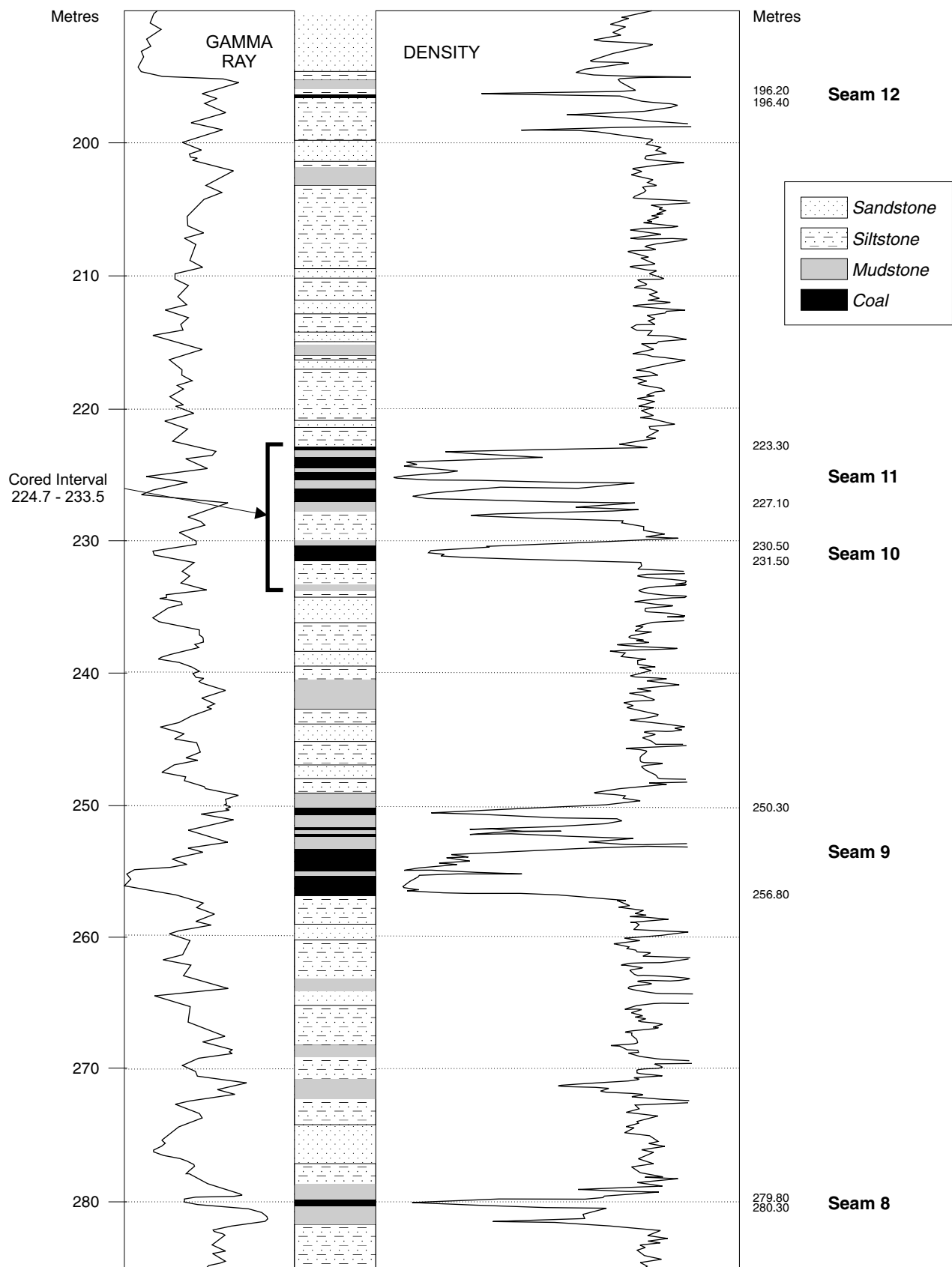
Figure 68. Detailed stratigraphic section of the coal seam intersections for the Smoky River Coal exploration borehole.
