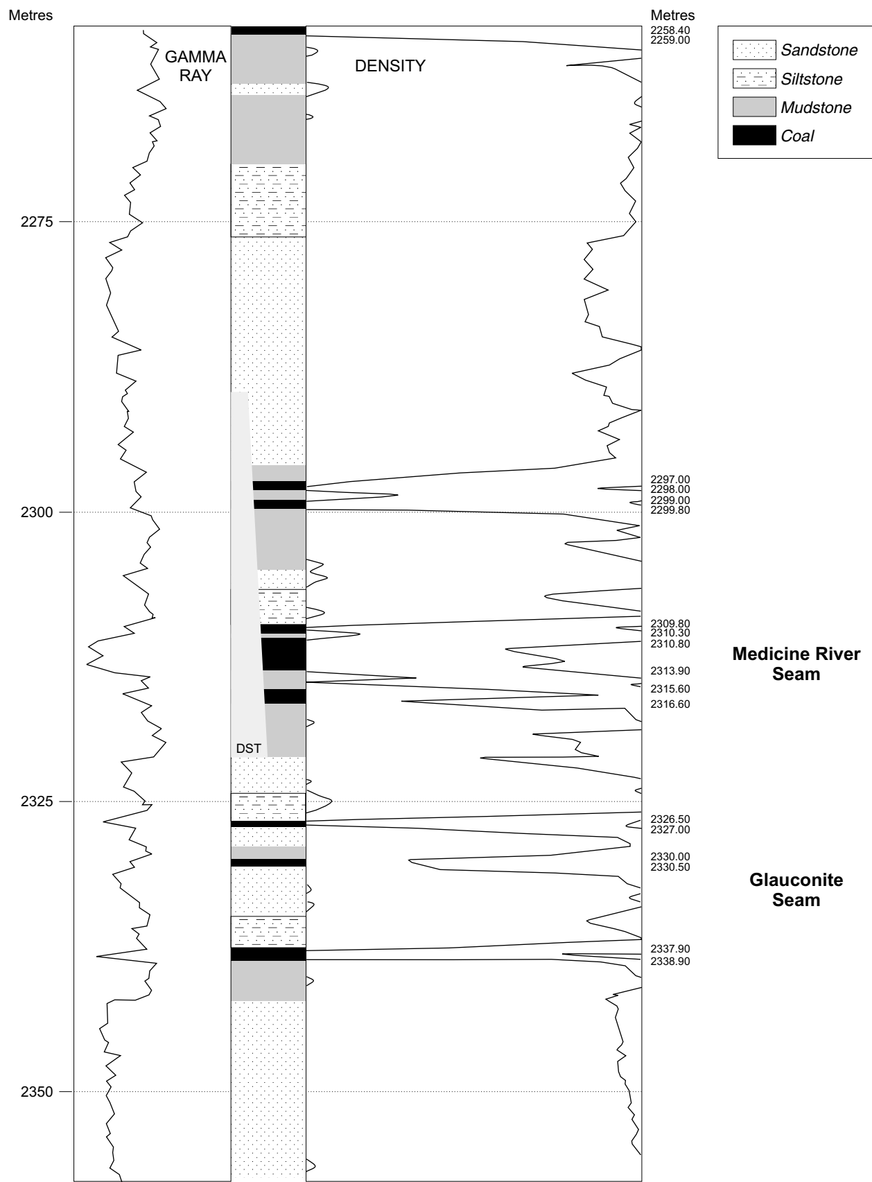
Figure 127. Detailed stratigraphic section of the Mannville Group coal measures intersected in the Wascana Brazeau borehole.
