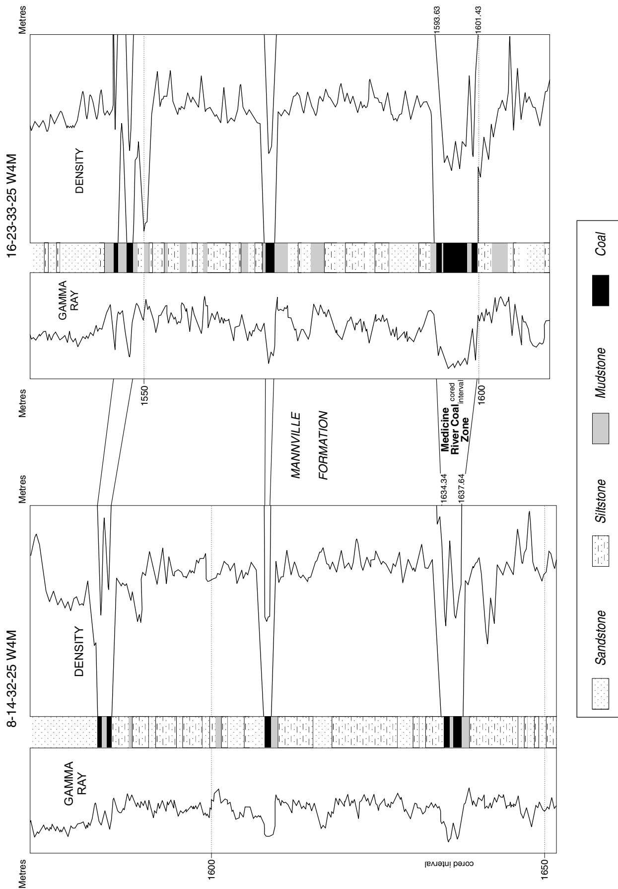
Figure 83. Detailed stratigraphic sections of the coal measures, Enron Twining 8-14 and 16-23 boreholes.
