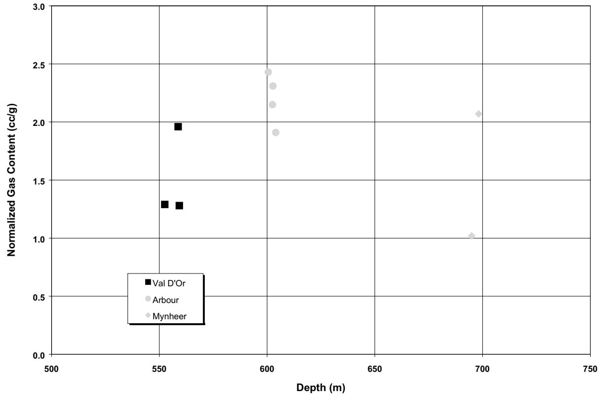
Figure 144. Normalized gas content versus depth of intersection, BHP Embarras samples.
