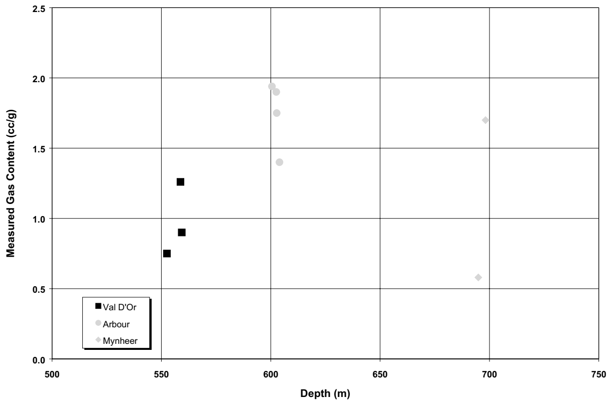
Figure 143. Measured gas content versus depth of intersection, BHP Embarras samples.
