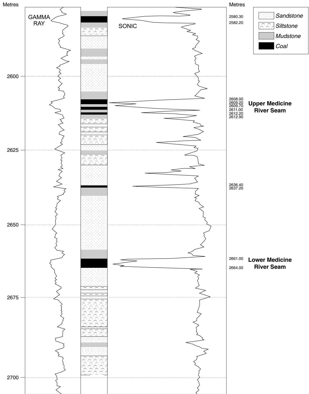
Figure 115. Detailed stratigraphic section of the Norcen Colt borehole.
