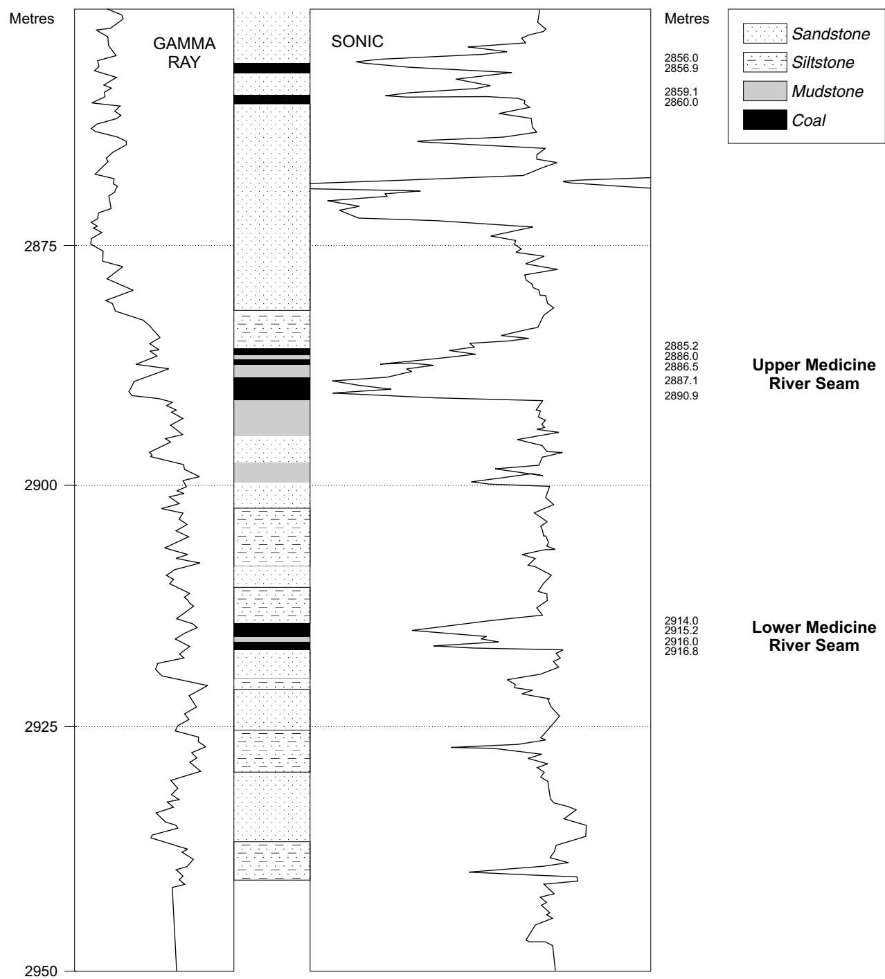
Figure 119. Detailed stratigraphic section of the lower Norcen Seaforth borehole.
