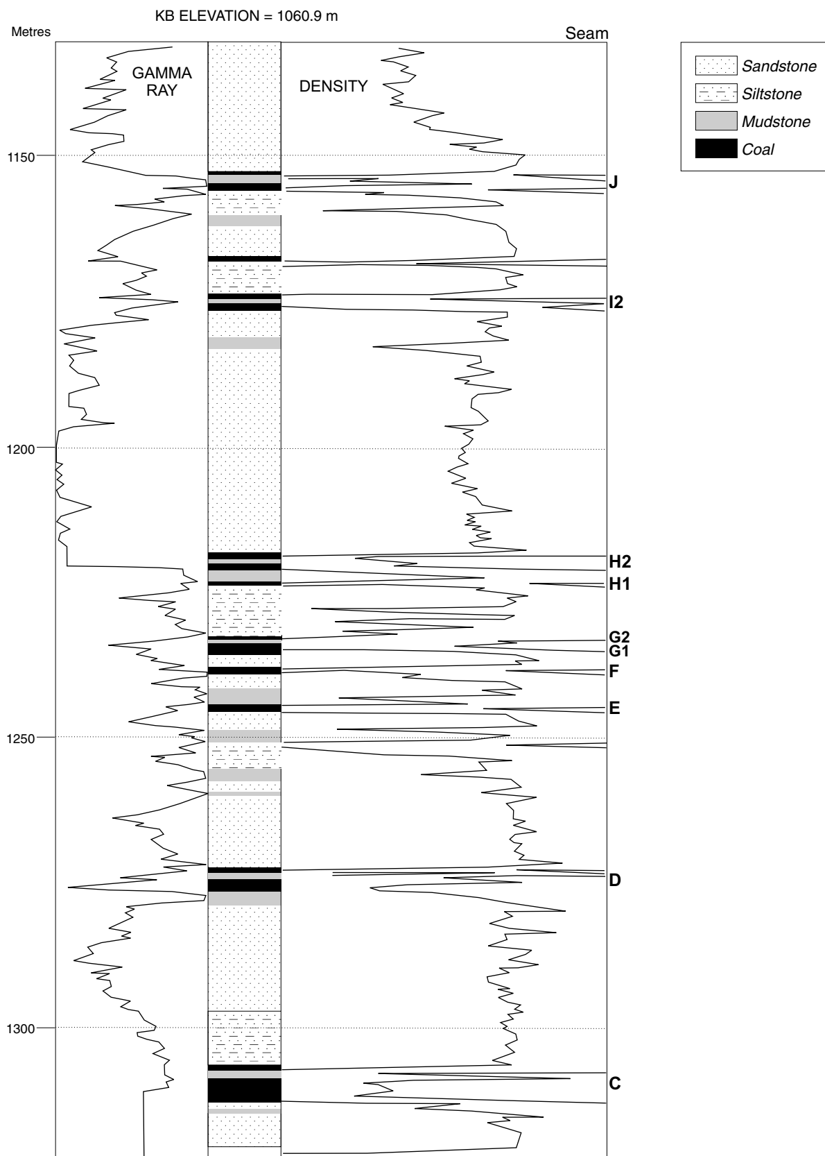
Figure 32. Detailed stratigraphic section of the Phillips d-93-B/93-I-15 borehole.
