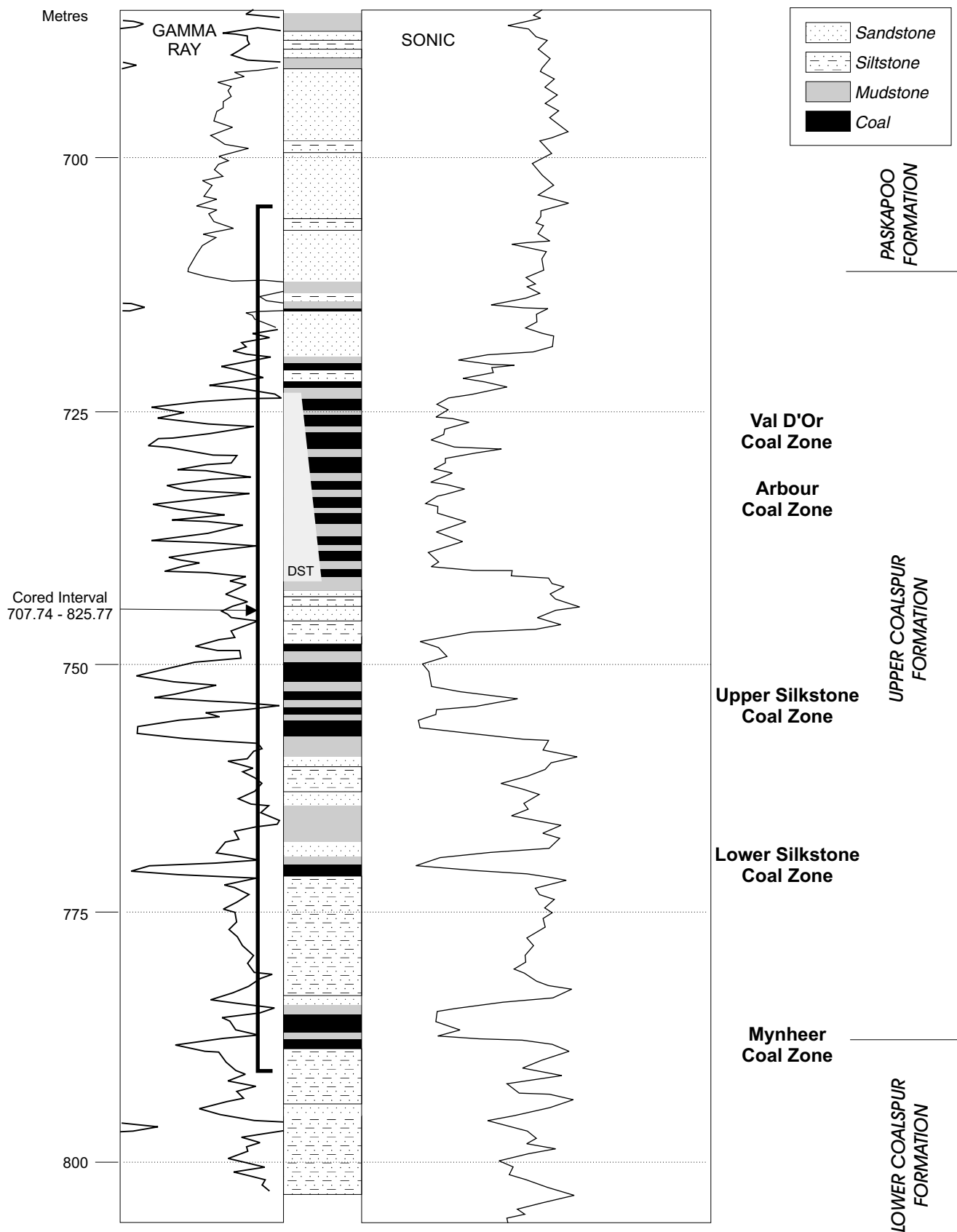
Figure 138. Detailed stratigraphic section illustrating the four major coal zones intersected in the BHP Pine Creek borehole.
