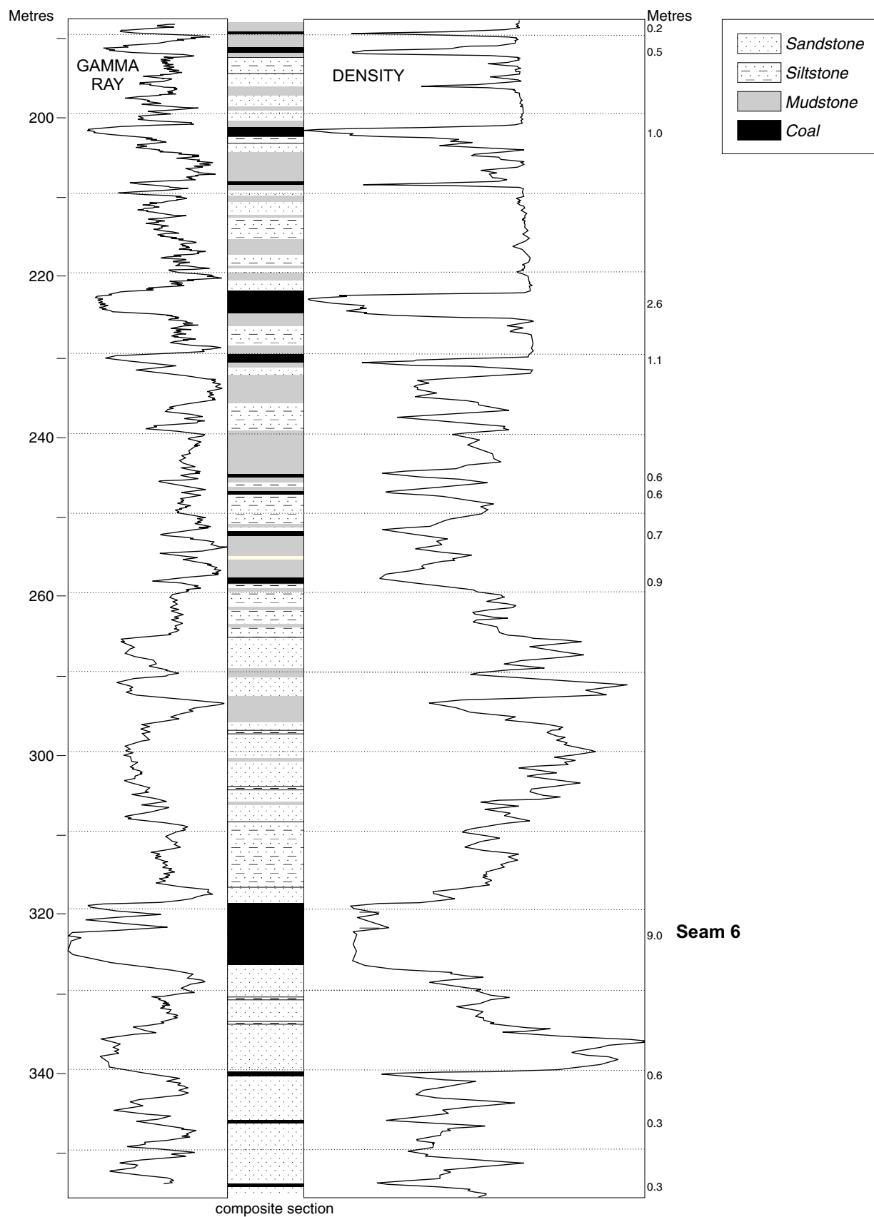
Figure 57. Detailed composite stratigraphic section of the Mist Mountain Formation coal measures encountered in the Canmore region.
