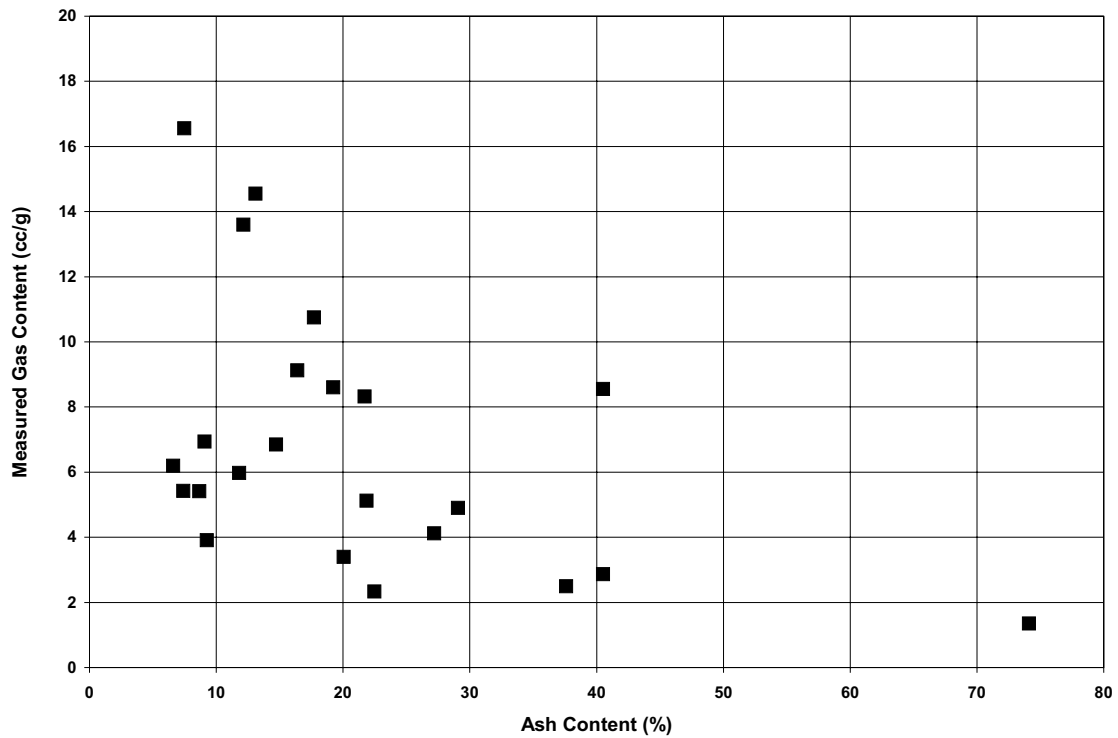
Figure 7. Gas content (as measured) versus ash content for all coal samples, wellbore a-65-E.
