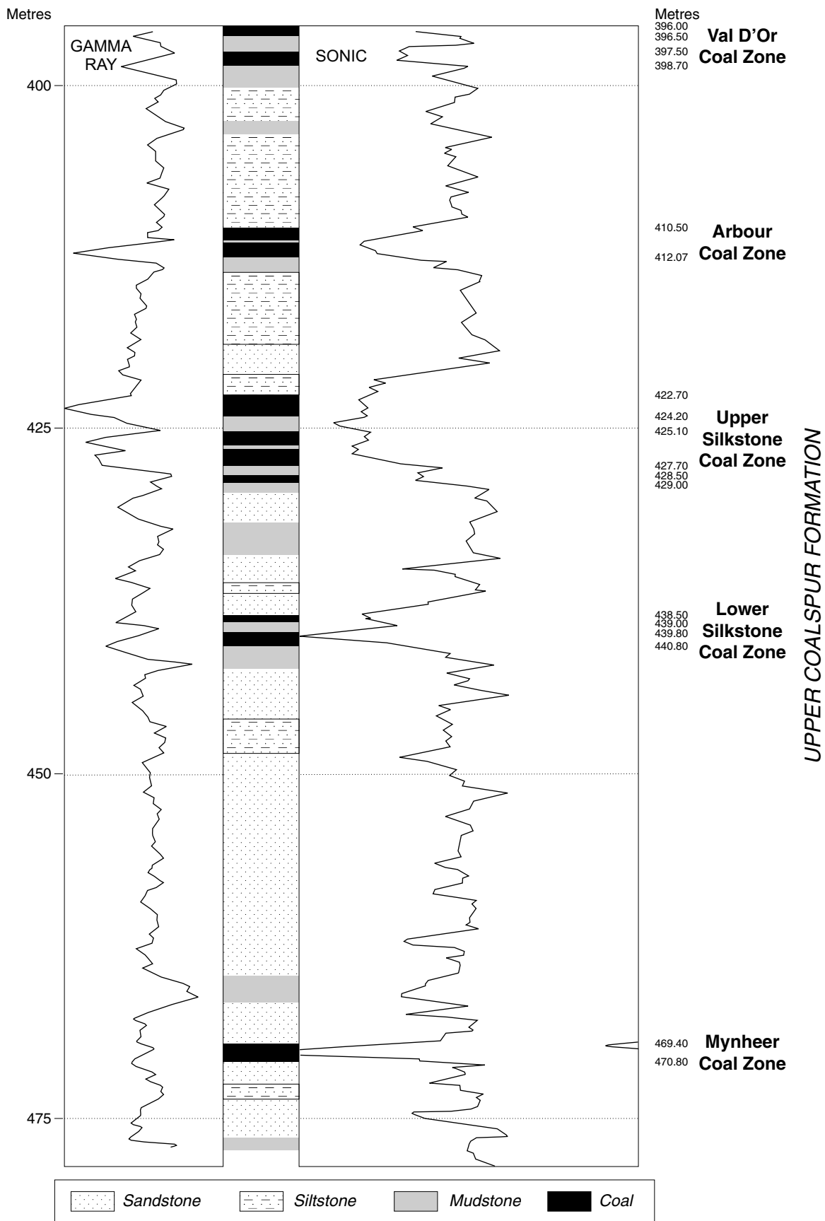
Figure 91. Detailed stratigraphic section of the Scollard Formation, Gulf Sylvan Lake borehole.
