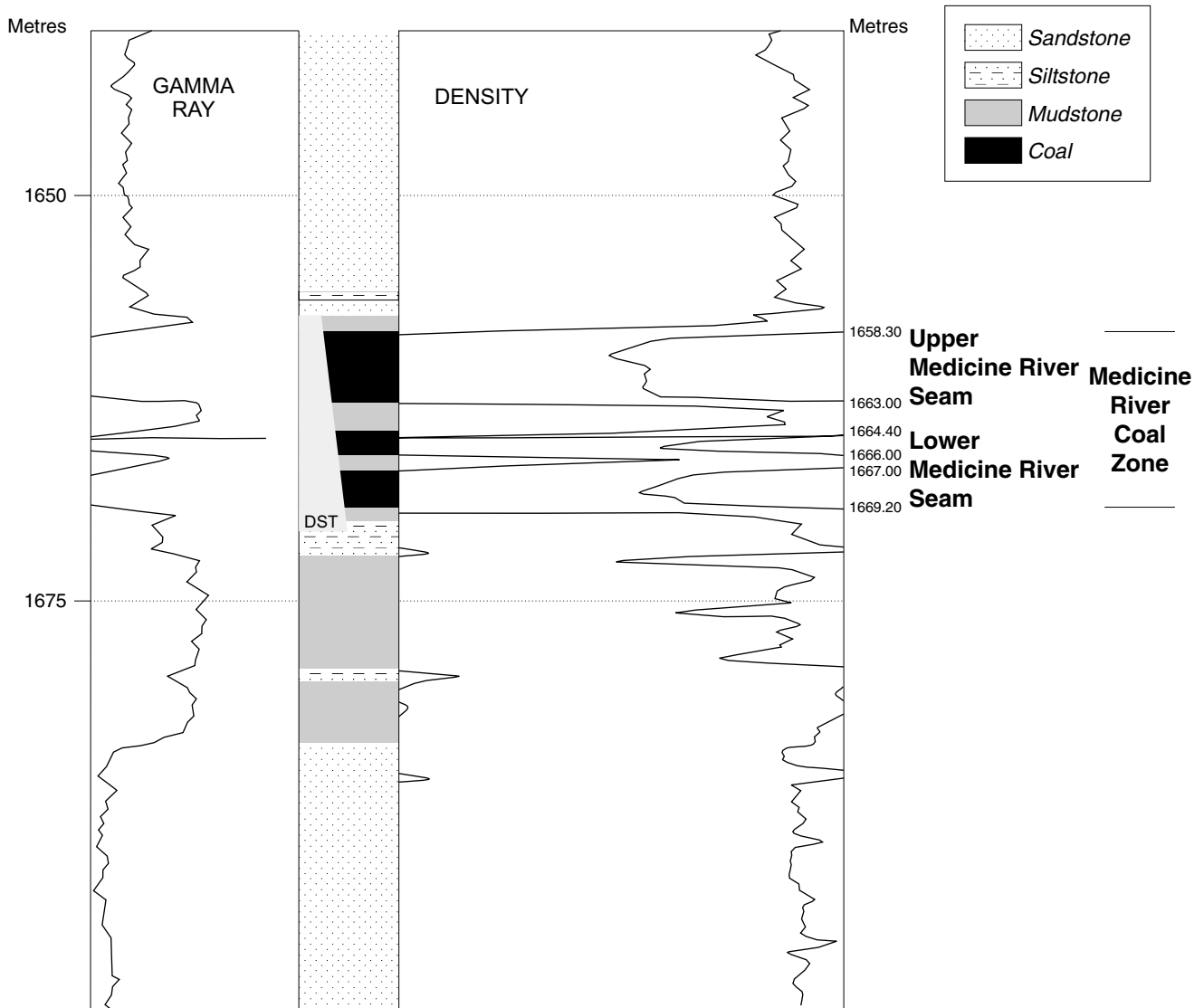
Figure 77. Detailed stratigraphic section of the Medicine River coal zone, PanCanadian Westerosé East borehole.
