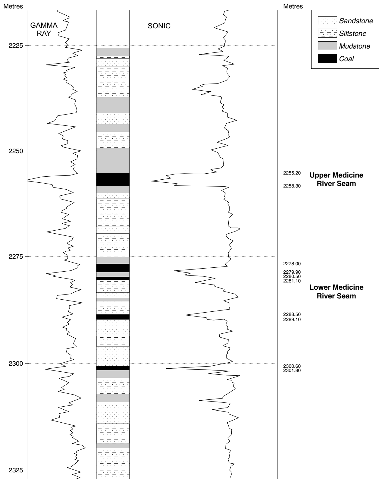
Figure 114. Detailed stratigraphic section of the Norcen Por Fir borehole.
