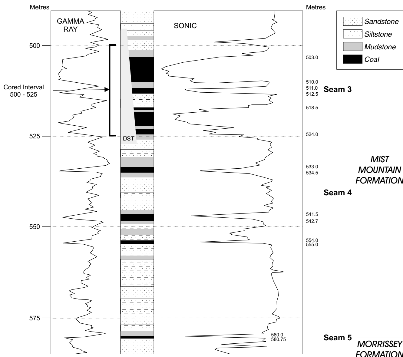
Figure 43. Detailed stratigraphic section of coal intersections for the Canadian Hunter No. 1 borehole.
