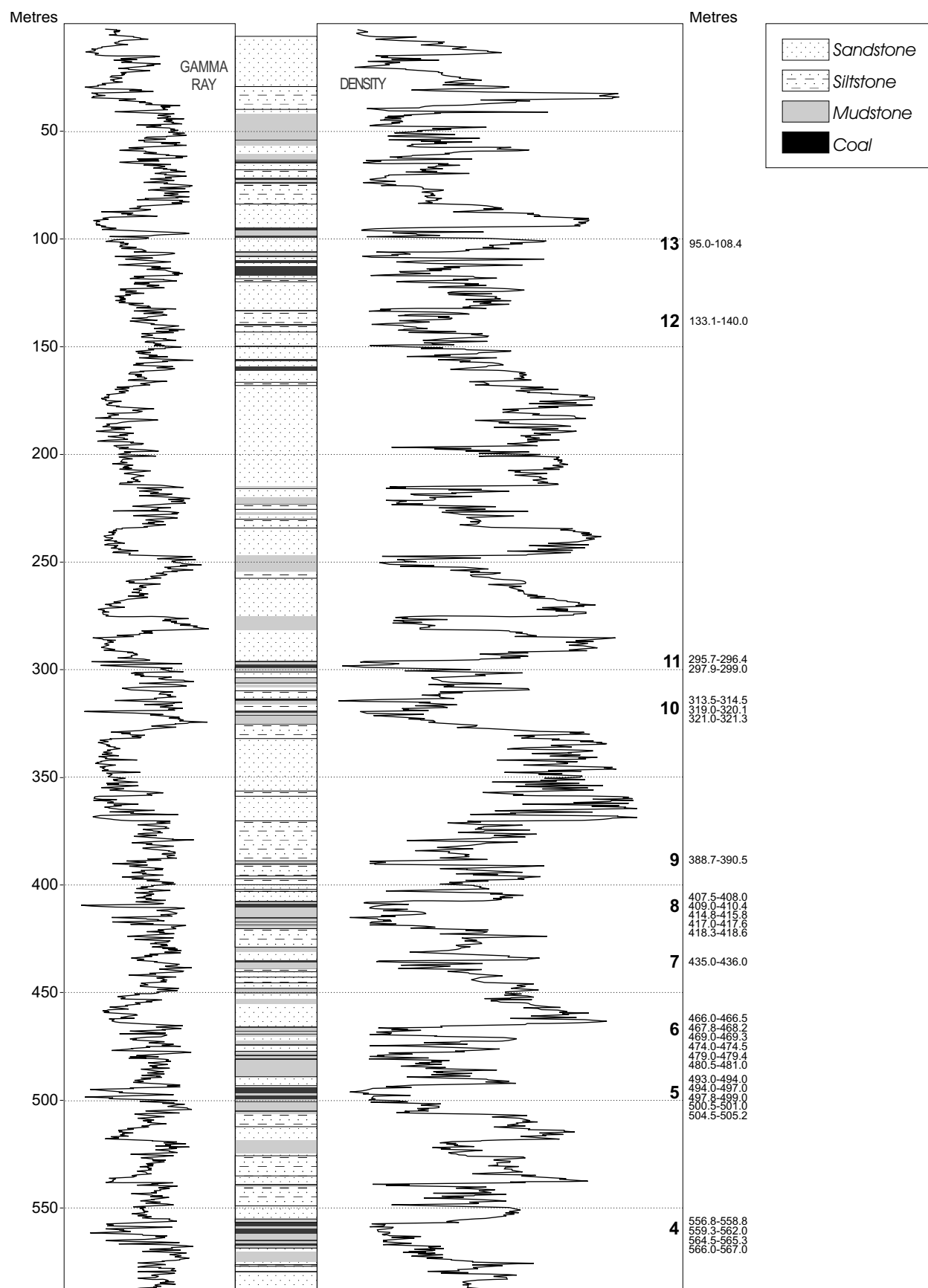
Figure 14. Detailed stratigraphic section of the KPP90-2 borehole.
