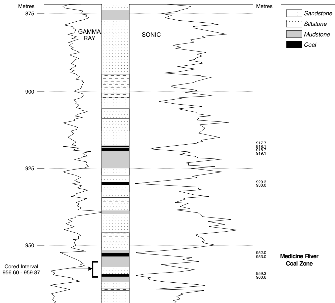
Figure 89. Detailed stratigraphic section of the AEC Suffield 13-01 borehole.
