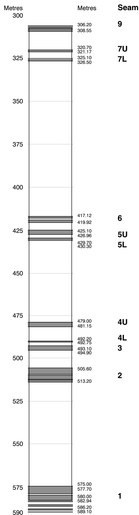
Figure 9. Stratigraphic section of the Gulf Lornel c-12-L borehole.
