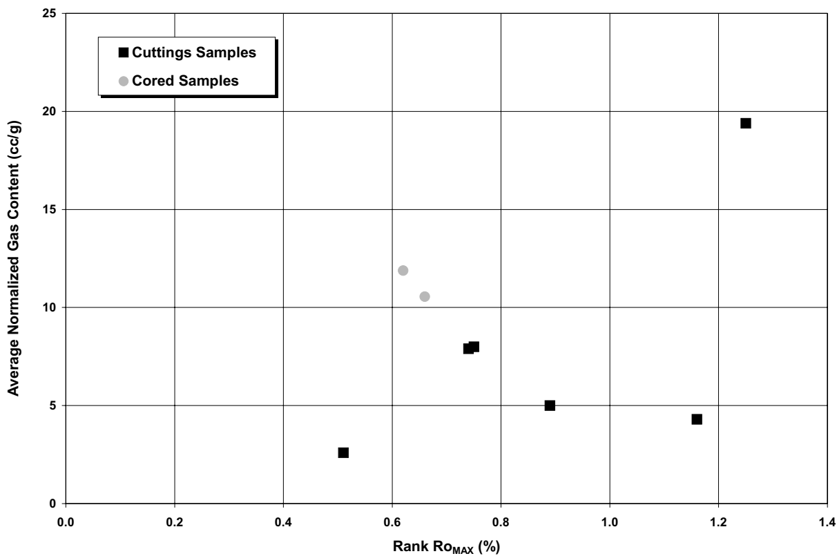
Figure 124. Normalized gas content versus rank for Mannville coal intersections.
