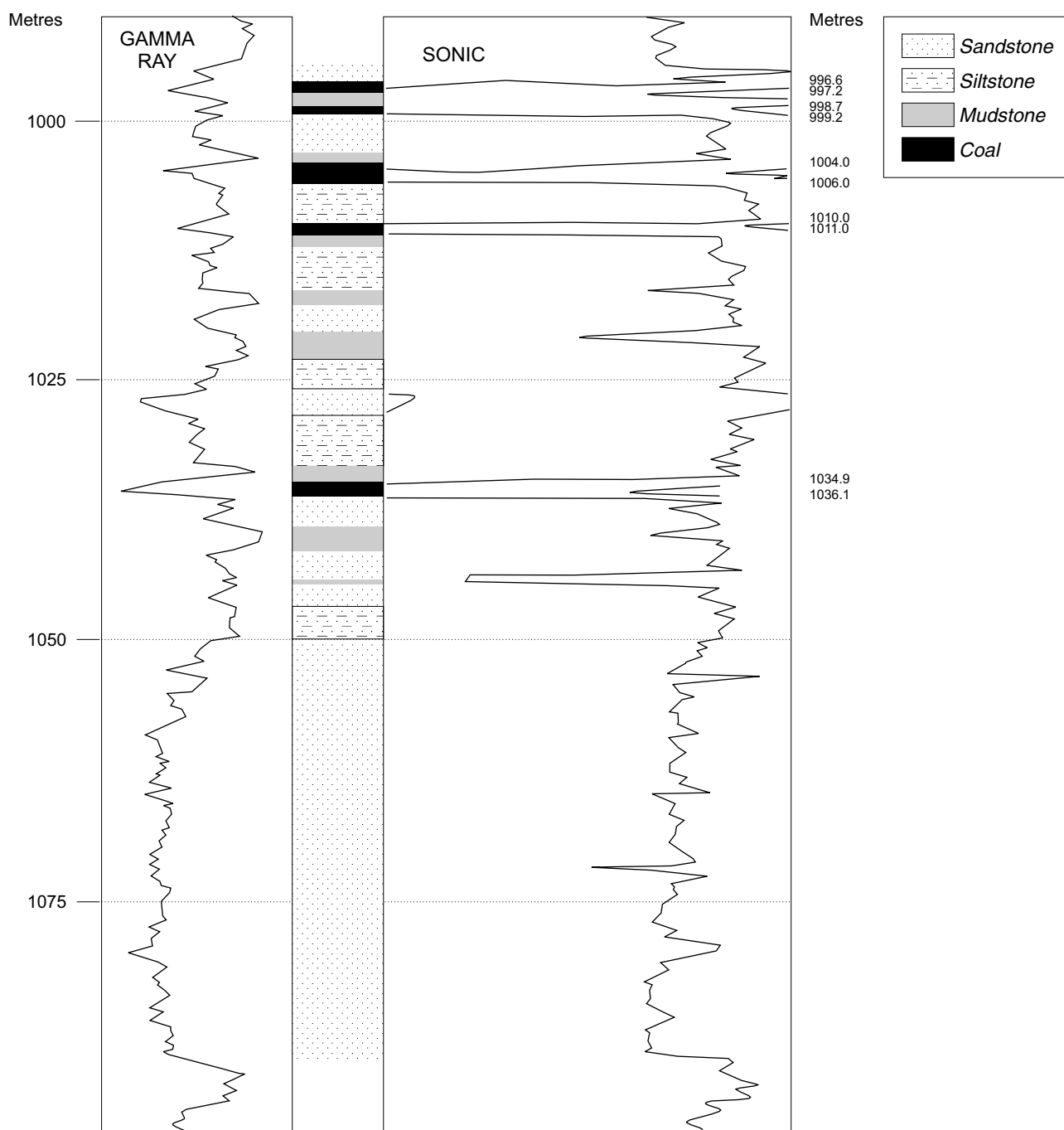
Figure 120. Detailed stratigraphic section of the Norwest Majeau borehole.
