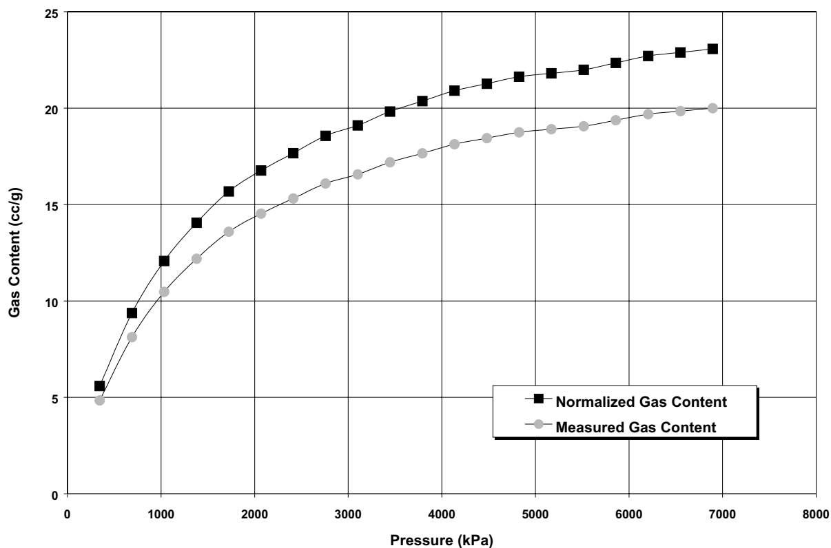
Figure 29. Adsorption isotherm for Seam 10, Elk Valley, illustrating measured and normalized gas curves. Adsorption temperature is 20°C.
