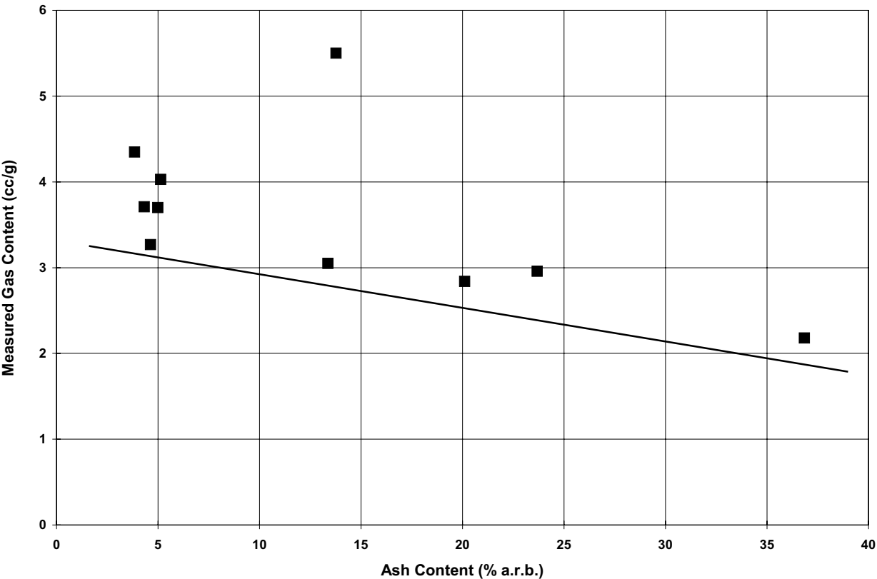
Figure 98. Measured gas content versus ash content for the Redwater desorption samples.
