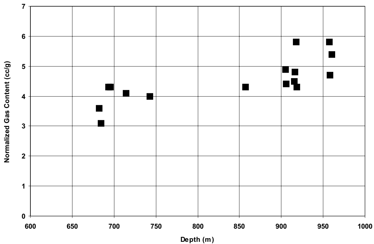
Figure 102. Normalized gas content versus depth of intersection, Amoco plains boreholes.
