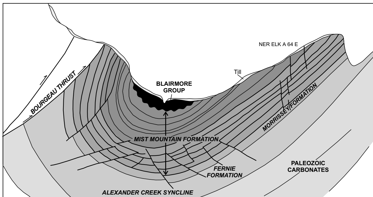
Figure 30. Schematic diagram of Alexander Creek Syncline illustrating regions of possible permeability enhancement.
