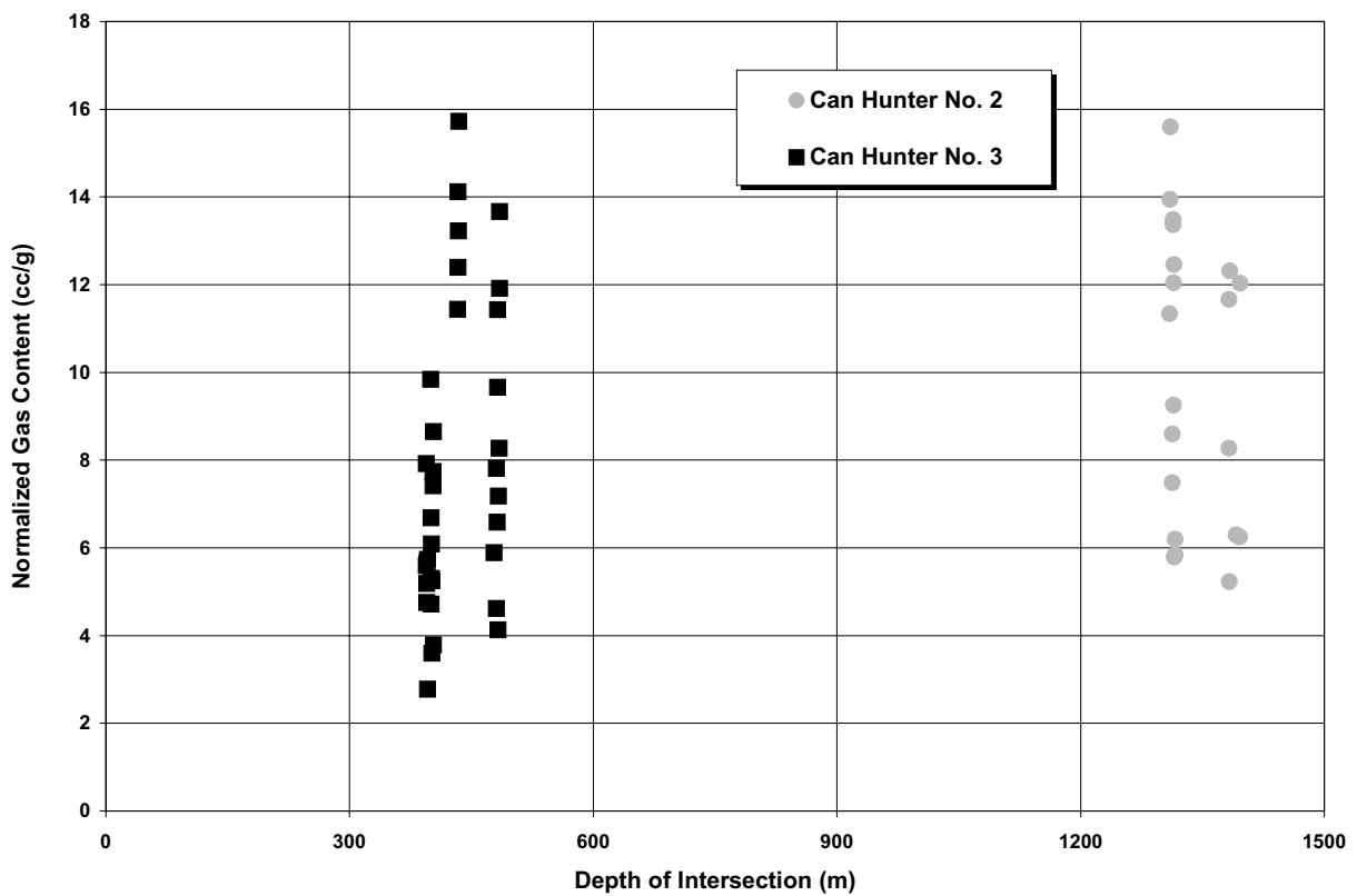
Figure 47. Normalized gas content versus depth of intersection, Canadian Hunter Nos. 2 and 3.
