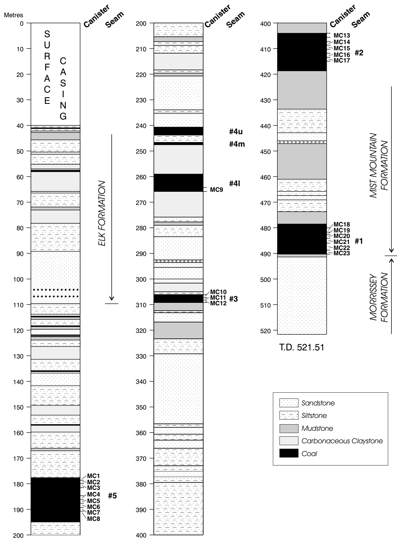
Figure 5. Stratigraphic section of the Mist Mountain Formation intersected in the a-65-E borehole.
