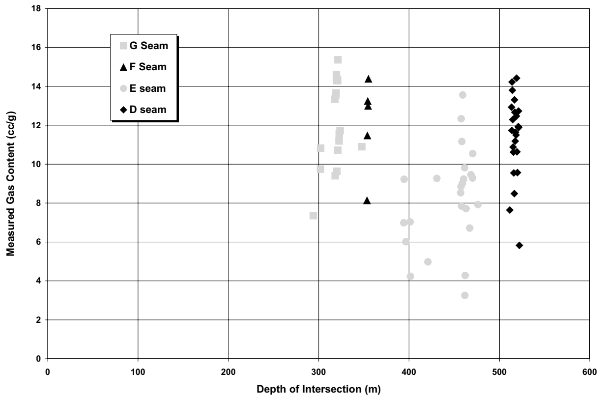
Figure 21. Gas content (as measured) versus depth of intersection, Fording coal samples.
