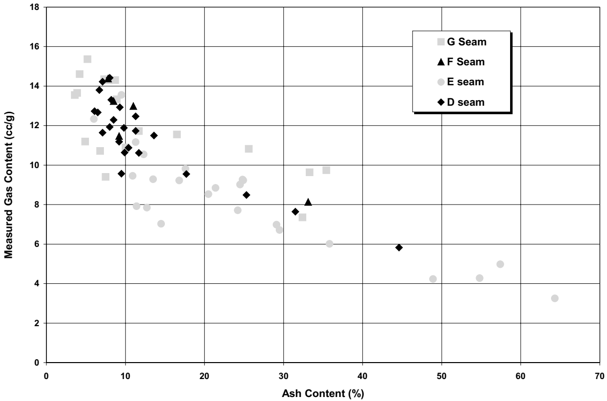
Figure 23. Gas content (as measured) versus ash content, Fording coal samples.
