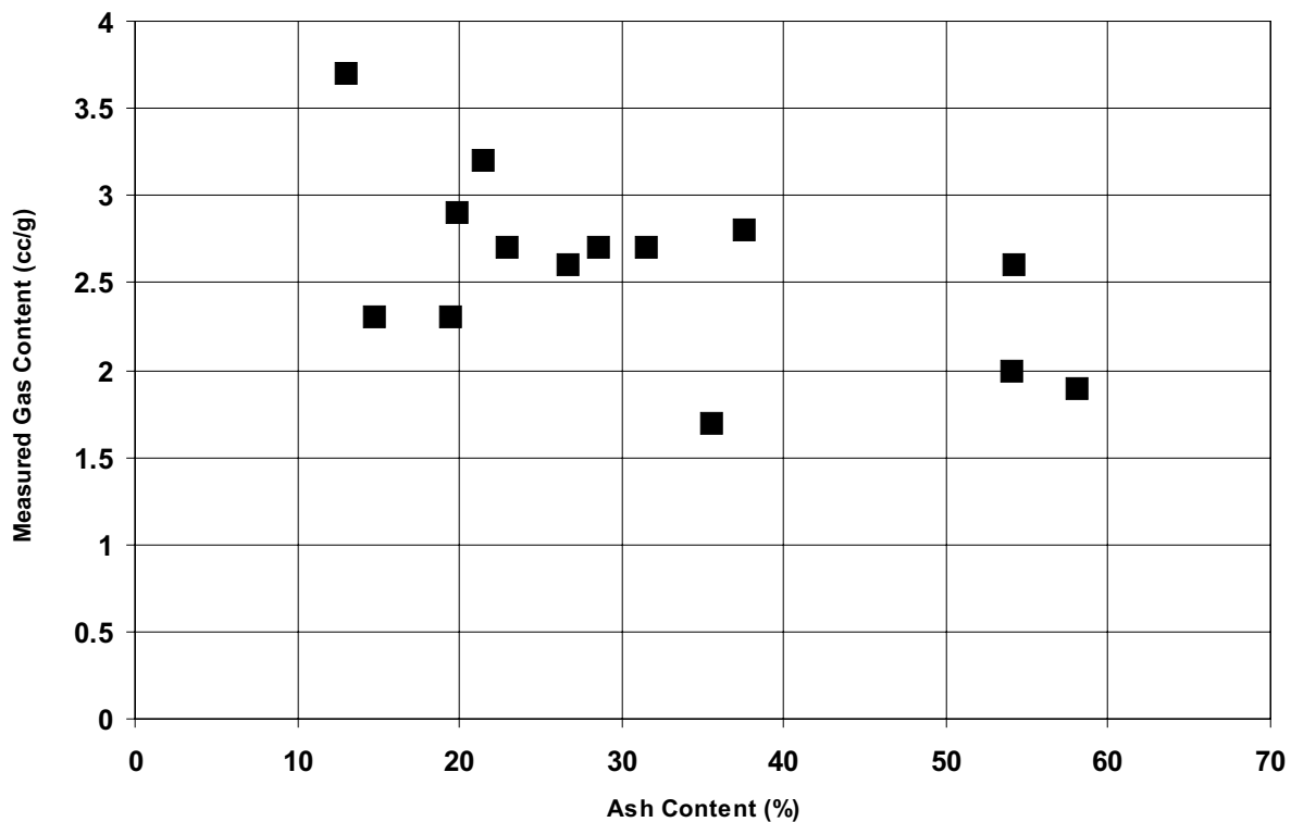
Figure 103. Measured gas content versus ash content, Amoco plains boreholes.
