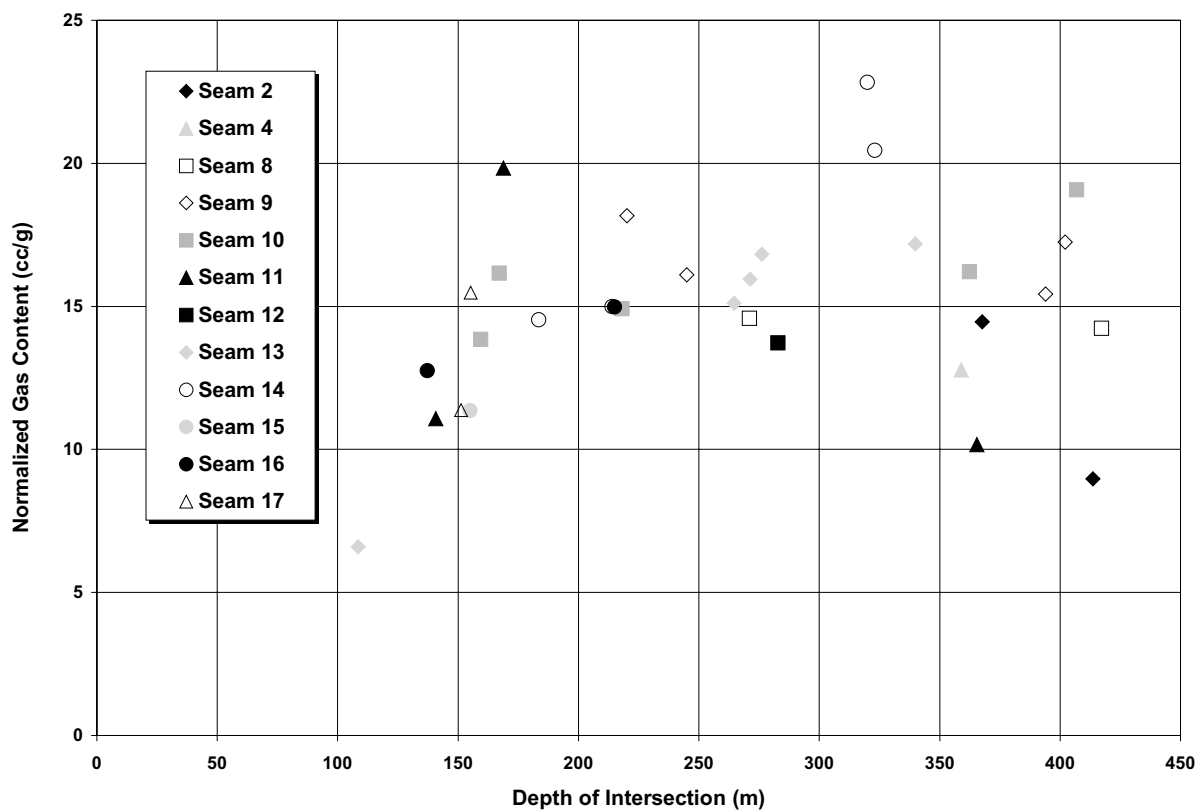
Figure 26. Normalized gas content versus depth of intersection, Elk Valley coal samples.
