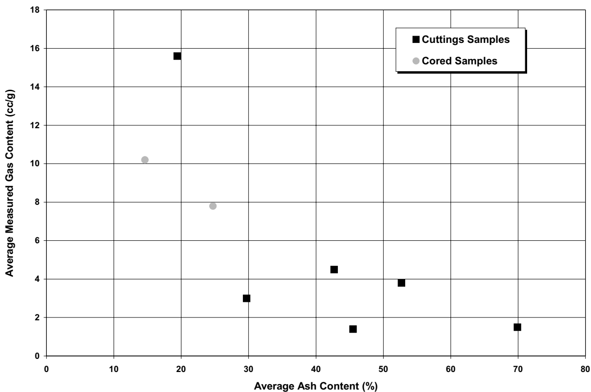
Figure 123. Measured gas content versus ash content for the Mannville coal intersections.
