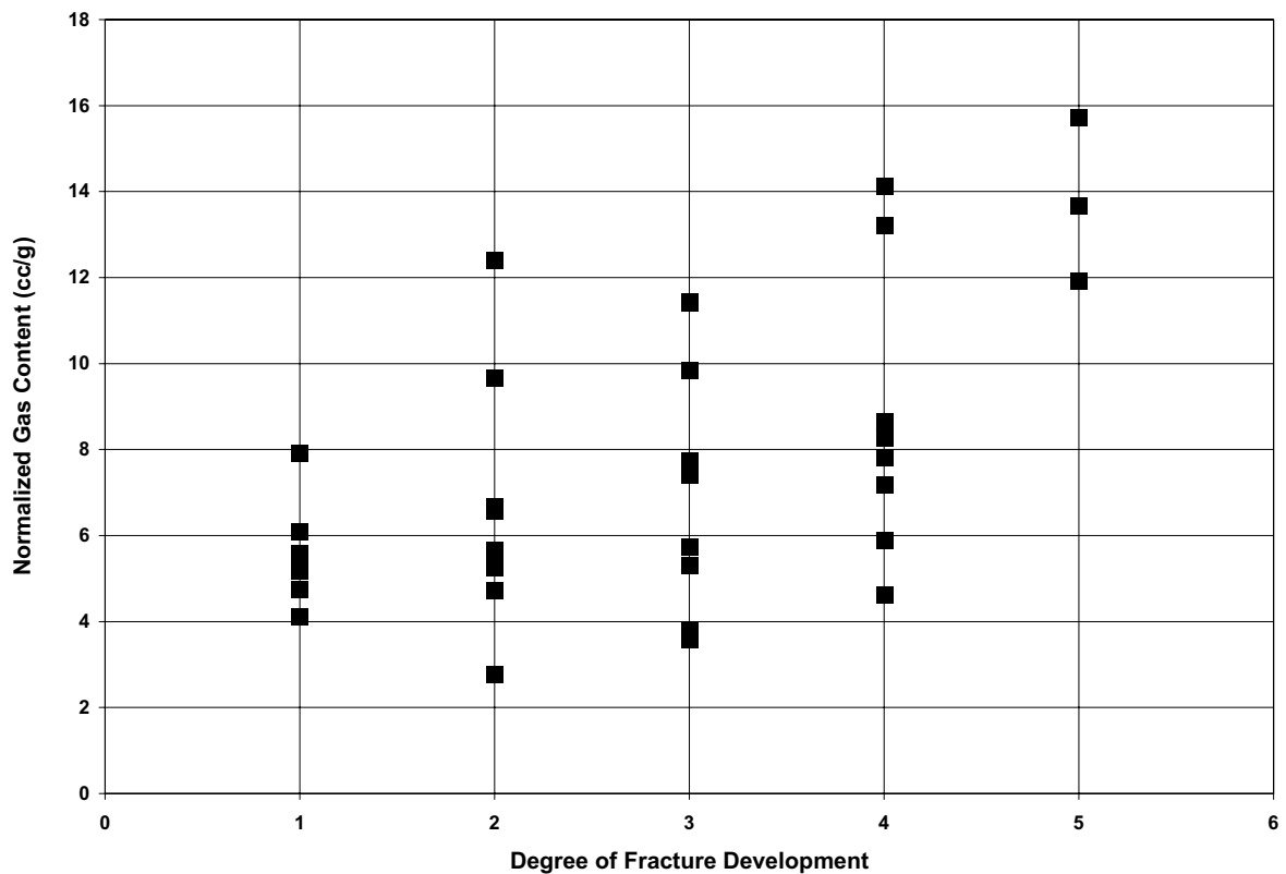
Figure 49. As measured gas content versus degree of fracture development. A large fracture number corresponds to well cleated coals with open fractures. A small number corresponds to coals that are either poorly cleated or the cleats of which are infilled with mineralization.
