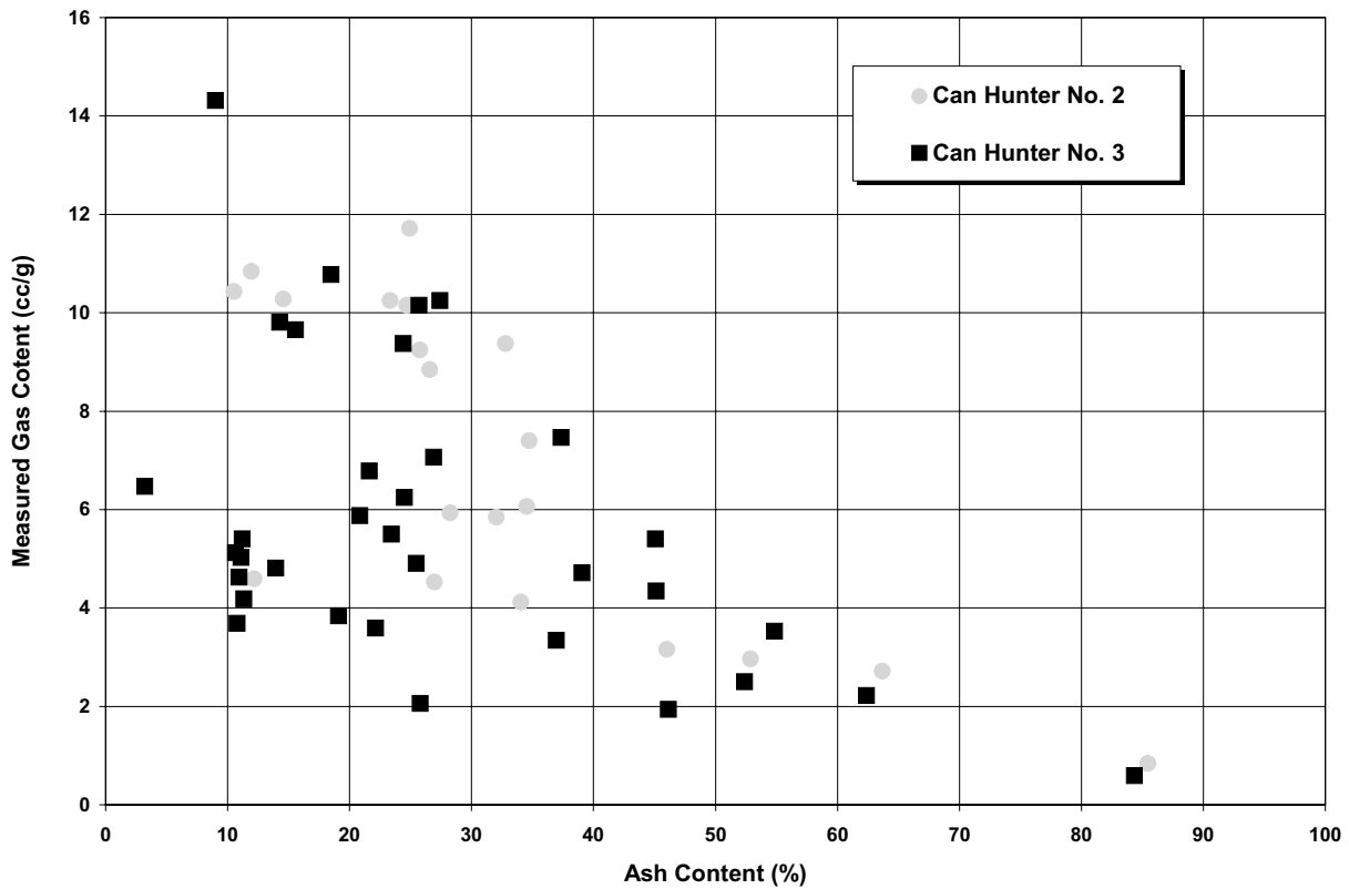
Figure 48. As measured gas content versus ash content for Canadian Hunter Nos. 2 and 3.
