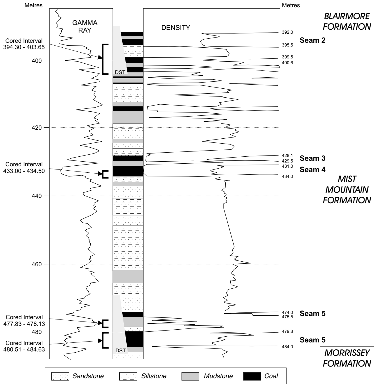
Figure 45. Detailed stratigraphic section of coal intersections for the Canadian Hunter No. 3 borehole.
