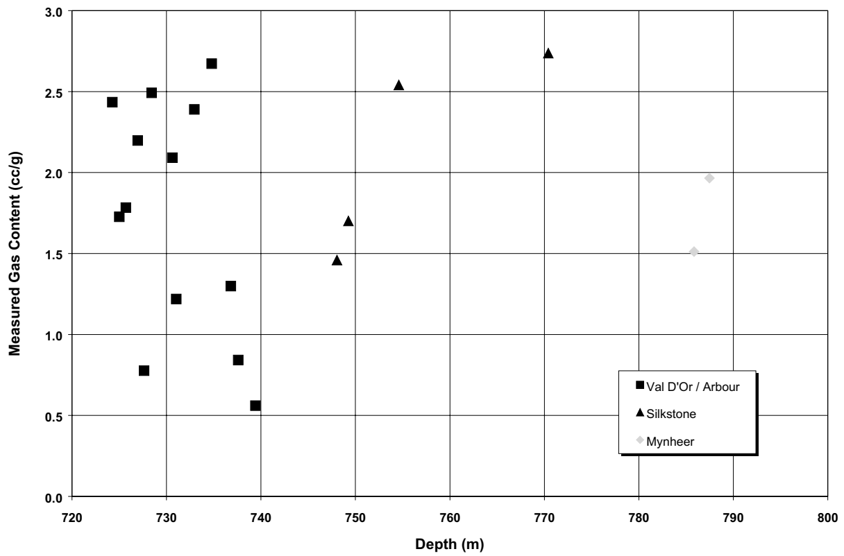
Figure 139. Measured gas content versus depth of intersection, BHP Pine Creek samples.
