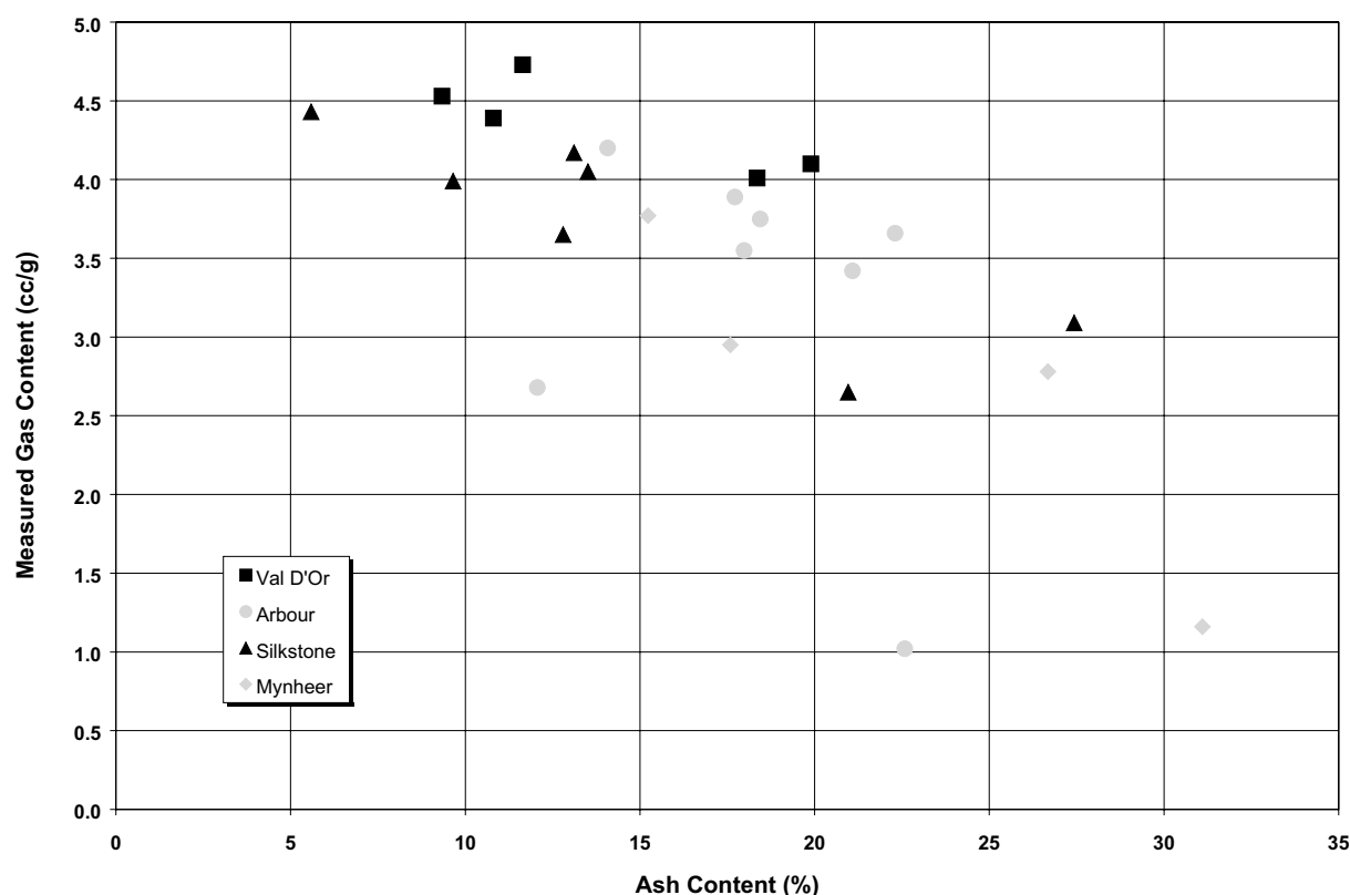
Figure 132. Measured gas content versus ash content (a.d.b.), BHP Pembina samples.
