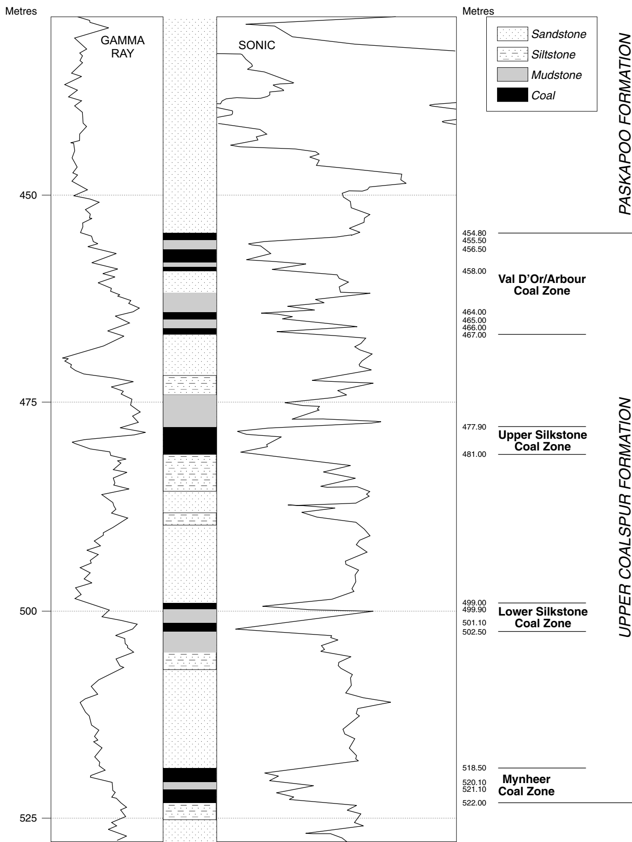
Figure 113. Detailed stratigraphic section of the Coalspur Formation, Norcen Seaforth borehole.
