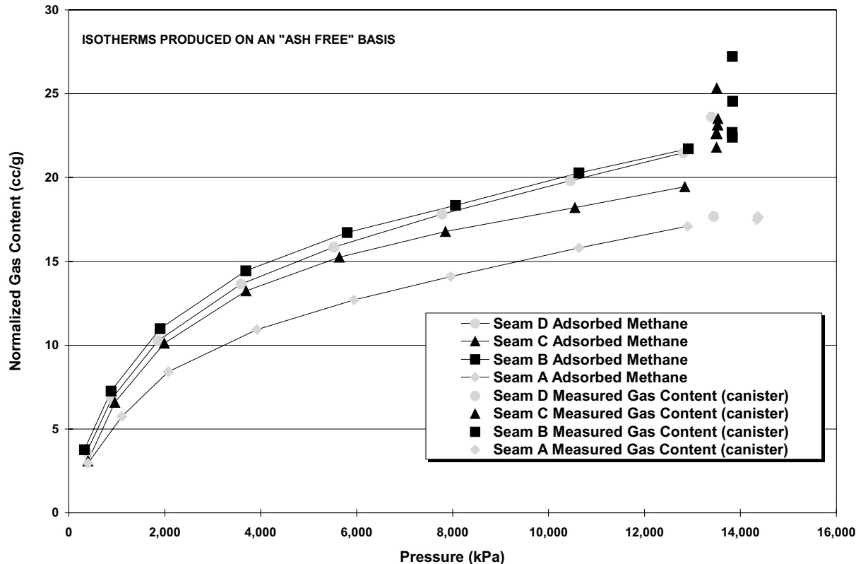
Figure 41. Normalized gas content and adsorption isotherm values for seams A to D on an ash-free equilibrium moisture basis versus pressure gradient (depth x 10.179) for borehole a-21-F.
