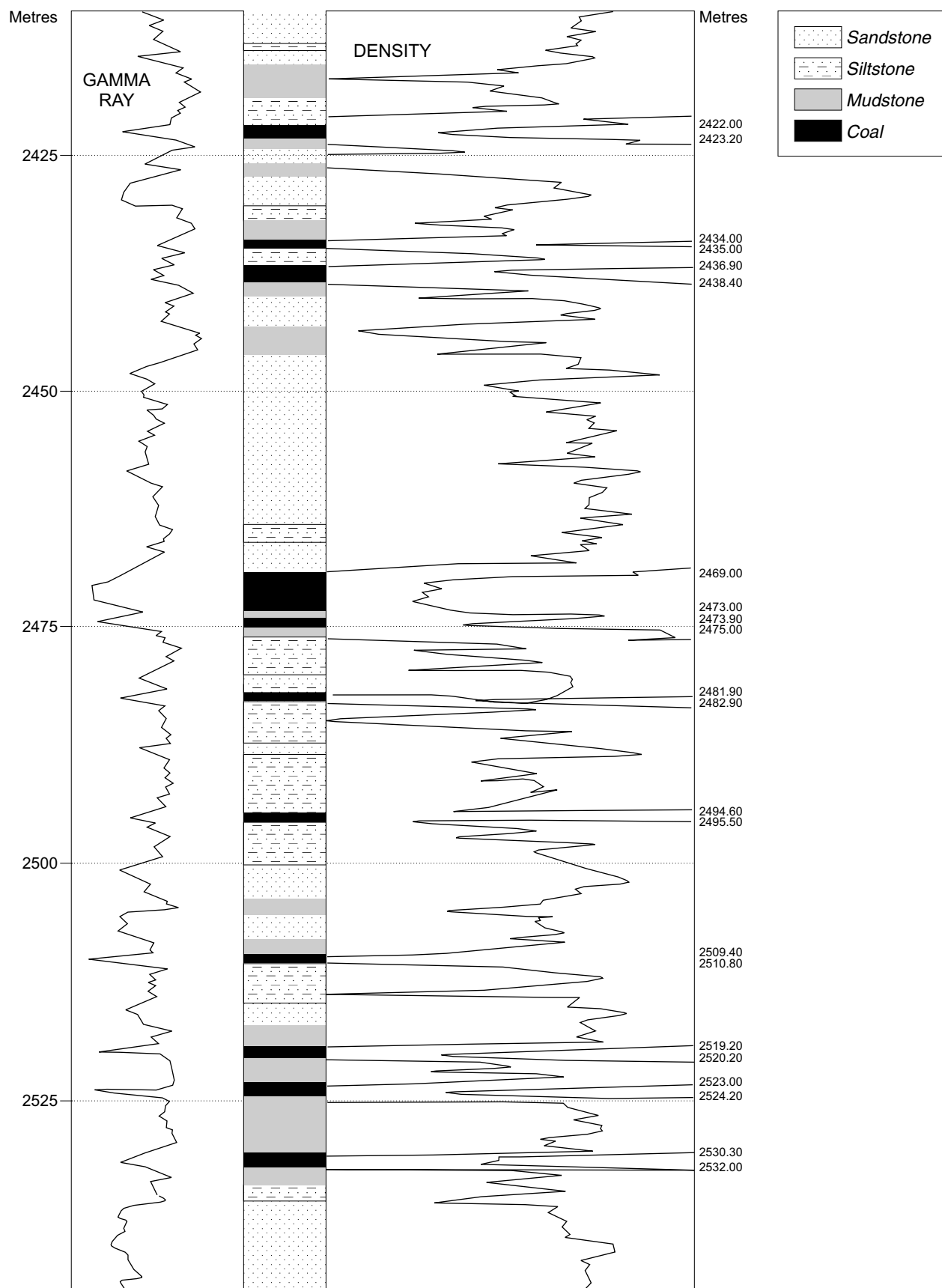
Figure 122. Detailed stratigraphic section of the Norcen Simonette borehole.
