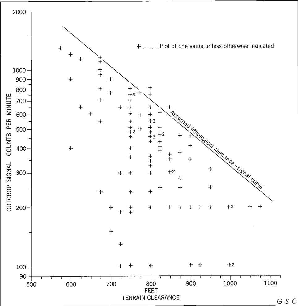
Figure 2. Typical outcrop clearance-signal plot, Read Bay argillaceous limestone.
