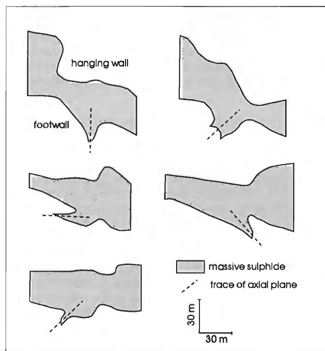
Figure 8. Schematic illustrations of footwall cusps. All sketches are looking north.
