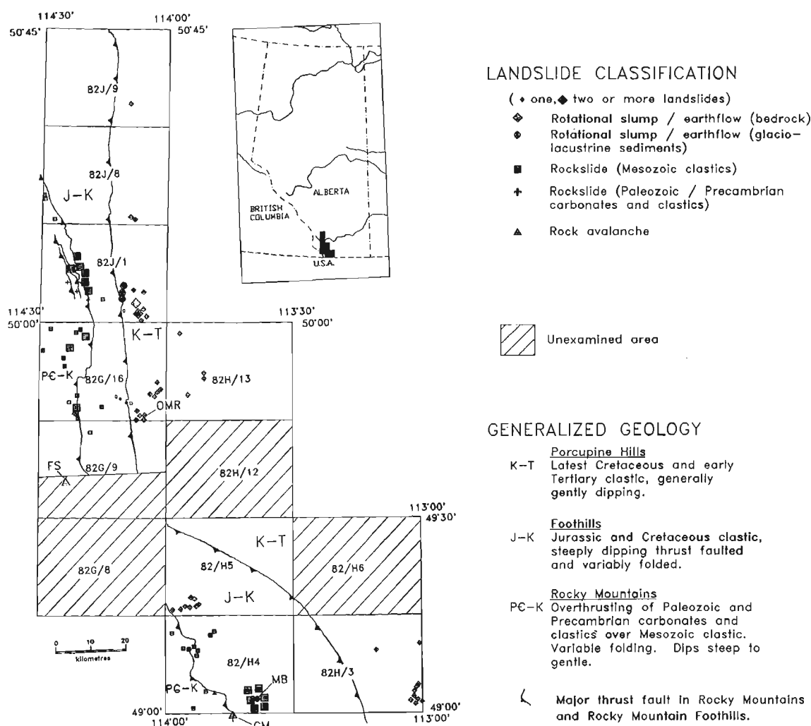
Figure 2. Regional characterization of landslides and associated bedrock/structural provinces. Bedrock geology generalized after Douglas (1950, 1952), Norris (1955, 1958), Okulitch and Woodsworth (1977). Locations: CM- Chief Mountain; FS- Frank Slide; MB- Mokowan Butte; OMR- Oldman River between its confluences with Callum Creek (north end) and Crowsnest River (south end) (particularly active area of slumping involving late Cretaceous bedrock and overlying glaciolacustrine sediments).
