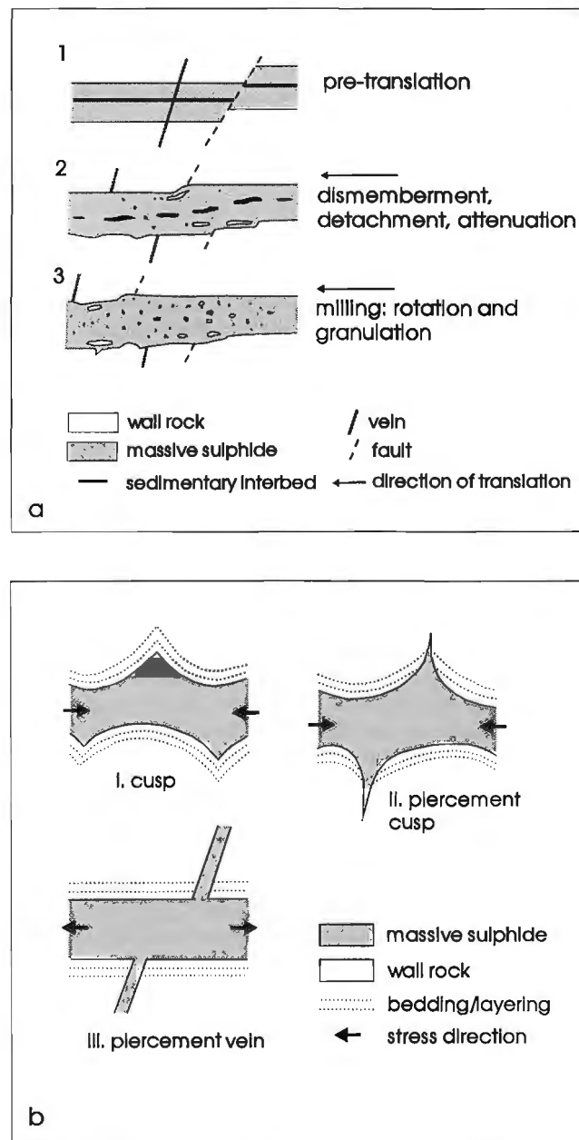
Figure 1. Schematic illustrations of: (a) the development of durchbewegung structure, and (b) piercement structure terminology (after Marshall and Gilligan, 1989).
