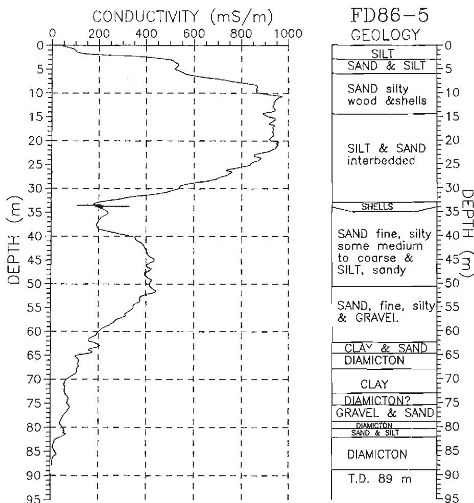
Figure 6. Conductivity and geological logs for borehole FD86-5 (from Hunter et al., 1993).
